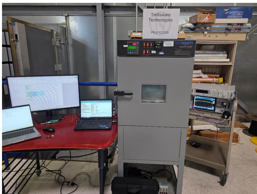
Figure 6 – Test setup (Frequency stability)
