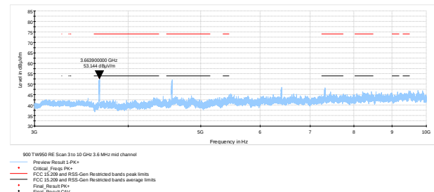
Figure 7.10-31: Radiated spurious emissions on emissions 3-10 GHz Mid channel TW950
