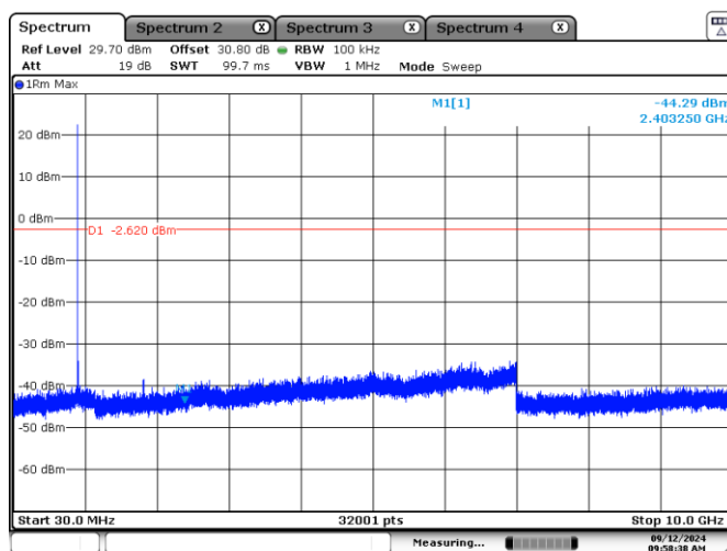
Figure 7.10-16: Conducted spurious emissions on 3.6 MHz High channel
