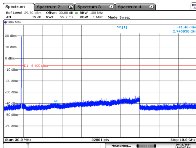
Figure 7.10-19: Conducted spurious emissions on 10 MHz High channel
