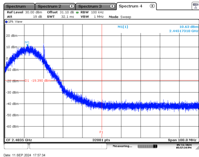
Figure 7.6-8: Band edge spurious emissions at 2483.5 MHz 20 MHz
