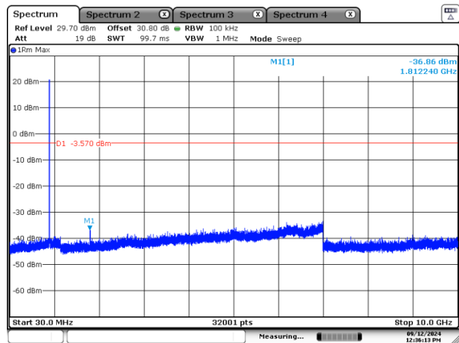
Figure 7.10-18: Conducted spurious emissions on 10 MHz Mid channel
