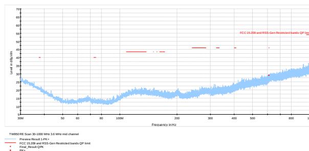
Figure 7.6-25: Radiated spurious emissions 30-1000 MHz
