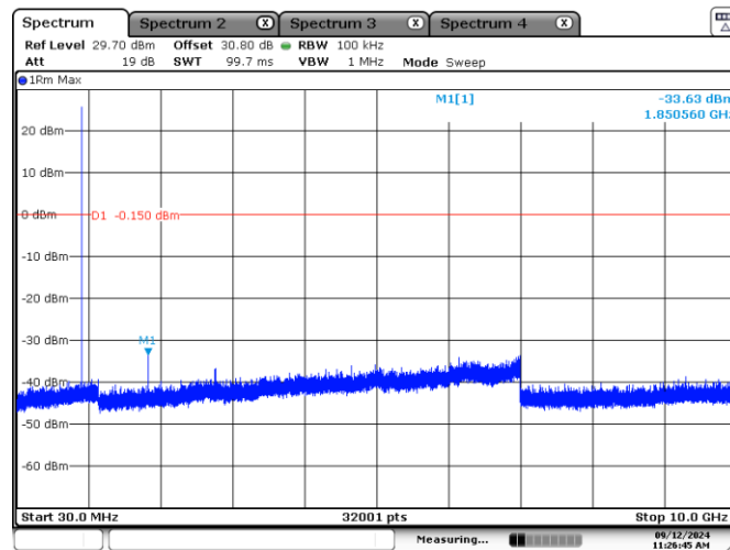
Figure 7.10-13: Conducted spurious emissions on 1.3 MHz High channel
