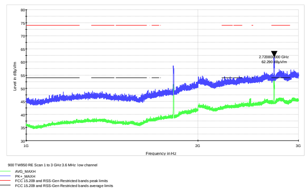
Figure 7.10-27: Radiated spurious emissions on emissions 1-3 GHz Low channel TW-950
