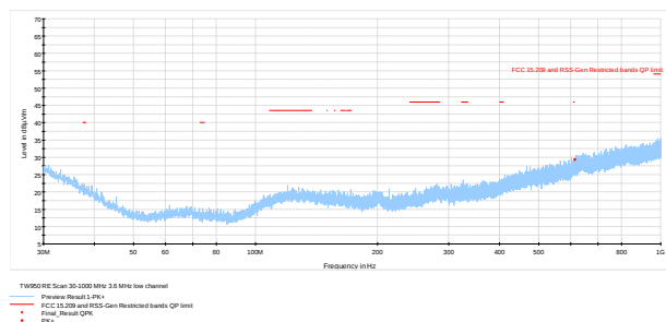
Figure 7.6-24: Radiated spurious emissions on 30-1000 MHz
