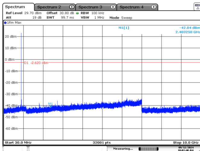
Figure 7.10-15: Conducted spurious emissions on 3.6 MHz Mid channel
