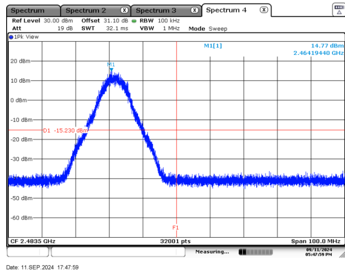
Figure 7.6-6: Band edge spurious emissions at 2483.5 MHz 10 MHz
