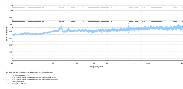
Figure 7.6-27: Radiated spurious emissions on emissions 1-18 GHz
