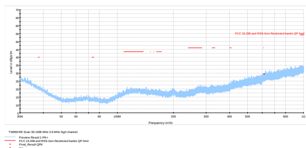
Figure 7.6-26: Radiated spurious emissions 30-1000 MHz
