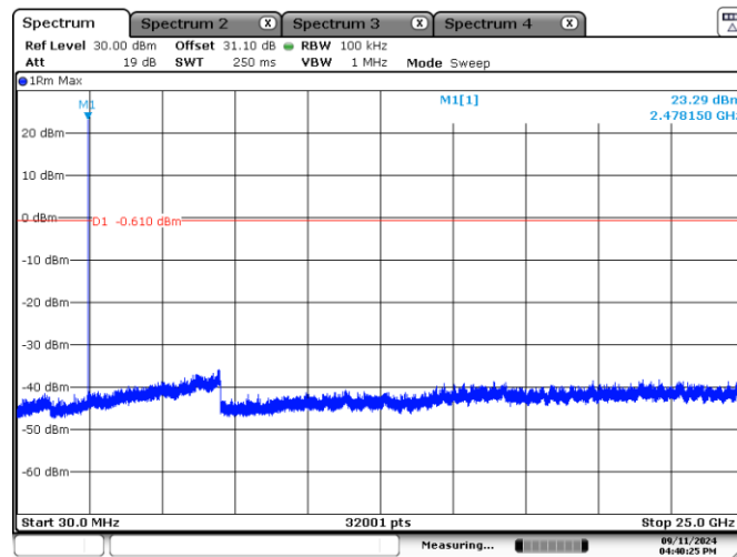
Figure 7.6-13: Conducted spurious emissions on 1.2 MHz High channel
