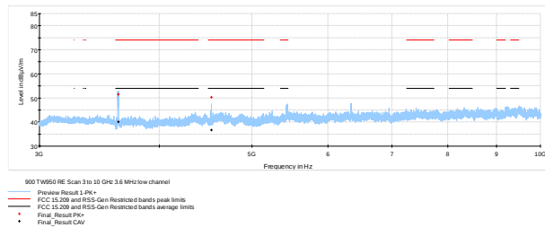
Figure 7.10-30: Radiated spurious emissions 3-10 GHz Low channel TW-950
