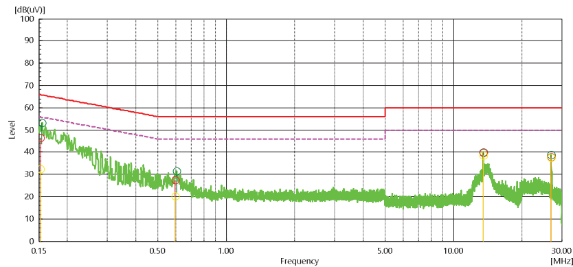
Figure 5: Conducted Emission on AC Mains Port, Spectral Diagram, 0.15 - 30MHz, Phase N (N), Mode A
