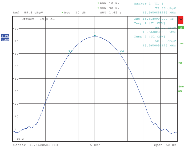
Figure 3: 99% Bandwidth, Mode A
