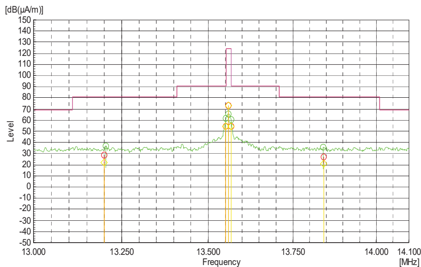
Figure 4: Field Strength of Fundamental, Spectral Diagram, Mode A
