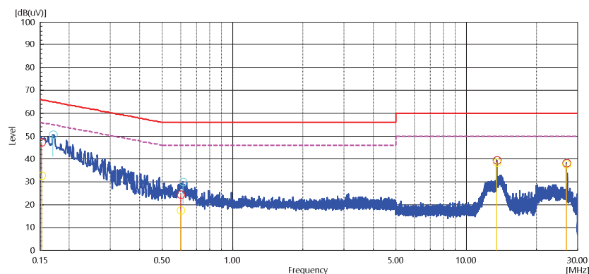
Figure 6: Conducted Emission on AC Mains Port, Spectral Diagram, 0.15 - 30MHz, Phase L1 (L), Mode A
