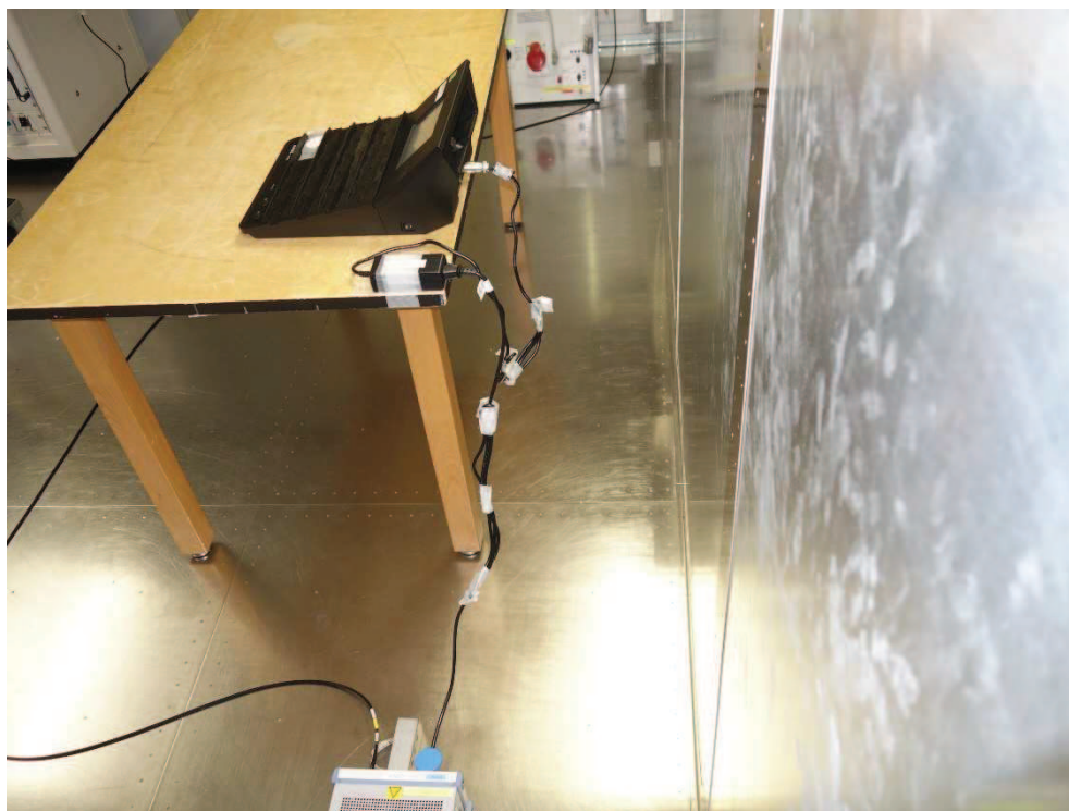
Photograph 7: Set-up for AC Power Line Conducted Emission of Transmitter, Rear View
