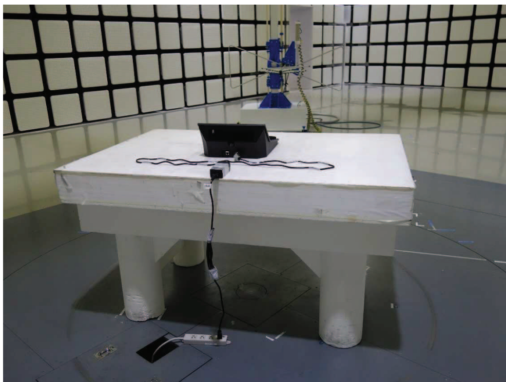
Photograph 11: Set-up for Radiated Emission of Transmitter, Rear View
