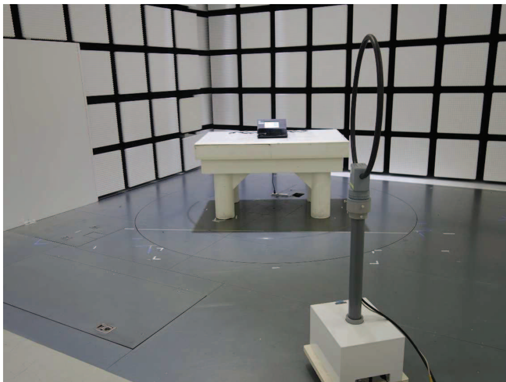
Photograph 8: Set-up for Radiated Emission of Transmitter Below 30MHz, Front View
