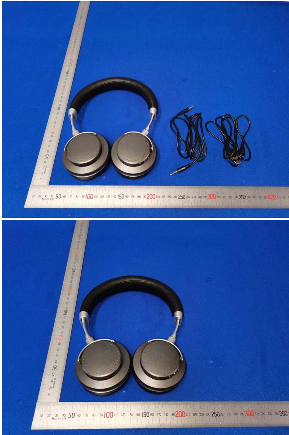
Outside View-BL-005
