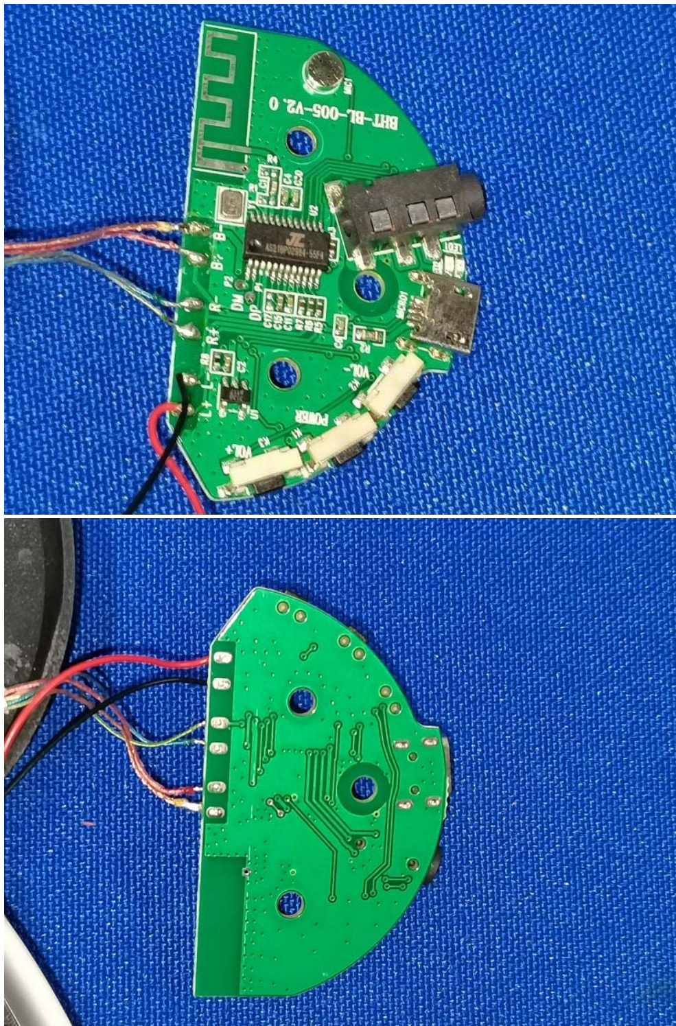
Inside View-BL-005
