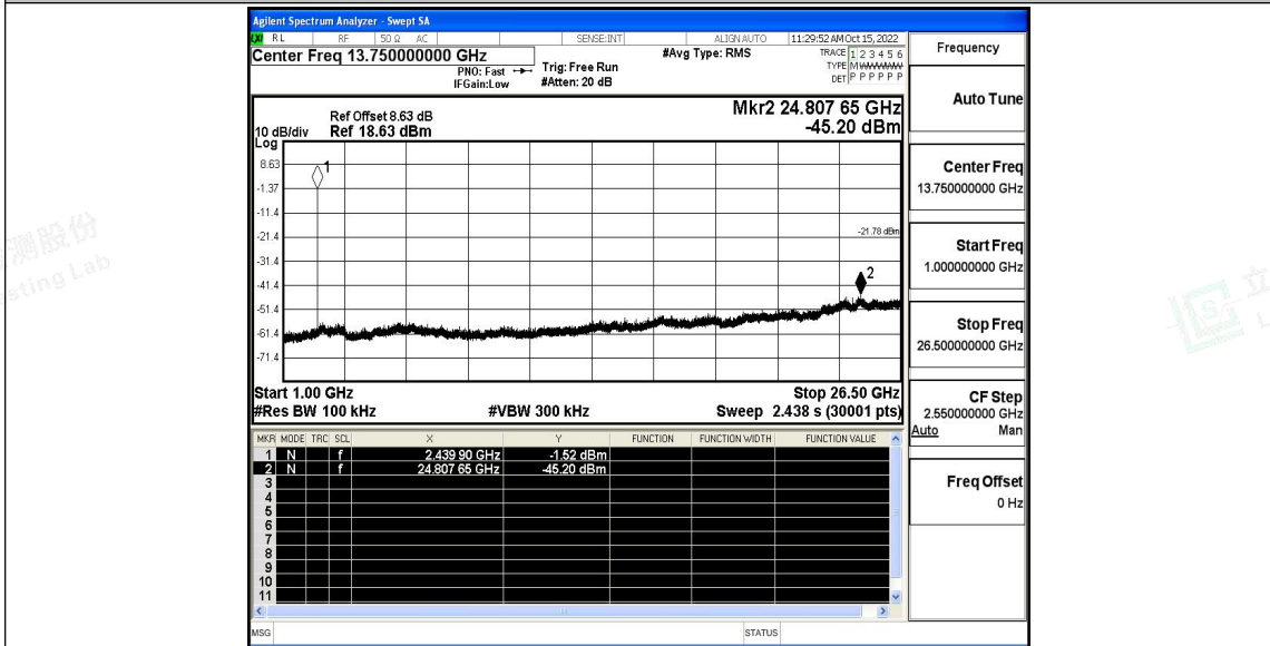
BLE_1M_Ant1_2480_0~Reference
