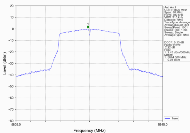
802.11a_HCH_5825MHz_Ant1_NTNV
