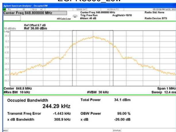
EGPRS850_High
