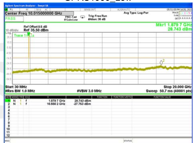
GPRS1900_Middle
