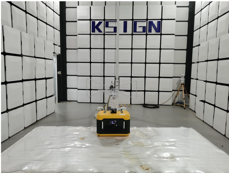
Radiated Measurement (Above 30MHz)
