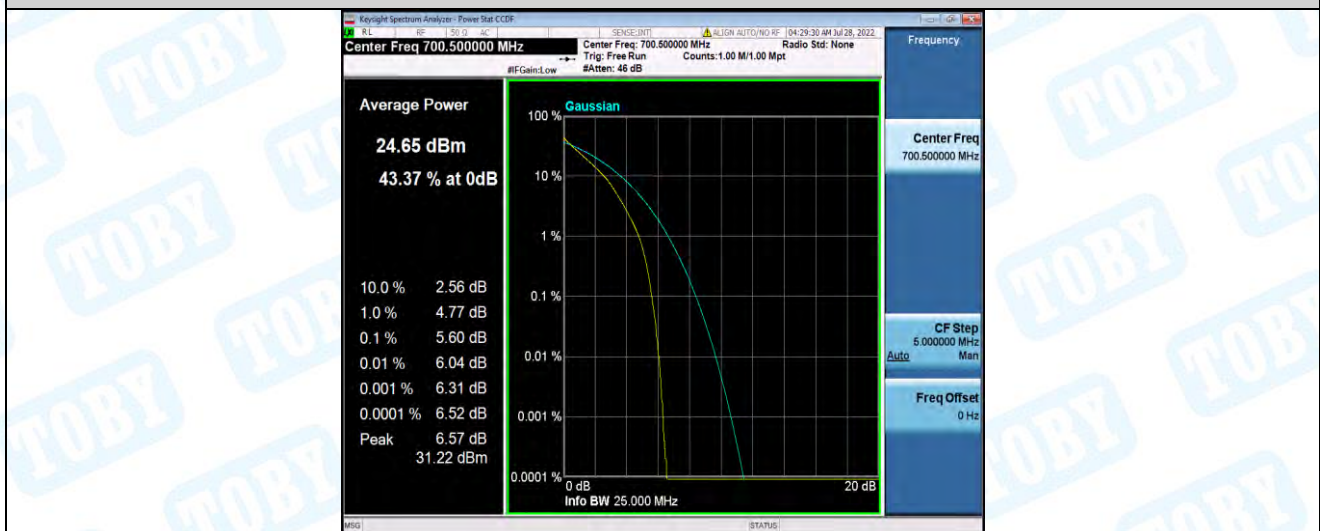
Band12-3MHz-QPSK-23095-1RB#0
