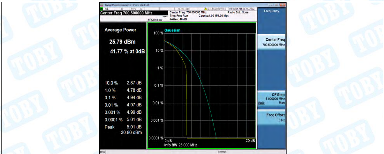
Band12-3MHz-QPSK-23025-15RB#0
