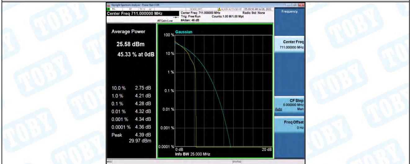
Band12-10MHz-QPSK-23130-50RB#0
