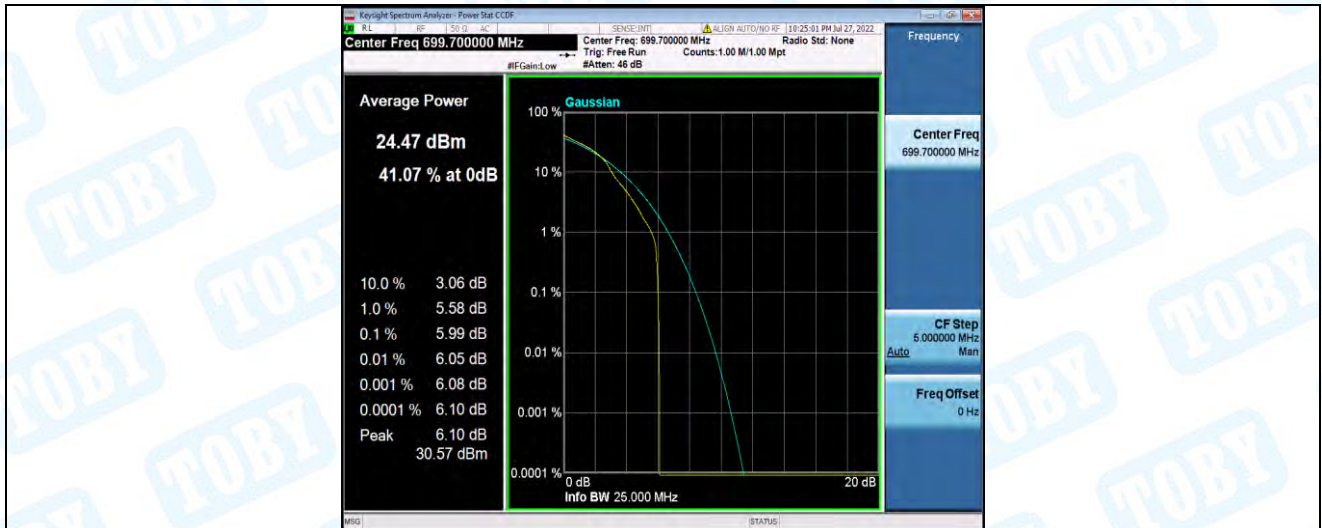
Band12-1.4MHz-16QAM-23017-6RB#0
