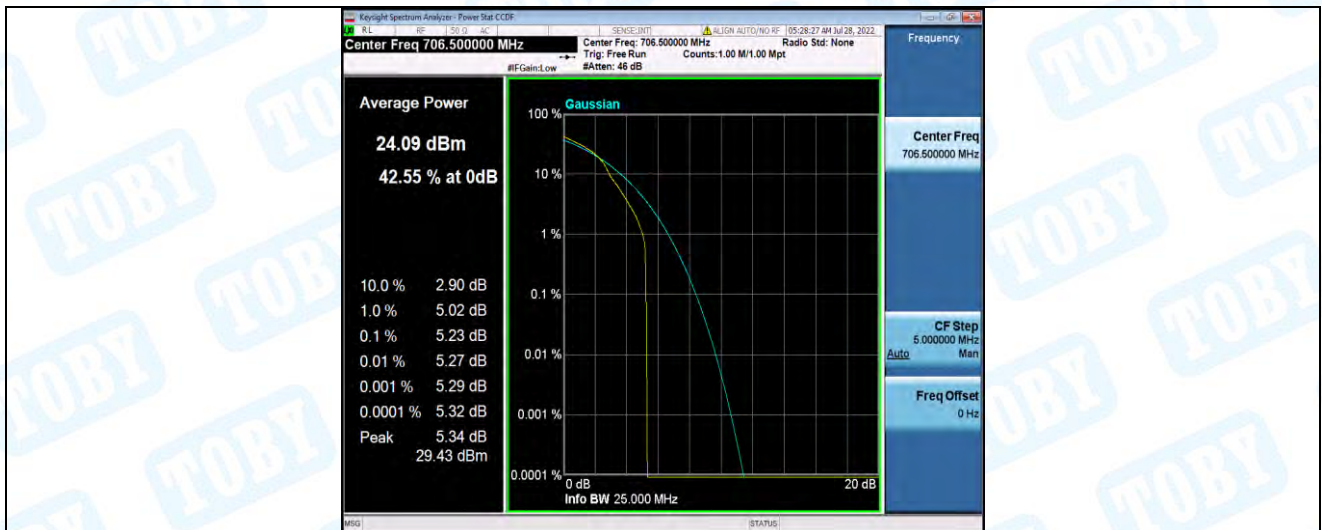
Band17-5MHz-16QAM-23755-25RB#0
