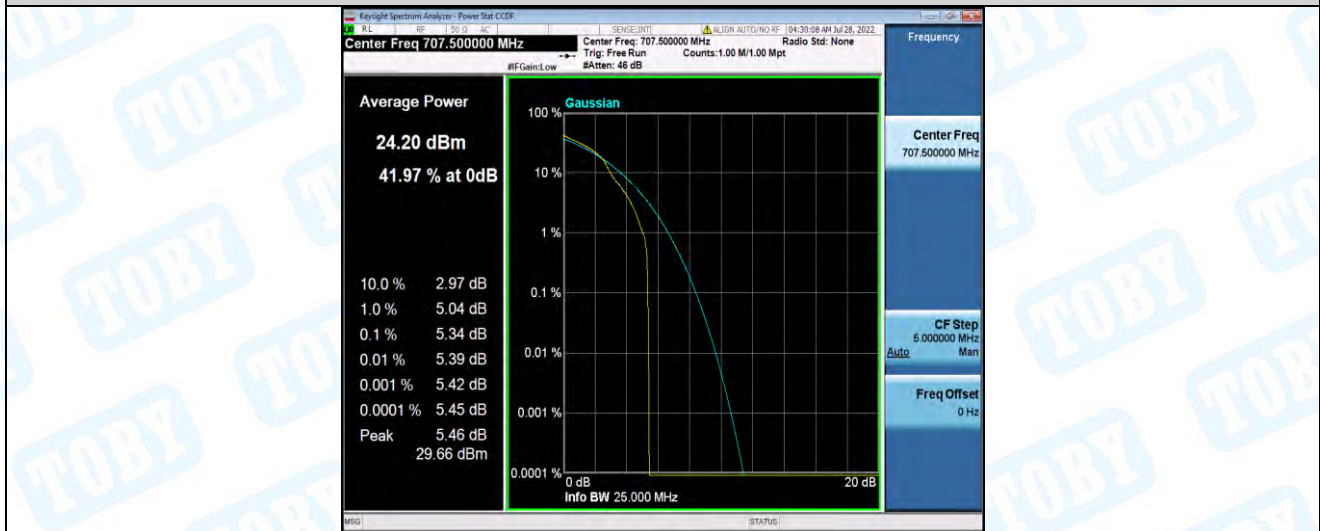
Band12-3MHz-16QAM-23095-15RB#0
