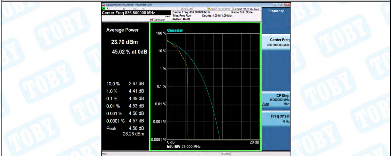
Band5-10MHz-QPSK-20525-50RB#0
