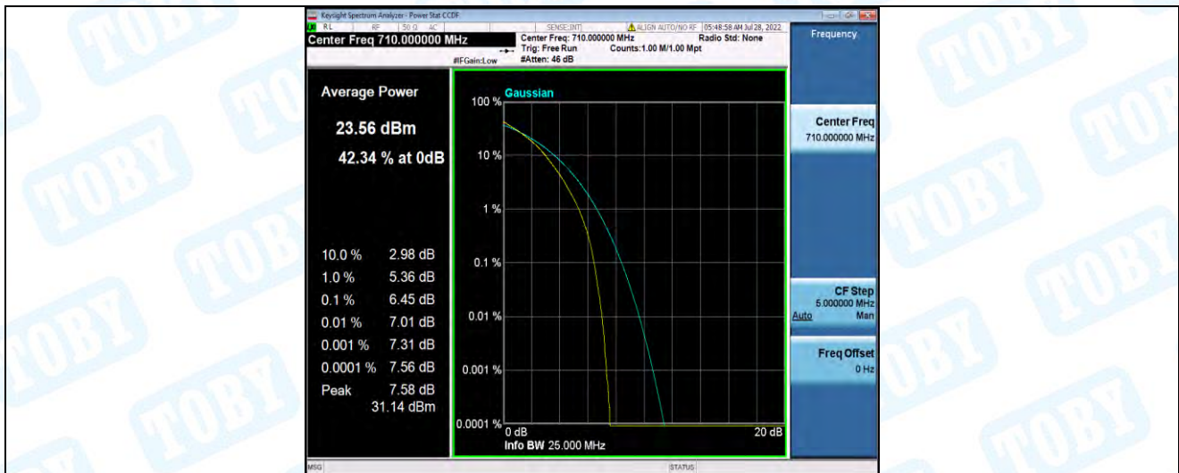
Band17-10MHz-16QAM-23800-1RB#0
