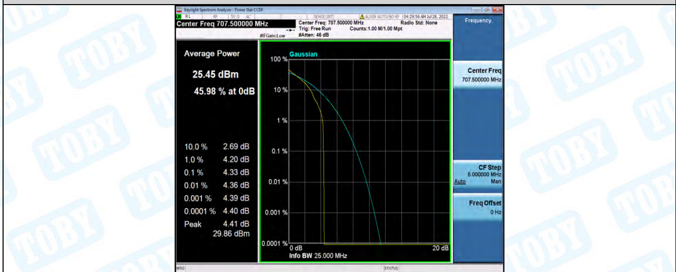
Band12-3MHz-QPSK-23095-15RB#0
