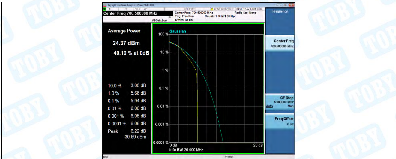
Band12-3MHz-16QAM-23025-15RB#0
