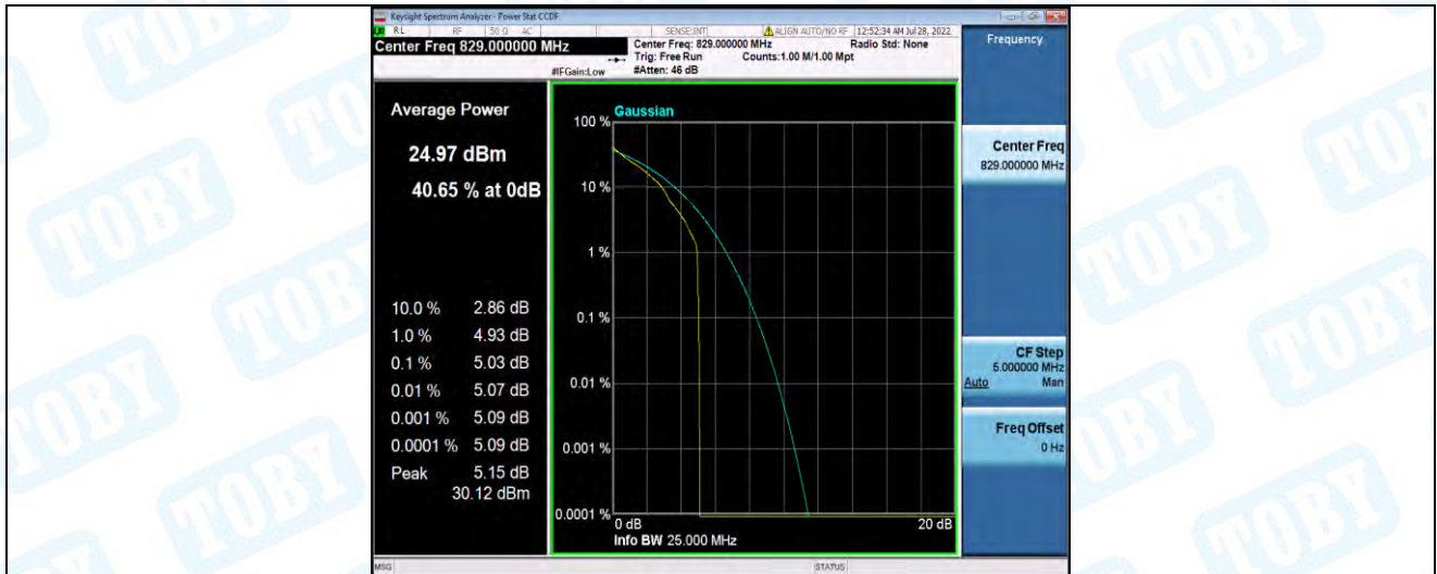
Band5-10MHz-QPSK-20450-50RB#0
