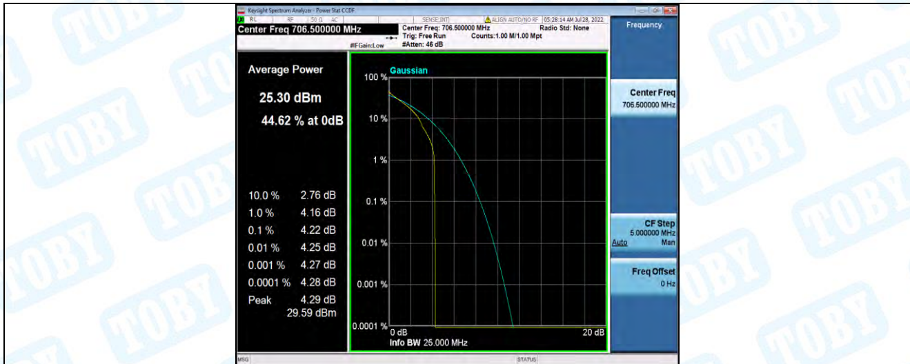
Band17-5MHz-QPSK-23755-25RB#0
