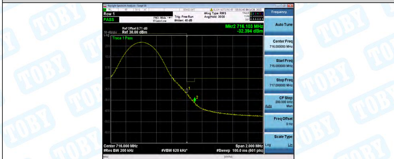
Band12-10MHz-16QAM-23130-50RB#0
