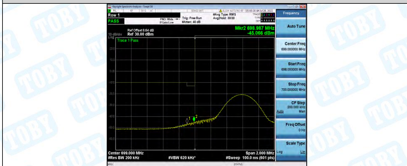
Band12-10MHz-16QAM-23060-50RB#0
