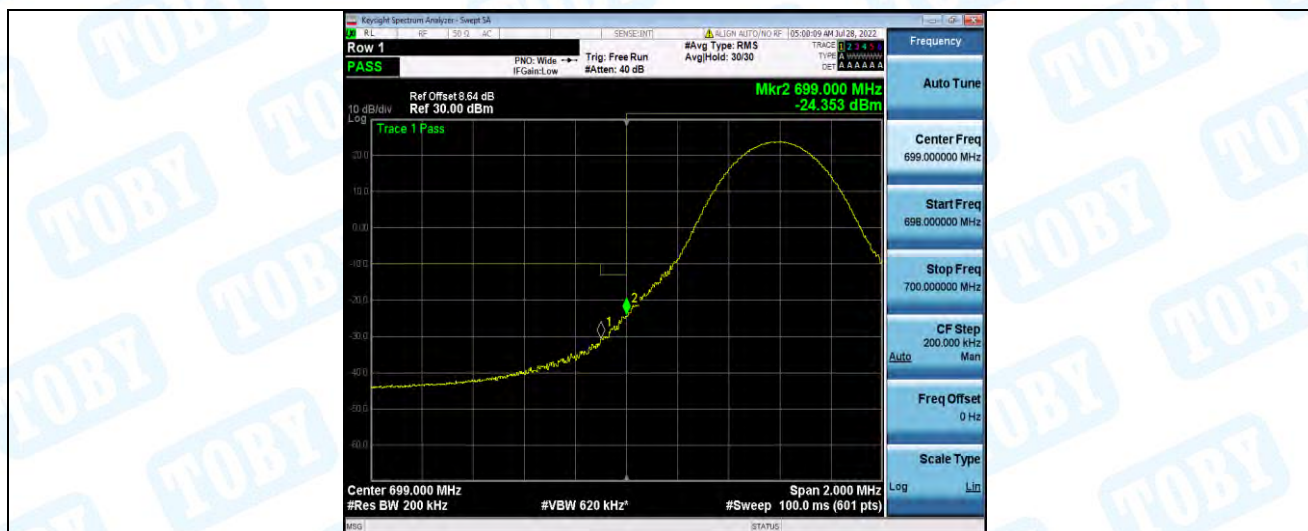
Band12-10MHz-16QAM-23060-1RB#49
