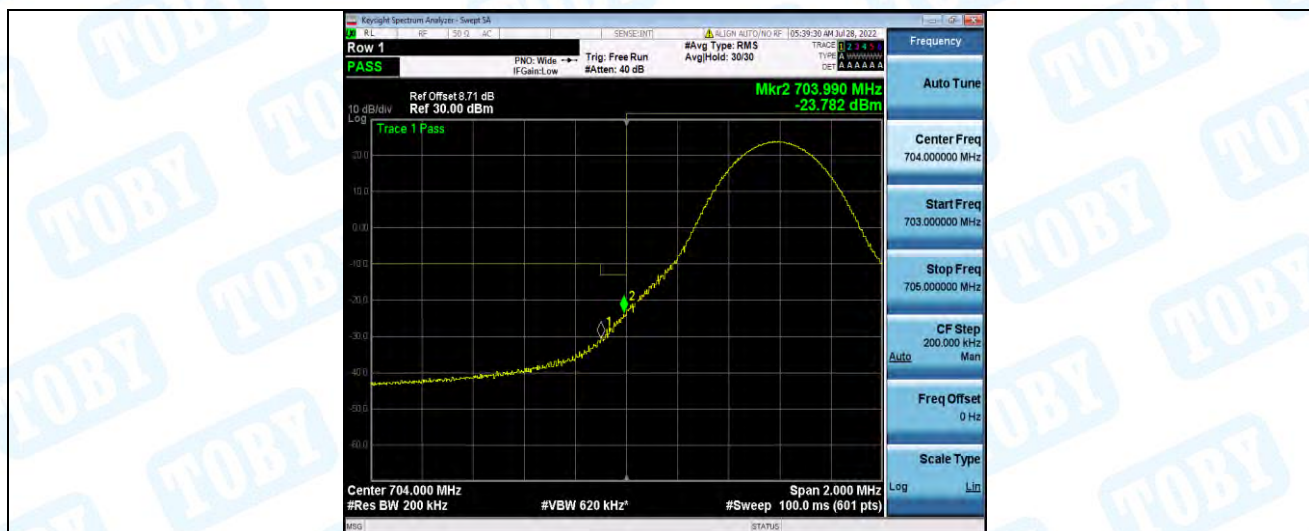
Band17-10MHz-16QAM-23780-1RB#49
