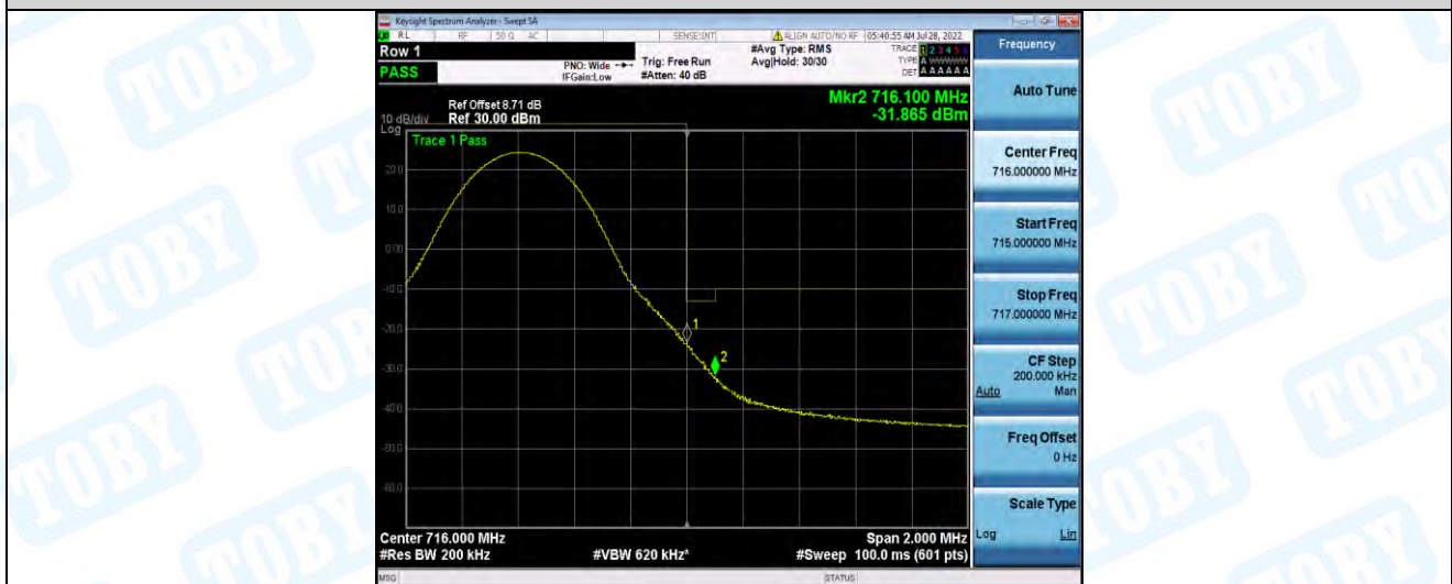
Band17-10MHz-QPSK-23800-50RB#0
