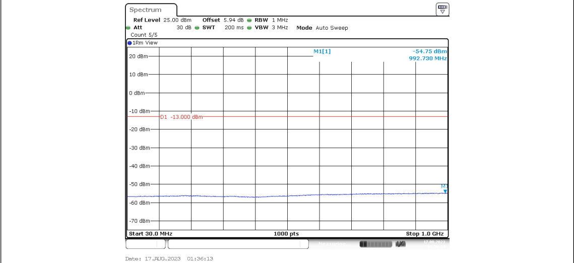
Band4-Stand-Alone-NaN-QPSK-20399-1@47-3.75kHz-30-1000--54.75--13-PASS
