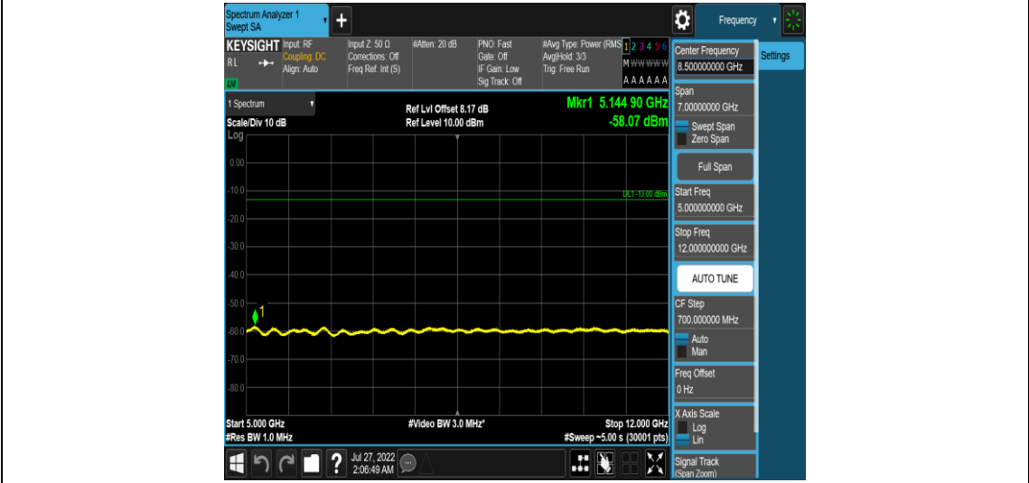
Band13-Stand-Alone-NaN-BPSK-23230-1@0-15kHz-5000-12000-5000~12000MHz@-58.07dB Bm--13-PASS
