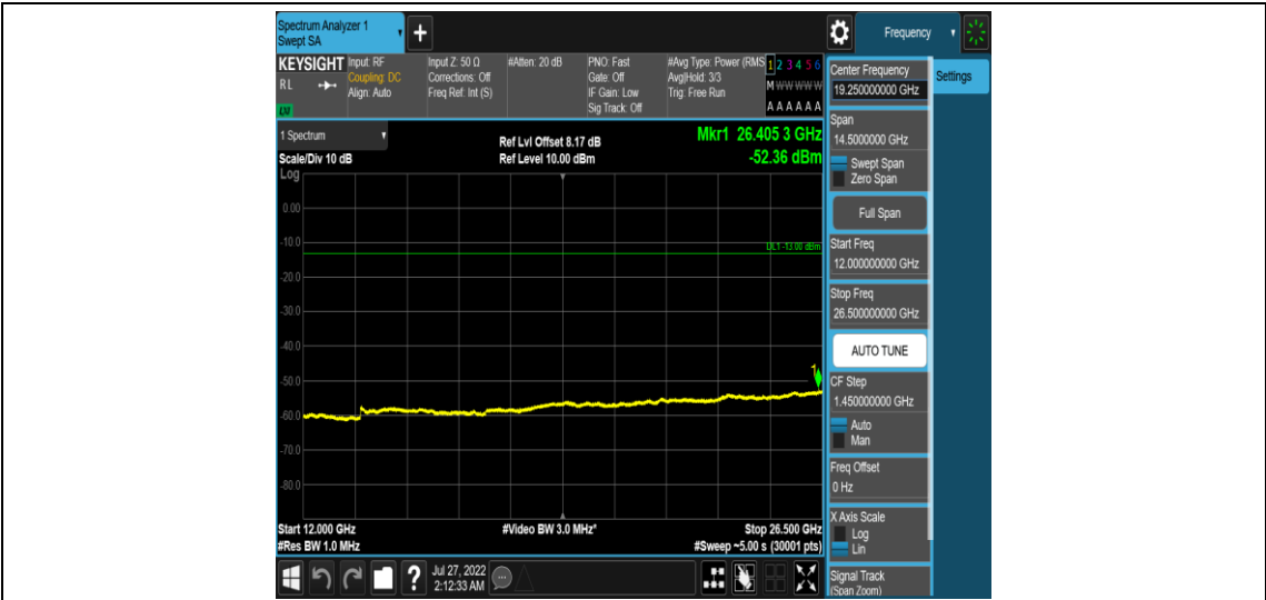
Band13-Stand-Alone-NaN-BPSK-23279-1@11-15kHz-12000-26500-12000~26500MHz@-52.36dBm--13-PASS
