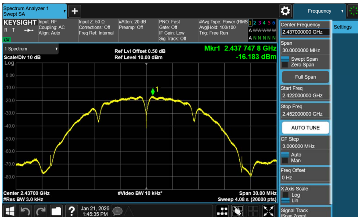
Figure 11: Power Spectral Density, 802.11b, 2437MHz
