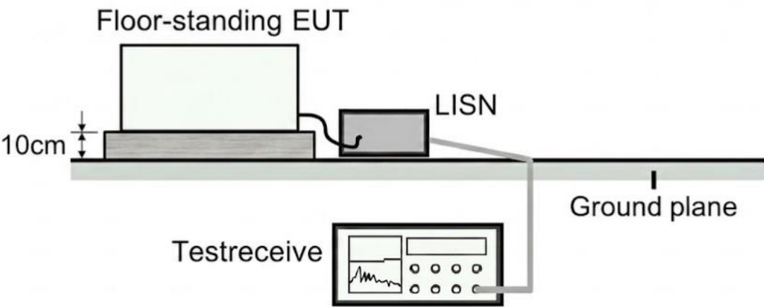
Diagram of Measurement Equipment Configuration for Conduction Measurement (Floor-standing)
