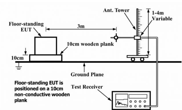
Diagram of Measurement Configuration for Radiation Test 30MHz-1000MHz (Floor-standing)
