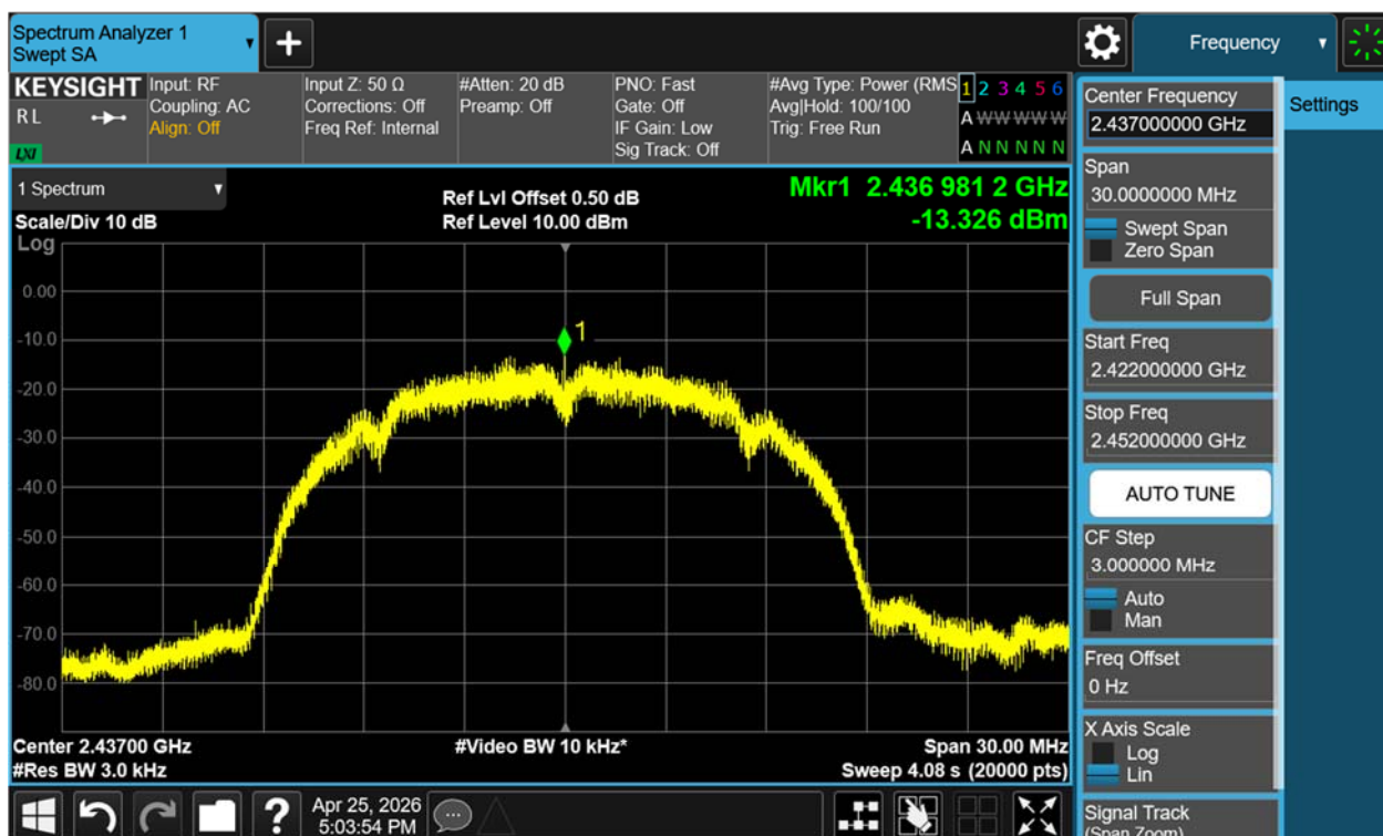
Figure 18: Power Spectral Density, 802.11b, 2437MHz
