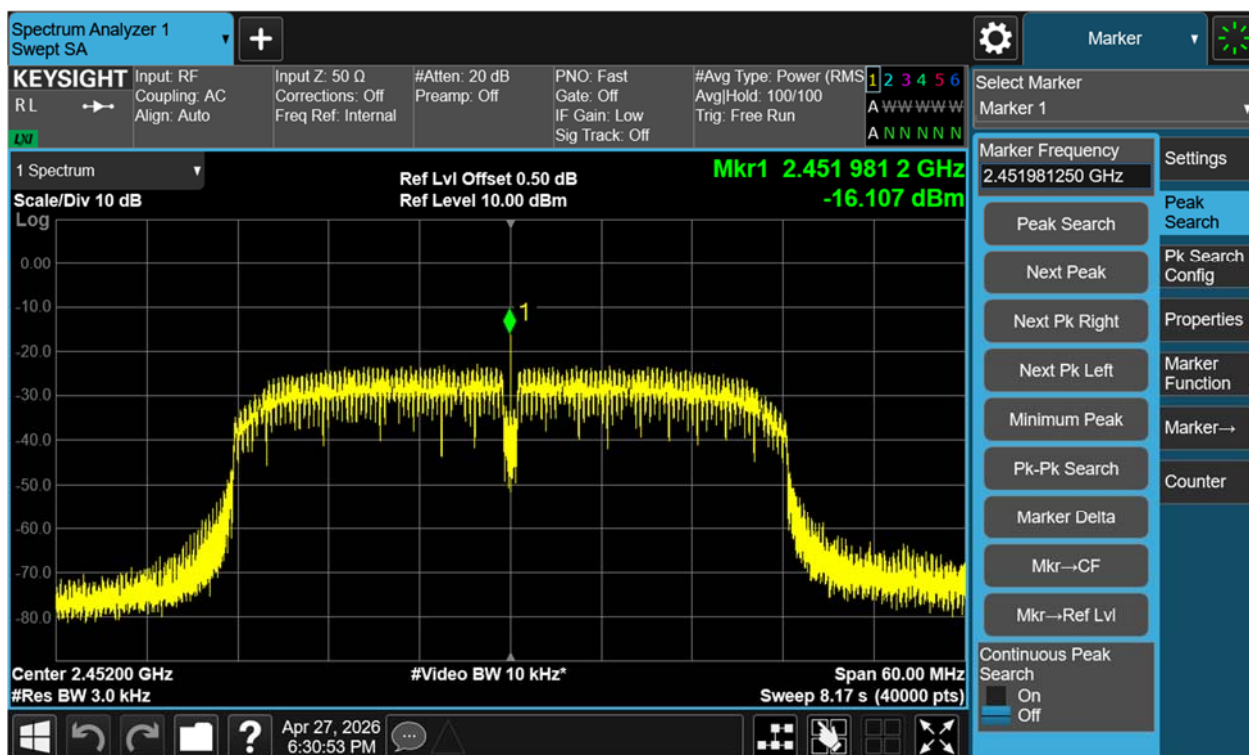
Figure 28: Power Spectral Density, 802.11n(HT40), 2452MHz
