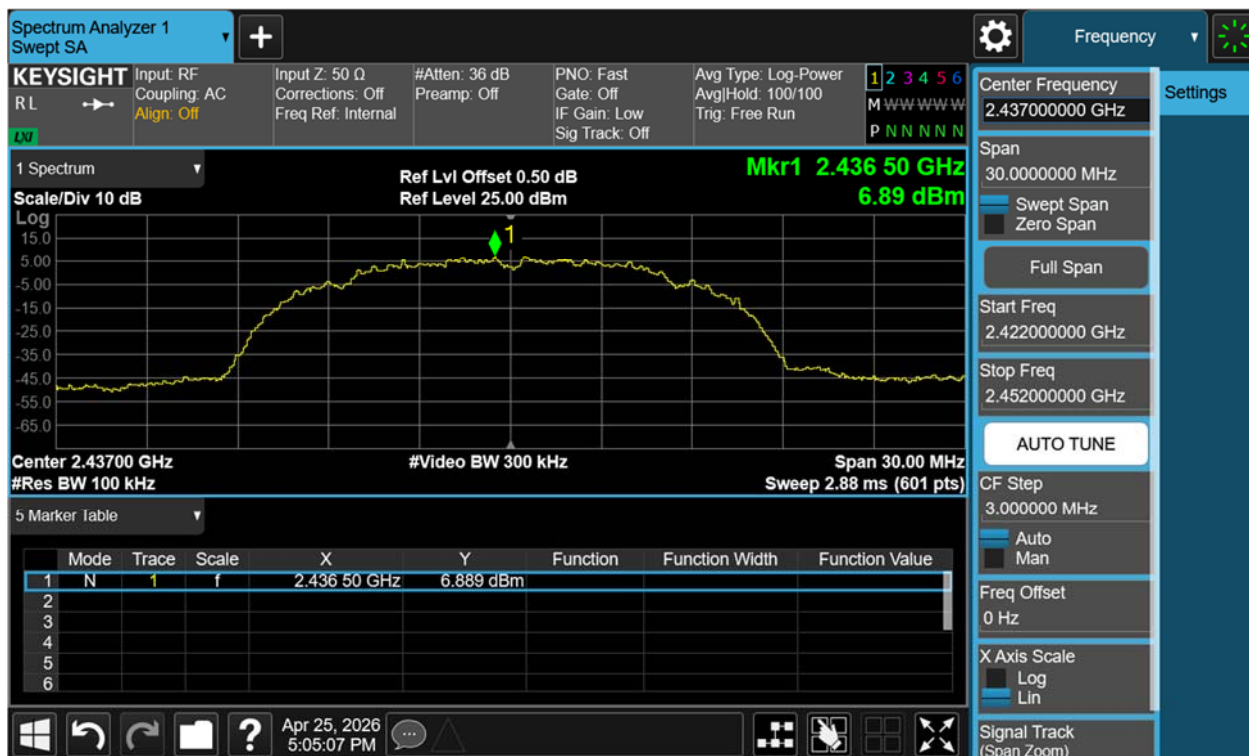
Figure 30: Conducted Spurious Emission & Authorized-band band-edge, 802.11b, 2437MHz Carrier Level
