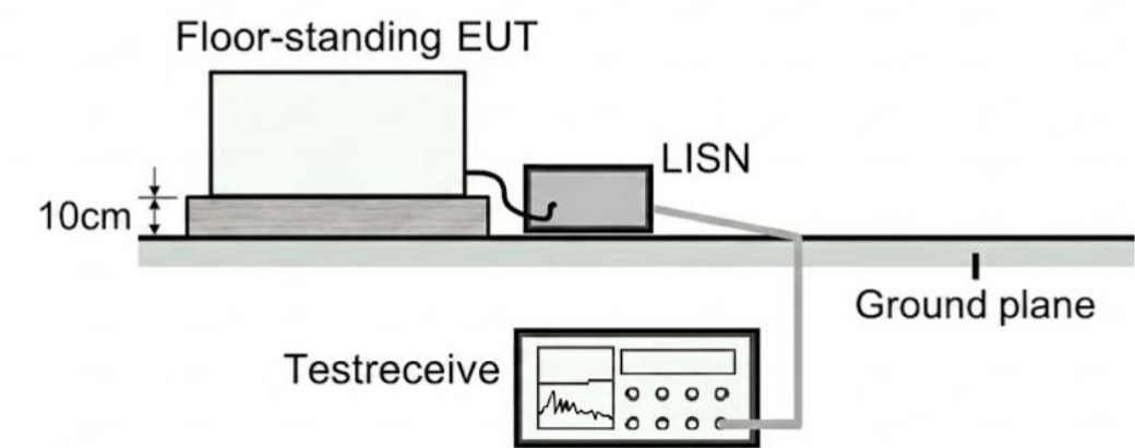
Diagram of Measurement Equipment Configuration for Conduction Measurement (Floor-standing)
