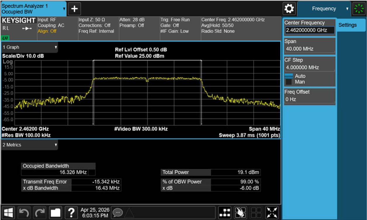
Figure 10: 6dB Bandwidth, 802.11g, 2462MHz
