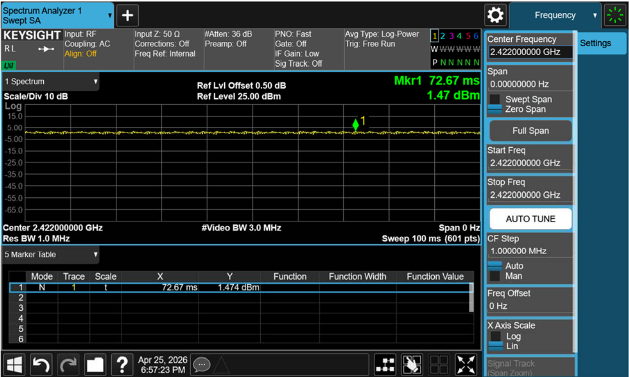
Figure 4: 802.11n40_Duty Cycle Plot
