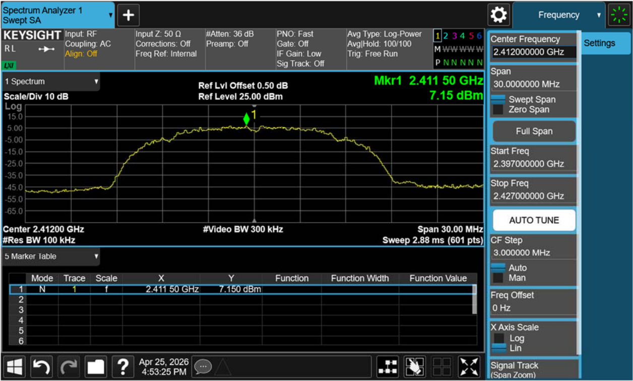
Figure 29: Conducted Spurious Emission & Authorized-band band-edge, 802.11b, 2412MHz Carrier Level
