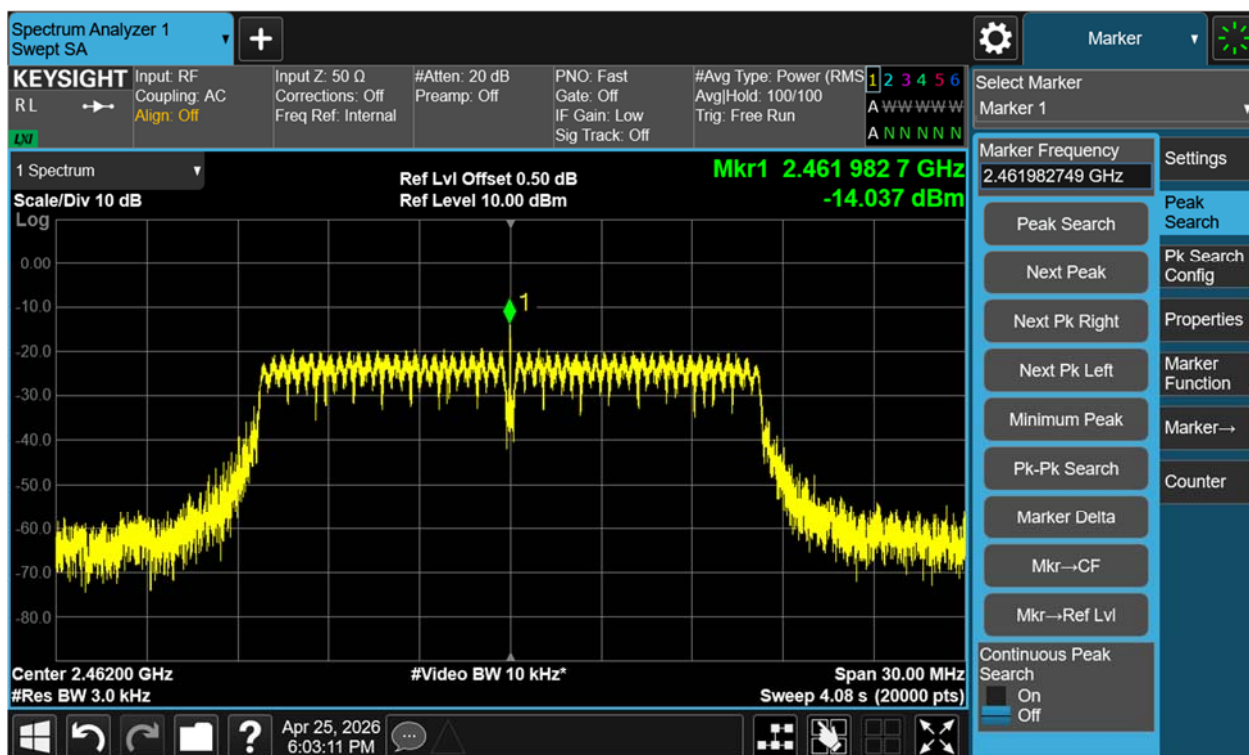
Figure 22: Power Spectral Density, 802.11g, 2462MHz
