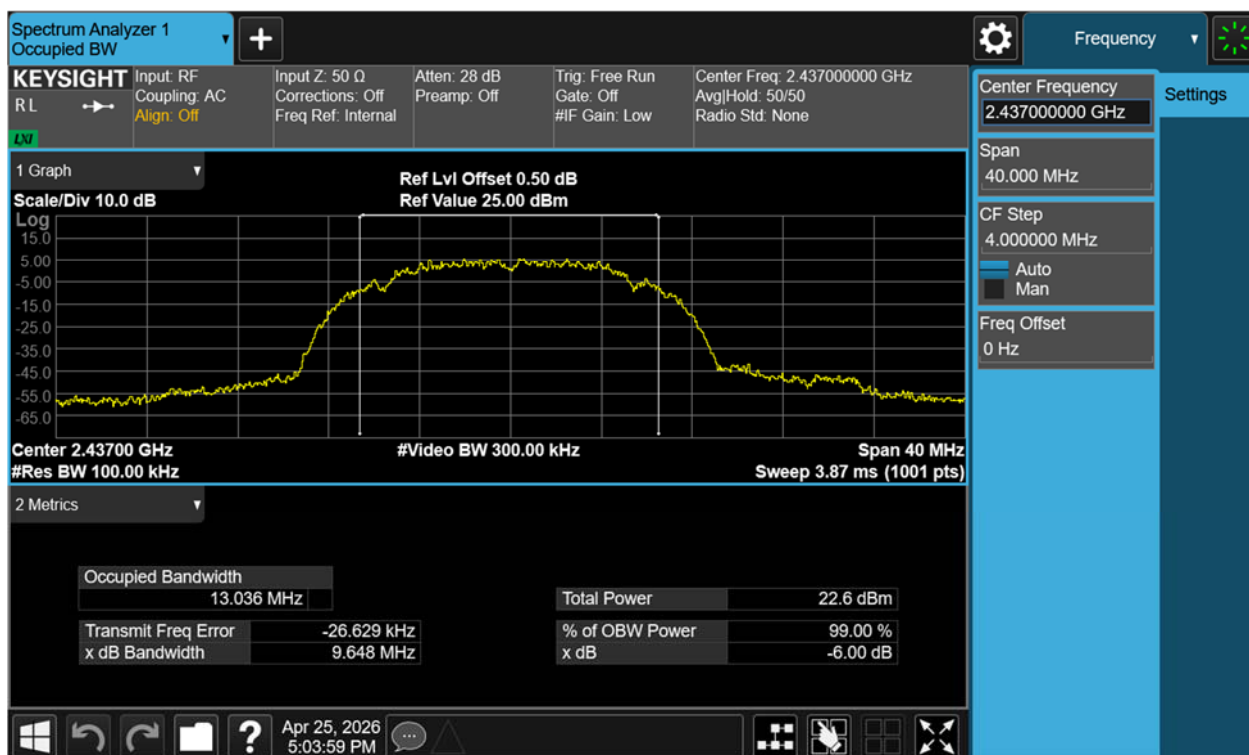
Figure 6: 6dB Bandwidth, 802.11b, 2437MHz
