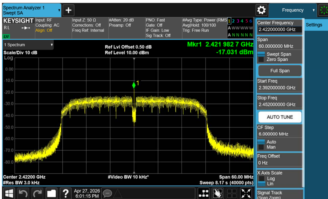
Figure 26: Power Spectral Density, 802.11n(HT40), 2422MHz
