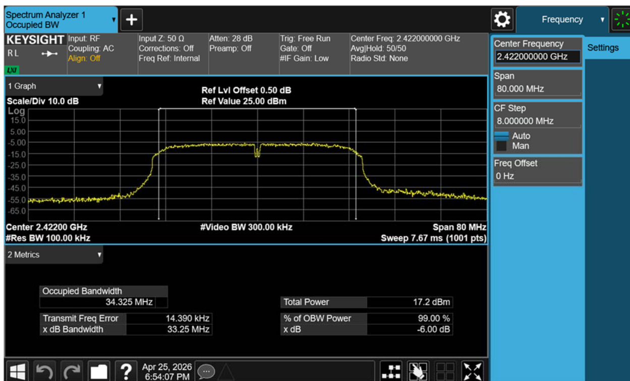
Figure 14: 6dB Bandwidth, 802.11n(HT40), 2422MHz
