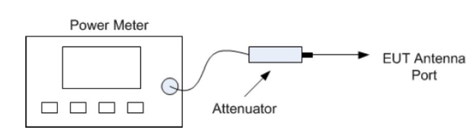
Diagram of Measurement Equipment Configuration for conducted output power setup
