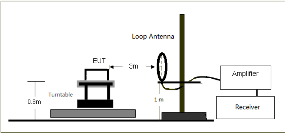
Diagram of Measurement Configuration for Radiation Test Below 30MHz
