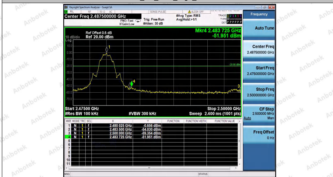
BLE_2M_Ant1_High_2480
