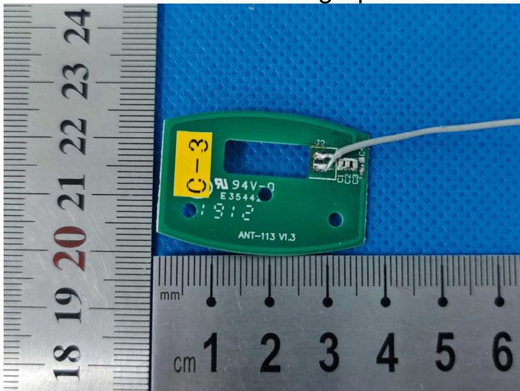
Antenna Photograph
