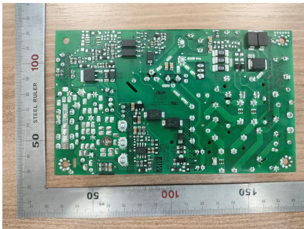
Photo 16: power supply
