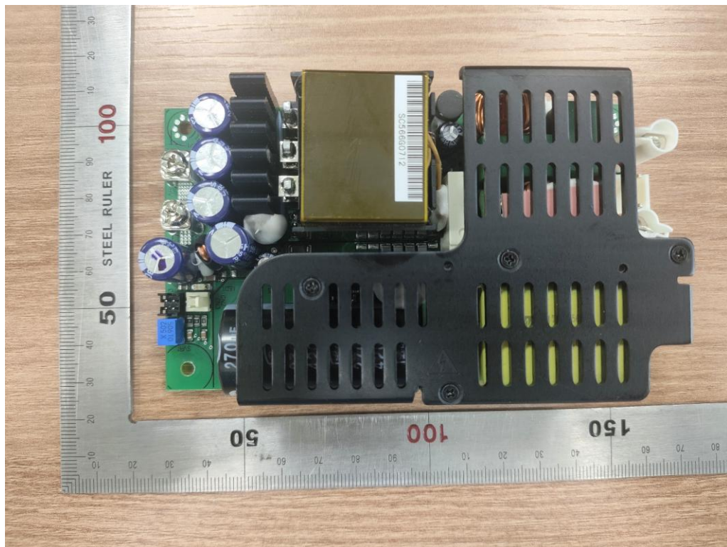
Photo 15: power supply
