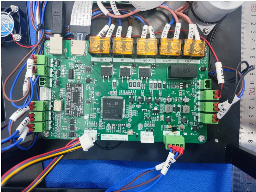
Photo 13: internal view
