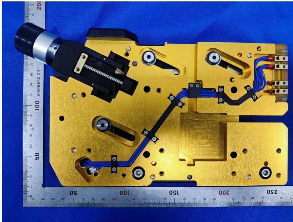
Photo 31: internal view of the single channel carrier
