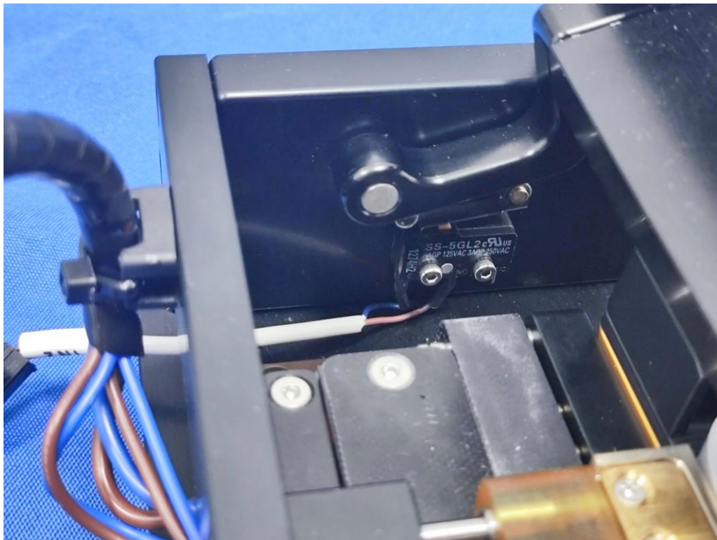
Photo 21: internal view
