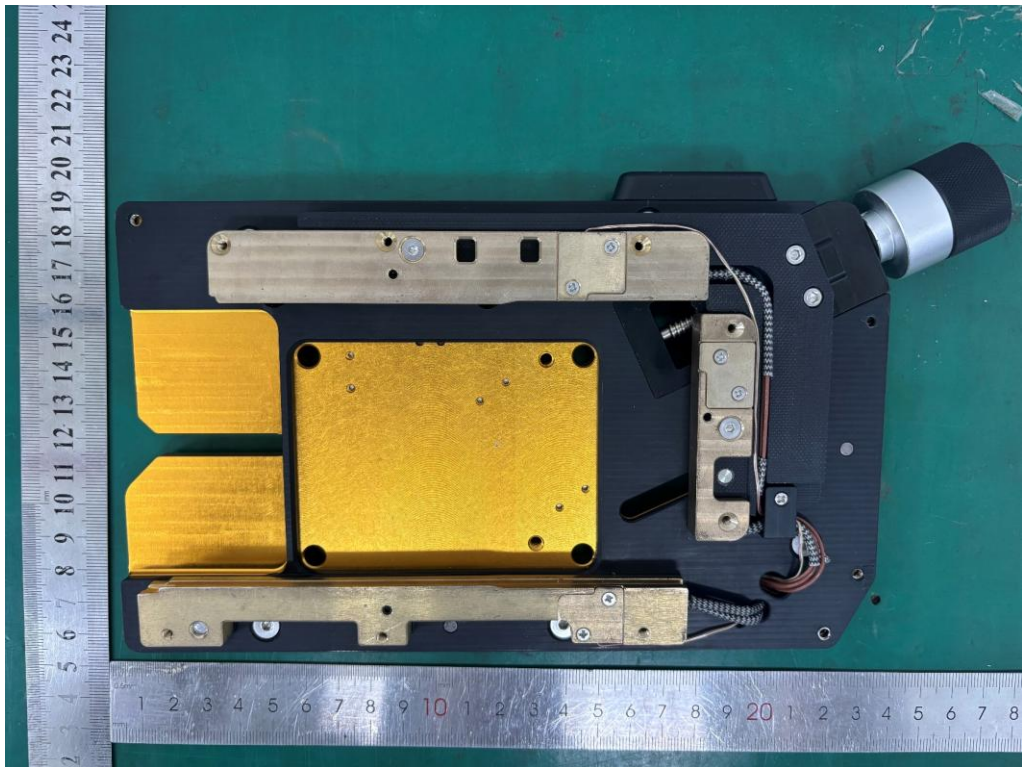
Photo 29: internal view of the dual channel carrier
