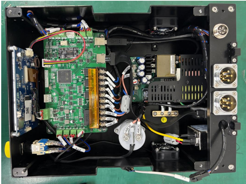
Photo 11: internal view
