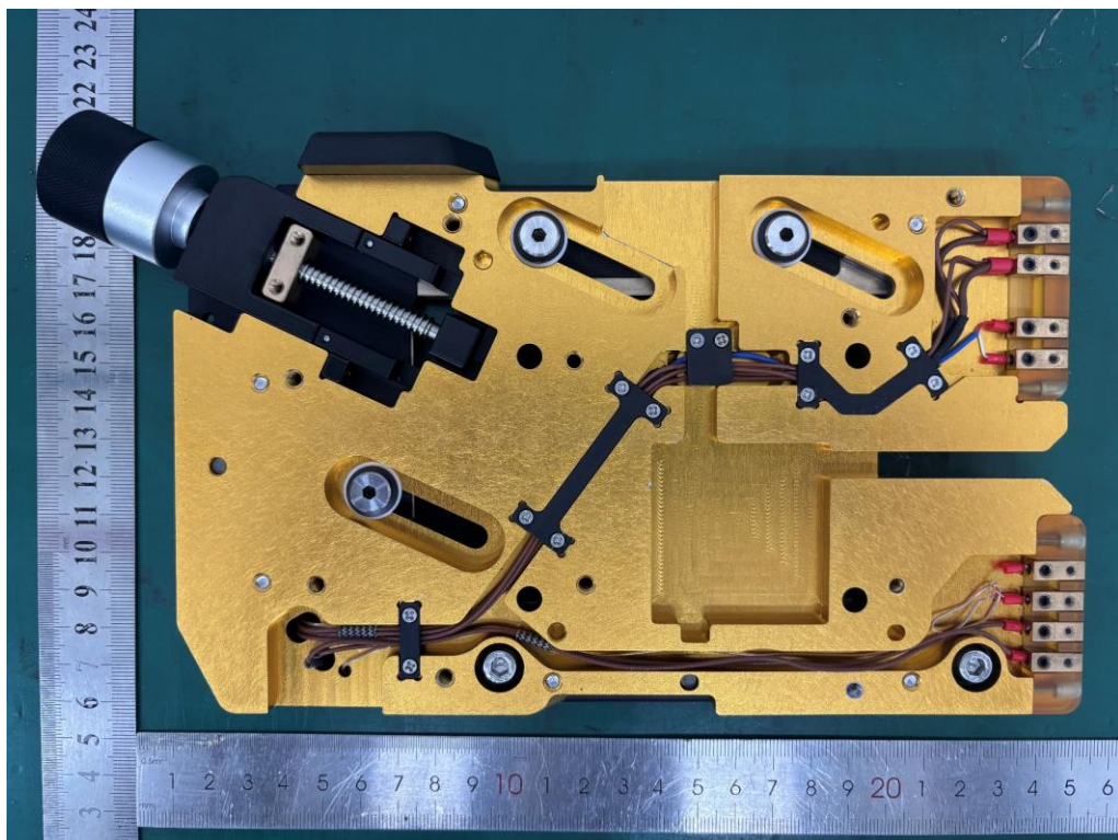
Photo 28: internal view of the dual channel carrier
