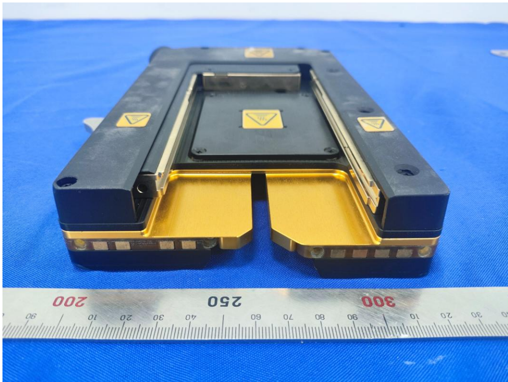
Photo 27: view of the dual channel carrier
