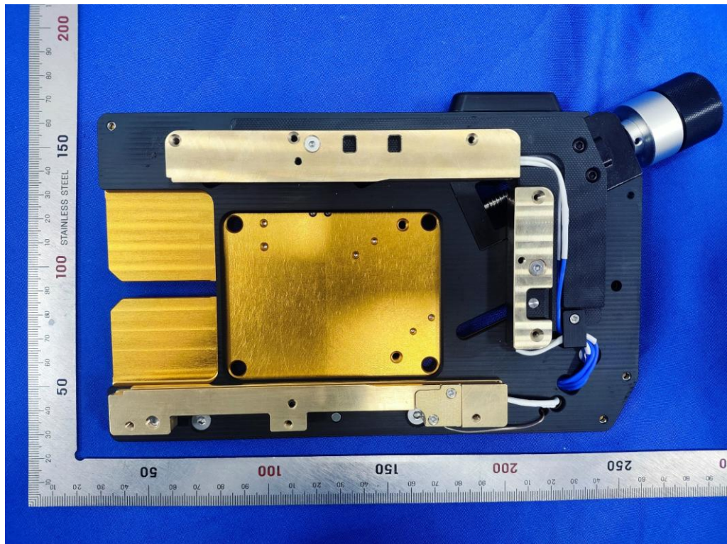
Photo 32: internal view of the single channel carrier
