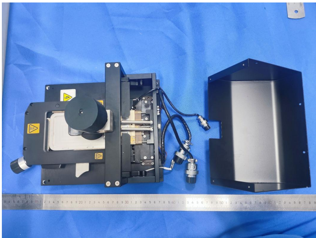
Photo 18: top internal view
