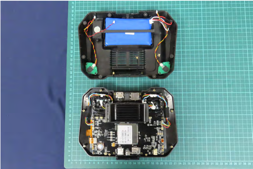
(1) EUT Photo
