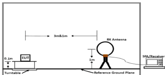
Below 30MHz Figure 1. Below 30MHz
