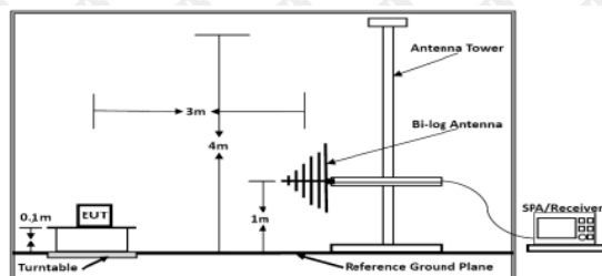
Below 1GHz Figure 2. 30MHz to 1GHz
