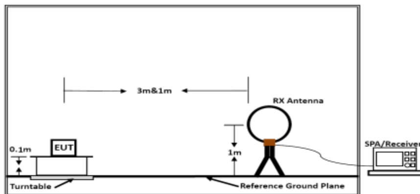
Figure 1. Below 30MHz
