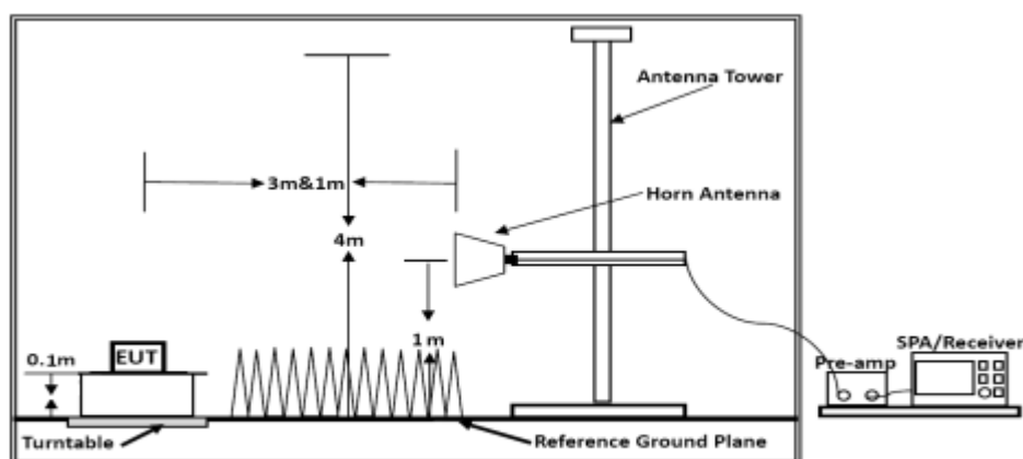
Figure 3. Above 1GHz
