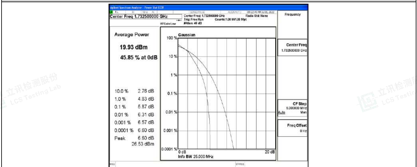
Band4-5MHz-16QAM-20375-1RB#0
