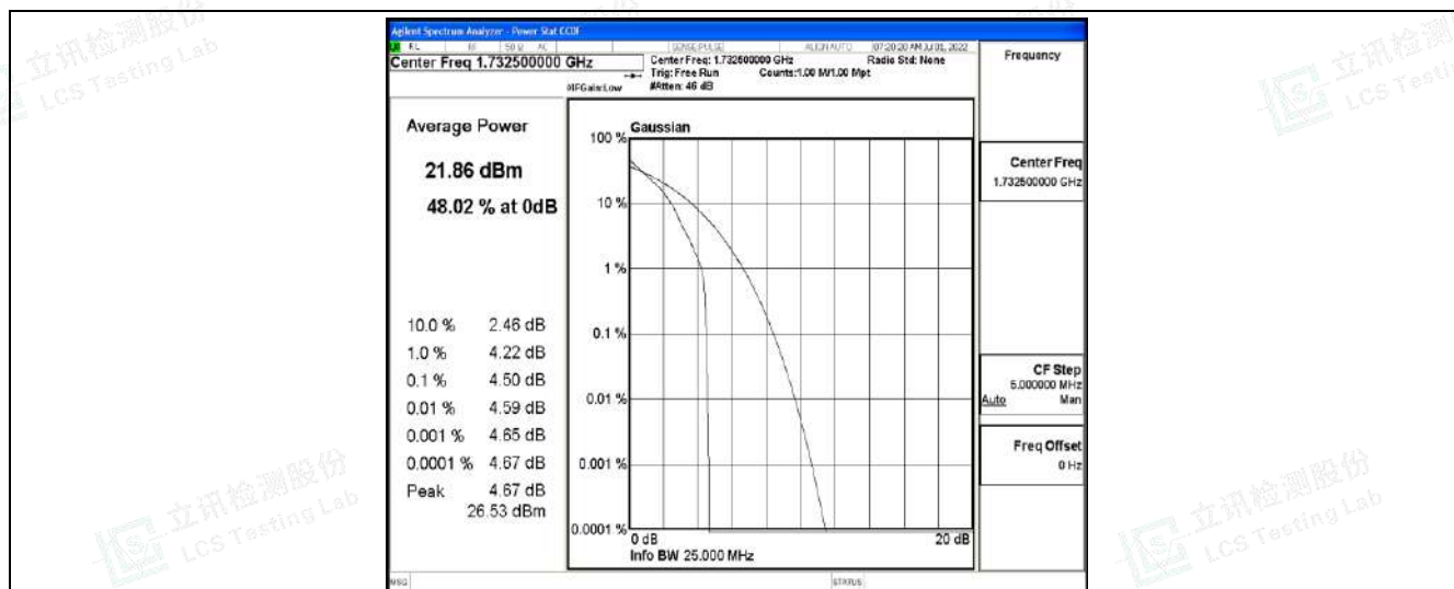
Band4-1.4MHz-QPSK-20175-6RB#0
