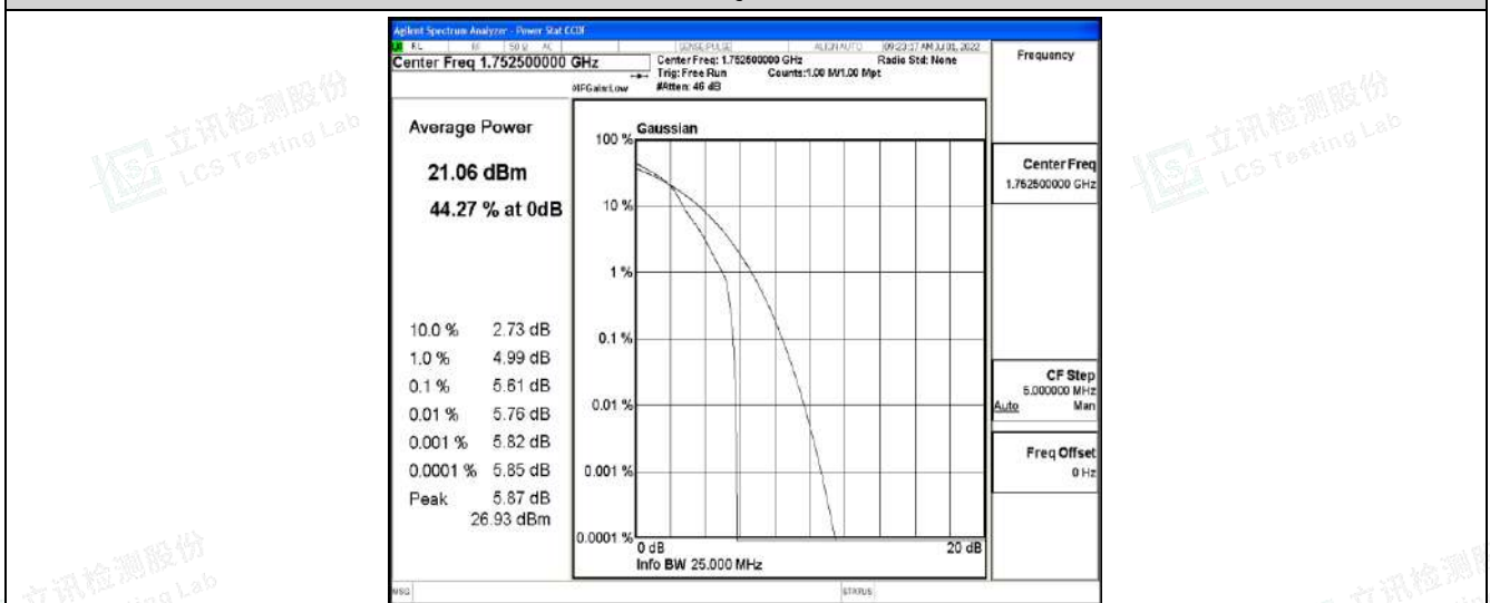
Band4-5MHz-16QAM-20375-1RB#0
