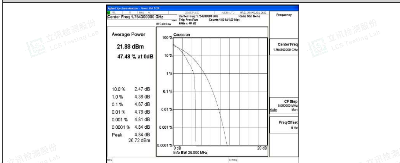
Band4-1.4MHz-QPSK-20393-1RB#0
