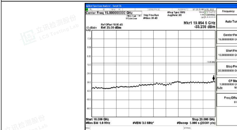
Band4-1.4MHz-16QAM-20393-1RB#0-Range5:10000~20000MHz
