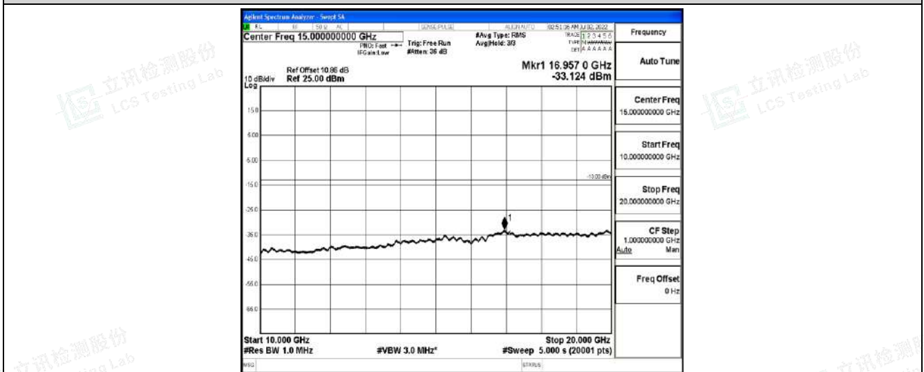
Band4-3MHz-16QAM-20175-1RB#0-Range5:10000~20000MHz
