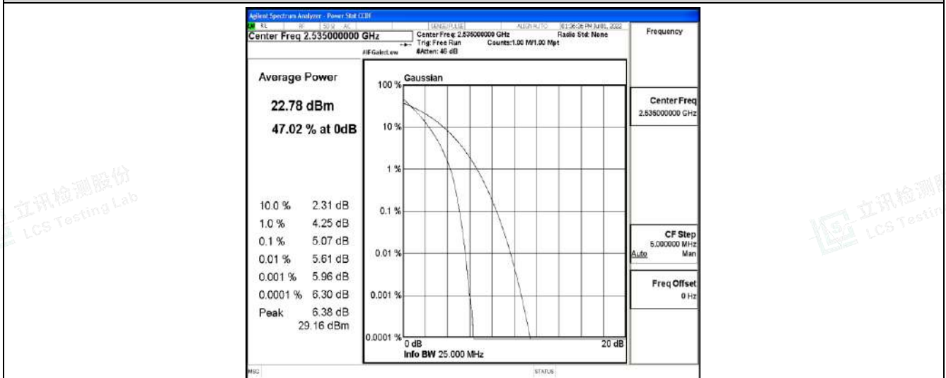
Band7-20MHz-QPSK-21350-1RB#0
