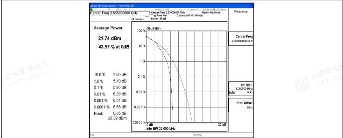
Band7-15MHz-16QAM-21375-1RB#0
