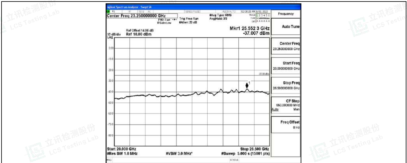
Band7-5MHz-16QAM-20775-1RB#0-Range1:0.009~0.15MHz
