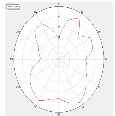
2450T90 Total
