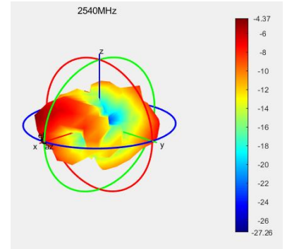
2300T90 Total
