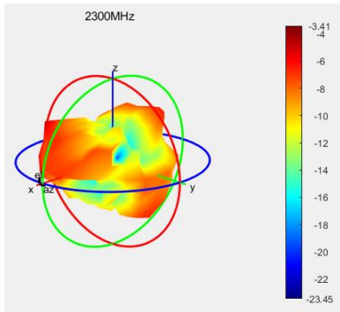
2300P0 Total
