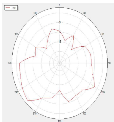
2300P90 Total
