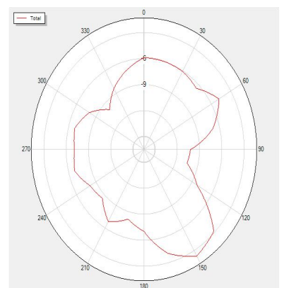
2300T90 Total
