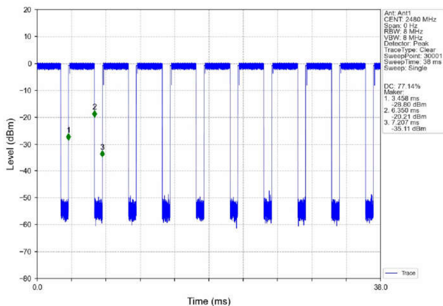
Pi/4DQPSK_2DH5_HCH_2480MHz_Ant1_NTNV
