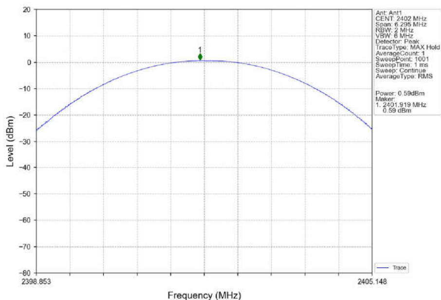
Pi/4DQPSK_2DH5_LCH_2402MHz_Ant1_NTNV
