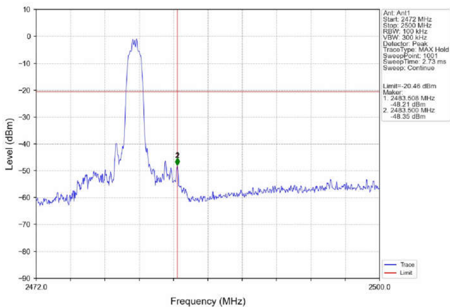
Pi/4DQPSK_2DH5_HCH_2480MHz_Ant1_NTNV
