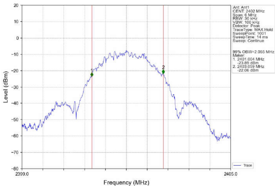
2M_LCH_2402MHz_Ant1_NTNV
