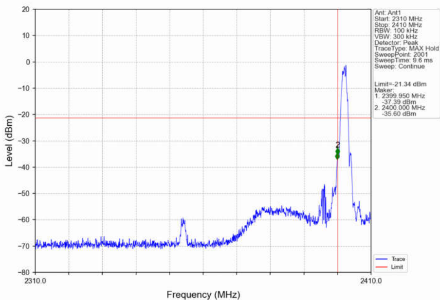
2M_LCH_2402MHz_Ant1_NTNV
