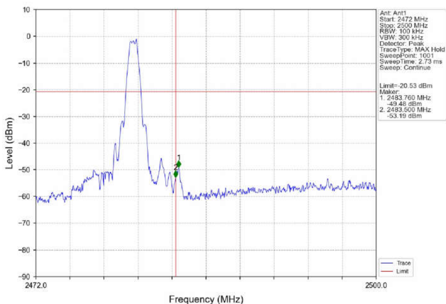
1M_HCH_2480MHz_Ant1_NTNV
