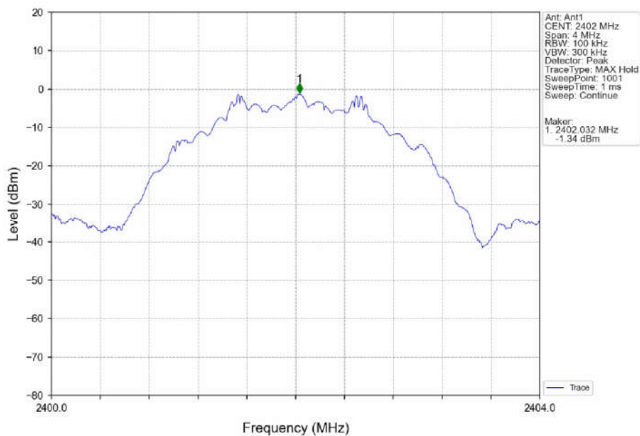
2M_LCH_2402MHz_Ant1_NTNV
