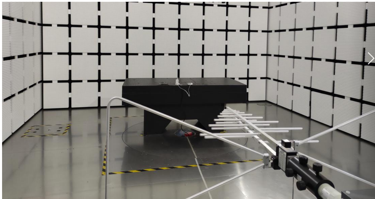
Radiated Measurement Photos
