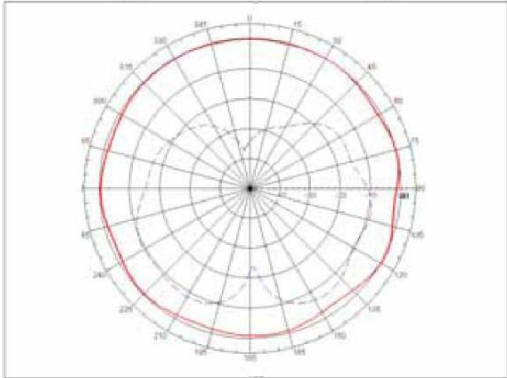
Far-field amplitude of YZ_plane.nsi
