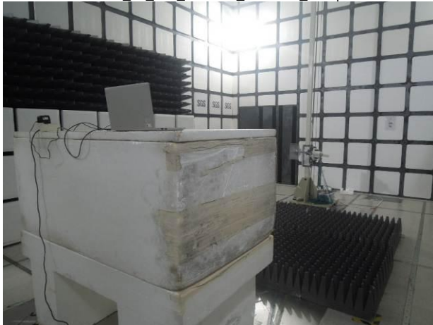
FCC_15_247_900MHz_Radiated_Setup
