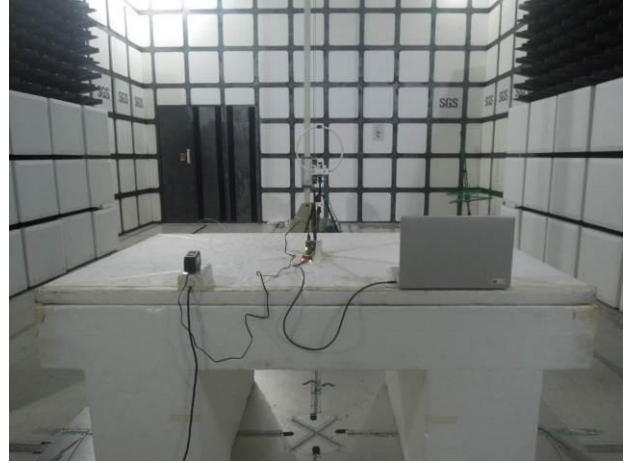
FCC_15_247_900MHz_Radiated_Setup
