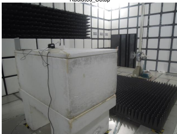
Radiated_Setup
