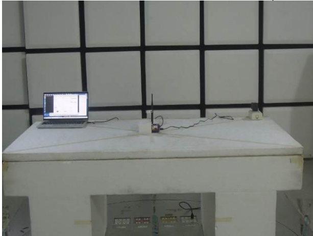
FCC_15_247_902~928MHz_OFDM_Radiated_Setup
