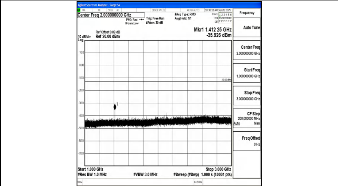
Band12_3MHz_QPSK_23095_1RB#0_1000~3000_1000~3000
