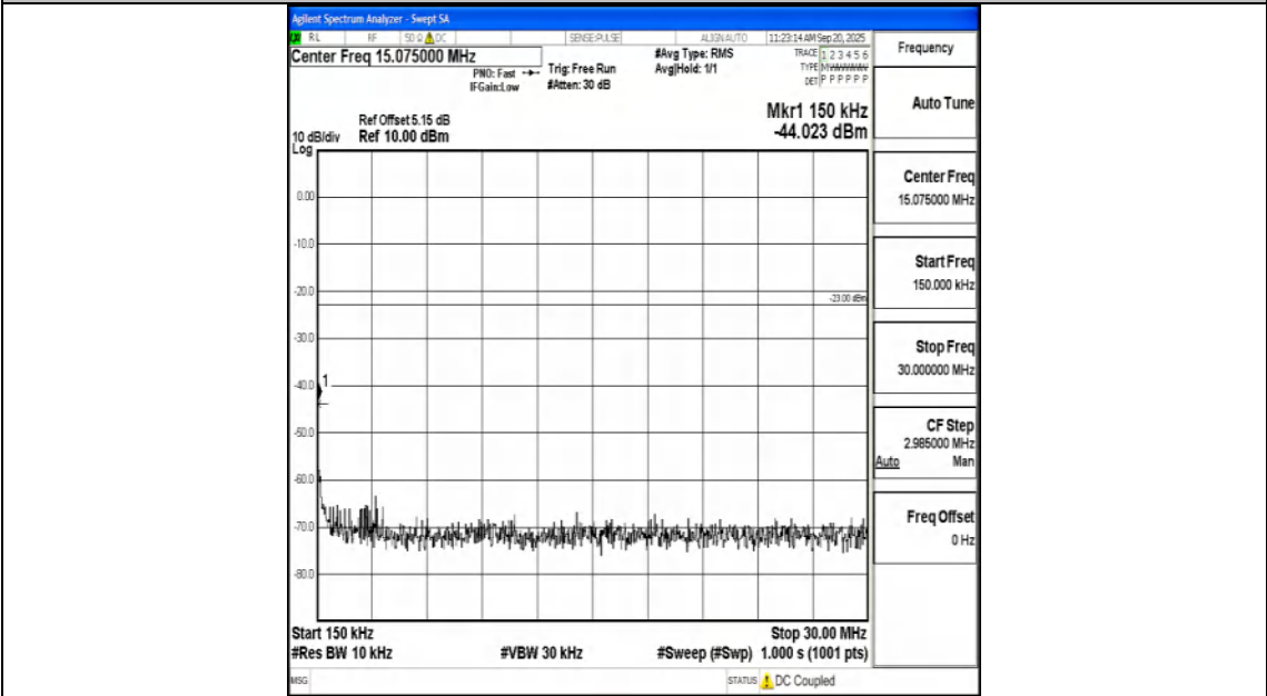
Band12_10MHz_QPSK_23130_1RB#0_0.15~30_0.15~30
