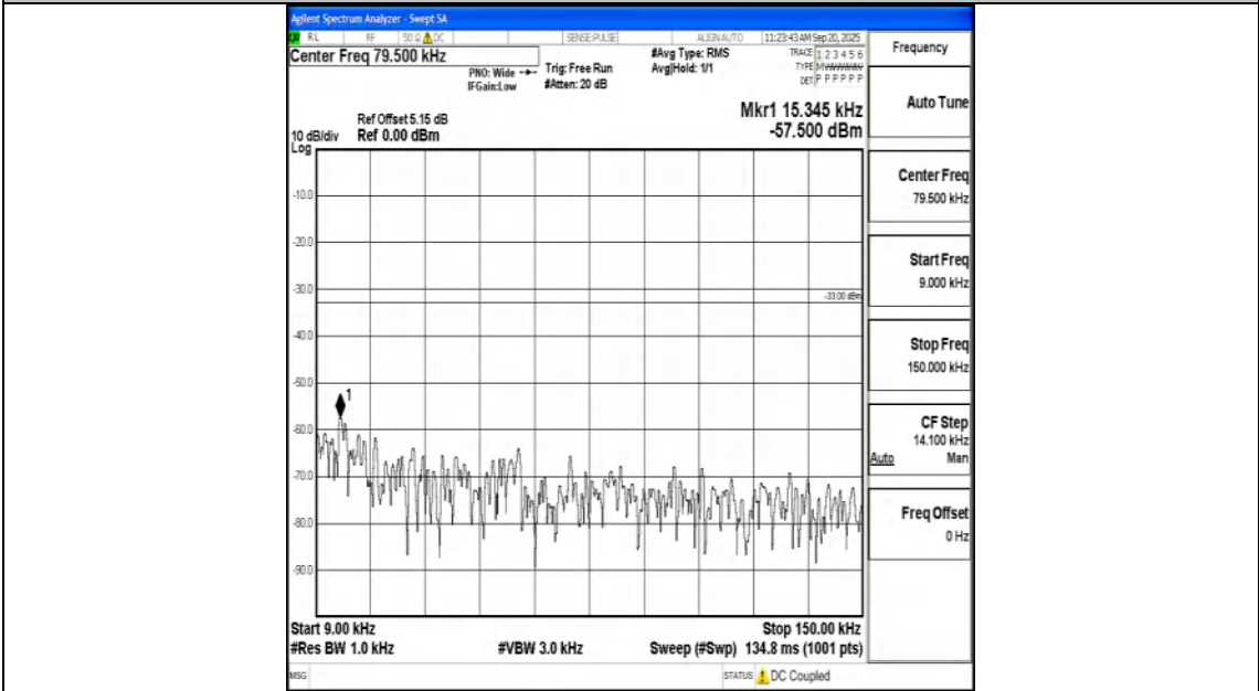
Band12_10MHz_16QAM_23130_1RB#0_0.009~0.15_0.009~0.15
