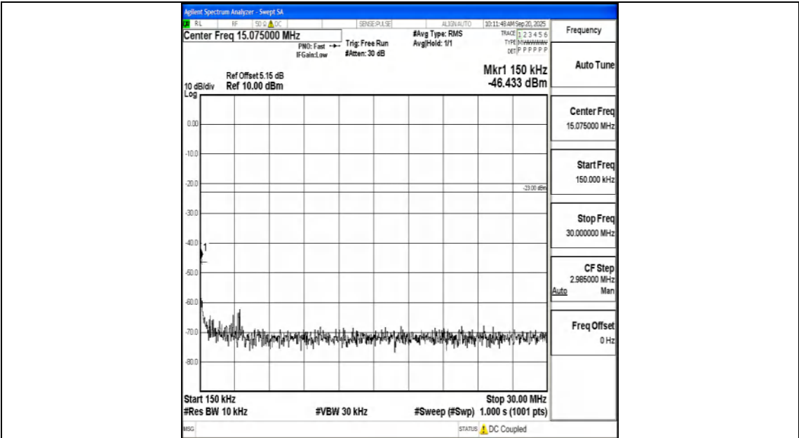
Band12_1.4MHz_16QAM_23173_1RB#0_0.15~30_0.15~30
