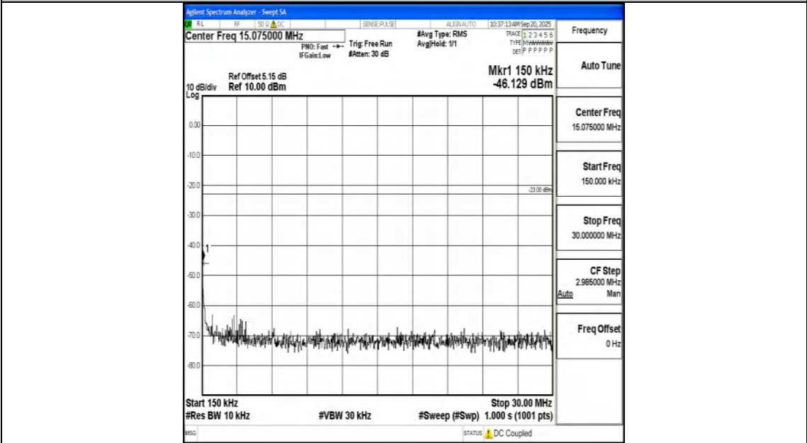
Band12_3MHz_QPSK_23025_1RB#0_0.15~30_0.15~30
