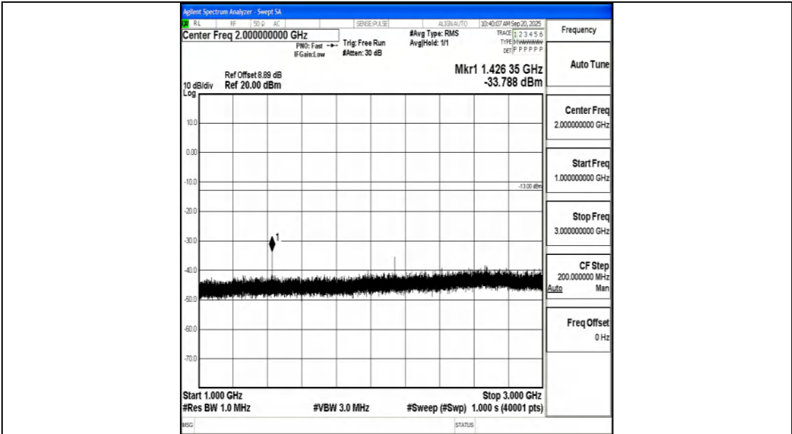
Band12_3MHz_16QAM_23165_1RB#0_1000~3000_1000~3000
