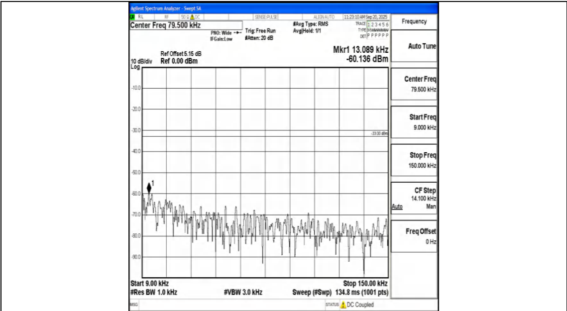
Band12_10MHz_QPSK_23130_1RB#0_0.009~0.15_0.009~0.15
