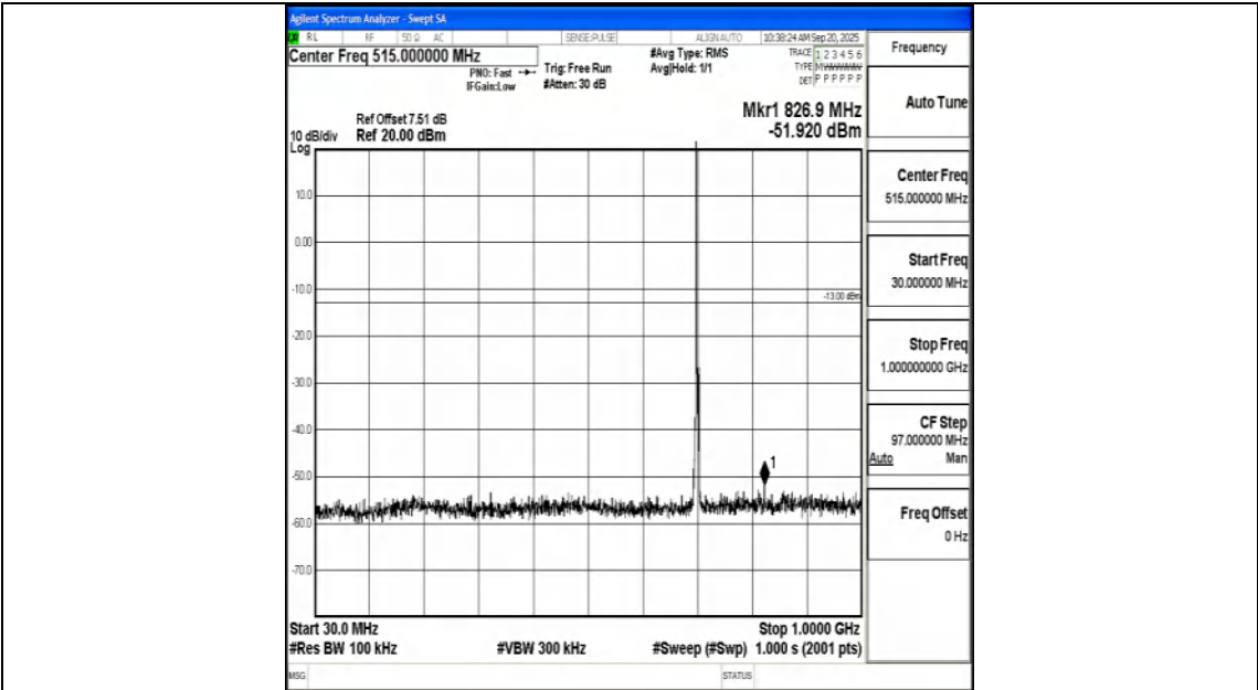
Band12_3MHz_QPSK_23095_1RB#0_30~1000_30~1000
