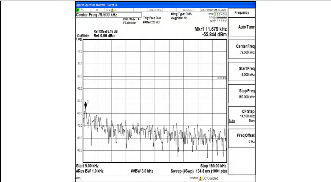
Band12_3MHz_QPSK_23025_1RB#0_0.009~0.15_0.009~0.15
