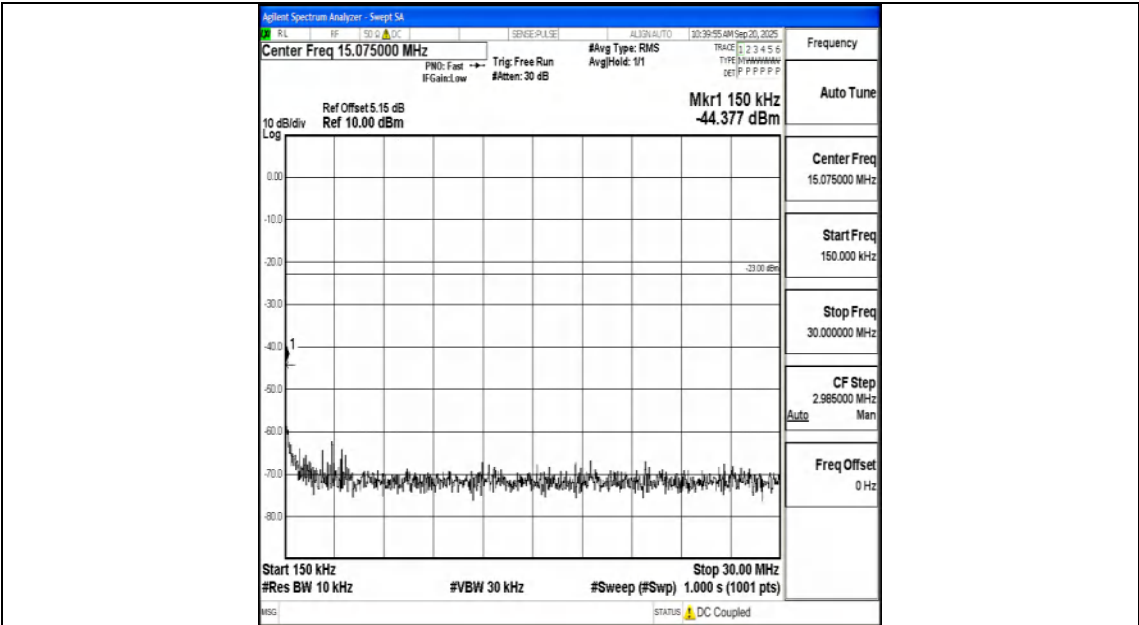
Band12_3MHz_16QAM_23165_1RB#0_0.15~30_0.15~30
