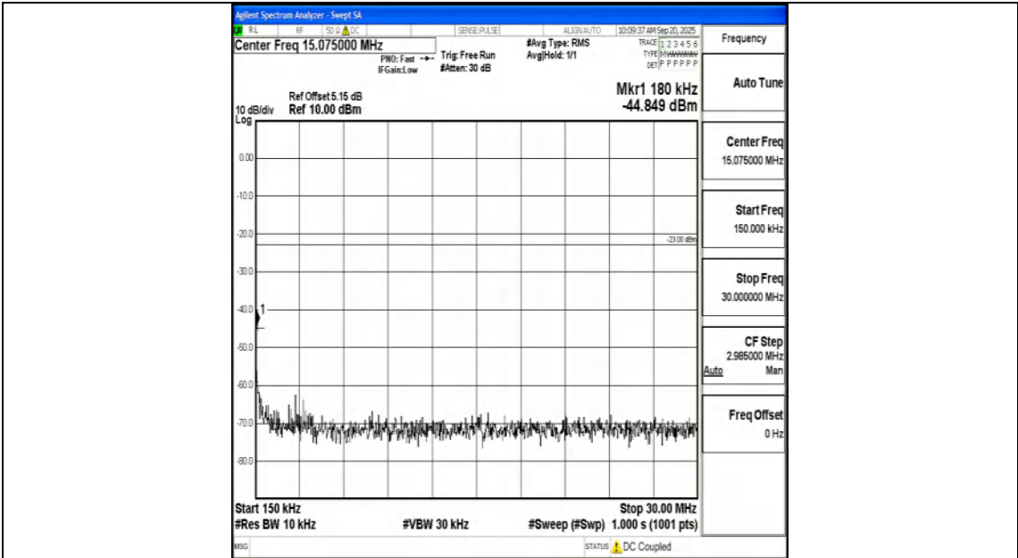
Band12_1.4MHz_16QAM_23017_1RB#0_0.15~30_0.15~30
