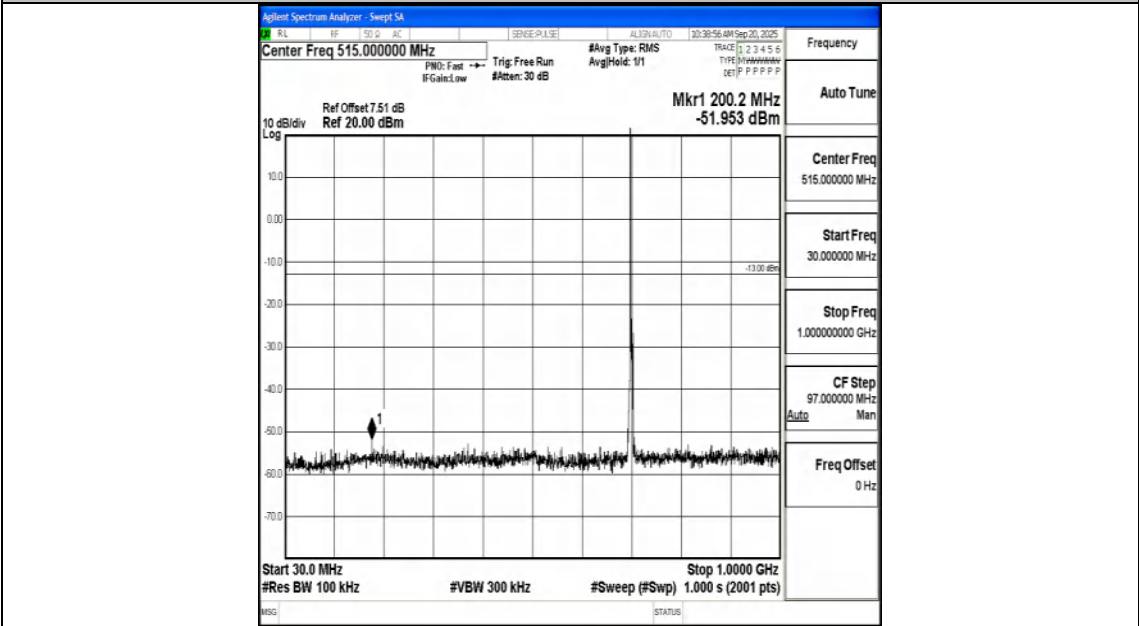
Band12_3MHz_16QAM_23095_1RB#0_30~1000_30~1000
