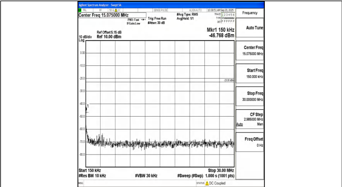
Band12_3MHz_16QAM_23095_1RB#0_0.15~30_0.15~30
