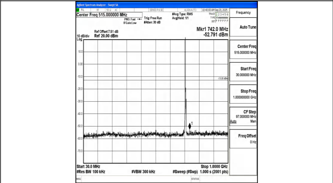
Band12_3MHz_16QAM_23165_1RB#0_30~1000_30~1000
