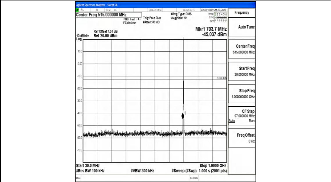
Band12_1.4MHz_16QAM_23095_1RB#0_30~1000_30~1000
