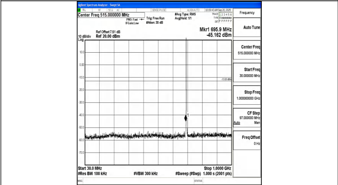
Band12_1.4MHz_16QAM_23017_1RB#0_30~1000_30~1000
