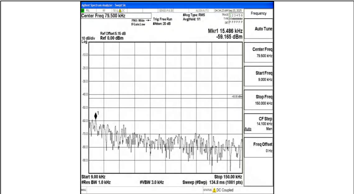
Band2_15MHz_16QAM_18900_1RB#0_0.009~0.15_0.009~0.15
