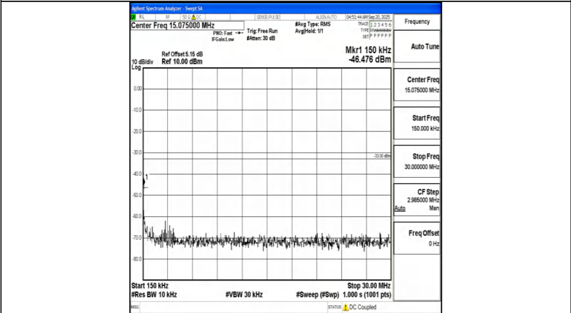
Band2_20MHz_16QAM_18700_1RB#0_0.15~30_0.15~30
