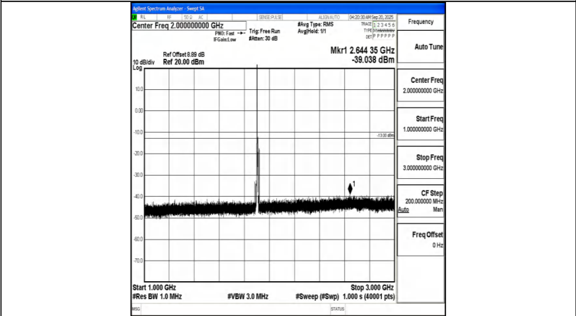
Band2_10MHz_QPSK_19150_1RB#0_1000~3000_1000~3000
