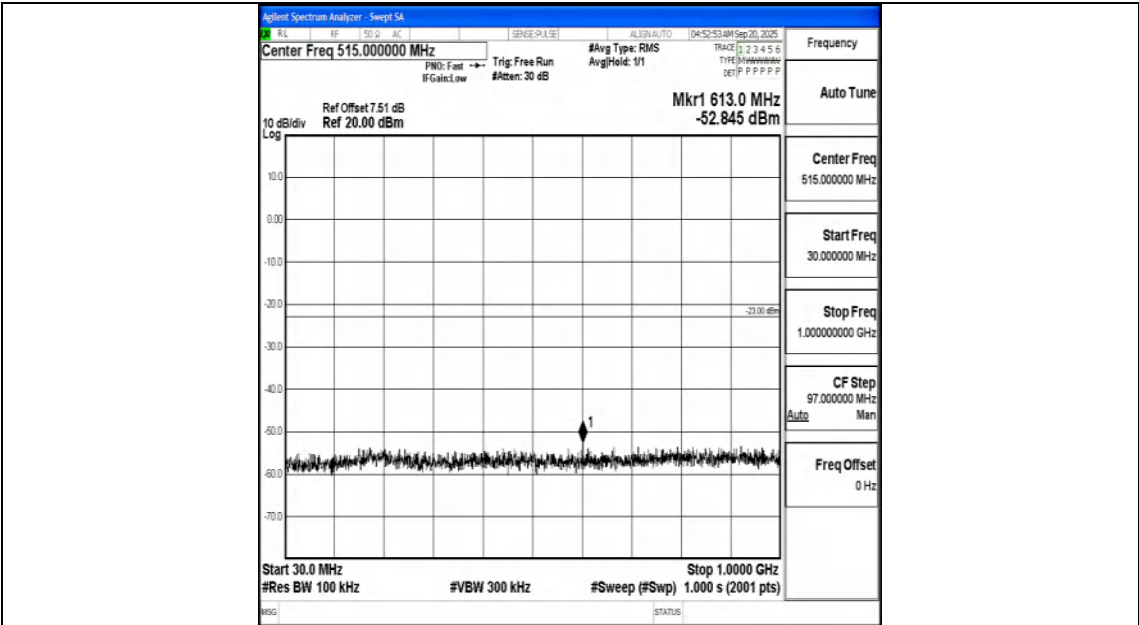
Band2_20MHz_16QAM_18900_1RB#0_30~1000_30~1000
