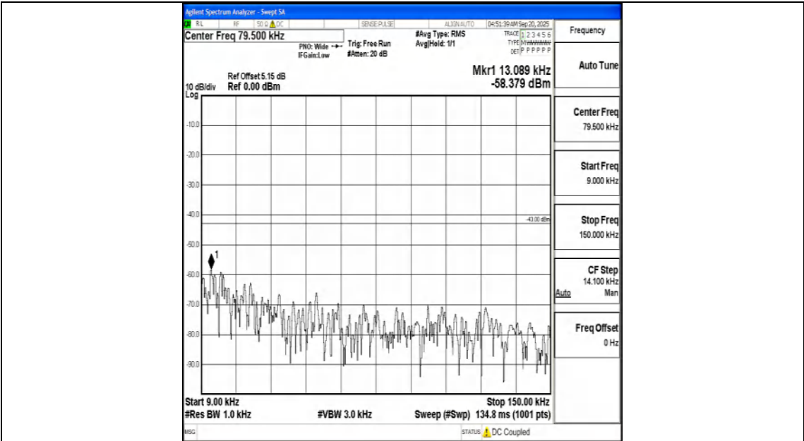
Band2_20MHz_16QAM_18700_1RB#0_0.009~0.15_0.009~0.15
