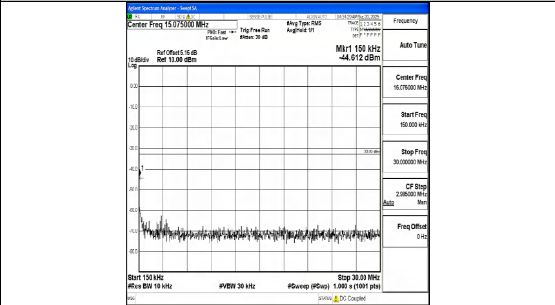
Band2_15MHz_16QAM_18900_1RB#0_0.15~30_0.15~30
