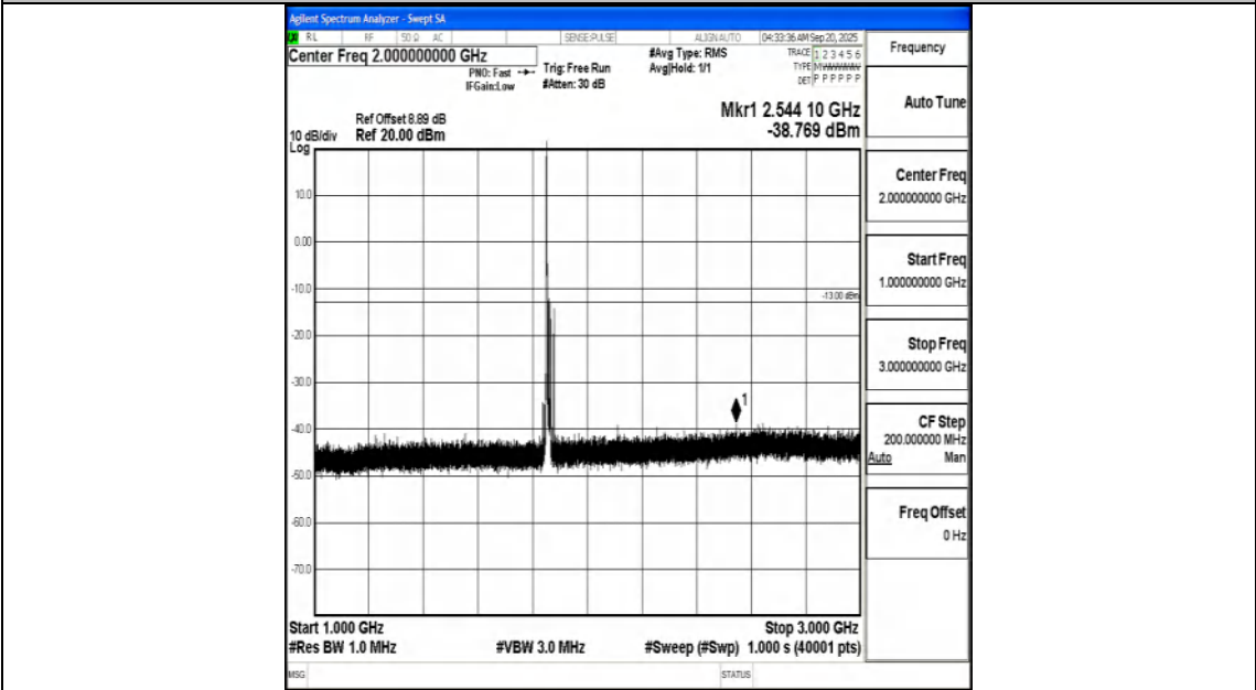
Band2_15MHz_16QAM_18675_1RB#0_1000~3000_1000~3000
