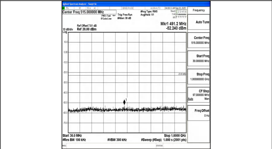
Band2_5MHz_16QAM_18900_1RB#0_30~1000_30~1000
