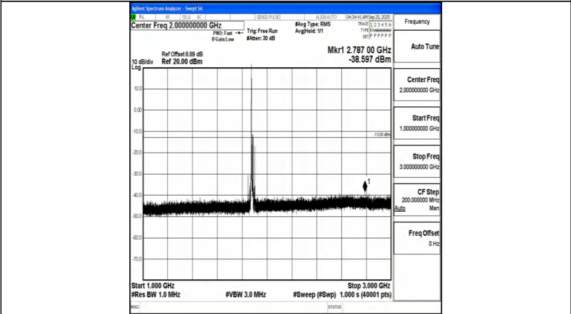
Band2_15MHz_16QAM_18900_1RB#0_1000~3000_1000~3000
