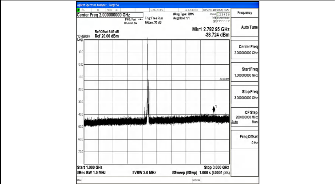
Band2_20MHz_16QAM_18900_1RB#0_1000~3000_1000~3000
