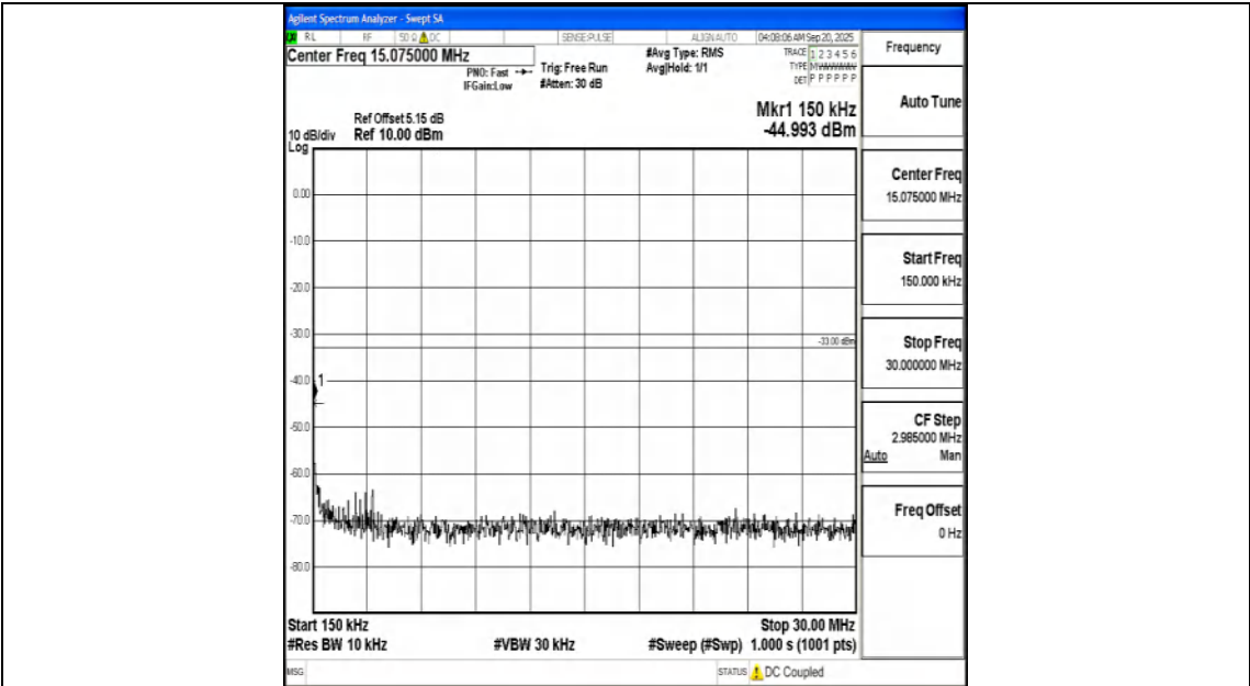
Band2_5MHz_16QAM_18900_1RB#0_0.15~30_0.15~30
