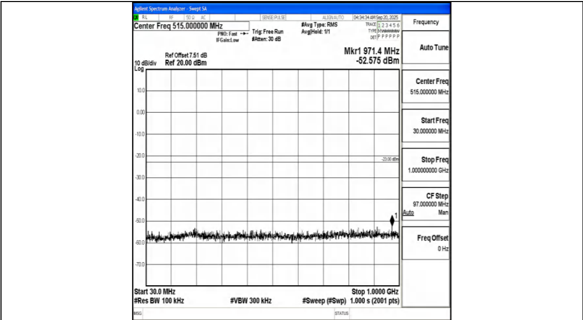
Band2_15MHz_16QAM_18900_1RB#0_30~1000_30~1000
