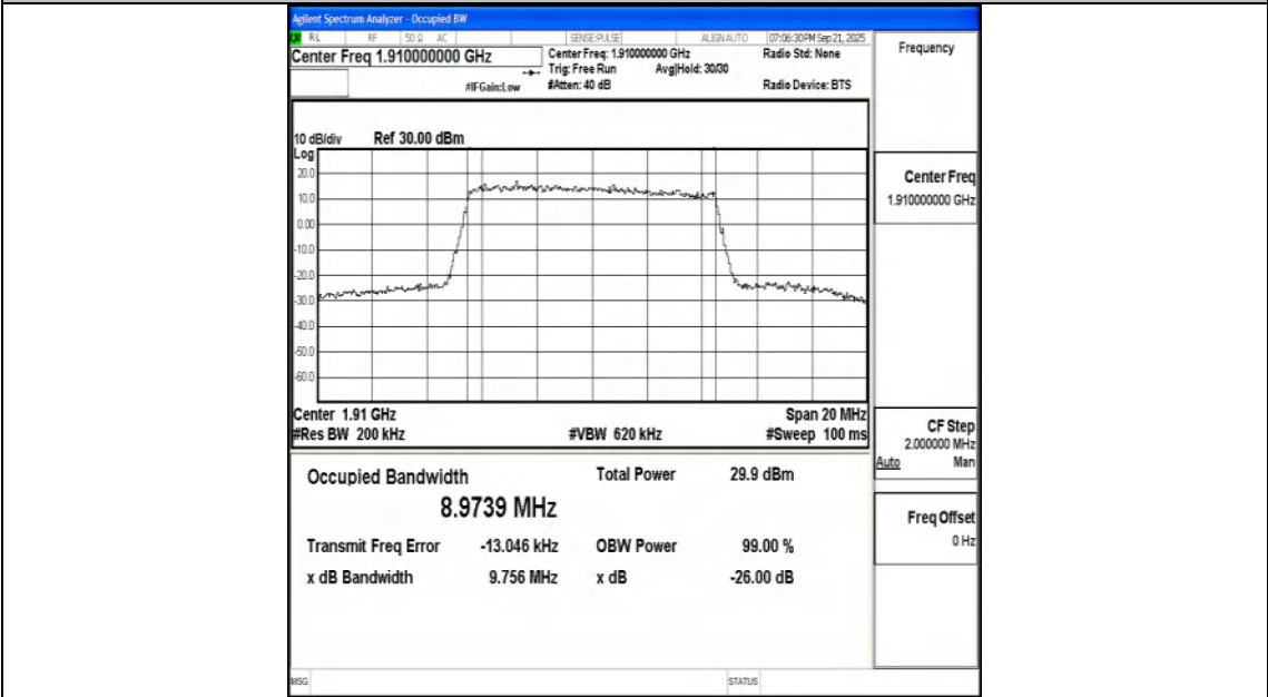
Band25-10MHz-16QAM-26640-50RB#0-PASS
