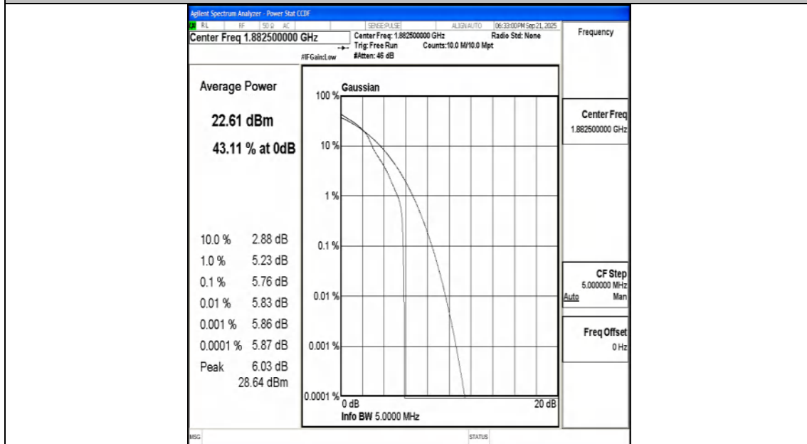
Band25-3MHz-16QAM-26365-1RB#0-PASS
