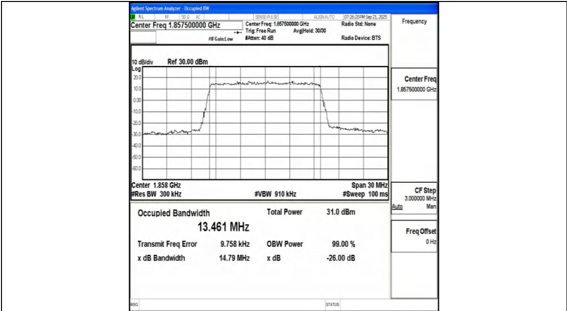
Band25-15MHz-QPSK-26115-75RB#0-PASS
