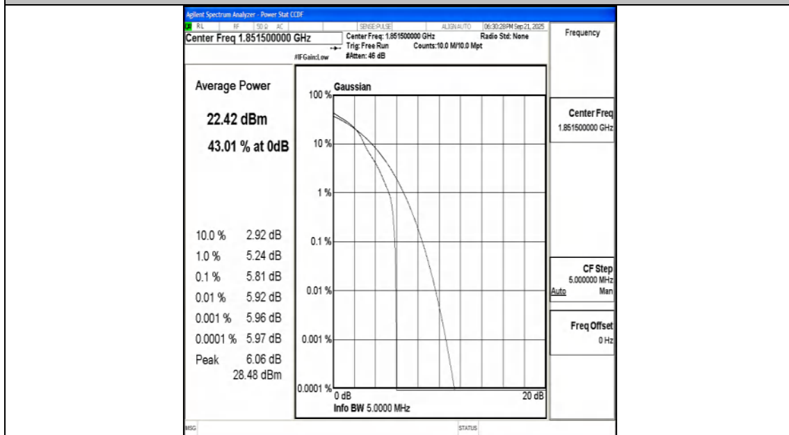
Band25-3MHz-16QAM-26055-1RB#0-PASS
