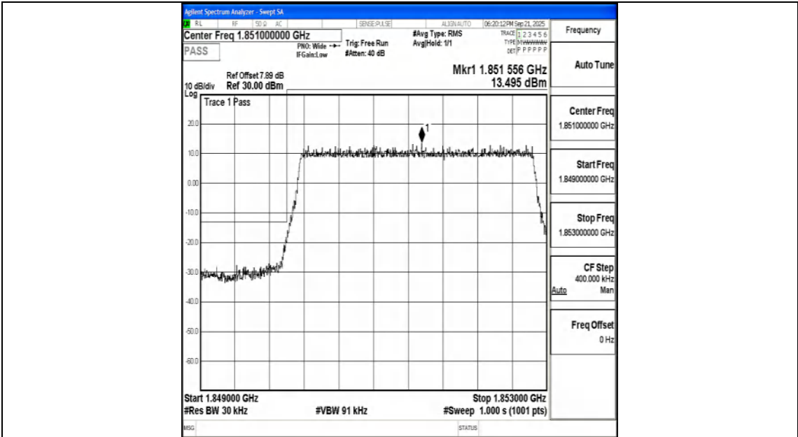
Band25_3MHz_QPSK_26055_15RB#0
