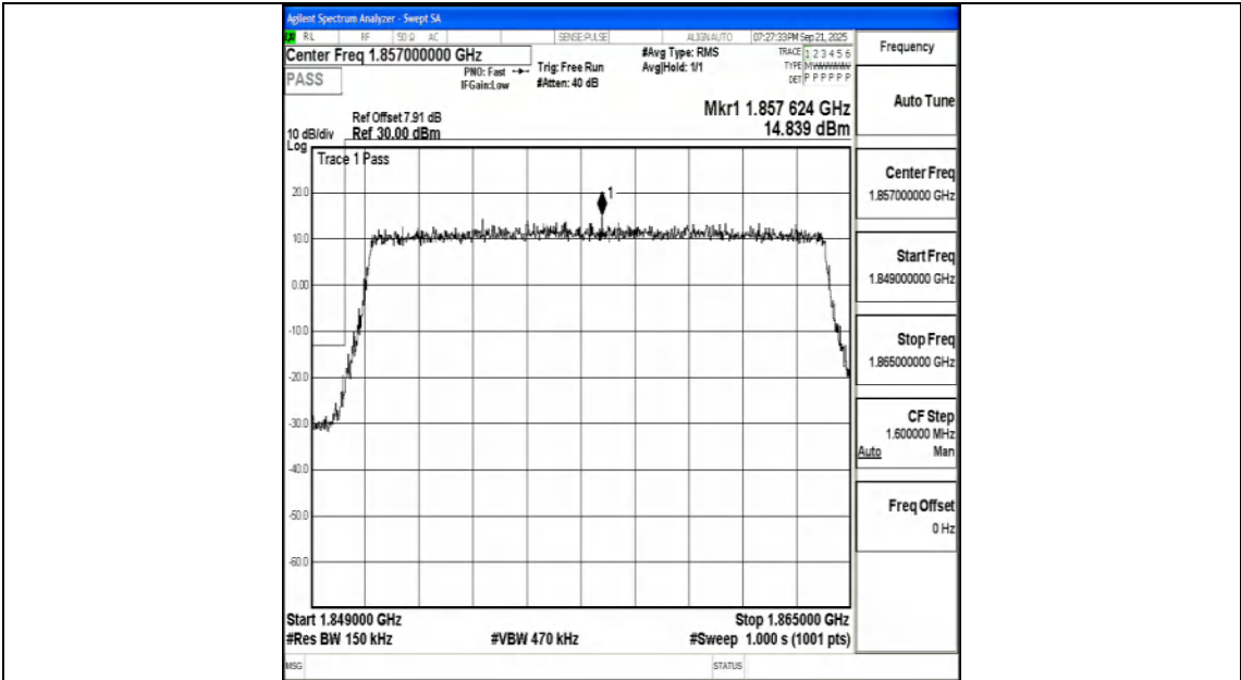
Band25_15MHz_QPSK_26115_75RB#0
