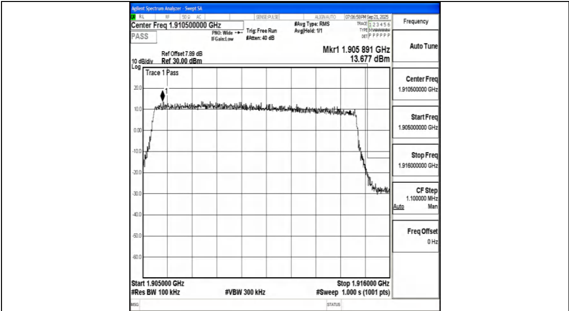
Band25_10MHz_QPSK_26640_50RB#0
