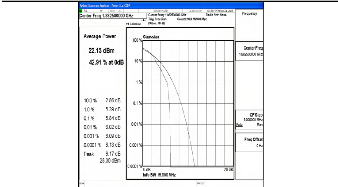
Band25-15MHz-16QAM-26365-1RB#0-PASS
