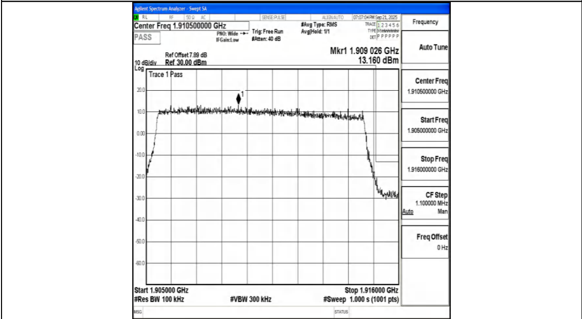
Band25_10MHz_16QAM_26640_50RB#0
