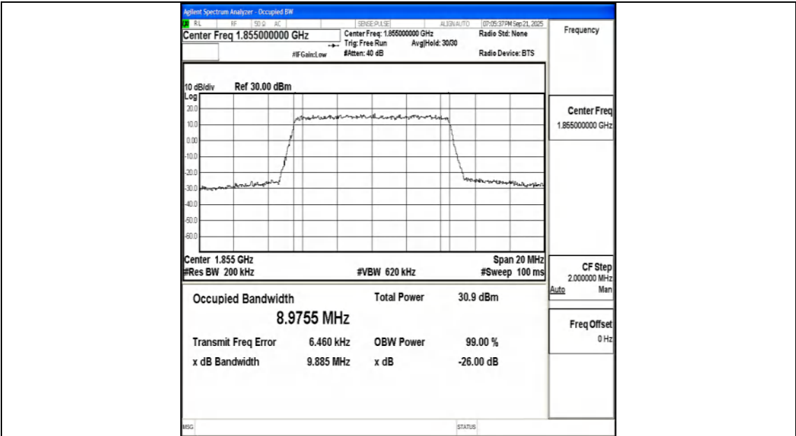
Band25-10MHz-QPSK-26090-50RB#0-PASS
