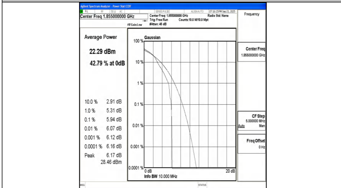
Band25-10MHz-16QAM-26090-1RB#0-PASS
