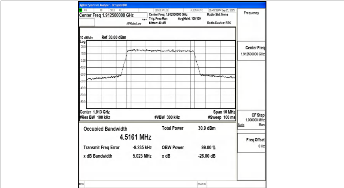
Band25-5MHz-QPSK-26665-25RB#0-PASS
