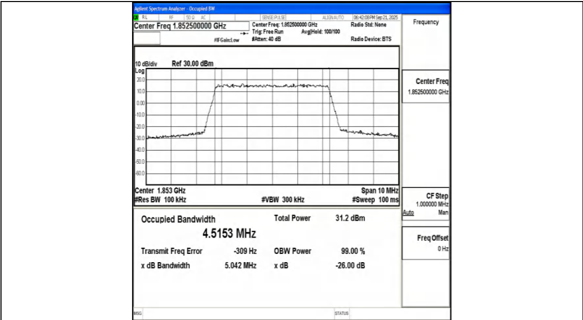
Band25-5MHz-QPSK-26065-25RB#0-PASS
