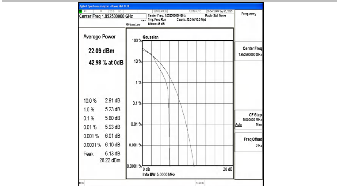
Band25-5MHz-16QAM-26065-1RB#0-PASS
