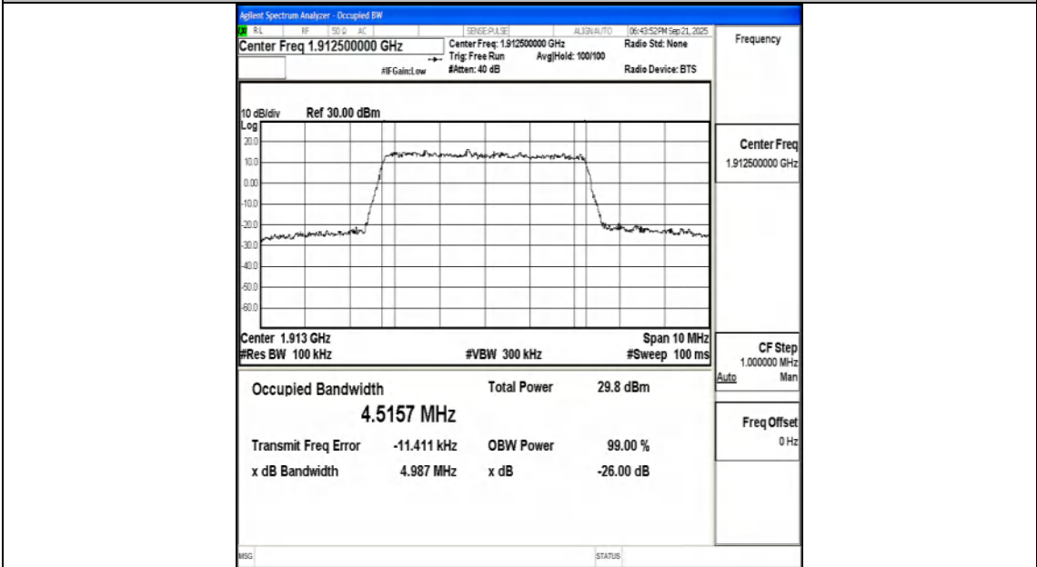
Band25-5MHz-16QAM-26665-25RB#0-PASS
