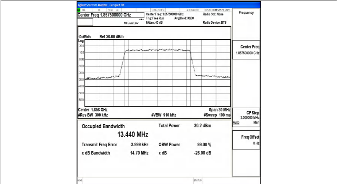
Band25-15MHz-16QAM-26115-75RB#0-PASS
