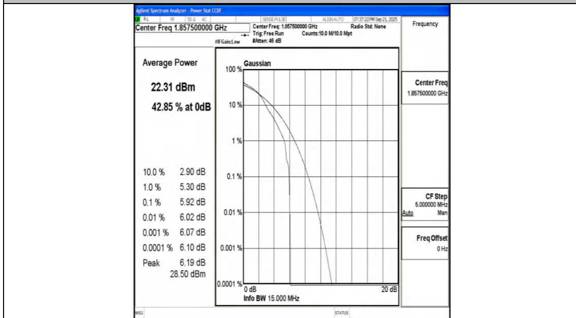
Band25-15MHz-16QAM-26115-1RB#0-PASS
