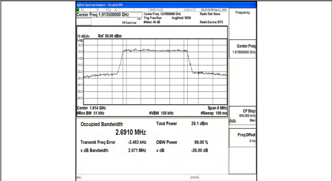
Band25-3MHz-16QAM-26675-15RB#0-PASS
