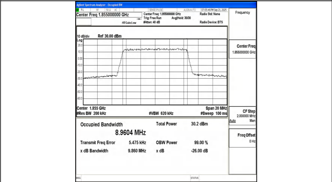
Band25-10MHz-16QAM-26090-50RB#0-PASS
