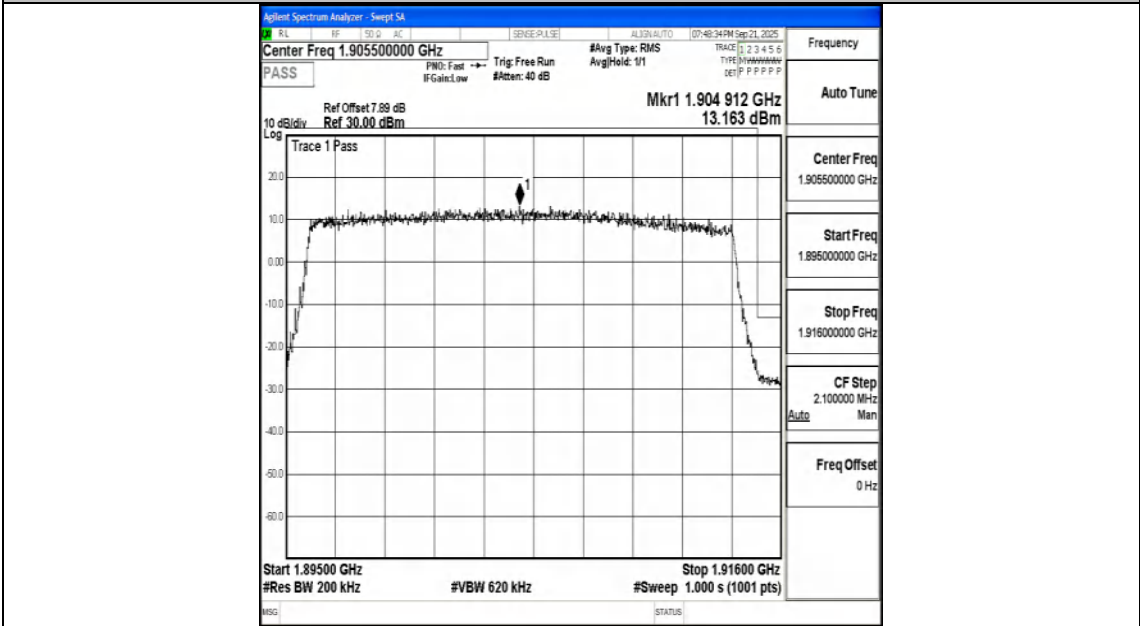
Band25_20MHz_16QAM_26590_100RB#0
