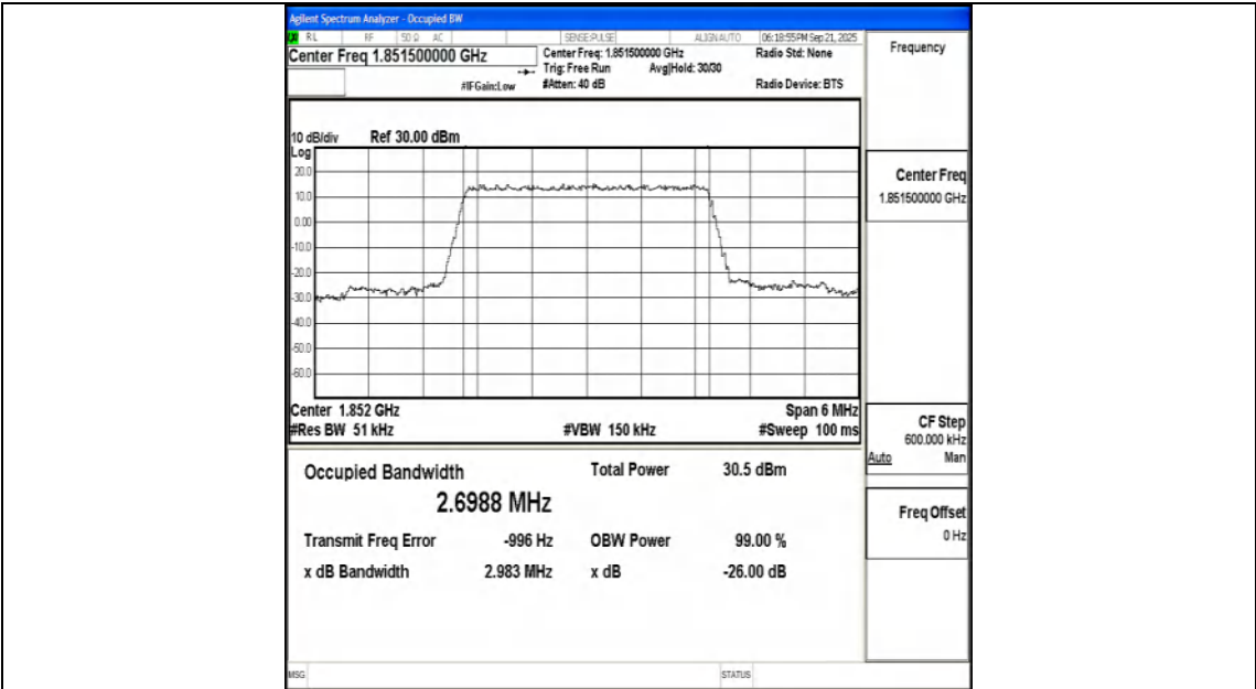
Band25-3MHz-QPSK-26055-15RB#0-PASS
