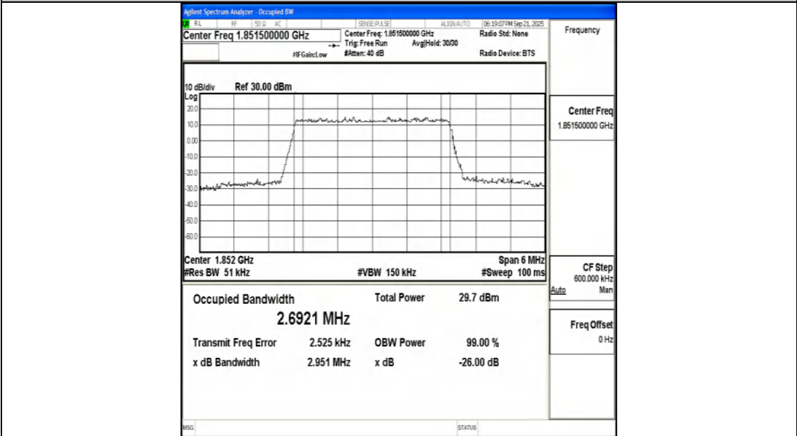
Band25-3MHz-16QAM-26055-15RB#0-PASS
