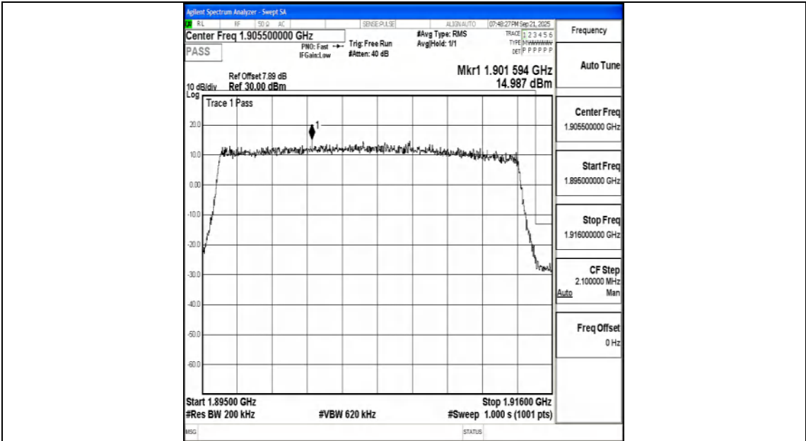
Band25_20MHz_QPSK_26590_100RB#0
