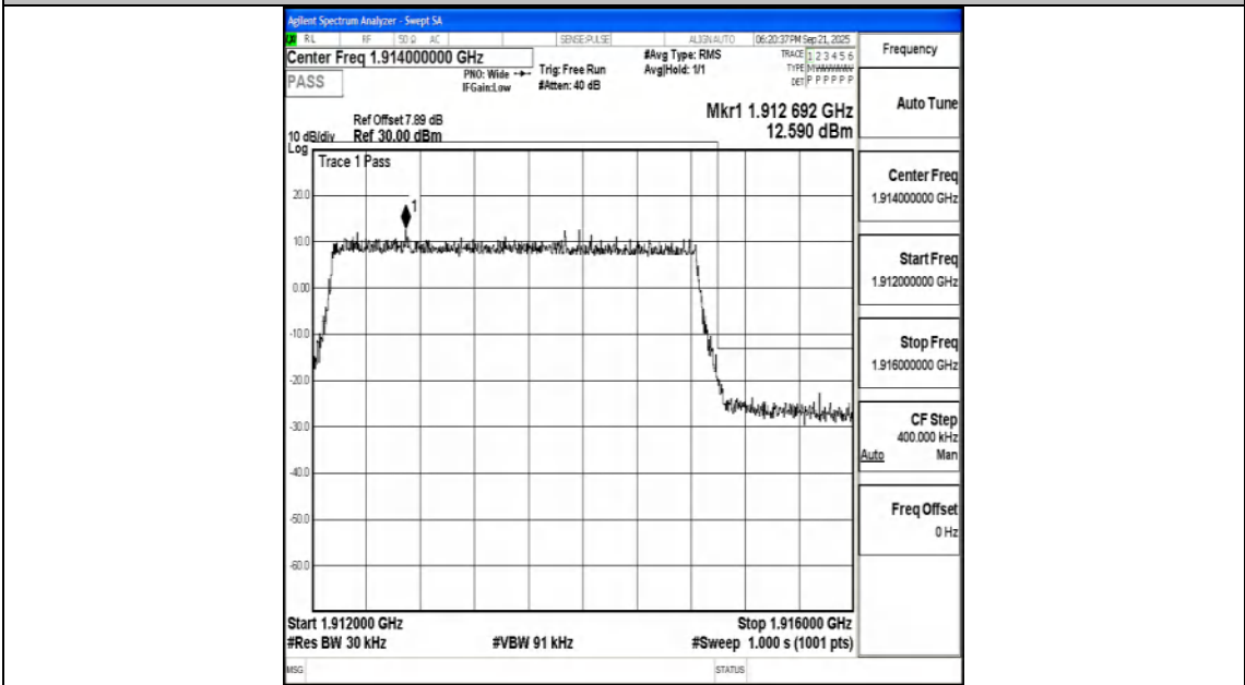
Band25_3MHz_16QAM_26675_15RB#0
