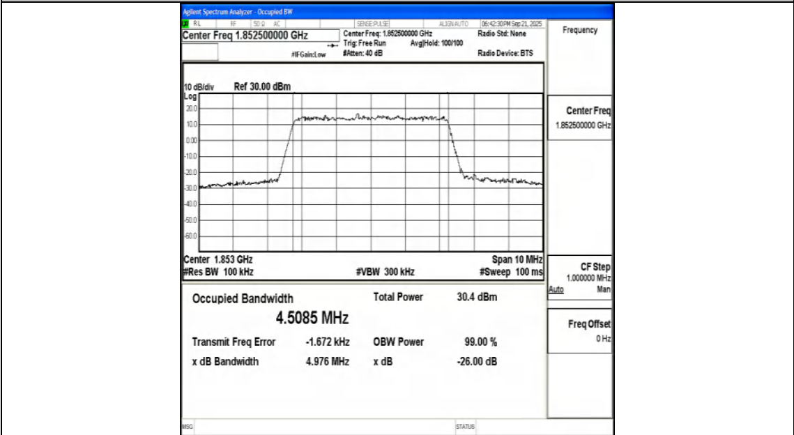
Band25-5MHz-16QAM-26065-25RB#0-PASS
