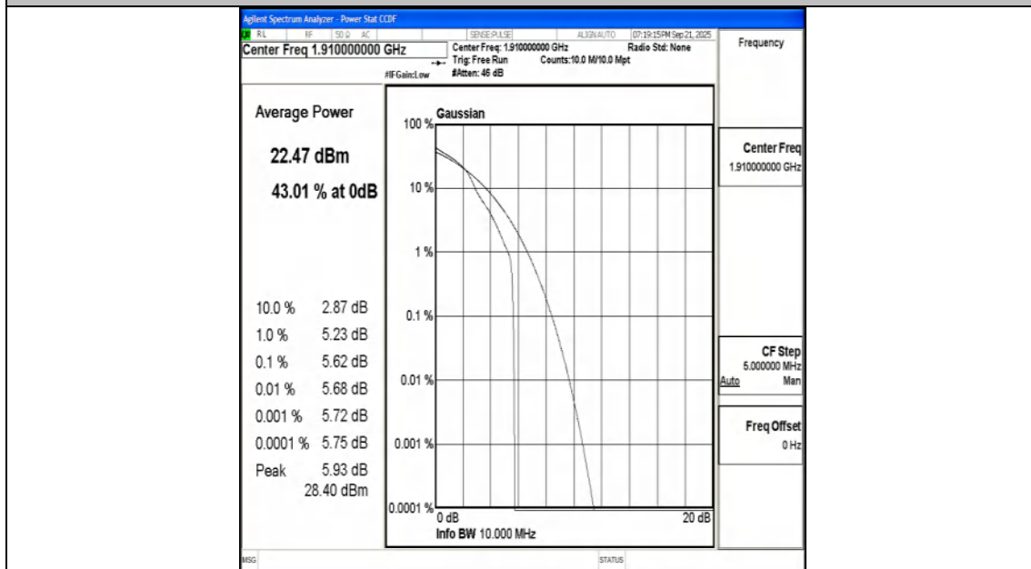
Band25-10MHz-16QAM-26640-1RB#0-PASS
