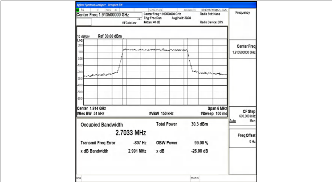
Band25-3MHz-QPSK-26675-15RB#0-PASS
