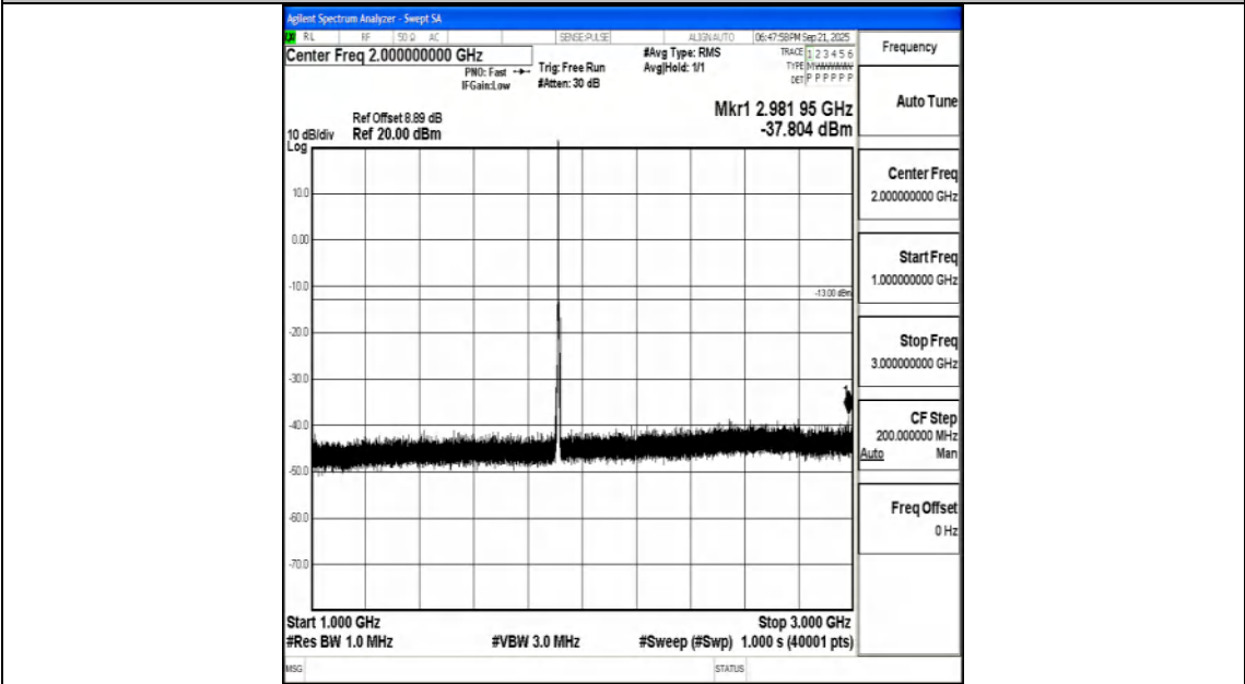
Band25_5MHz_16QAM_26665_1RB#0_1000~3000_1000~3000
