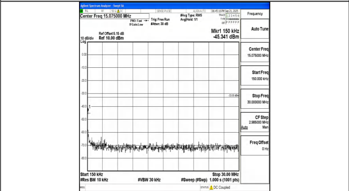
Band25_5MHz_16QAM_26065_1RB#0_0.15~30_0.15~30
