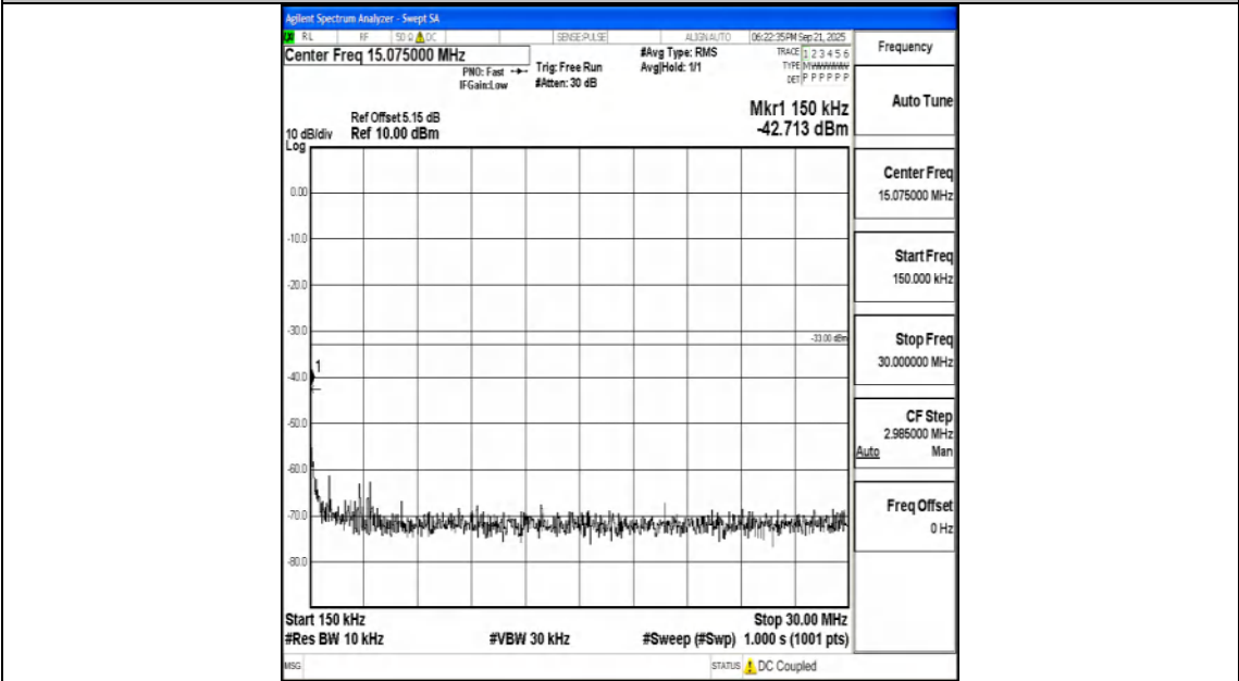
Band25_3MHz_16QAM_26365_1RB#0_0.15~30_0.15~30
