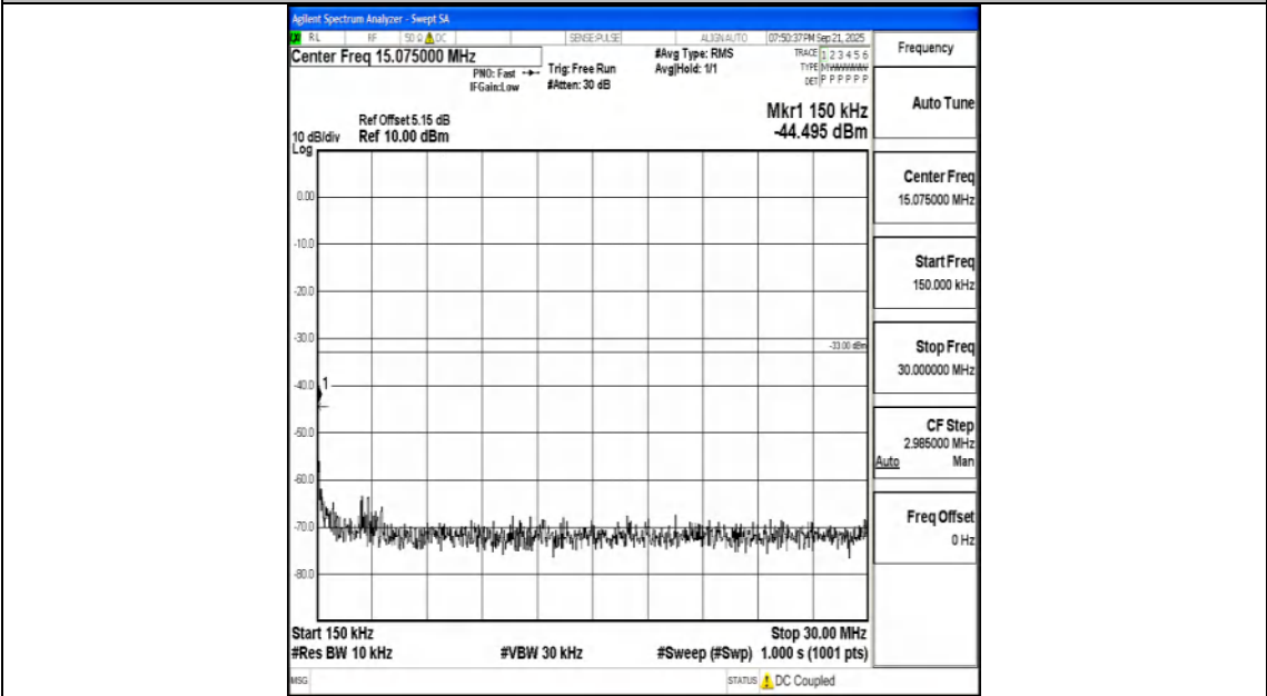
Band25_20MHz_16QAM_26365_1RB#0_0.15~30_0.15~30
