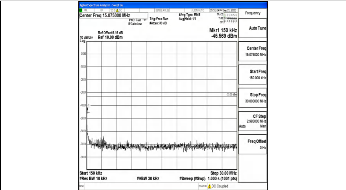
Band25_1.4MHz_QPSK_26365_1RB#0_0.15~30_0.15~30
