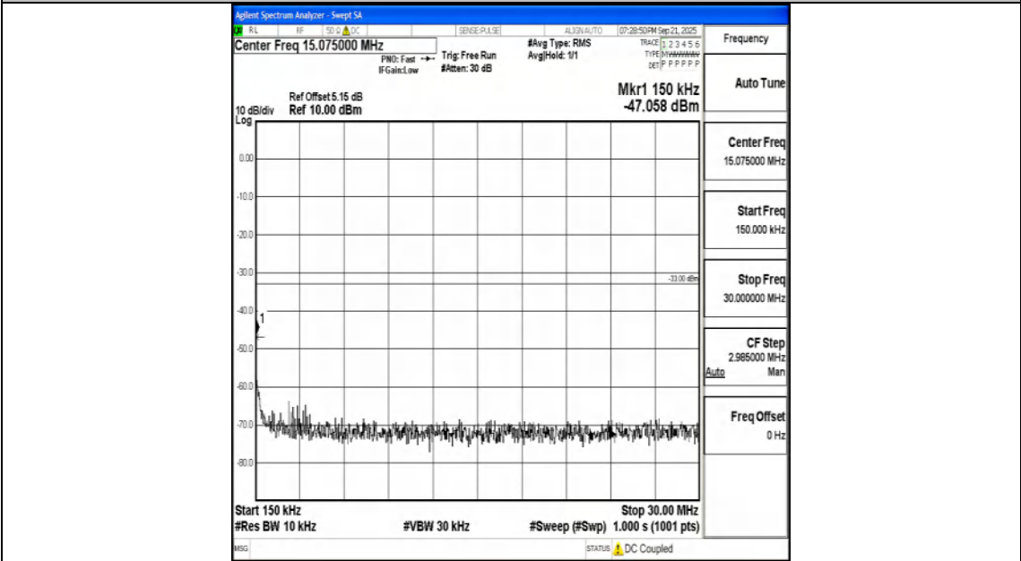
Band25_15MHz_16QAM_26115_1RB#0_0.15~30_0.15~30
