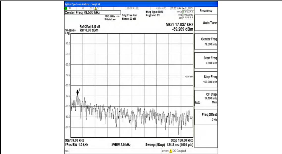
Band25_20MHz_16QAM_26365_1RB#0_0.009~0.15_0.009~0.15
