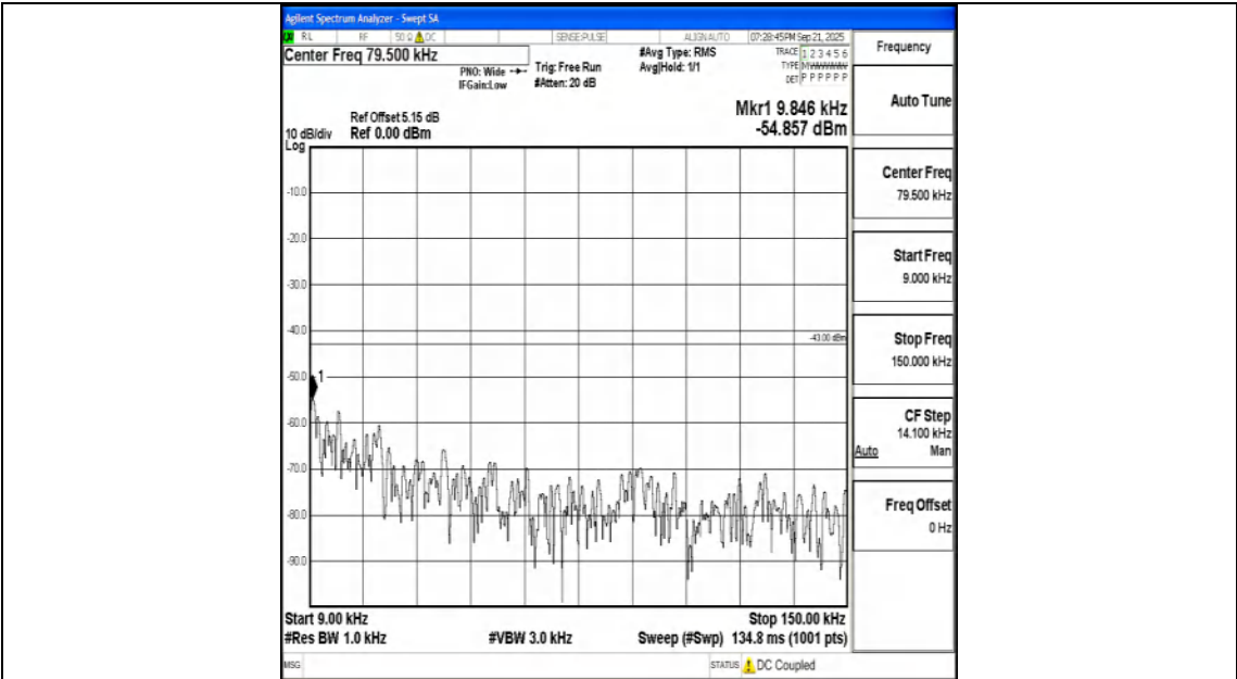
Band25_15MHz_16QAM_26115_1RB#0_0.009~0.15_0.009~0.15
