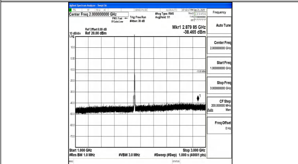
Band25_10MHz_16QAM_26640_1RB#0_1000~3000_1000~3000
