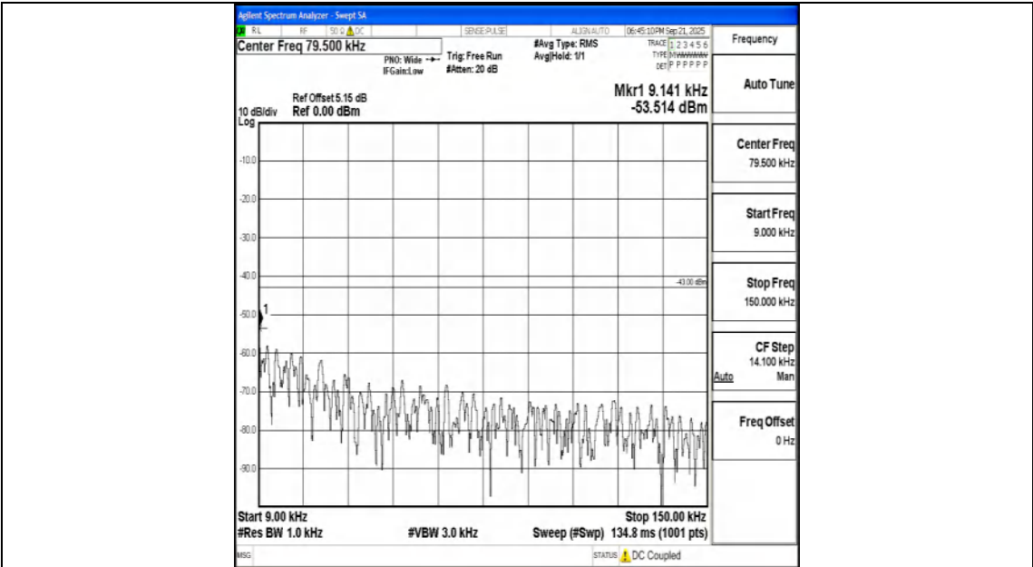
Band25_5MHz_16QAM_26065_1RB#0_0.009~0.15_0.009~0.15
