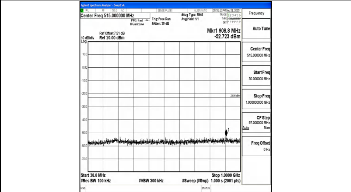
Band25_1.4MHz_QPSK_26365_1RB#0_30~1000_30~1000
