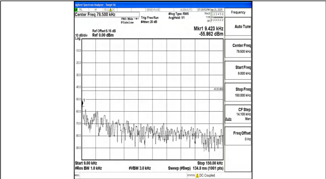
Band25_15MHz_16QAM_26365_1RB#0_0.009~0.15_0.009~0.15
