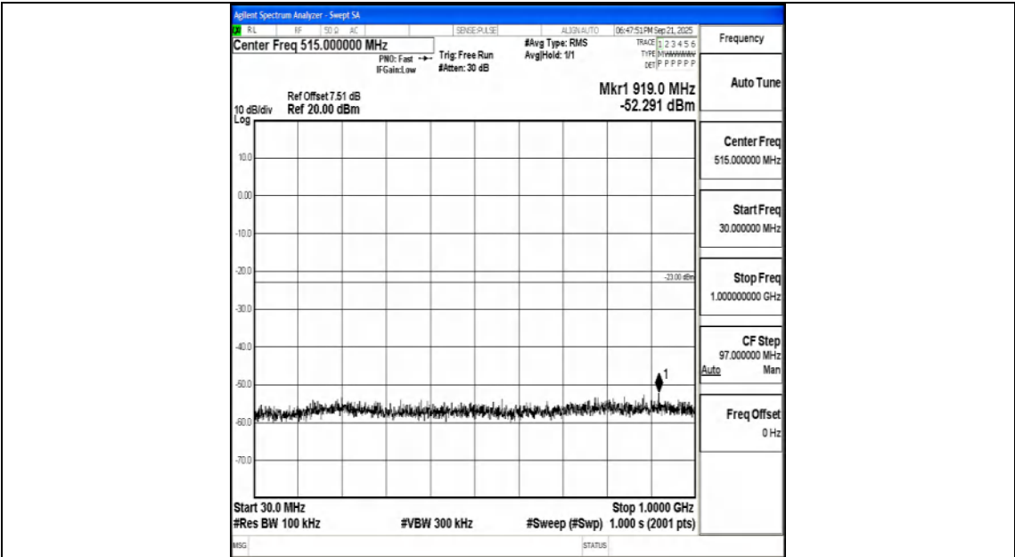
Band25_5MHz_16QAM_26665_1RB#0_30~1000_30~1000
