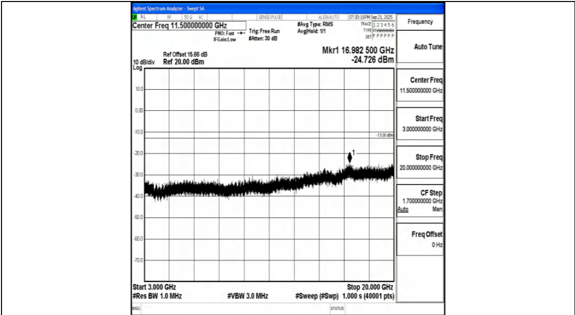
Band25_15MHz_16QAM_26365_1RB#0_3000~20000_3000~20000
