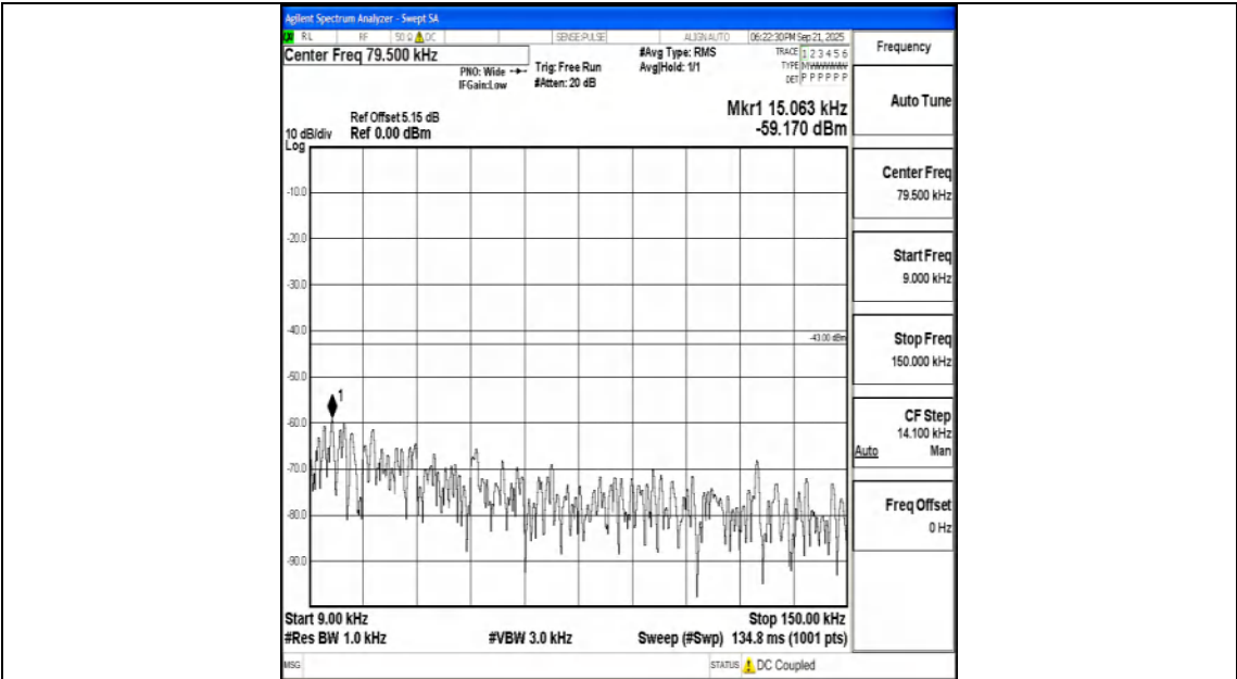
Band25_3MHz_16QAM_26365_1RB#0_0.009~0.15_0.009~0.15
