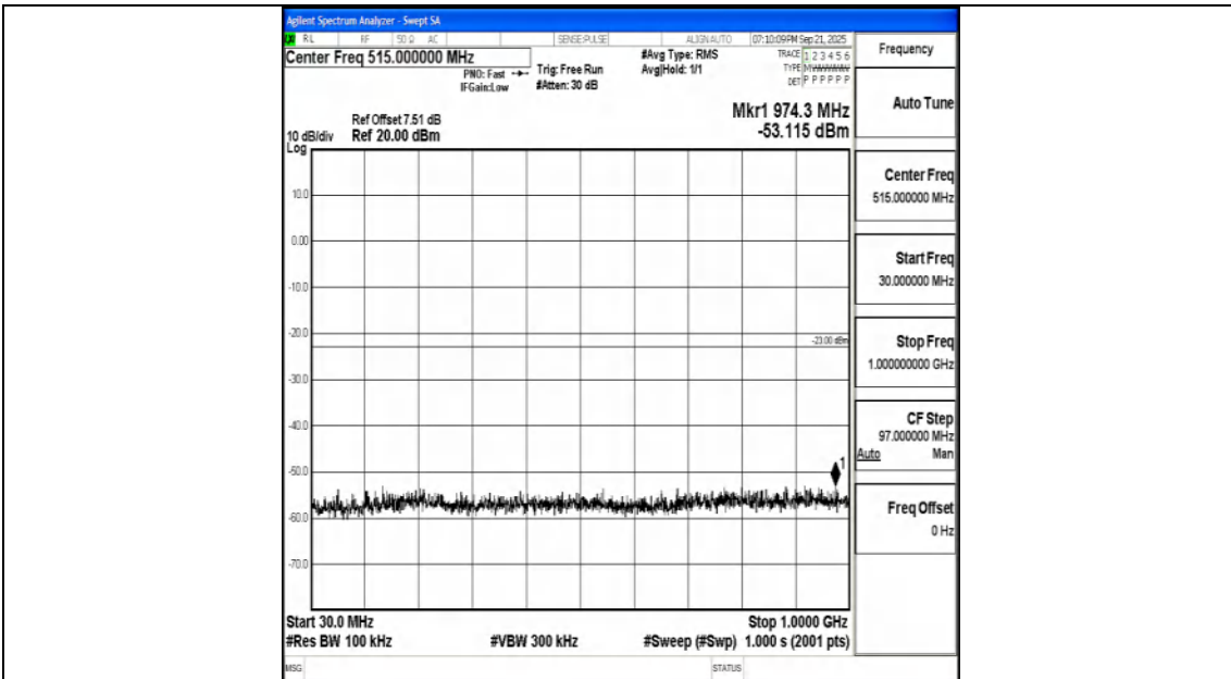
Band25_10MHz_16QAM_26640_1RB#0_30~1000_30~1000
