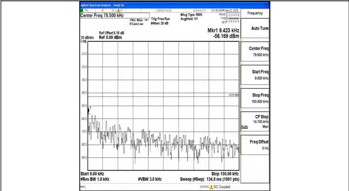
Band25_15MHz_QPSK_26615_1RB#0_0.009~0.15_0.009~0.15
