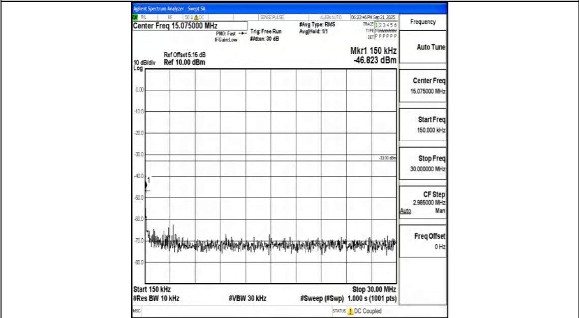
Band25_3MHz_16QAM_26675_1RB#0_0.15~30_0.15~30
