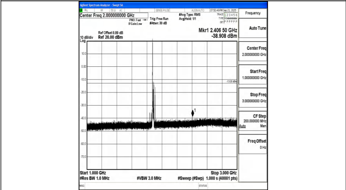
Band25_20MHz_16QAM_26365_1RB#0_1000~3000_1000~3000
