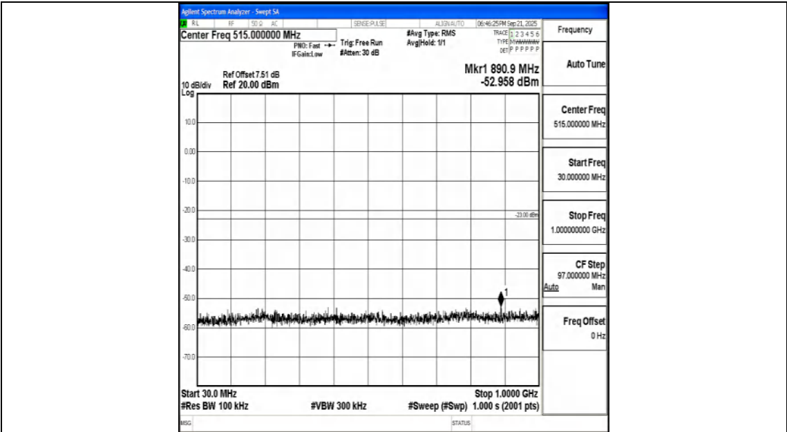
Band25_5MHz_16QAM_26365_1RB#0_30~1000_30~1000
