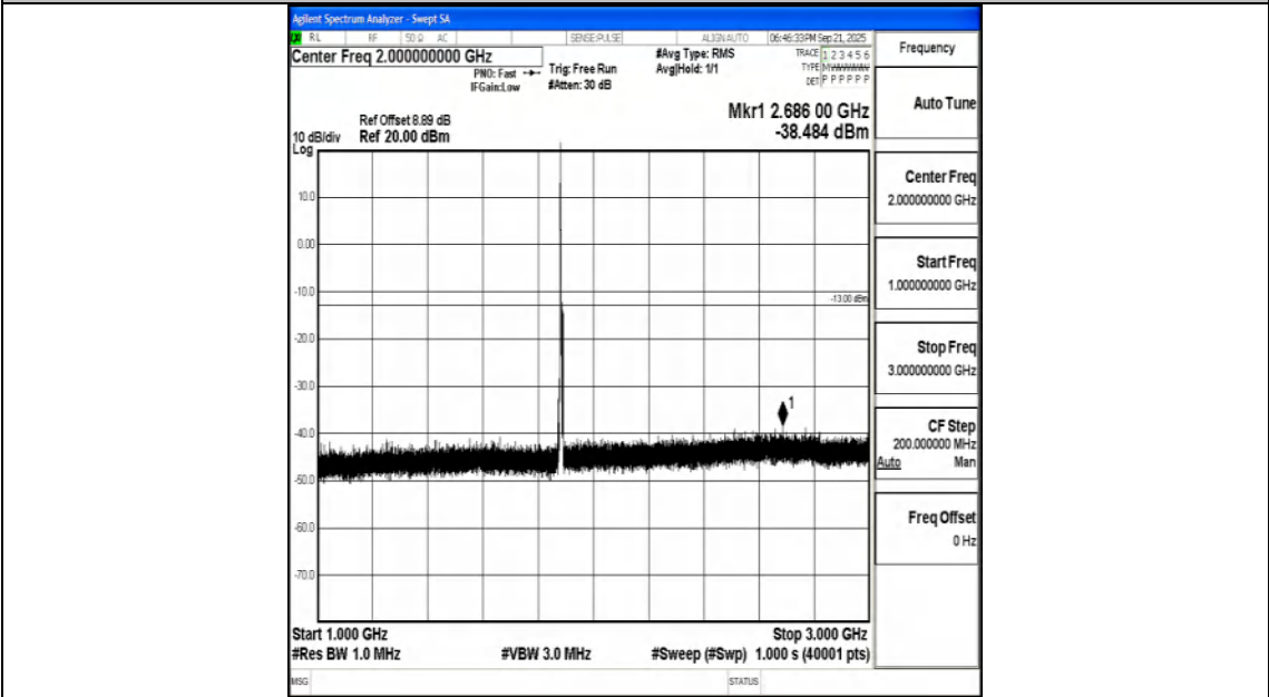
Band25_5MHz_16QAM_26365_1RB#0_1000~3000_1000~3000
