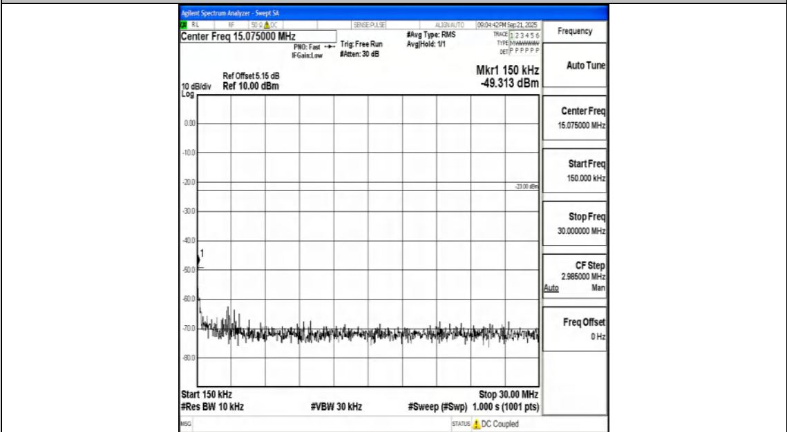
Band26_5MHz_16QAM_26740_1RB#0_0.15~30_0.15~30
