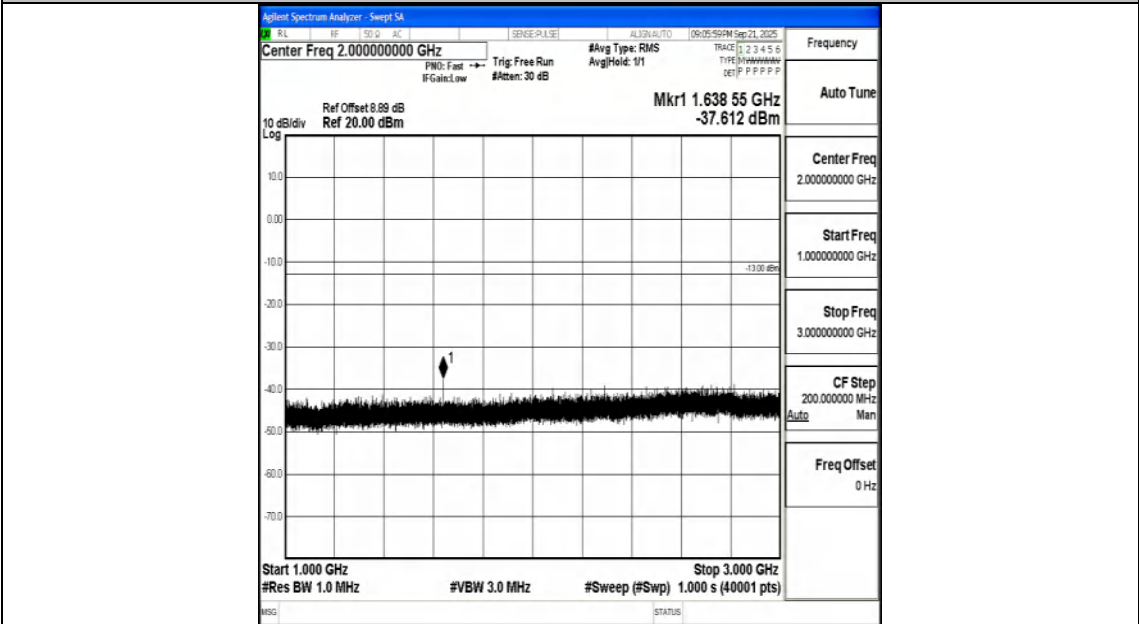
Band26_5MHz_16QAM_26765_1RB#0_1000~3000_1000~3000
