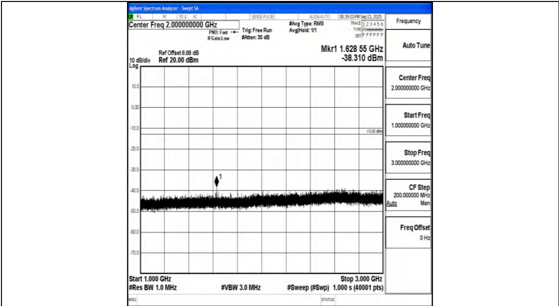
Band26_3MHz_QPSK_26705_1RB#0_1000~3000_1000~3000
