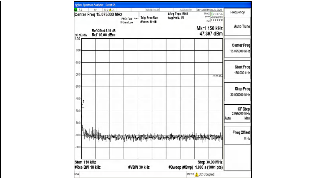
Band26_3MHz_QPSK_26775_1RB#0_0.15~30_0.15~30
