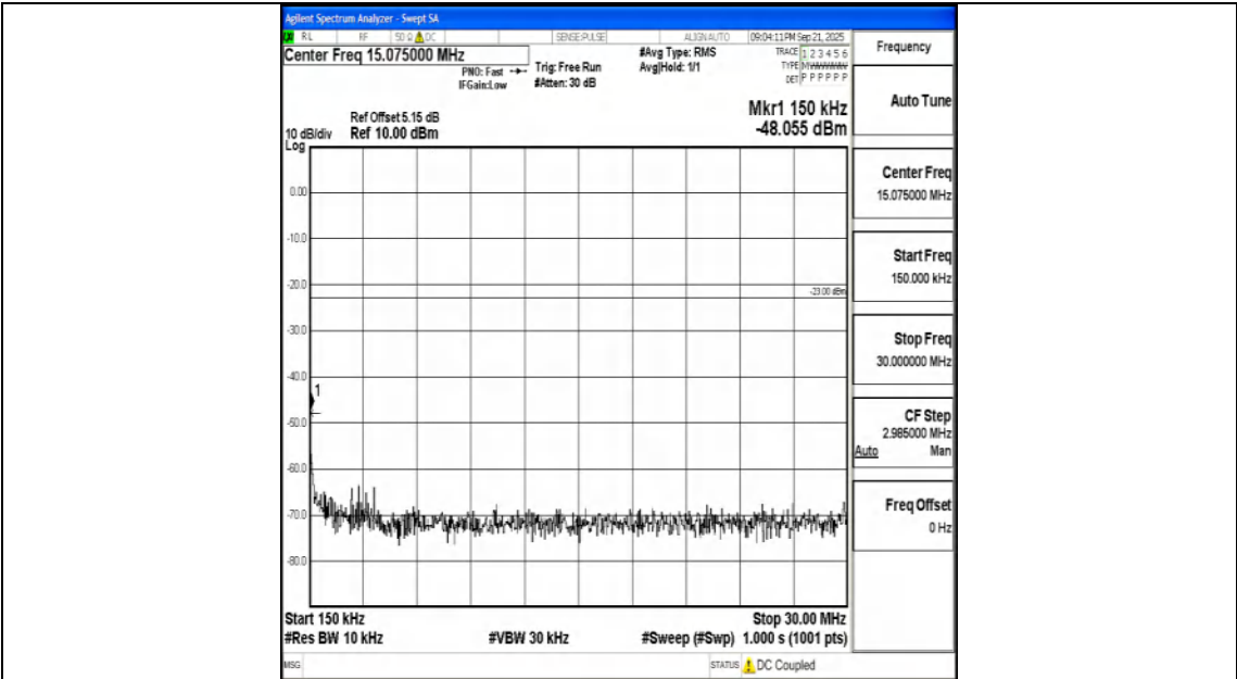
Band26_5MHz_QPSK_26740_1RB#0_0.15~30_0.15~30
