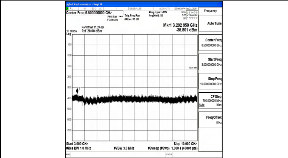
Band26_5MHz_QPSK_26740_1RB#0_3000~10000_3000~10000
