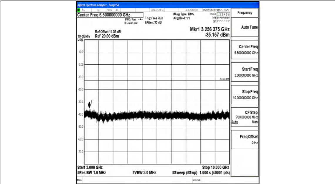
Band26_5MHz_QPSK_26765_1RB#0_3000~10000_3000~10000
