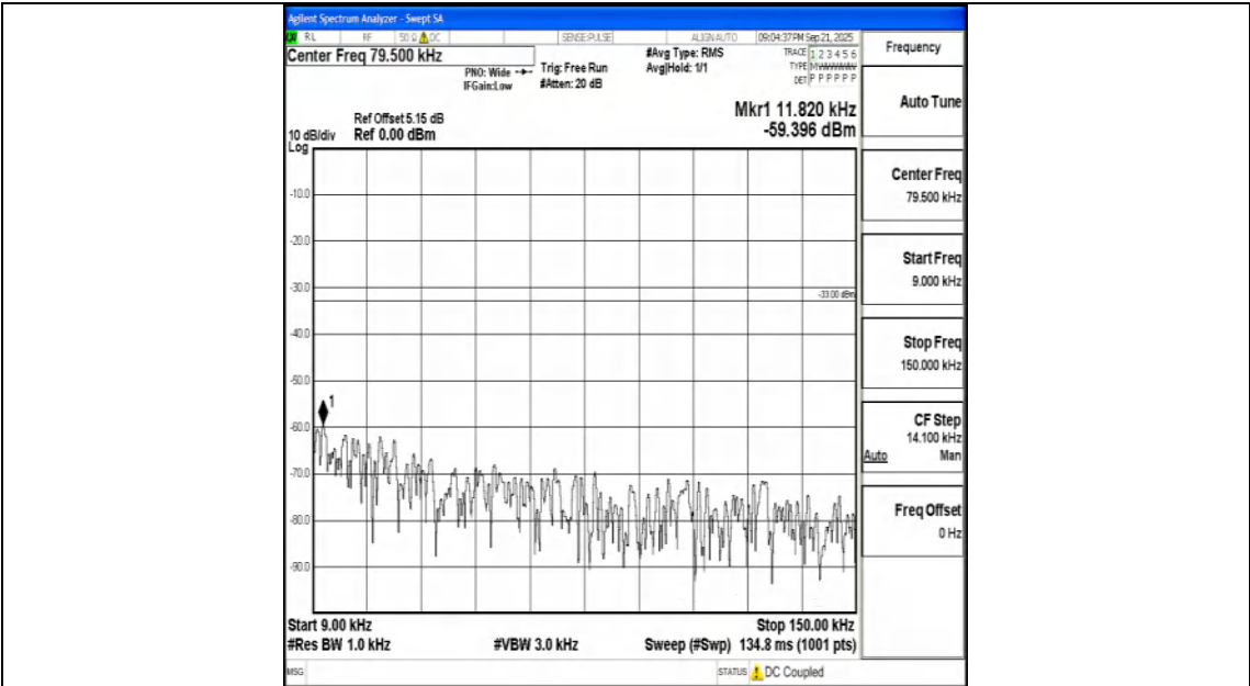
Band26_5MHz_16QAM_26740_1RB#0_0.009~0.15_0.009~0.15
