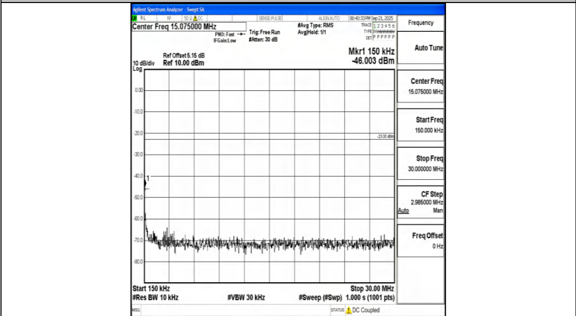
Band26_3MHz_16QAM_26740_1RB#0_0.15~30_0.15~30
