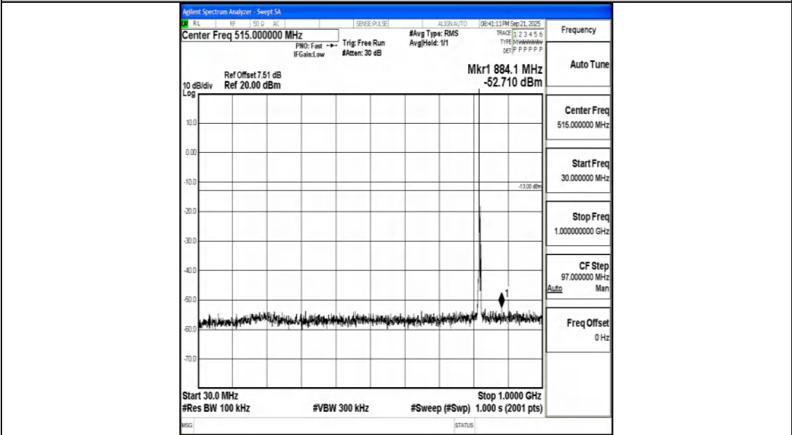
Band26_3MHz_QPSK_26775_1RB#0_30~1000_30~1000
