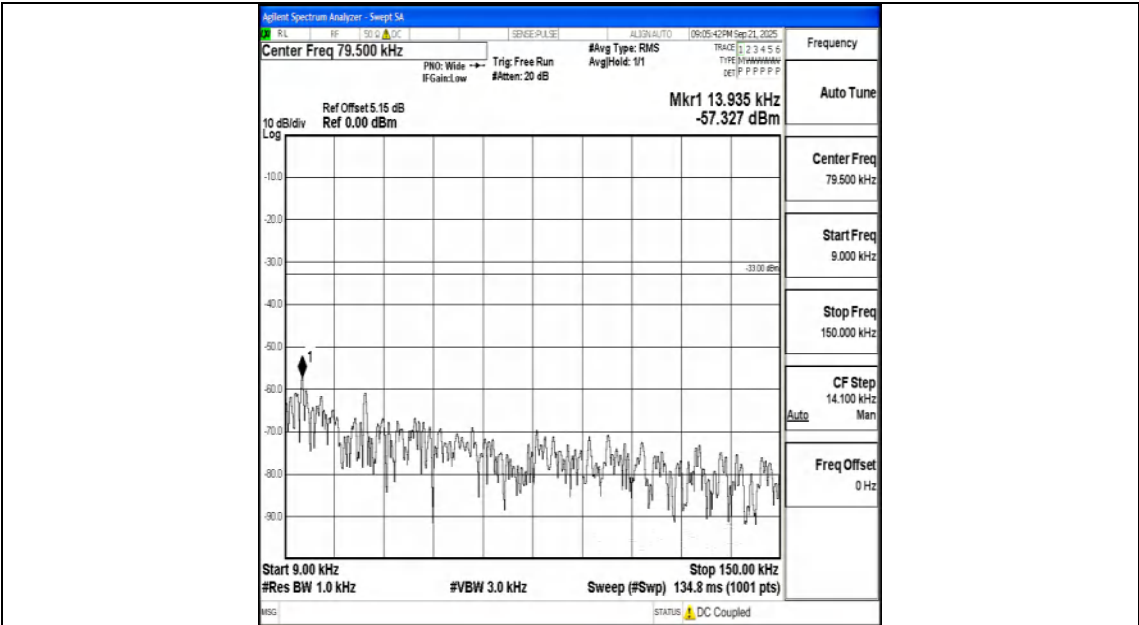
Band26_5MHz_16QAM_26765_1RB#0_0.009~0.15_0.009~0.15
