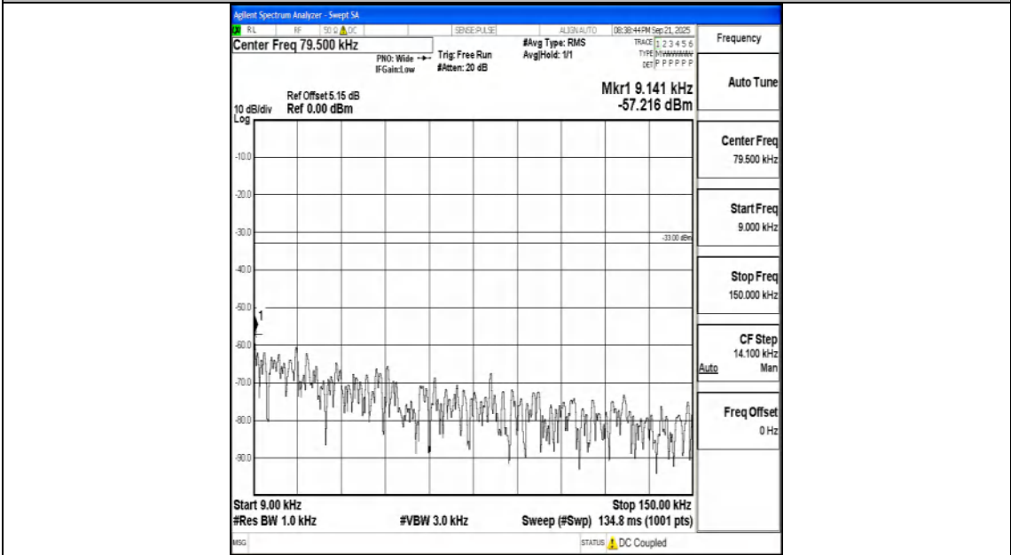
Band26_3MHz_QPSK_26705_1RB#0_0.009~0.15_0.009~0.15
