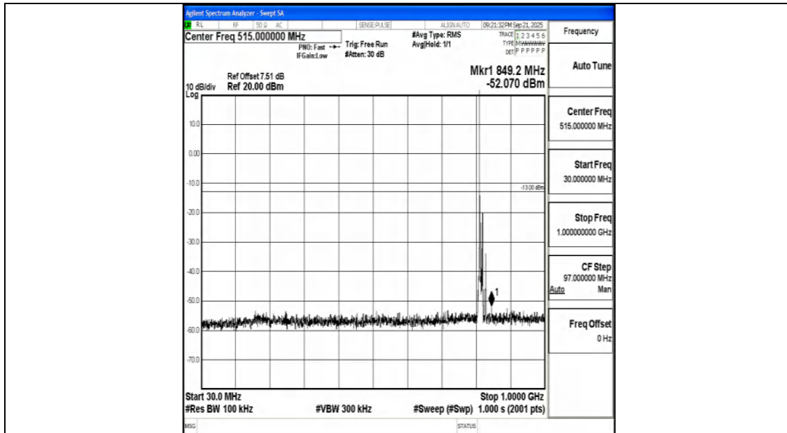
Band26_10MHz_16QAM_26740_1RB#0_30~1000_30~1000
