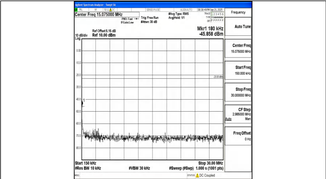
Band26_3MHz_QPSK_26705_1RB#0_0.15~30_0.15~30
