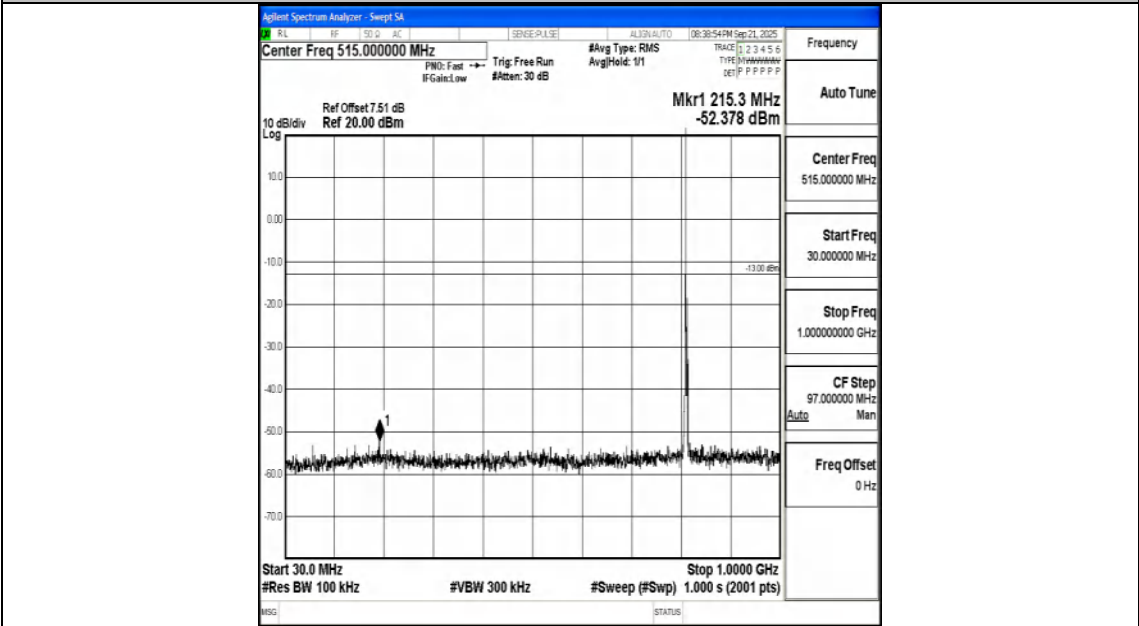
Band26_3MHz_QPSK_26705_1RB#0_30~1000_30~1000
