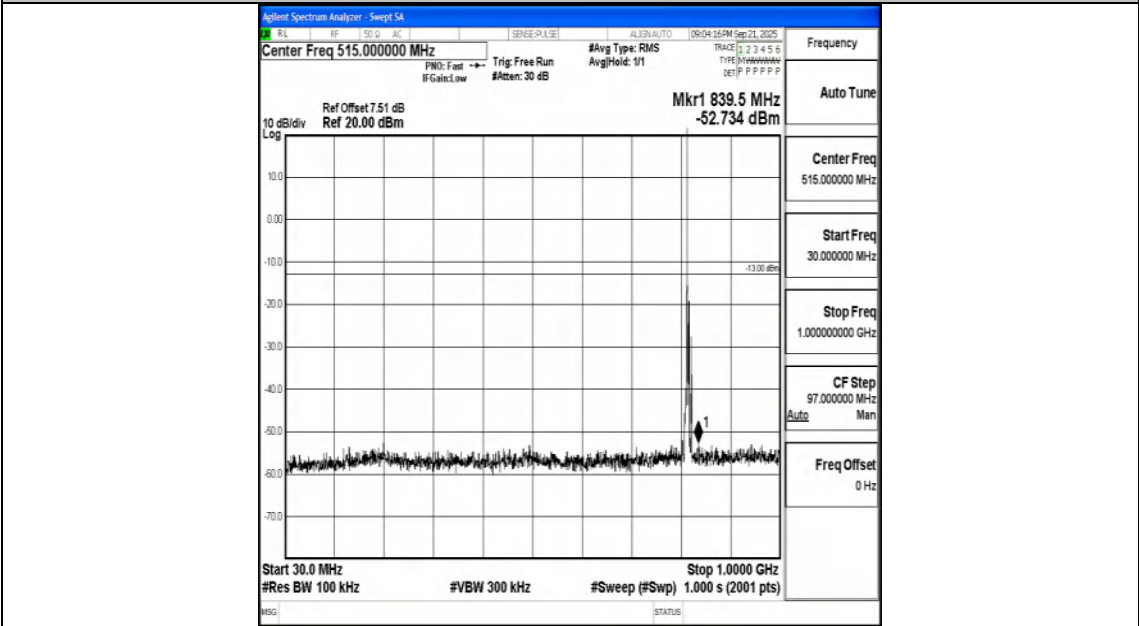
Band26_5MHz_QPSK_26740_1RB#0_30~1000_30~1000
