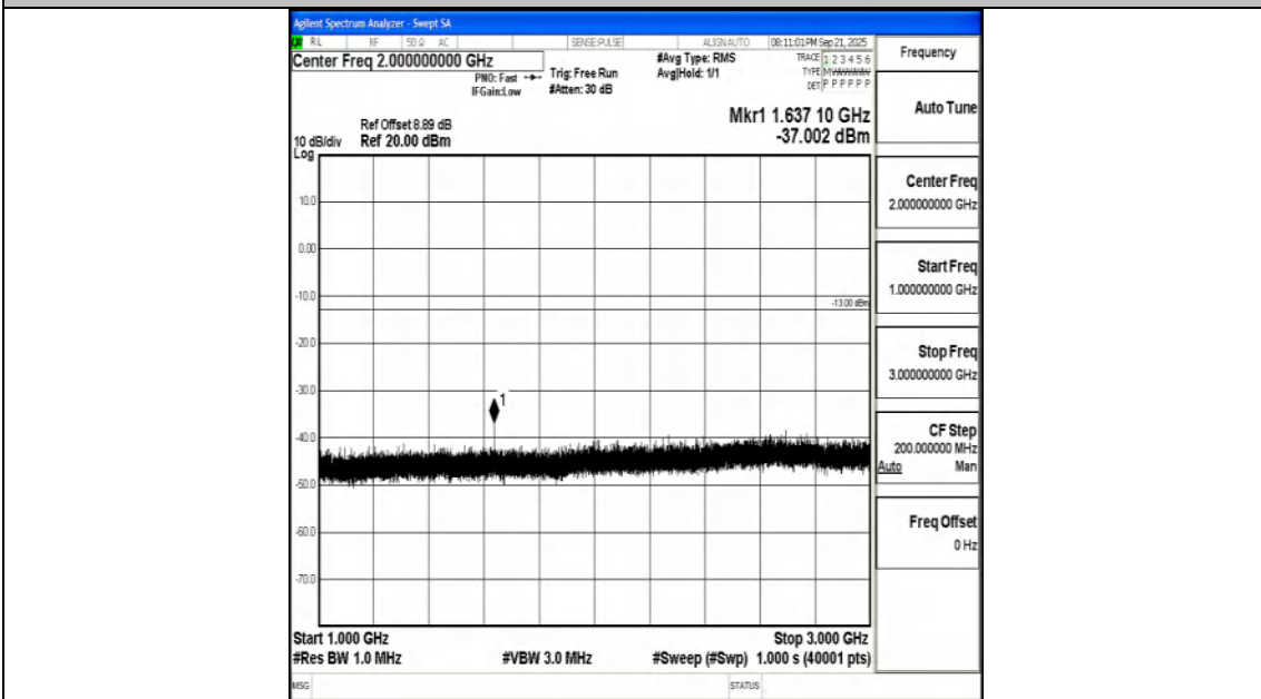
Band26_1.4MHz_16QAM_26740_1RB#0_1000~3000_1000~3000
