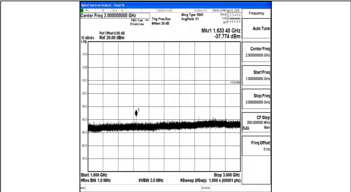
Band26_5MHz_QPSK_26740_1RB#0_1000~3000_1000~3000
