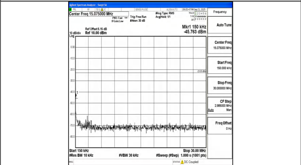
Band26_5MHz_16QAM_26765_1RB#0_0.15~30_0.15~30
