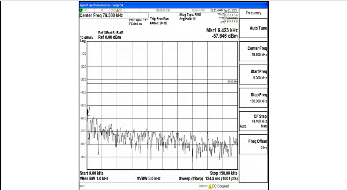
Band26_1.4MHz_16QAM_26783_1RB#0_0.009~0.15_0.009~0.15
