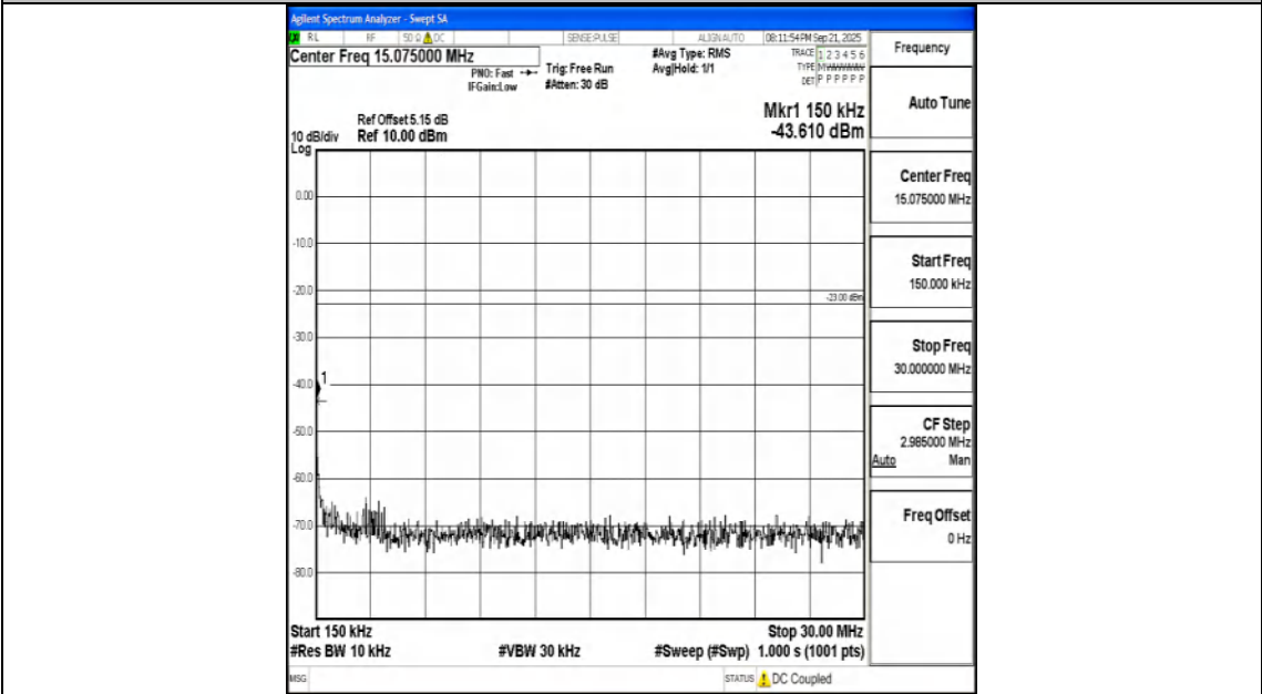
Band26_1.4MHz_16QAM_26783_1RB#0_0.15~30_0.15~30
