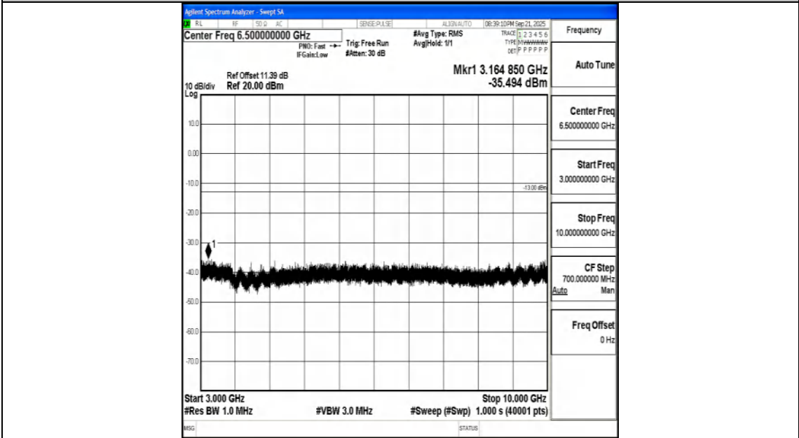
Band26_3MHz_QPSK_26705_1RB#0_3000~10000_3000~10000
