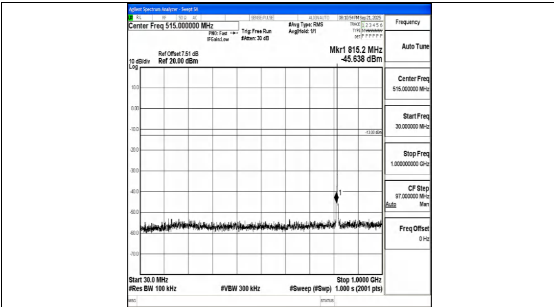
Band26_1.4MHz_16QAM_26740_1RB#0_30~1000_30~1000
