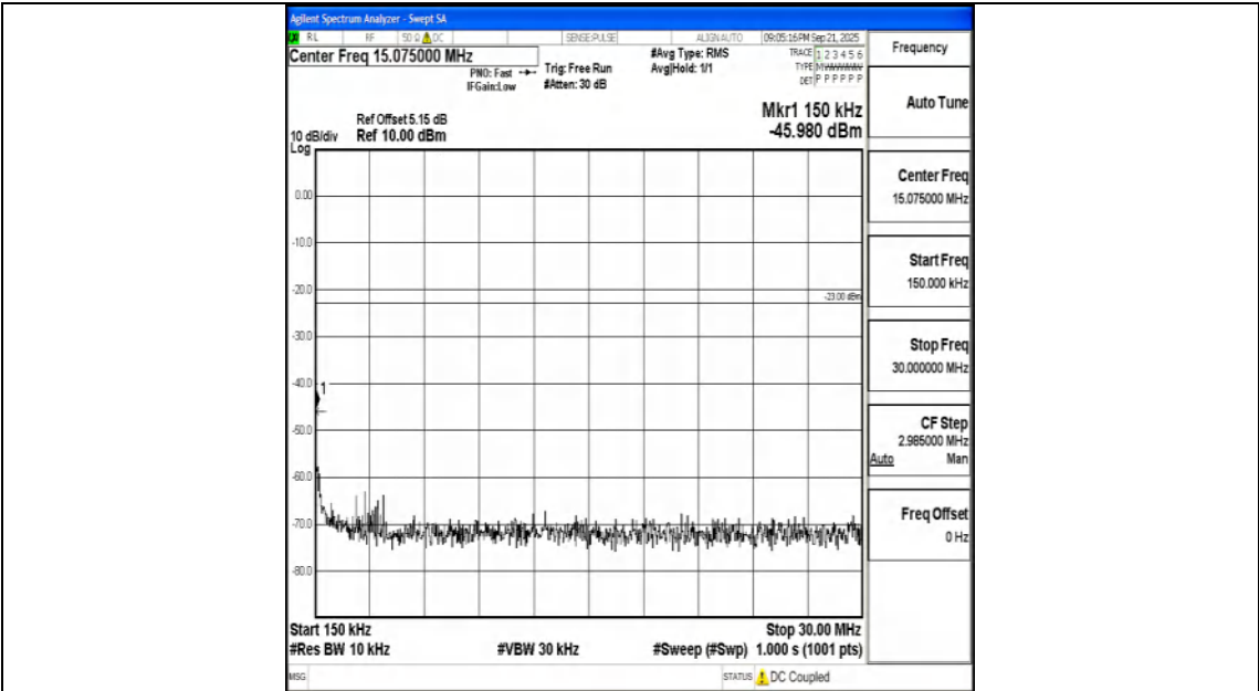
Band26_5MHz_QPSK_26765_1RB#0_0.15~30_0.15~30
