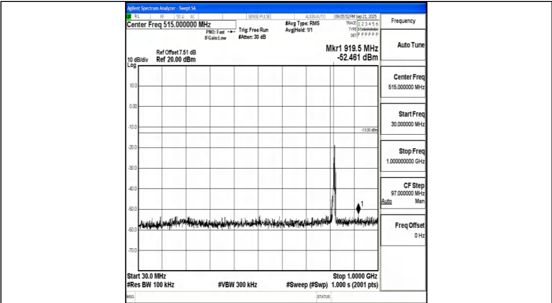
Band26_5MHz_16QAM_26765_1RB#0_30~1000_30~1000
