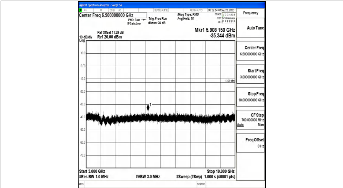
Band26_1.4MHz_16QAM_26783_1RB#0_3000~10000_3000~10000
