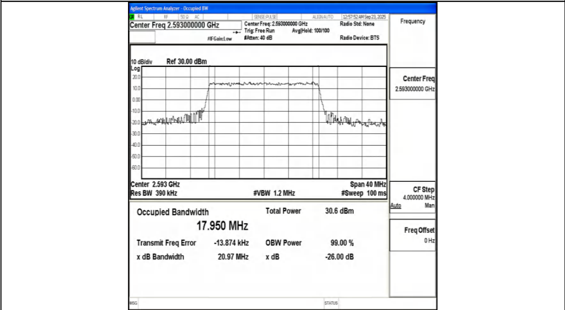
Band41-20MHz-16QAM-40620-100RB#0-PASS
