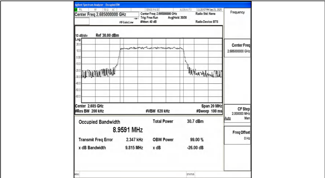
Band41-10MHz-QPSK-41540-50RB#0-PASS
