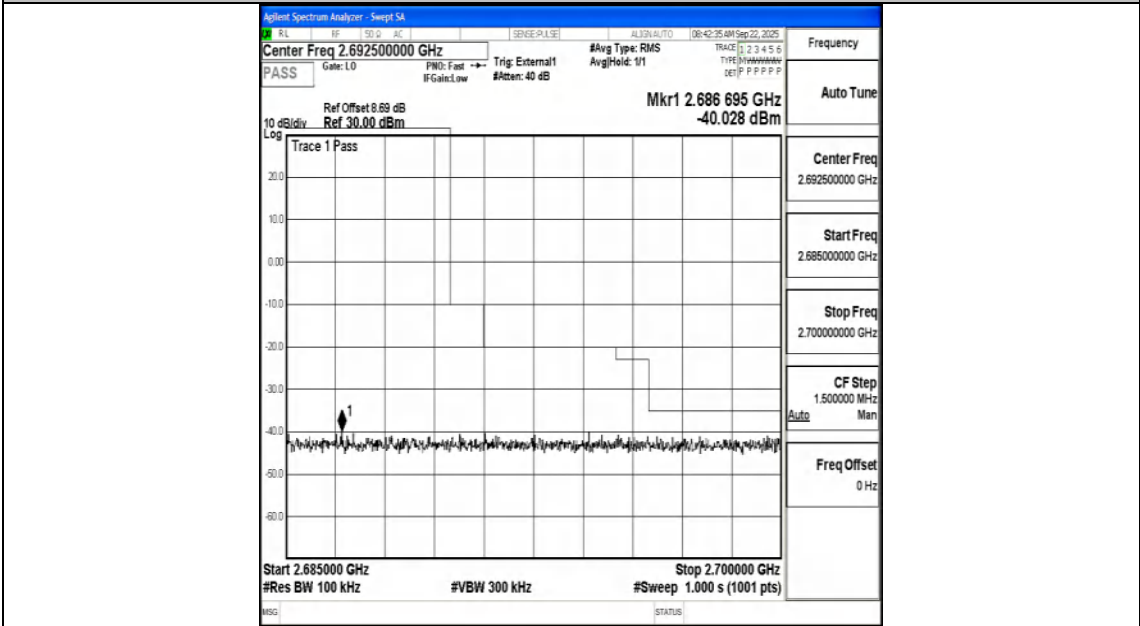
Band41_5MHz_QPSK_41565_25RB#0
