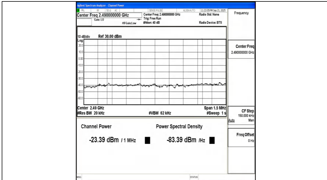
Band41_10MHz_QPSK_39700_50RB#0_Final1
