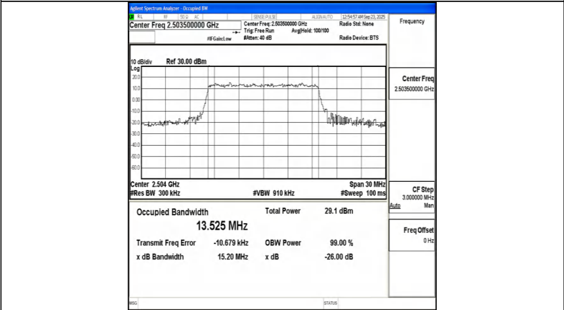
Band41-15MHz-16QAM-39725-75RB#0-PASS
