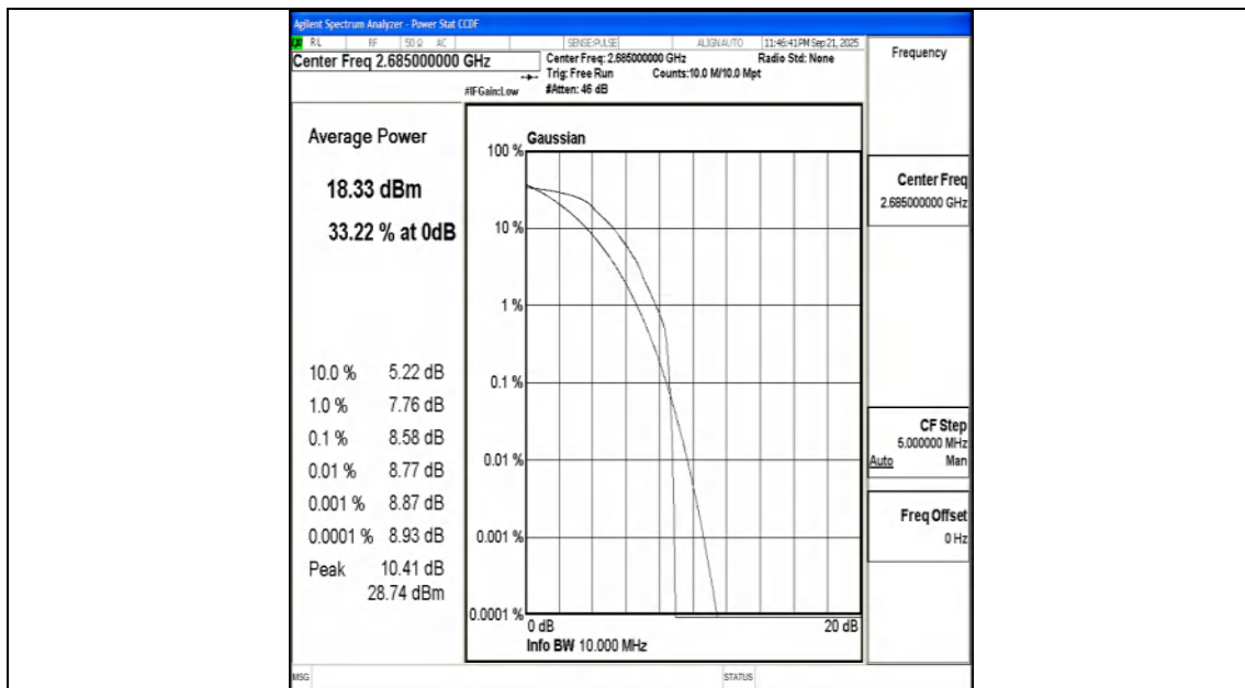
Band41-10MHz-QPSK-41540-1RB#0-PASS
