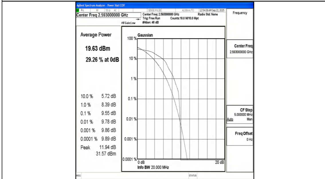
Band41-20MHz-16QAM-40620-1RB#0-PASS
