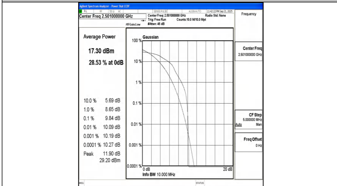
Band41-10MHz-16QAM-39700-1RB#0-PASS
