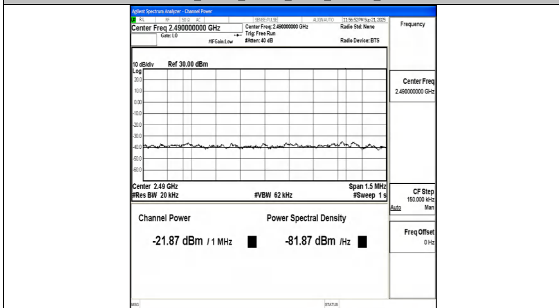
Band41_15MHz_QPSK_39725_75RB#0_Final1
