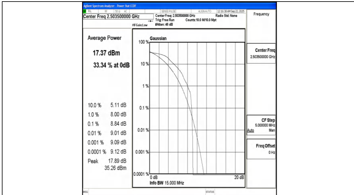
Band41-15MHz-QPSK-39725-1RB#0-PASS
