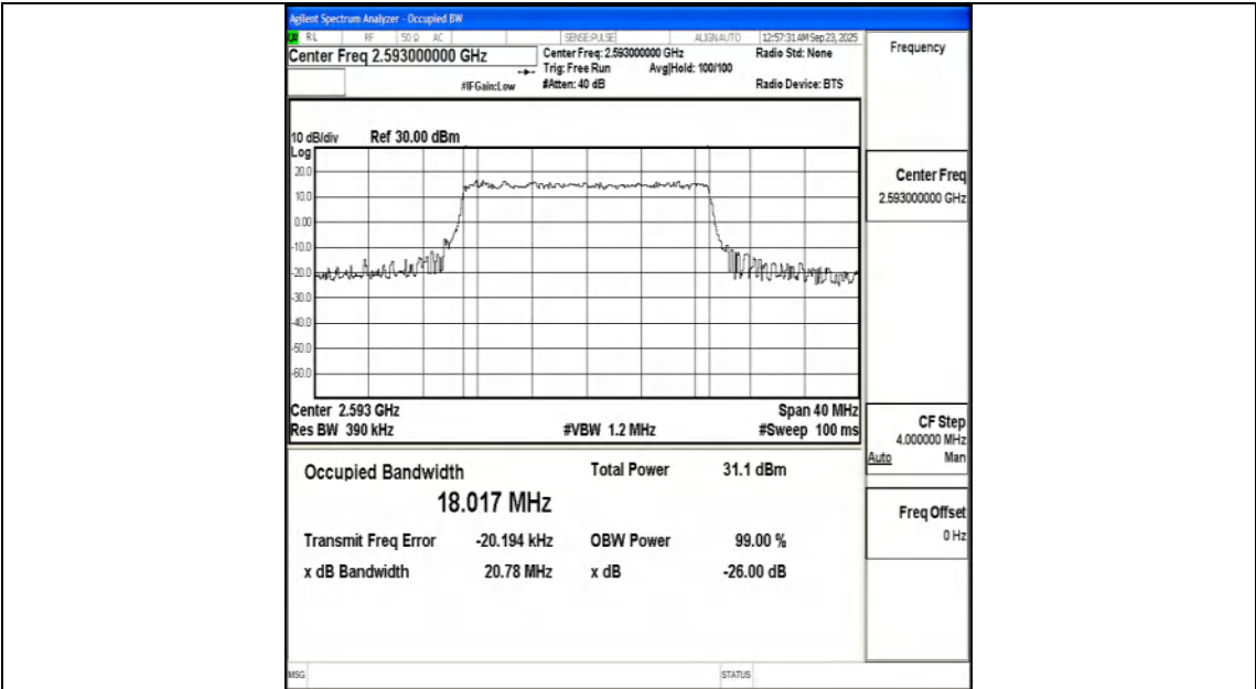
Band41-20MHz-QPSK-40620-100RB#0-PASS
