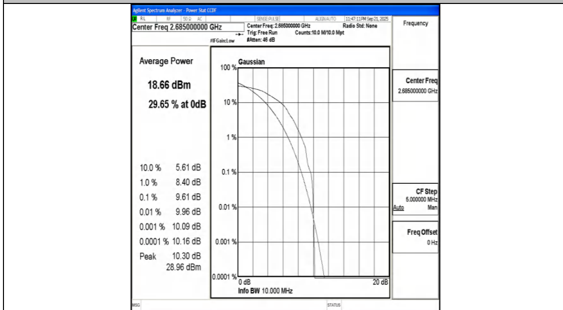
Band41-10MHz-16QAM-41540-1RB#0-PASS
