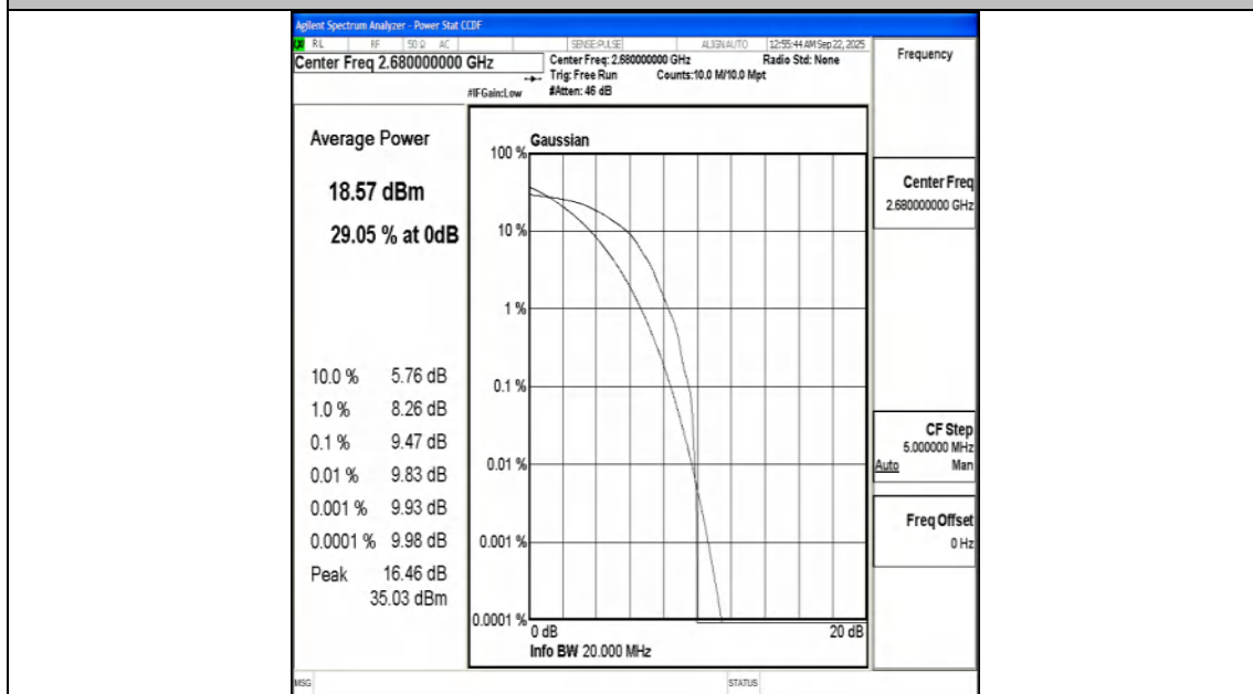
Band41-20MHz-16QAM-41490-1RB#0-PASS
