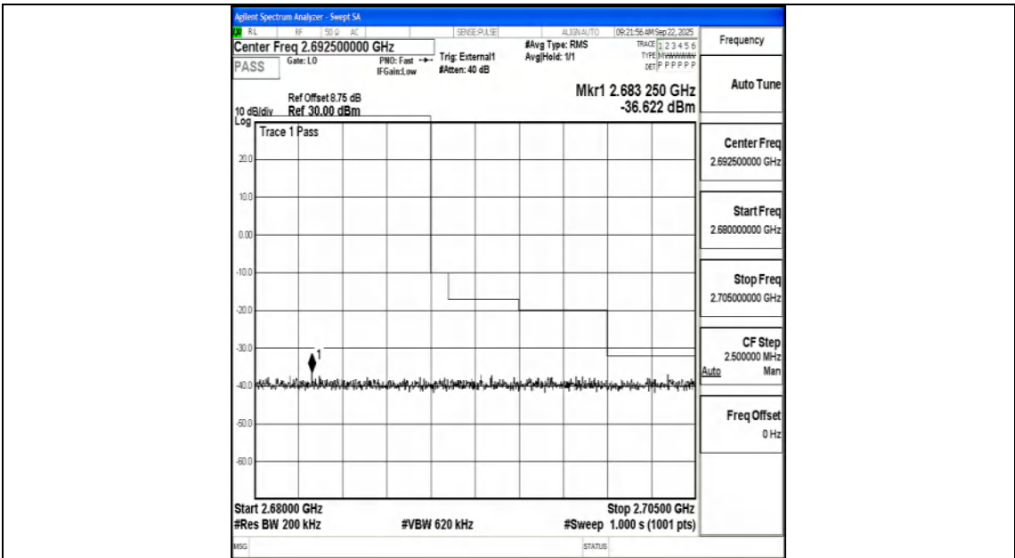
Band41_10MHz_16QAM_41540_50RB#0
