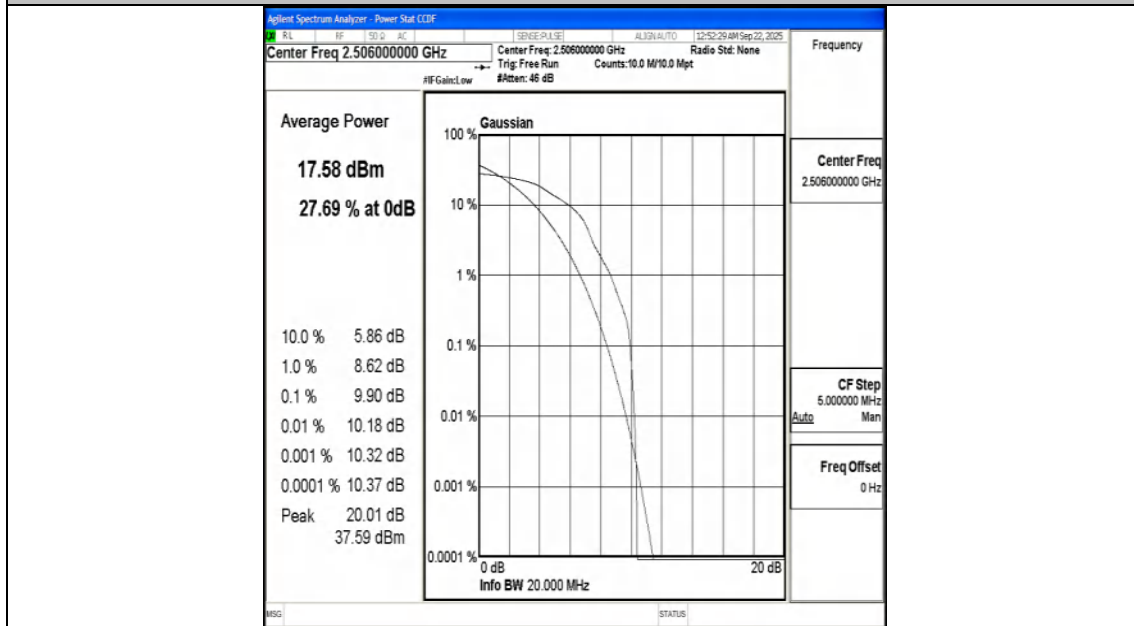
Band41-20MHz-16QAM-39750-1RB#0-PASS
