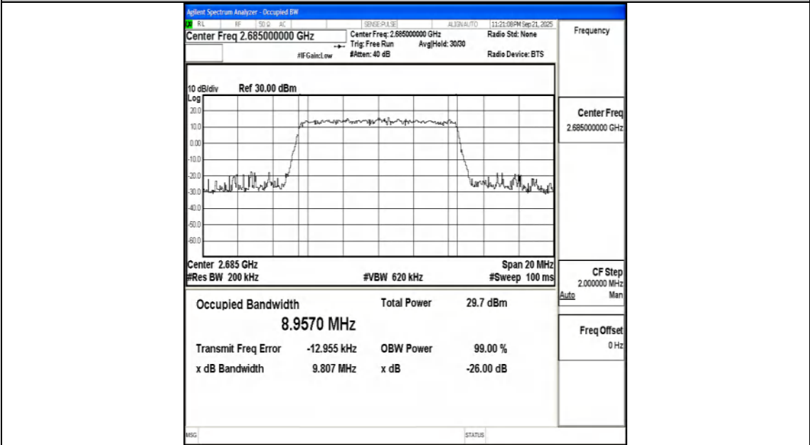
Band41-10MHz-16QAM-41540-50RB#0-PASS
