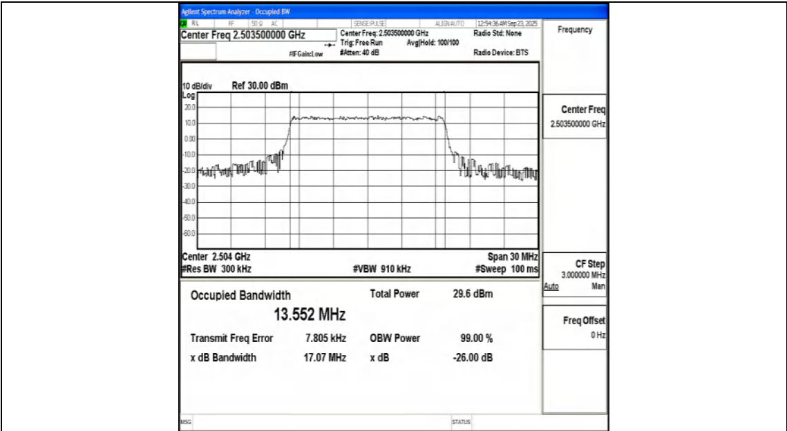
Band41-15MHz-QPSK-39725-75RB#0-PASS
