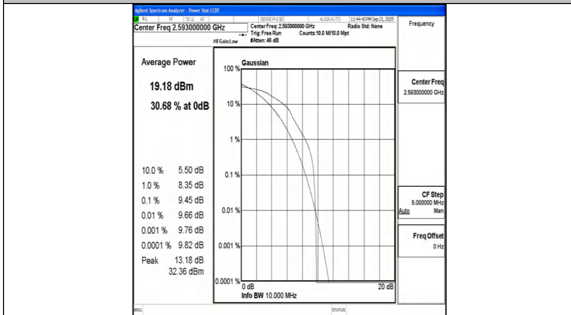
Band41-10MHz-16QAM-40620-1RB#0-PASS
