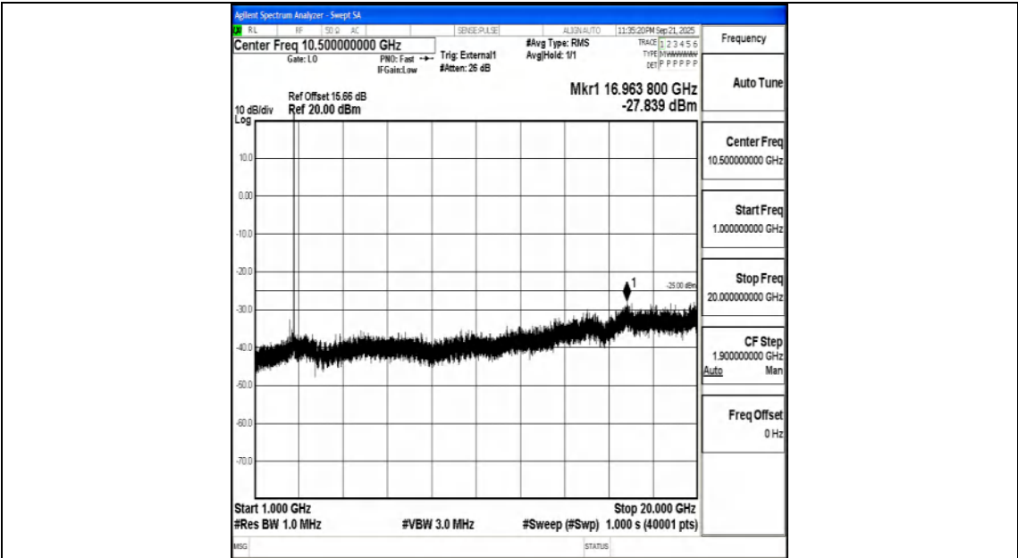
Band41_10MHz_16QAM_41540_1RB#0_1000~20000_1000~20000
