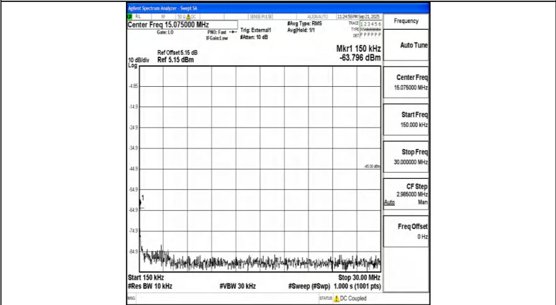
Band41_10MHz_QPSK_39700_1RB#0_0.15~30_0.15~30
