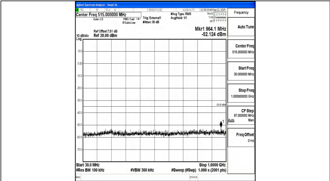
Band41_20MHz_QPSK_40620_1RB#0_30~1000_30~1000
