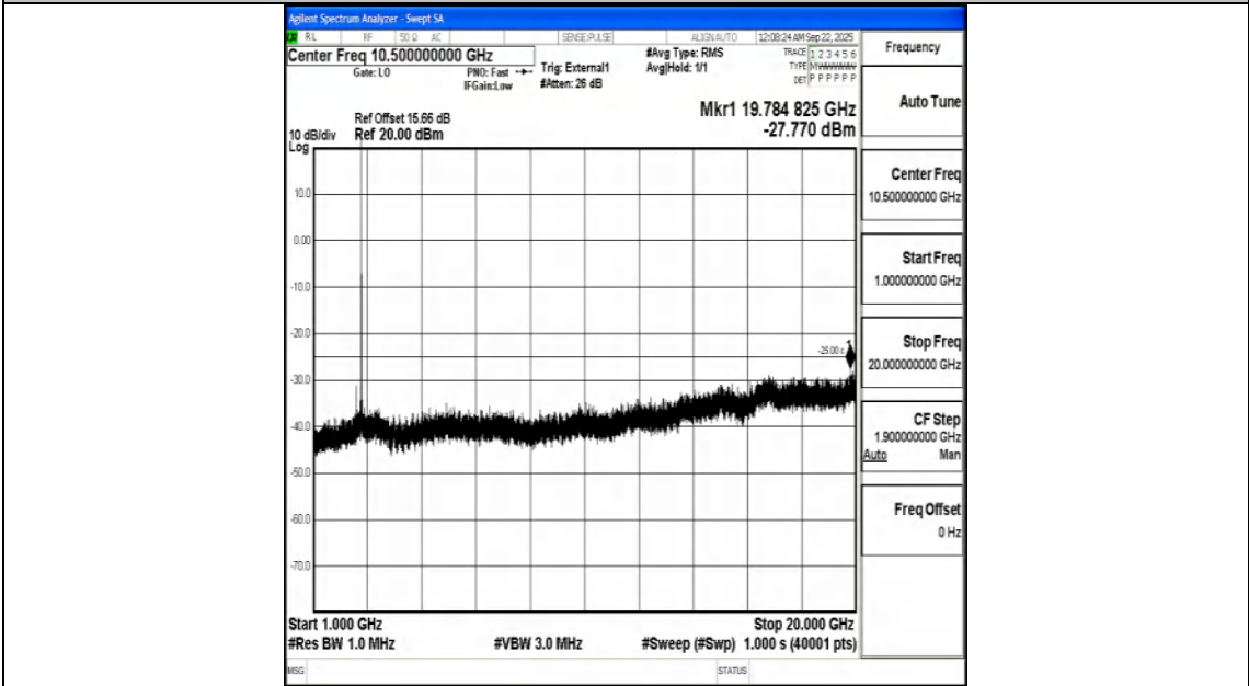
Band41_15MHz_QPSK_41515_1RB#0_1000~20000_1000~20000
