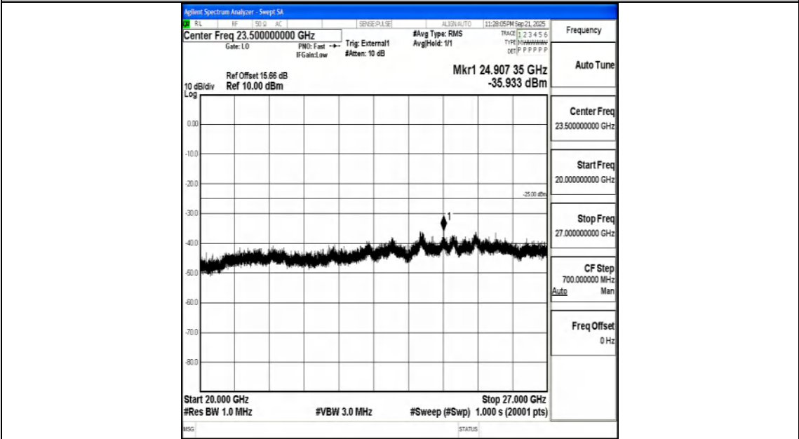
Band41_10MHz_16QAM_39700_1RB#0_20000~27000_20000~27000
