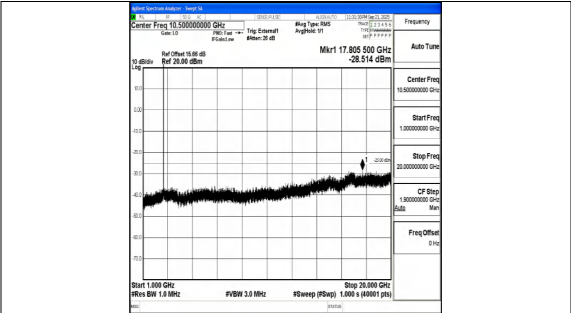
Band41_10MHz_16QAM_40620_1RB#0_1000~20000_1000~20000
