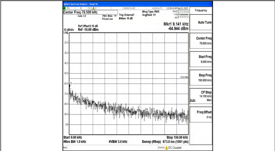
Band41_20MHz_16QAM_39750_1RB#0_0.009~0.15_0.009~0.15
