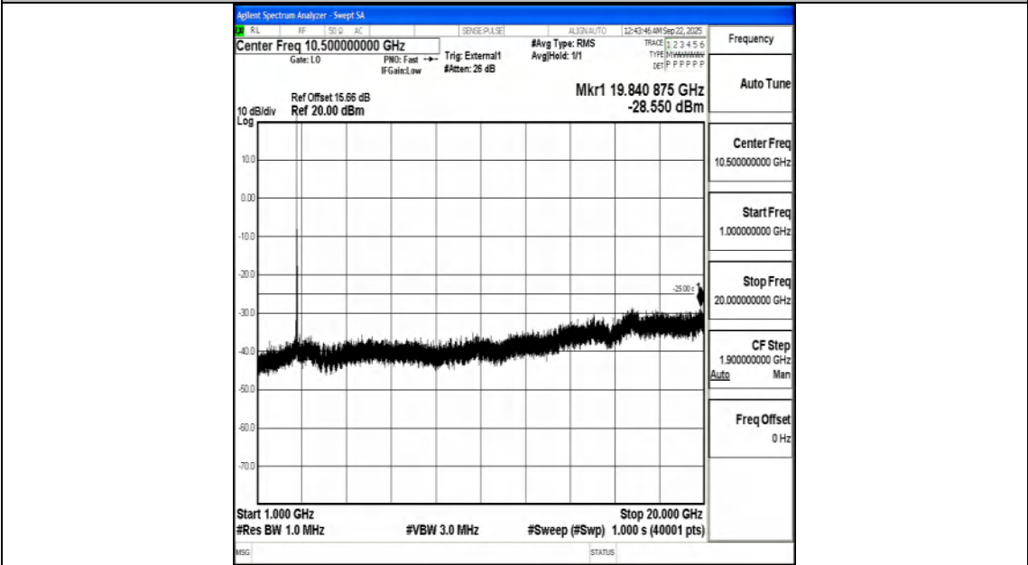
Band41_20MHz_QPSK_41490_1RB#0_1000~20000_1000~20000
