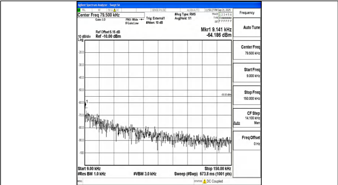
Band41_15MHz_QPSK_39725_1RB#0_0.009~0.15_0.009~0.15
