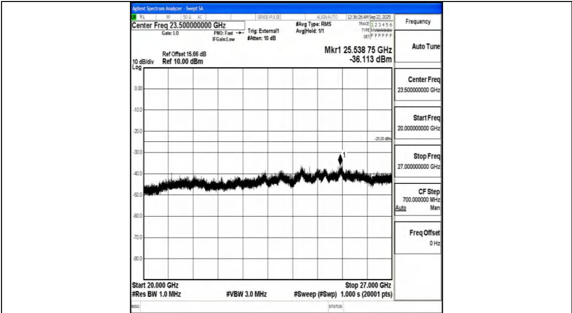
Band41_20MHz_QPSK_39750_1RB#0_20000~27000_20000~27000
