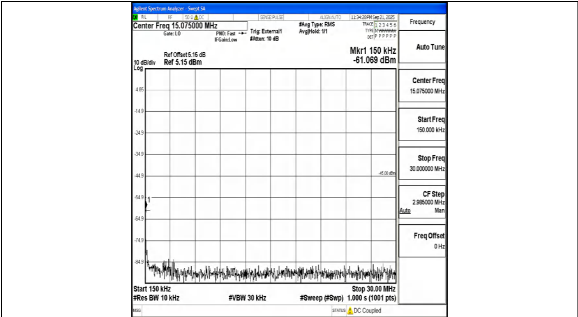
Band41_10MHz_16QAM_41540_1RB#0_0.15~30_0.15~30
