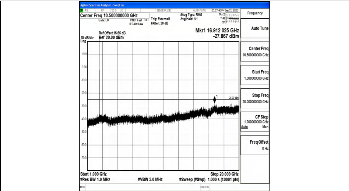
Band41_10MHz_16QAM_39700_1RB#0_1000~20000_1000~20000
