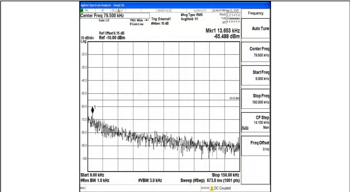
Band41_5MHz_QPSK_40620_1RB#0_0.009~0.15_0.009~0.15
