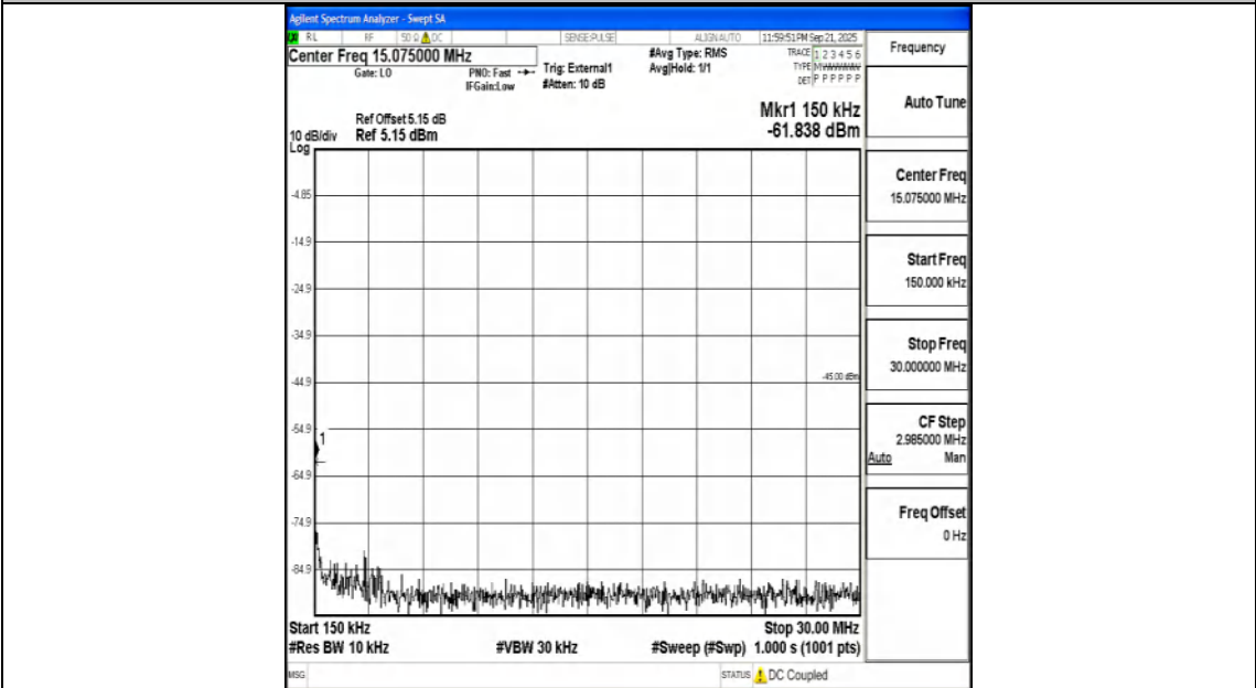
Band41_15MHz_QPSK_39725_1RB#0_0.15~30_0.15~30
