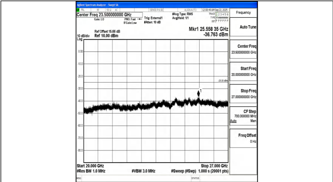
Band41_15MHz_QPSK_41515_1RB#0_20000~27000_20000~27000
