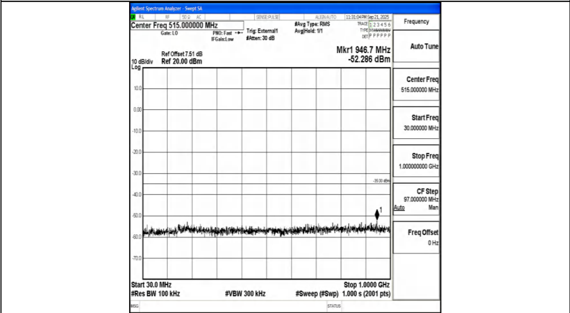
Band41_10MHz_16QAM_40620_1RB#0_30~1000_30~1000
