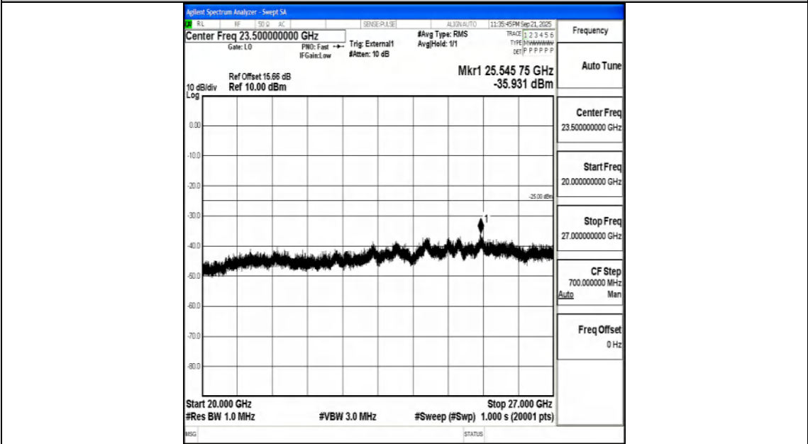
Band41_10MHz_16QAM_41540_1RB#0_20000~27000_20000~27000
