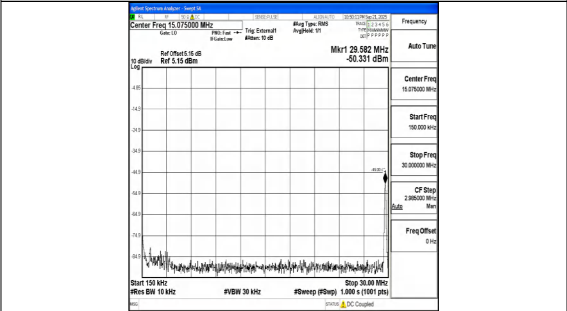
Band41_5MHz_QPSK_40620_1RB#0_0.15~30_0.15~30
