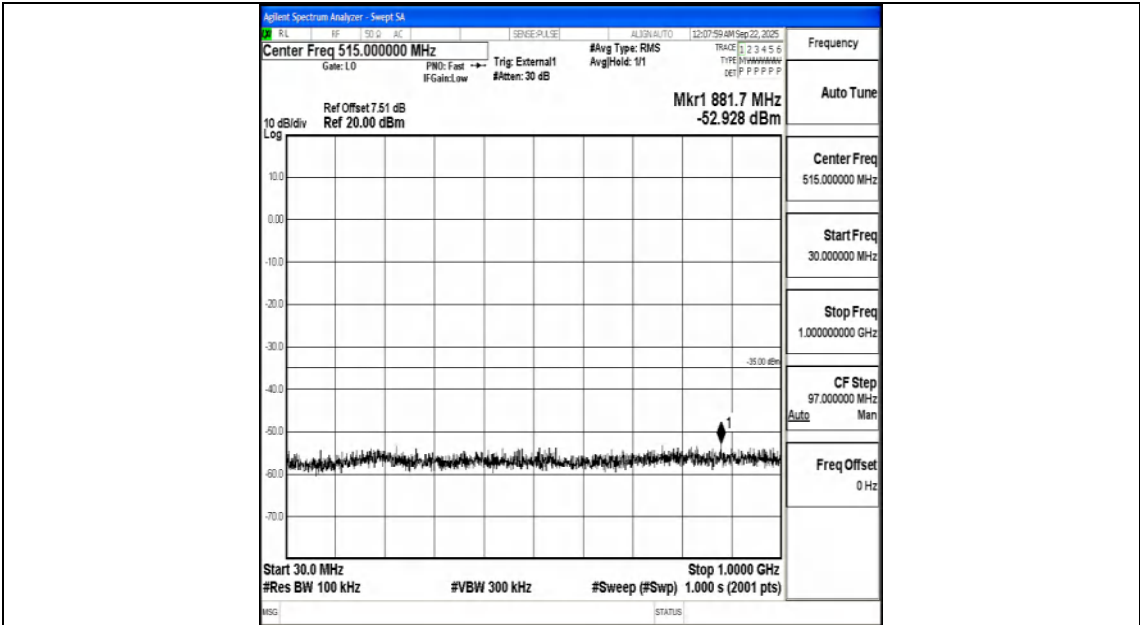
Band41_15MHz_QPSK_41515_1RB#0_30~1000_30~1000
