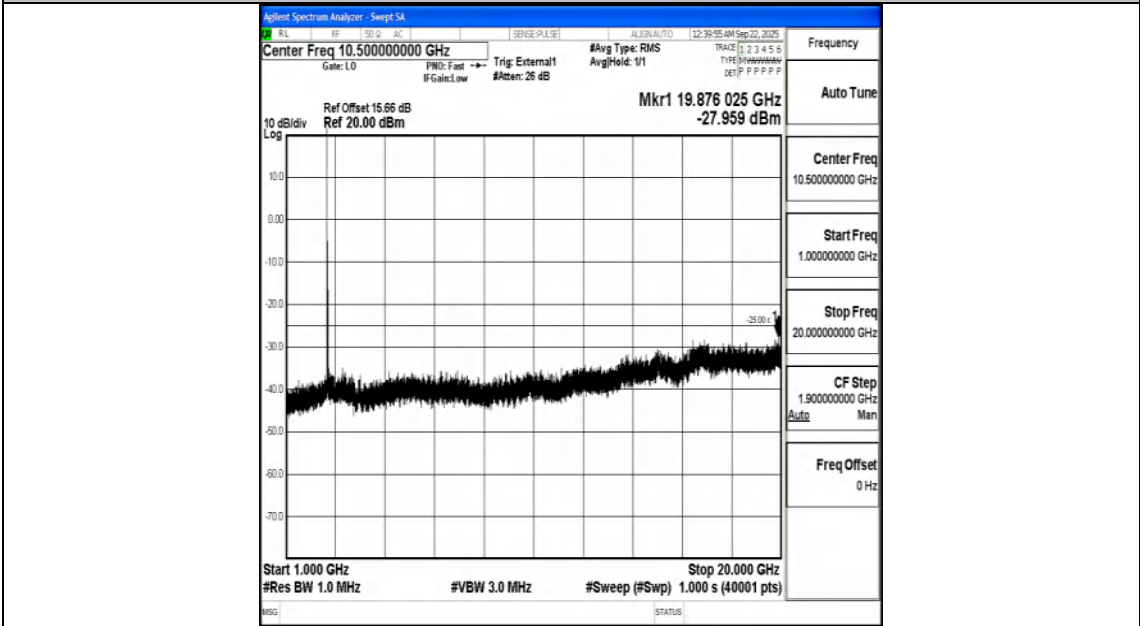
Band41_20MHz_QPSK_40620_1RB#0_1000~20000_1000~20000
