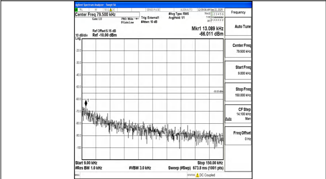
Band41_15MHz_16QAM_41515_1RB#0_0.009~0.15_0.009~0.15
