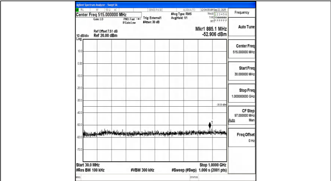
Band41_15MHz_QPSK_40620_1RB#0_30~1000_30~1000
