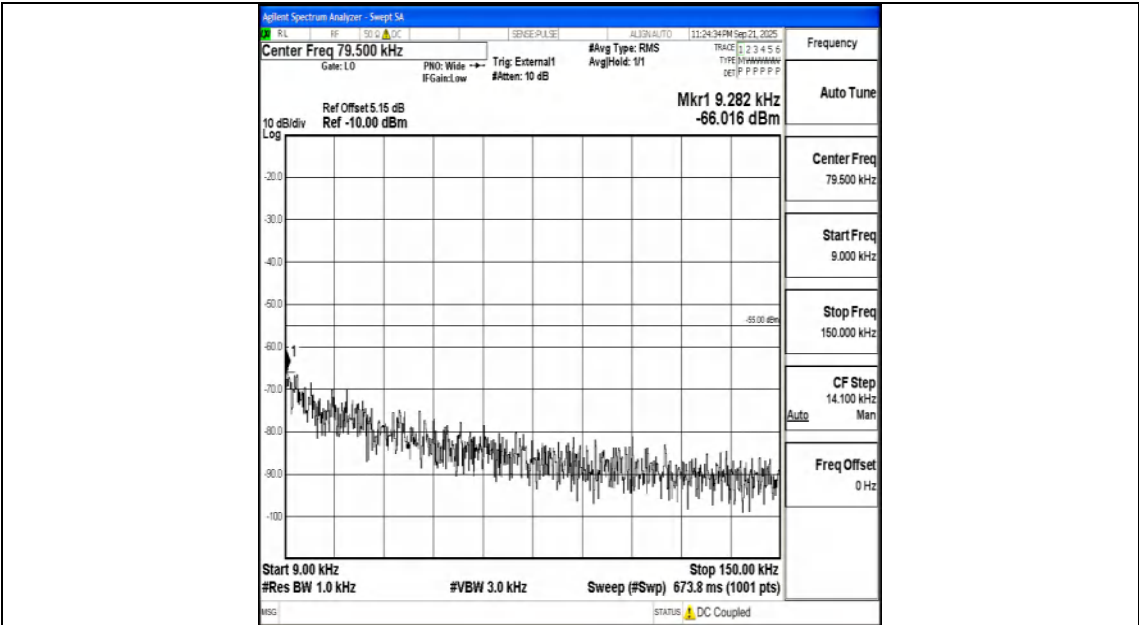
Band41_10MHz_QPSK_39700_1RB#0_0.009~0.15_0.009~0.15
