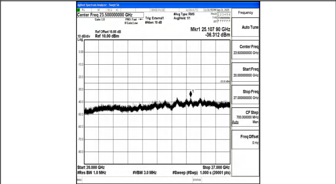
Band41_10MHz_16QAM_40620_1RB#0_20000~27000_20000~27000
