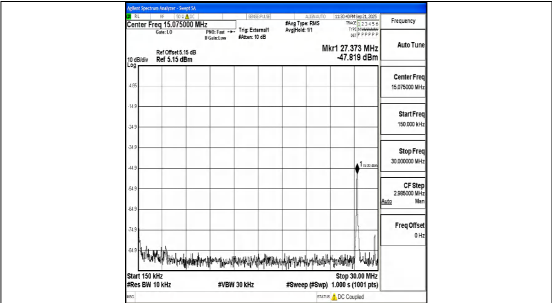
Band41_10MHz_16QAM_40620_1RB#0_0.15~30_0.15~30
