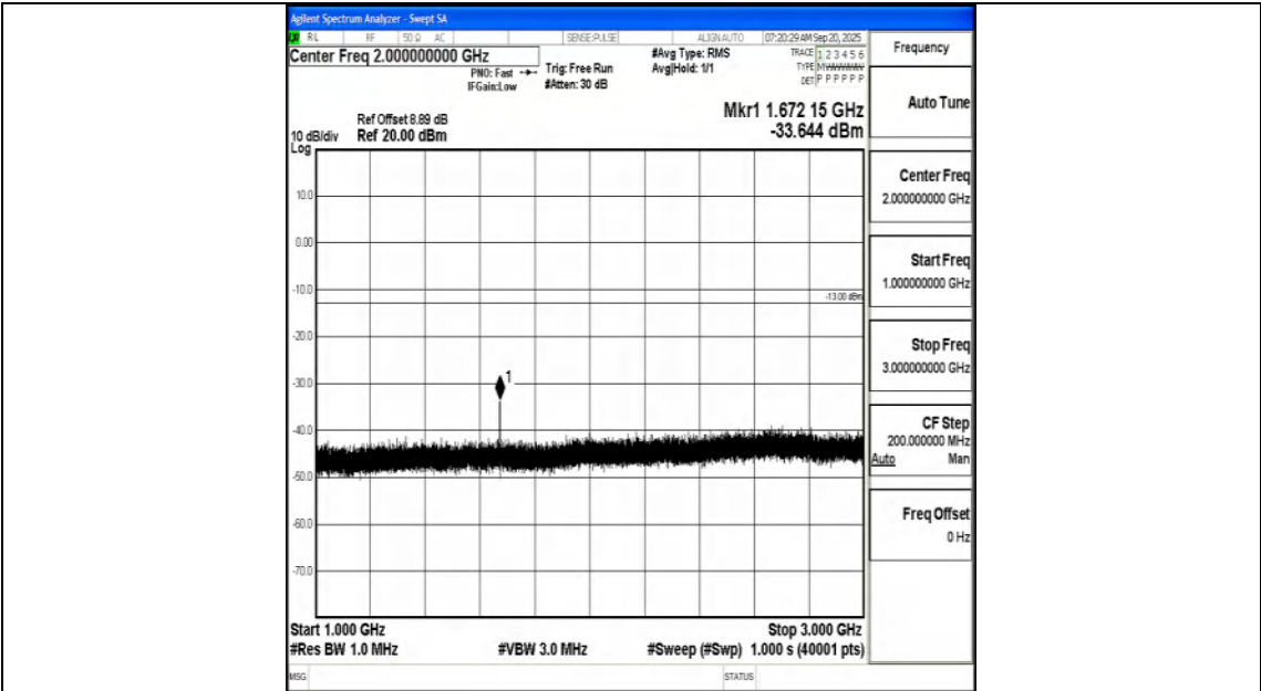
Band5_1.4MHz_16QAM_20525_1RB#0_1000~3000_1000~3000
