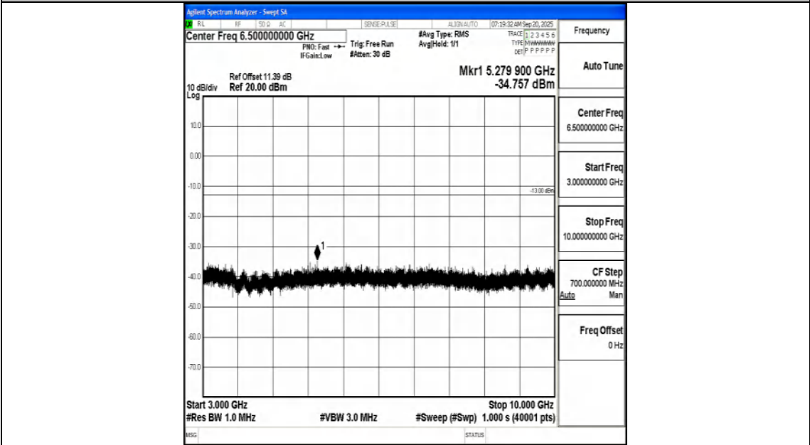
Band5_1.4MHz_16QAM_20407_1RB#0_3000~10000_3000~10000
