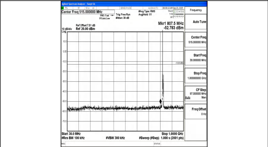
Band5_5MHz_16QAM_20425_1RB#0_30~1000_30~1000
