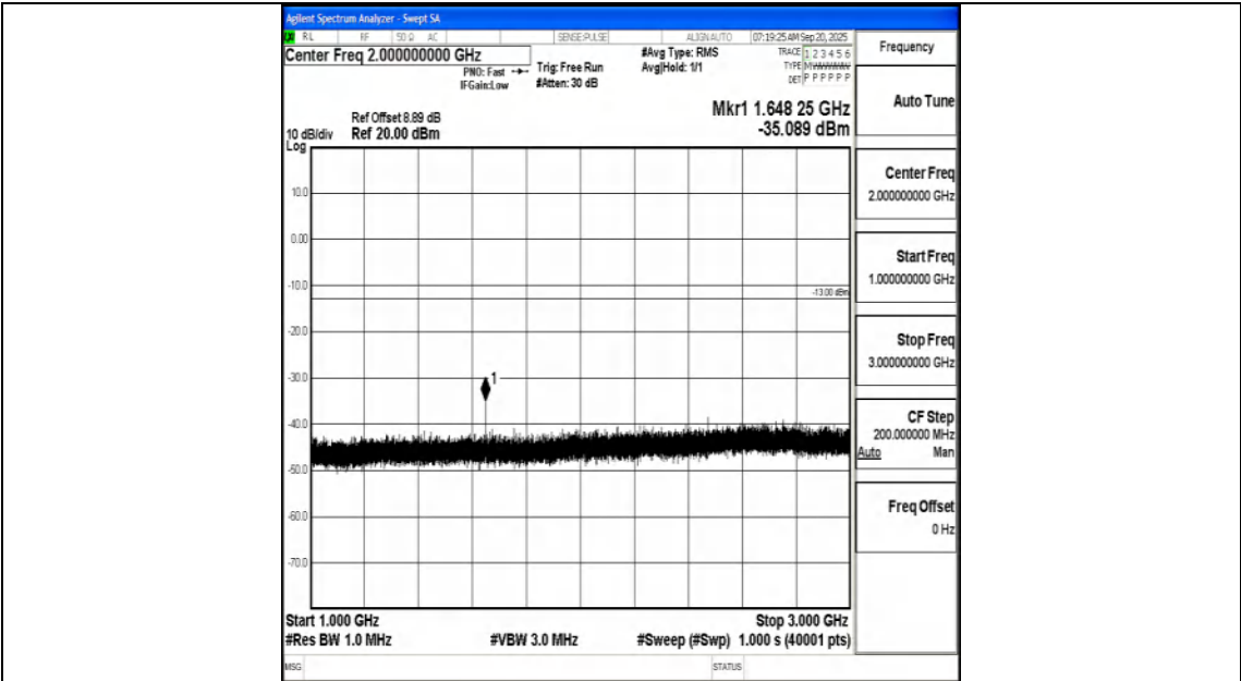
Band5_1.4MHz_16QAM_20407_1RB#0_1000~3000_1000~3000
