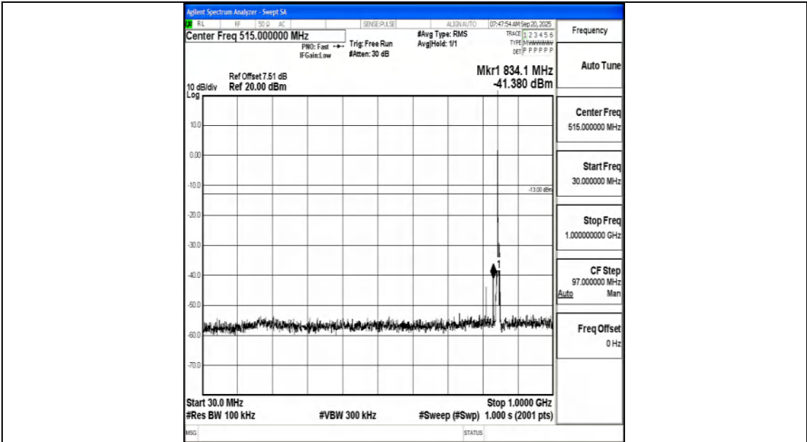
Band5_3MHz_QPSK_20635_1RB#0_30~1000_30~1000
