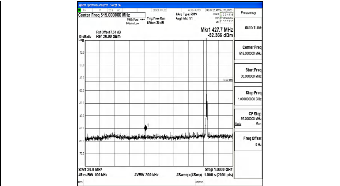
Band5_5MHz_QPSK_20425_1RB#0_30~1000_30~1000
