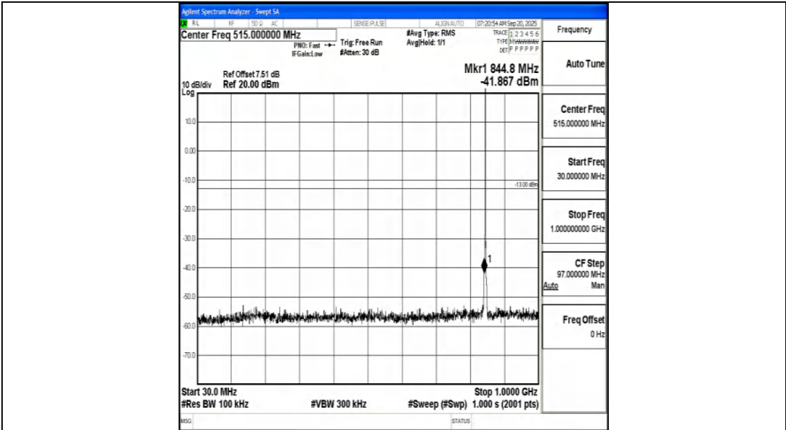
Band5_1.4MHz_QPSK_20643_1RB#0_30~1000_30~1000
