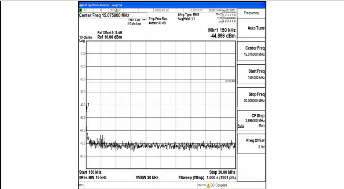
Band5_5MHz_16QAM_20425_1RB#0_0.15~30_0.15~30
