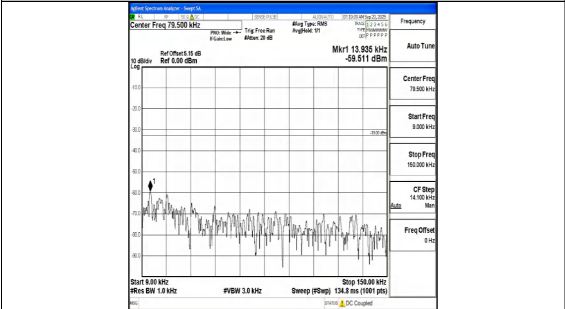
Band5_1.4MHz_16QAM_20407_1RB#0_0.009~0.15_0.009~0.15
