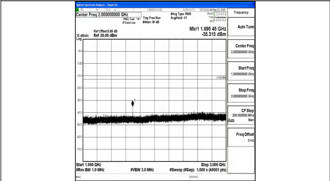
Band5_1.4MHz_QPSK_20643_1RB#0_1000~3000_1000~3000
