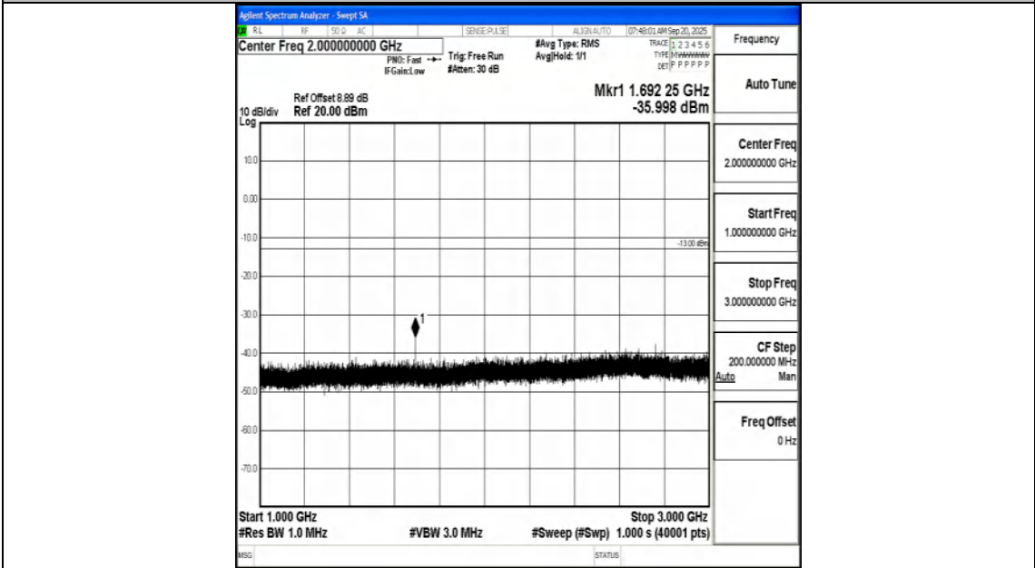
Band5_3MHz_QPSK_20635_1RB#0_1000~3000_1000~3000
