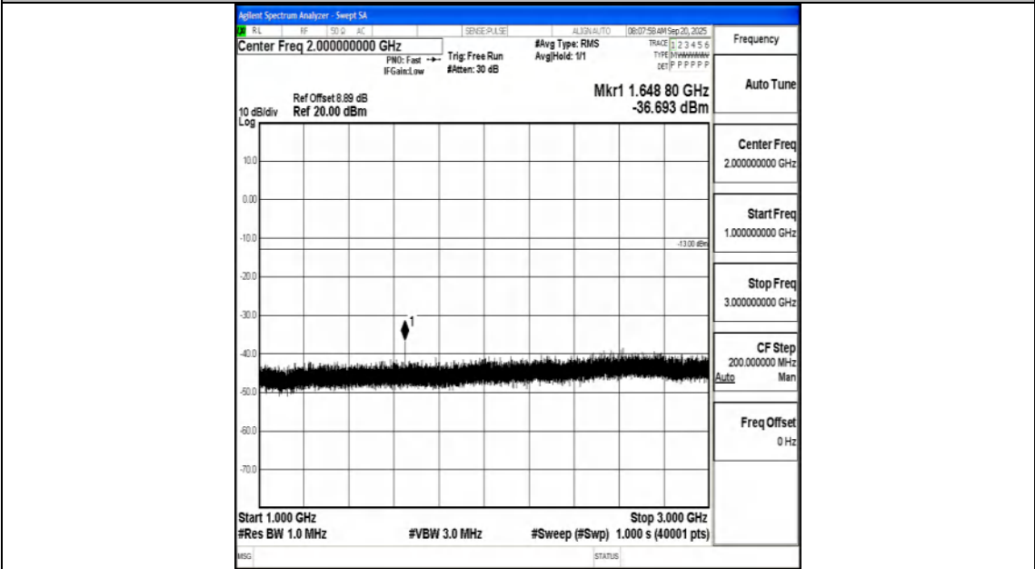
Band5_5MHz_QPSK_20425_1RB#0_1000~3000_1000~3000
