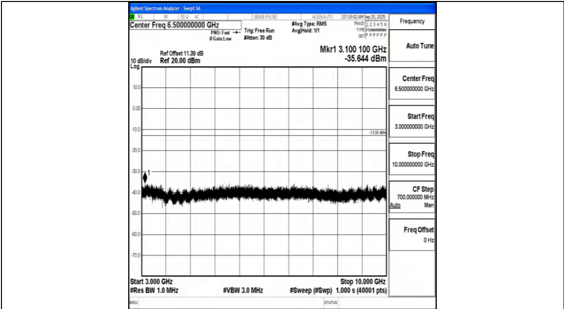
Band5_1.4MHz_QPSK_20407_1RB#0_3000~10000_3000~10000
