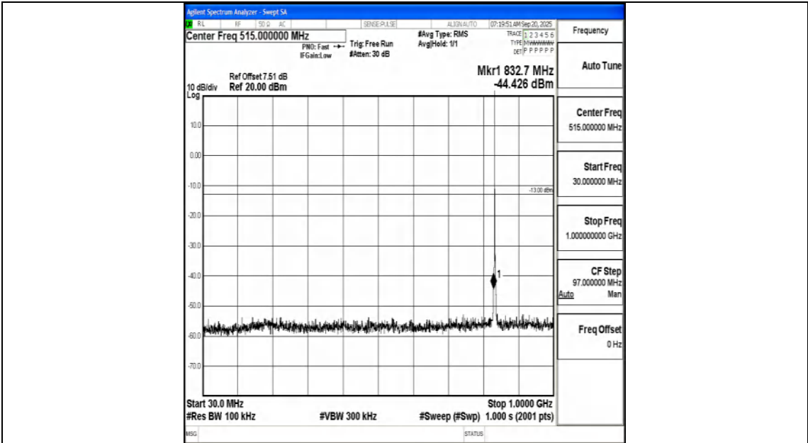
Band5_1.4MHz_QPSK_20525_1RB#0_30~1000_30~1000
