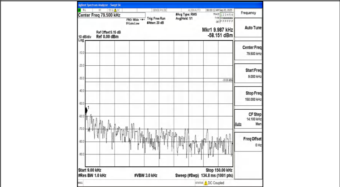
Band5_5MHz_16QAM_20425_1RB#0_0.009~0.15_0.009~0.15
