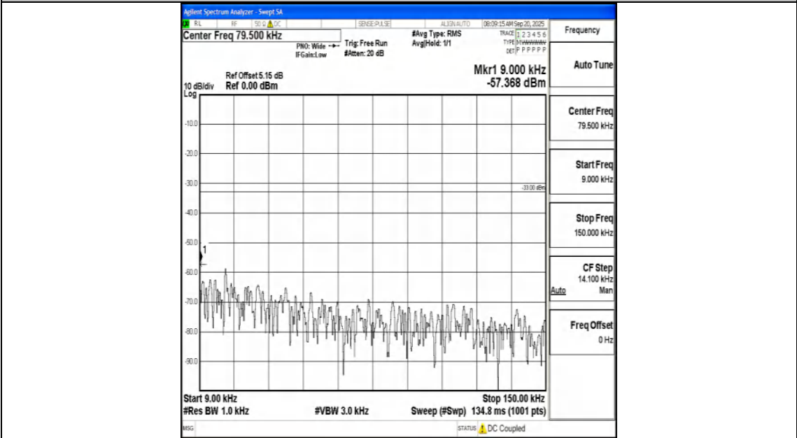
Band5_5MHz_16QAM_20525_1RB#0_0.009~0.15_0.009~0.15
