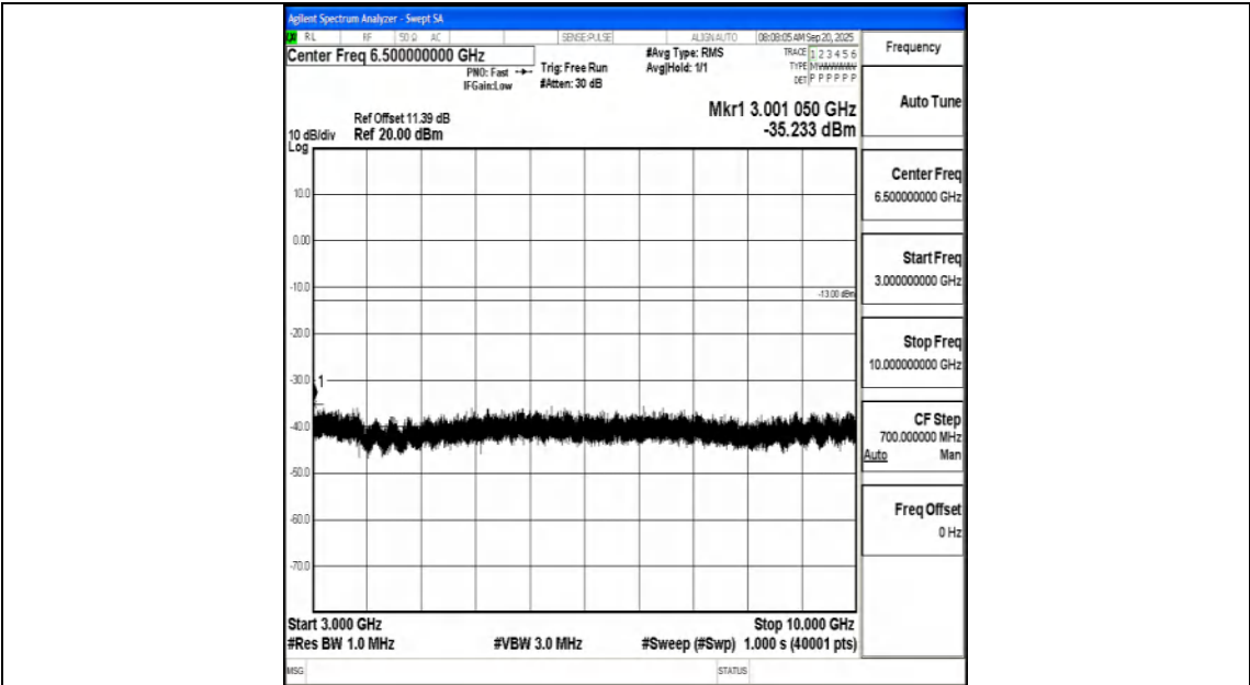
Band5_5MHz_QPSK_20425_1RB#0_3000~10000_3000~10000
