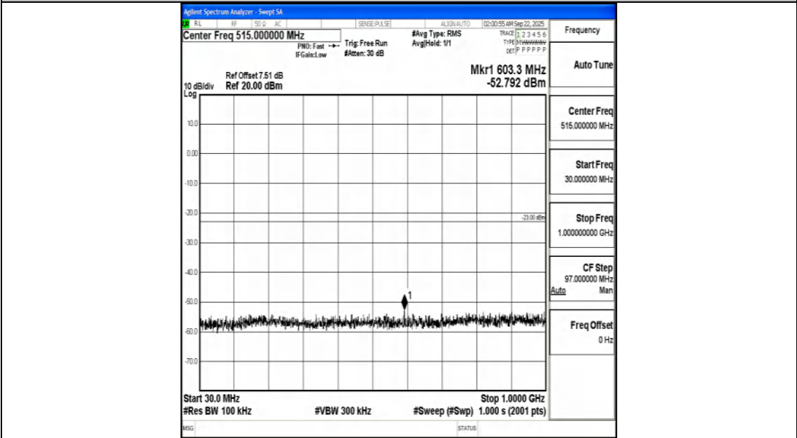
Band66_5MHz_QPSK_131997_1RB#0_30~1000_30~1000
