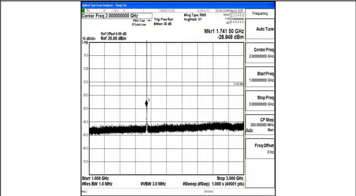
Band66_1.4MHz_16QAM_132322_1RB#0_1000~3000_1000~3000
