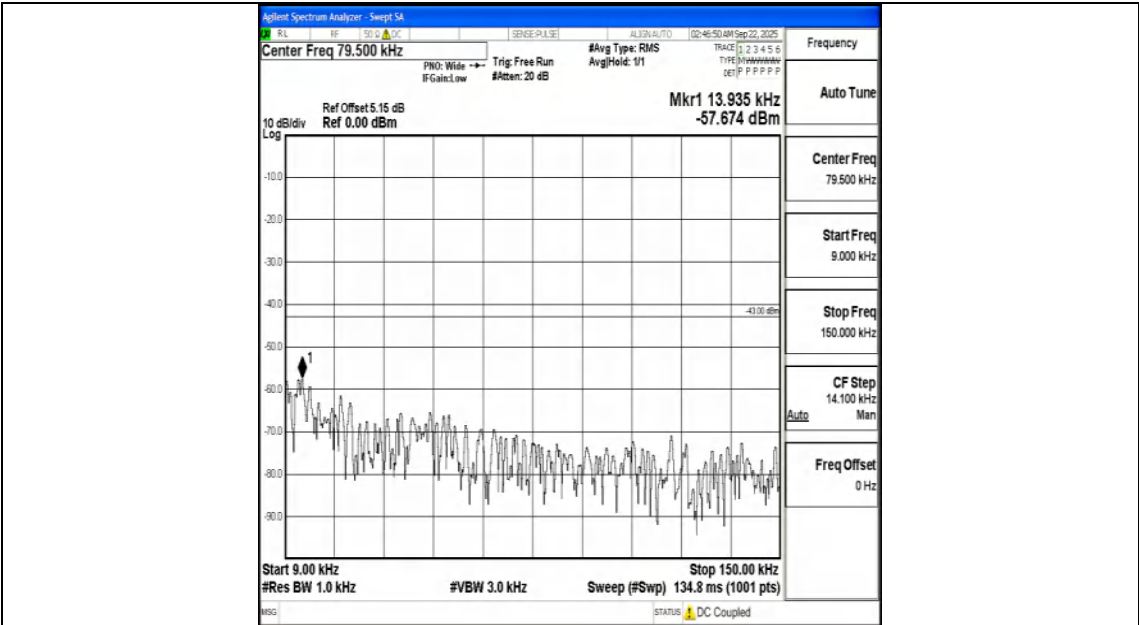
Band66_15MHz_16QAM_132047_1RB#0_0.009~0.15_0.009~0.15
