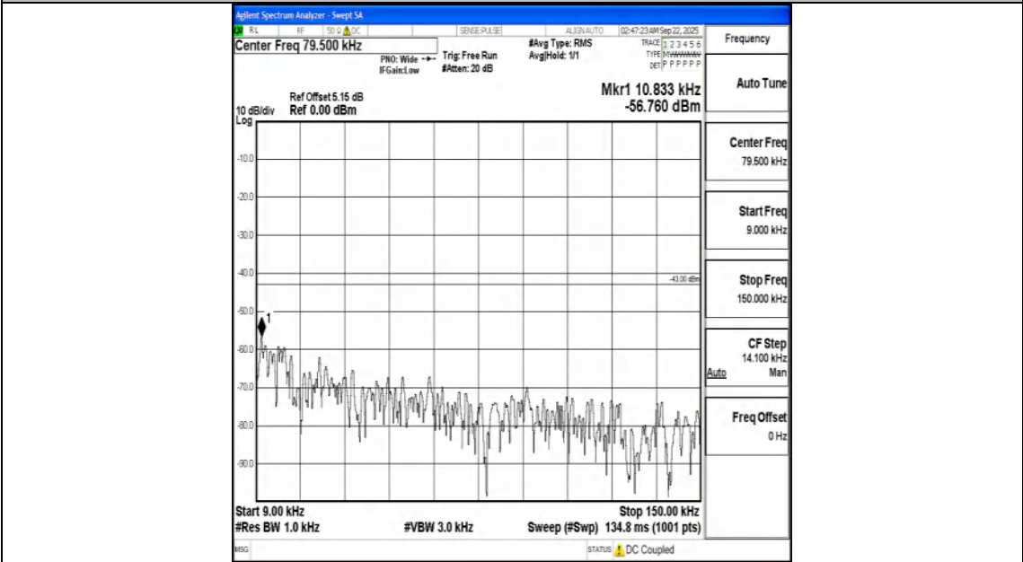
Band66_15MHz_QPSK_132322_1RB#0_0.009~0.15_0.009~0.15
