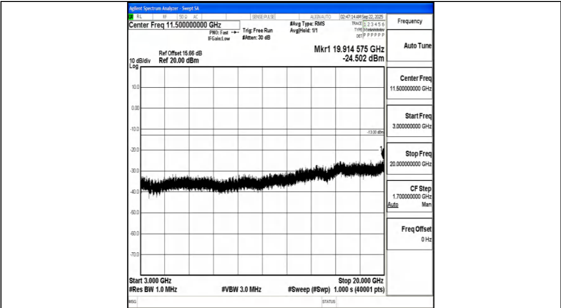
Band66_15MHz_16QAM_132047_1RB#0_3000~20000_3000~20000
