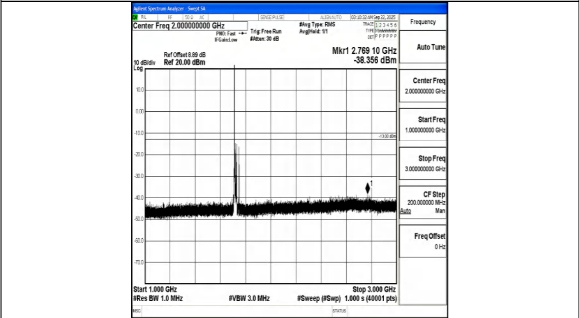
Band66_20MHz_16QAM_132072_1RB#0_1000~3000_1000~3000
