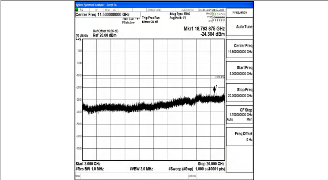
Band66_3MHz_QPSK_131987_1RB#0_3000~20000_3000~20000
