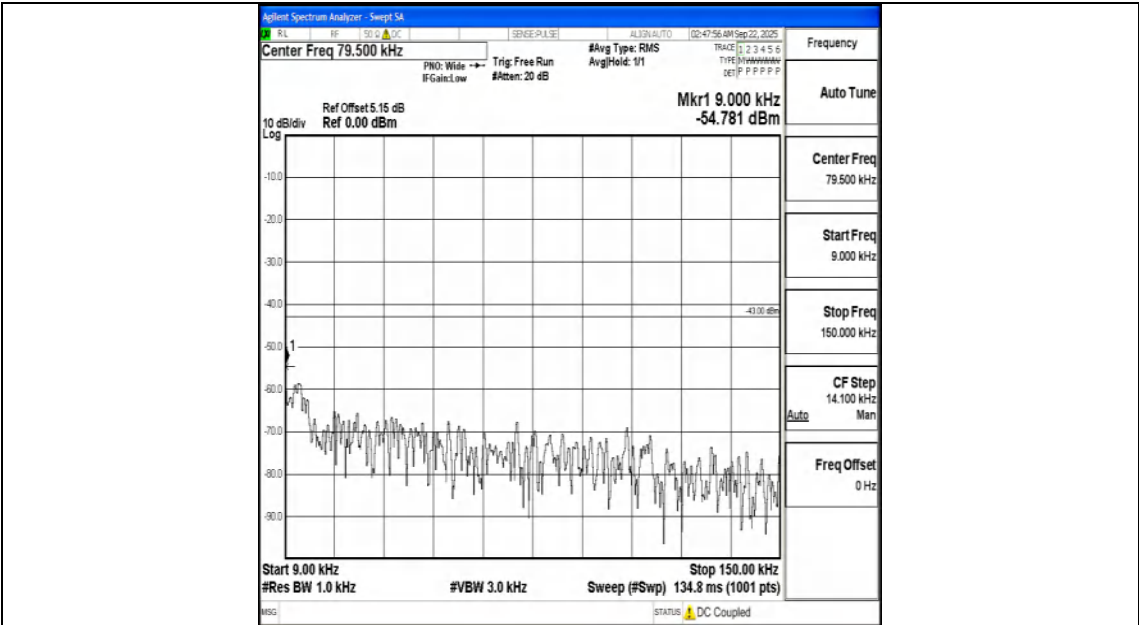
Band66_15MHz_16QAM_132322_1RB#0_0.009~0.15_0.009~0.15
