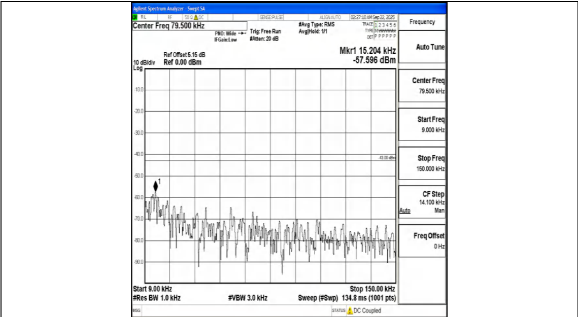
Band66_10MHz_16QAM_132622_1RB#0_0.009~0.15_0.009~0.15
