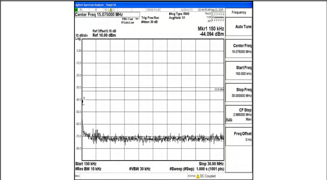
Band66_15MHz_16QAM_132047_1RB#0_0.15~30_0.15~30
