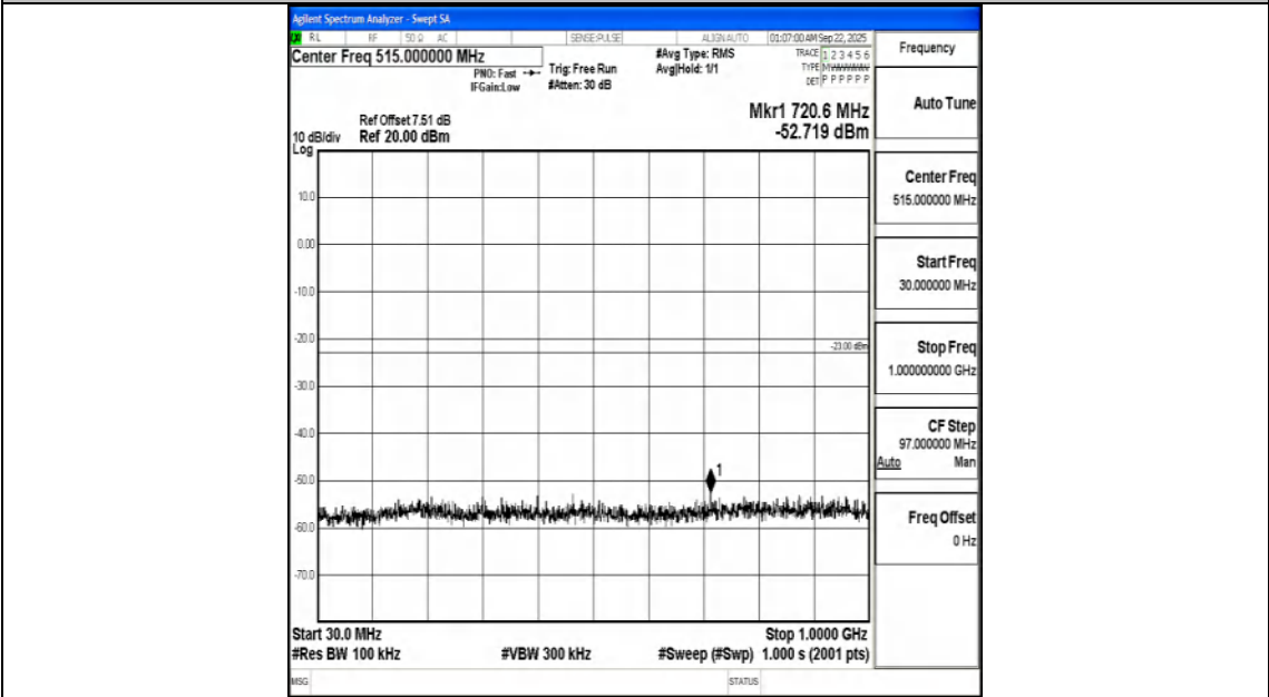
Band66_1.4MHz_QPSK_132665_1RB#0_30~1000_30~1000
