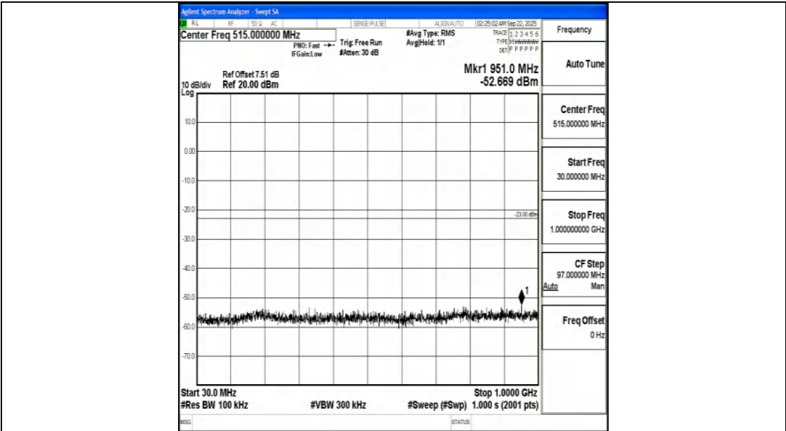
Band66_10MHz_16QAM_132022_1RB#0_30~1000_30~1000
