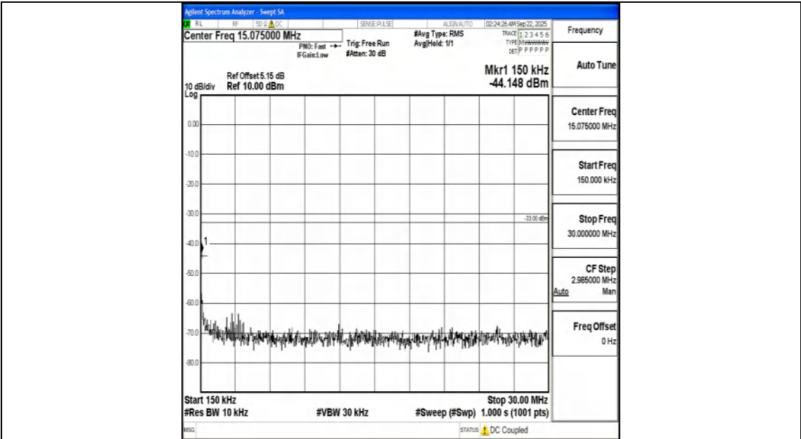
Band66_10MHz_QPSK_132022_1RB#0_0.15~30_0.15~30
