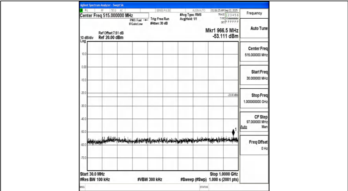
Band66_1.4MHz_16QAM_132322_1RB#0_30~1000_30~1000
