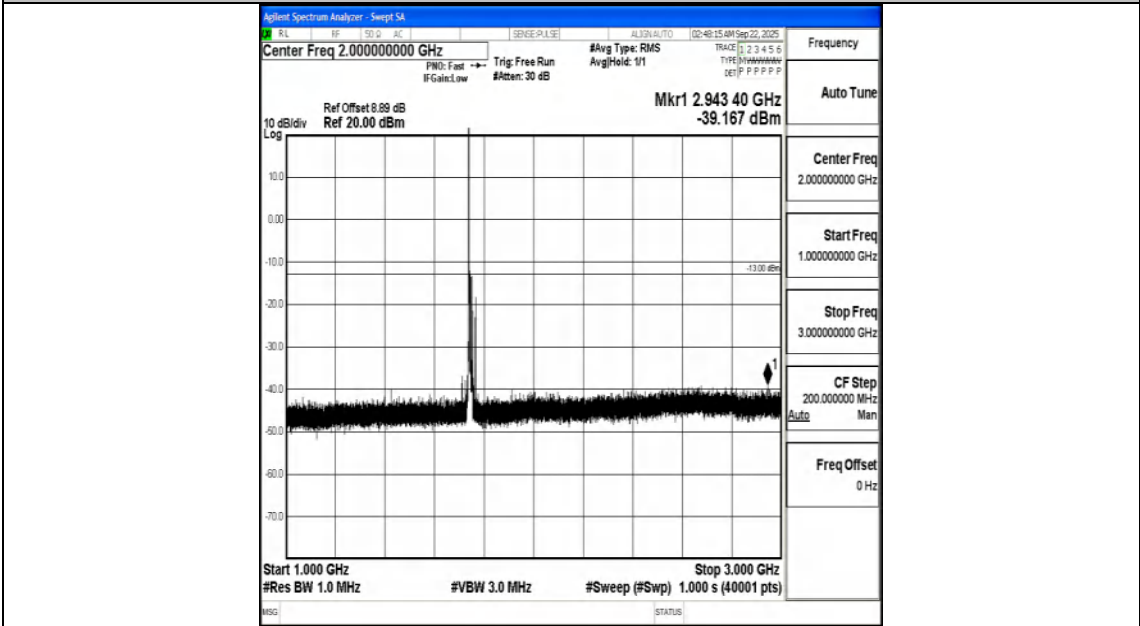
Band66_15MHz_16QAM_132322_1RB#0_1000~3000_1000~3000
