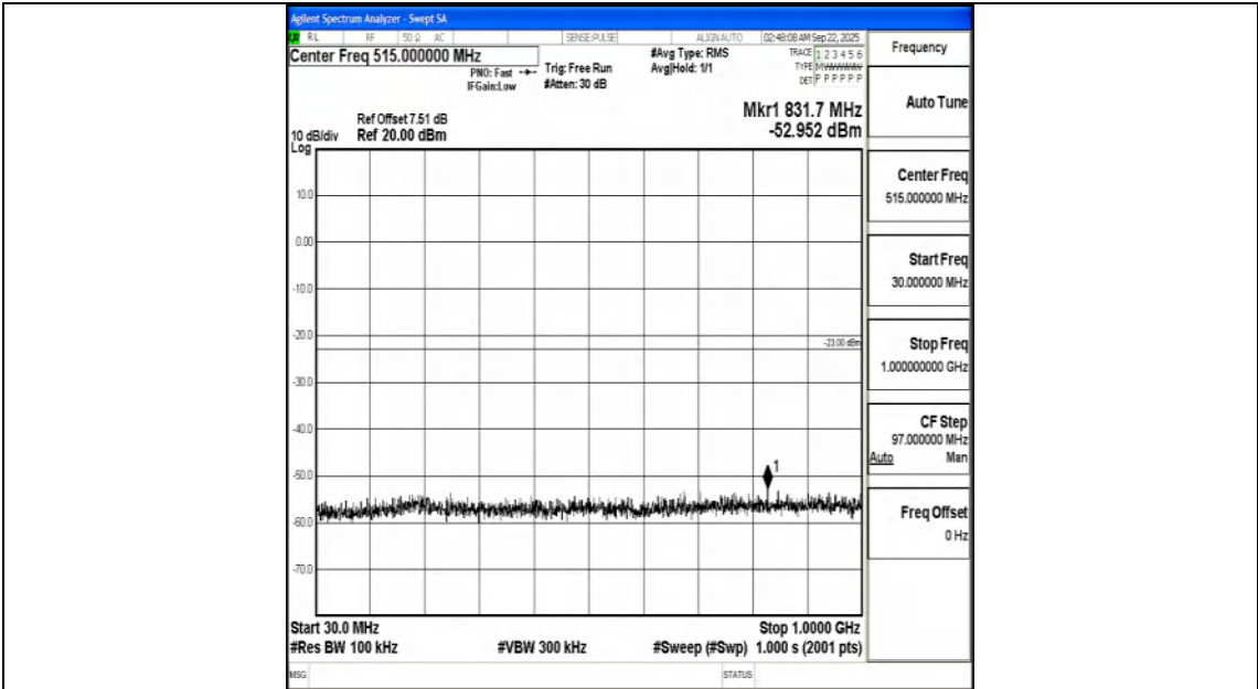
Band66_15MHz_16QAM_132322_1RB#0_30~1000_30~1000
