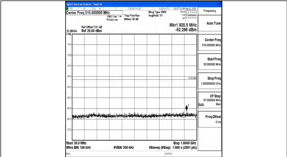
Band66_10MHz_16QAM_132622_1RB#0_30~1000_30~1000
