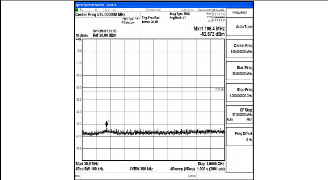
Band66_10MHz_QPSK_132022_1RB#0_30~1000_30~1000
