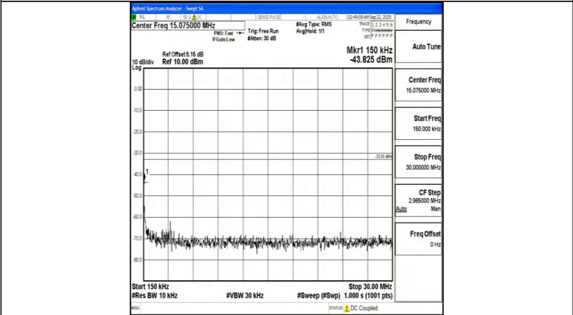
Band66_15MHz_16QAM_132597_1RB#0_0.15~30_0.15~30
