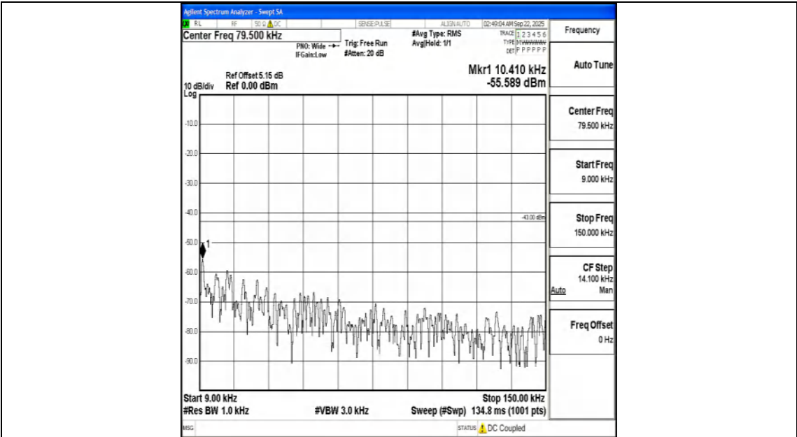
Band66_15MHz_16QAM_132597_1RB#0_0.009~0.15_0.009~0.15
