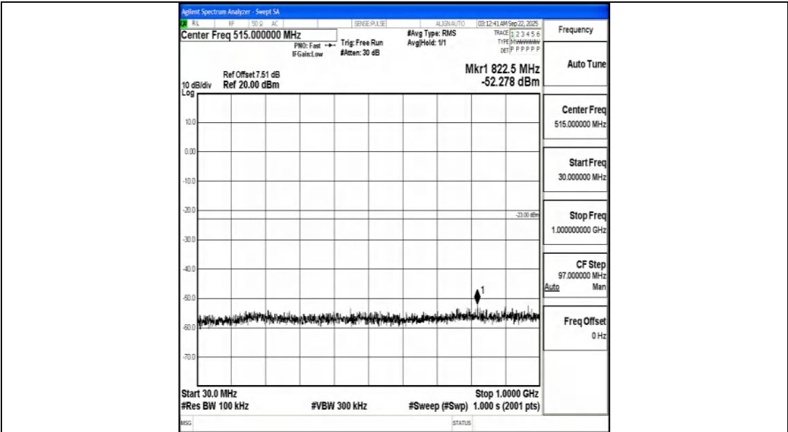
Band66_20MHz_16QAM_132572_1RB#0_30~1000_30~1000
