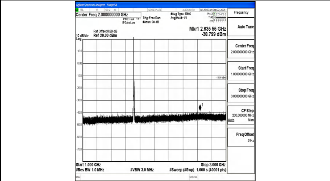
Band66_10MHz_16QAM_132022_1RB#0_1000~3000_1000~3000
