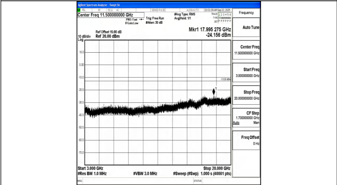
Band66_5MHz_QPSK_131997_1RB#0_3000~20000_3000~20000
