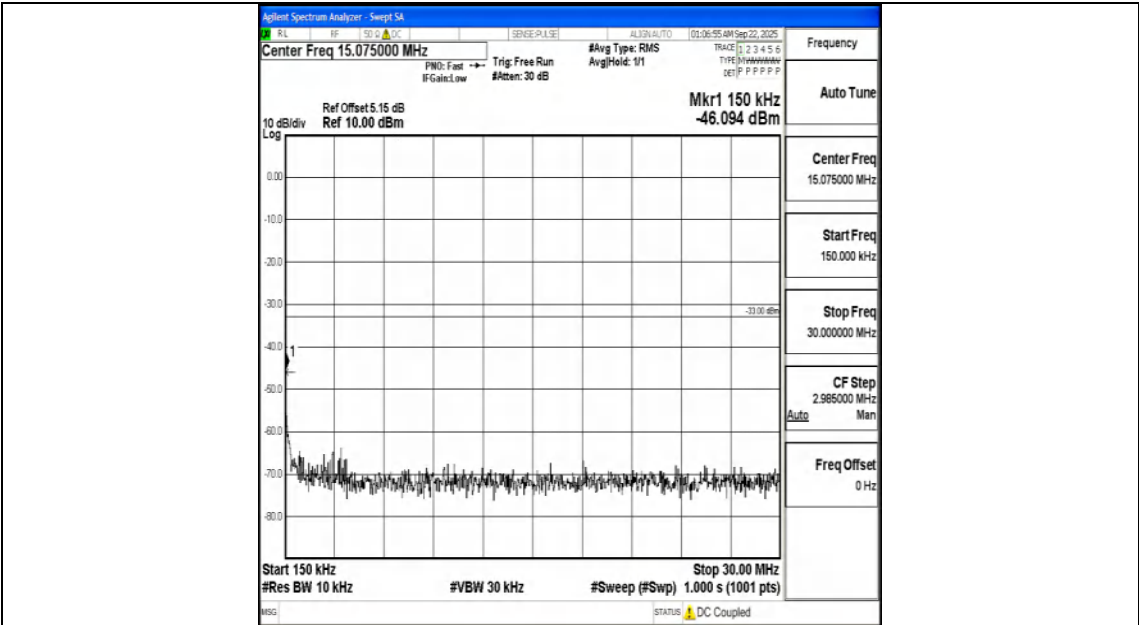
Band66_1.4MHz_QPSK_132665_1RB#0_0.15~30_0.15~30
