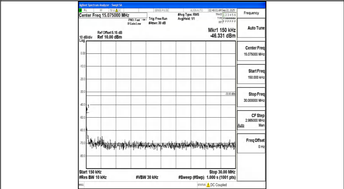
Band66_15MHz_16QAM_132322_1RB#0_0.15~30_0.15~30
