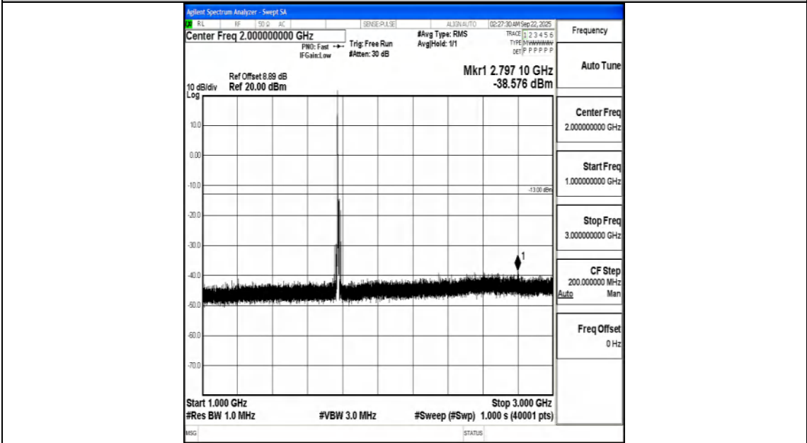
Band66_10MHz_16QAM_132622_1RB#0_1000~3000_1000~3000
