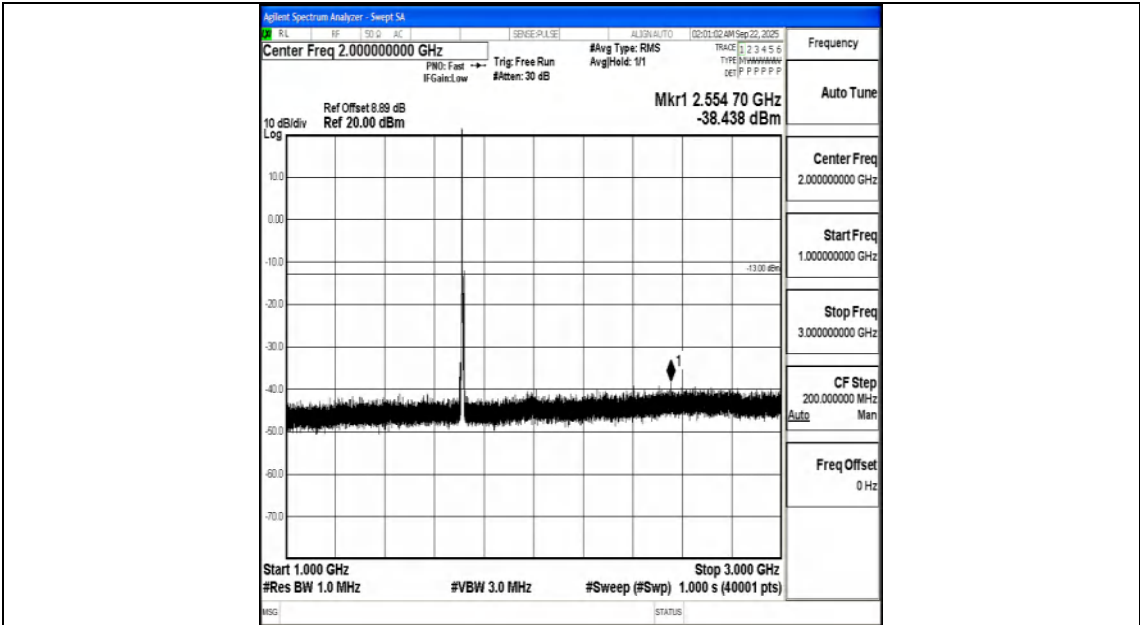
Band66_5MHz_QPSK_131997_1RB#0_1000~3000_1000~3000
