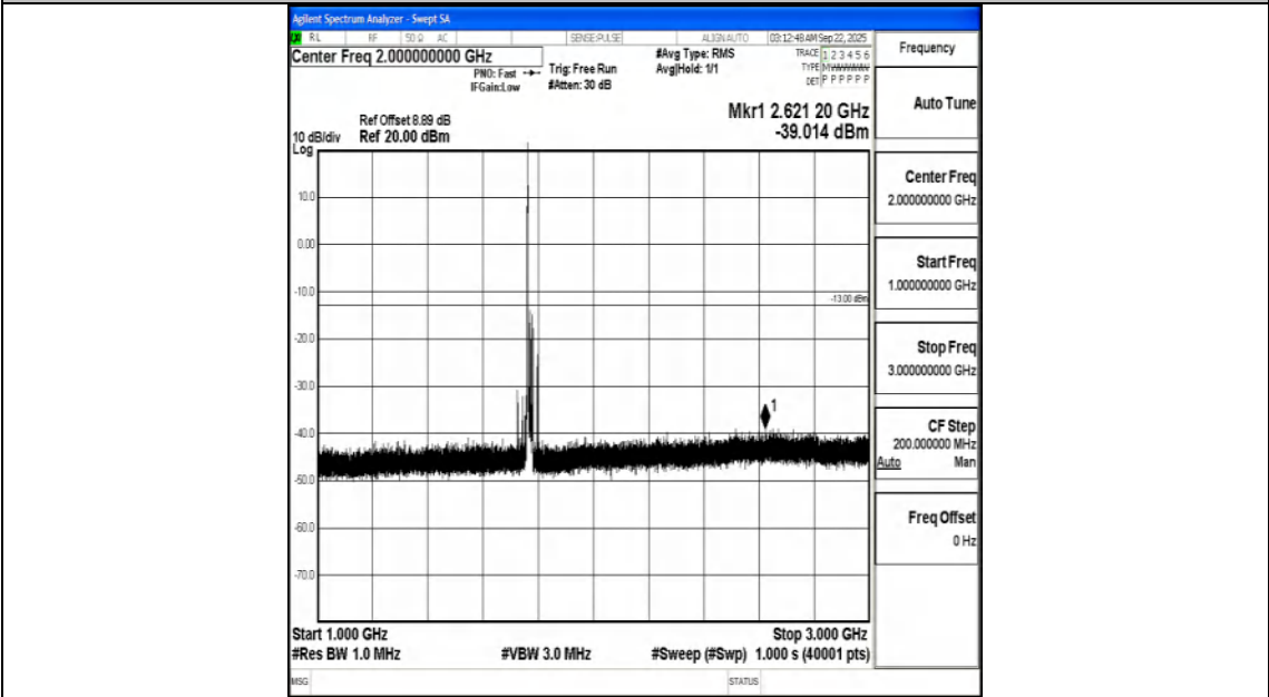
Band66_20MHz_16QAM_132572_1RB#0_1000~3000_1000~3000
