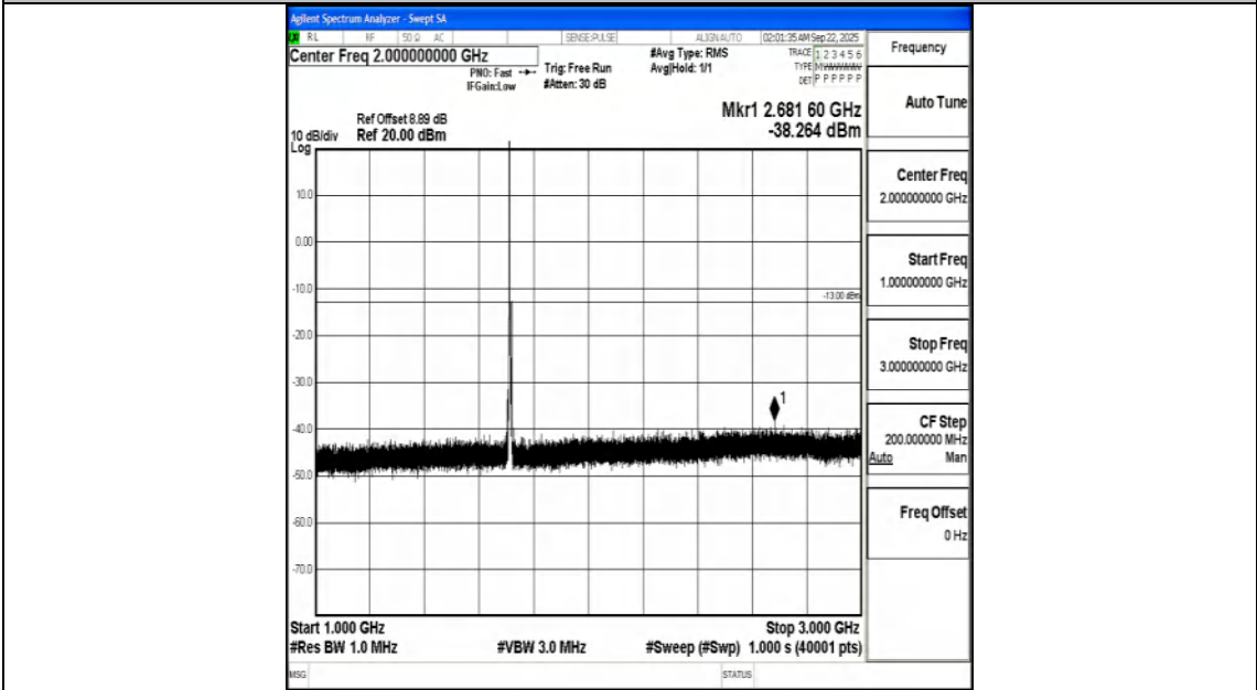
Band66_5MHz_16QAM_131997_1RB#0_1000~3000_1000~3000
