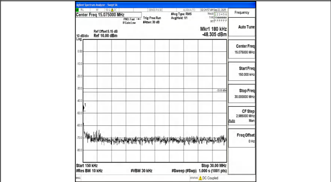
Band66_10MHz_16QAM_132022_1RB#0_0.15~30_0.15~30
