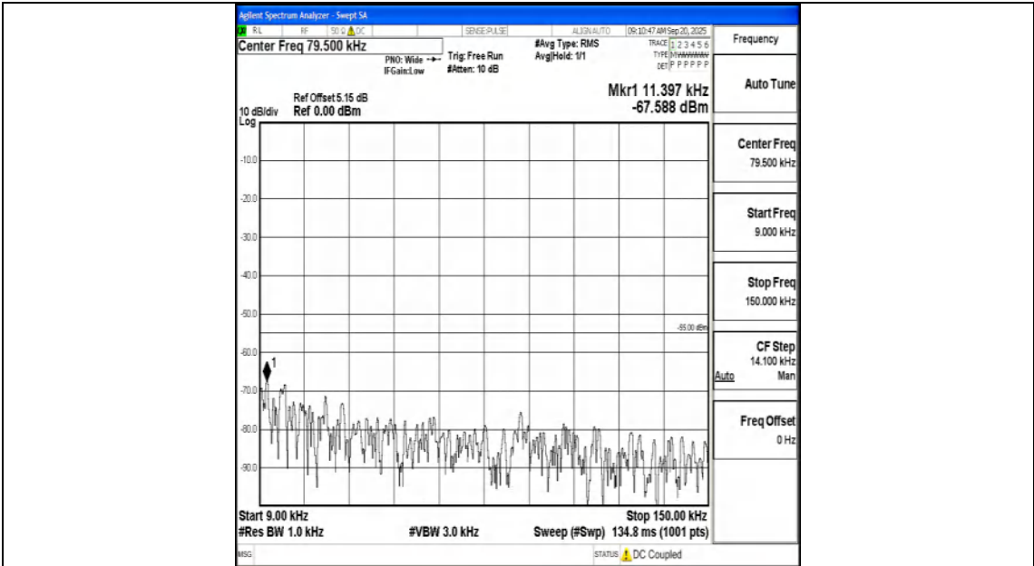
Band7_10MHz_QPSK_21100_1RB#0_0.009~0.15_0.009~0.15
