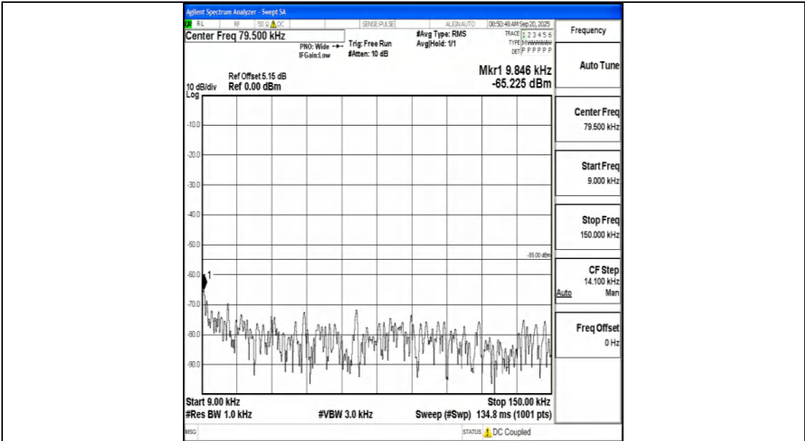
Band7_5MHz_QPSK_21425_1RB#0_0.009~0.15_0.009~0.15
