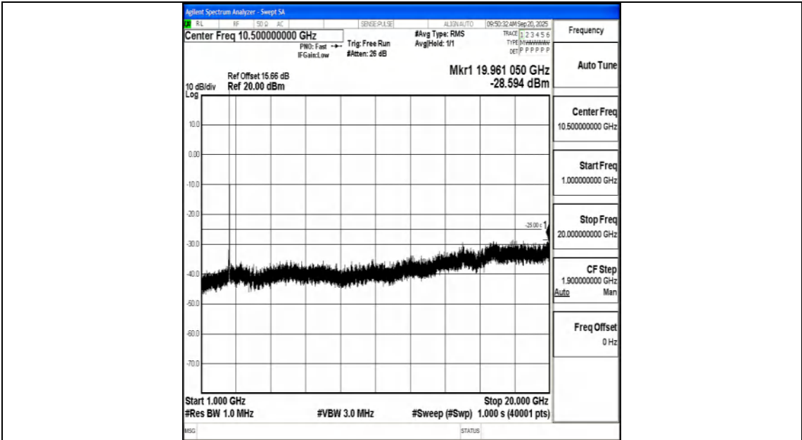
Band7_20MHz_16QAM_21100_1RB#0_1000~20000_1000~20000
