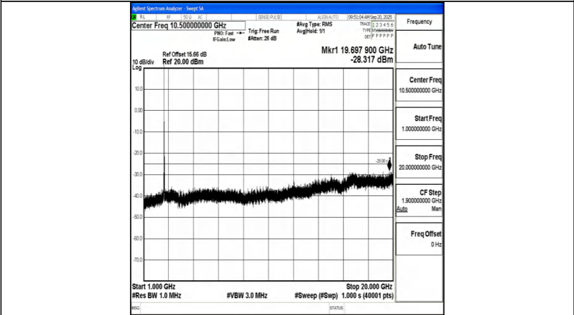
Band7_20MHz_QPSK_21350_1RB#0_1000~20000_1000~20000
