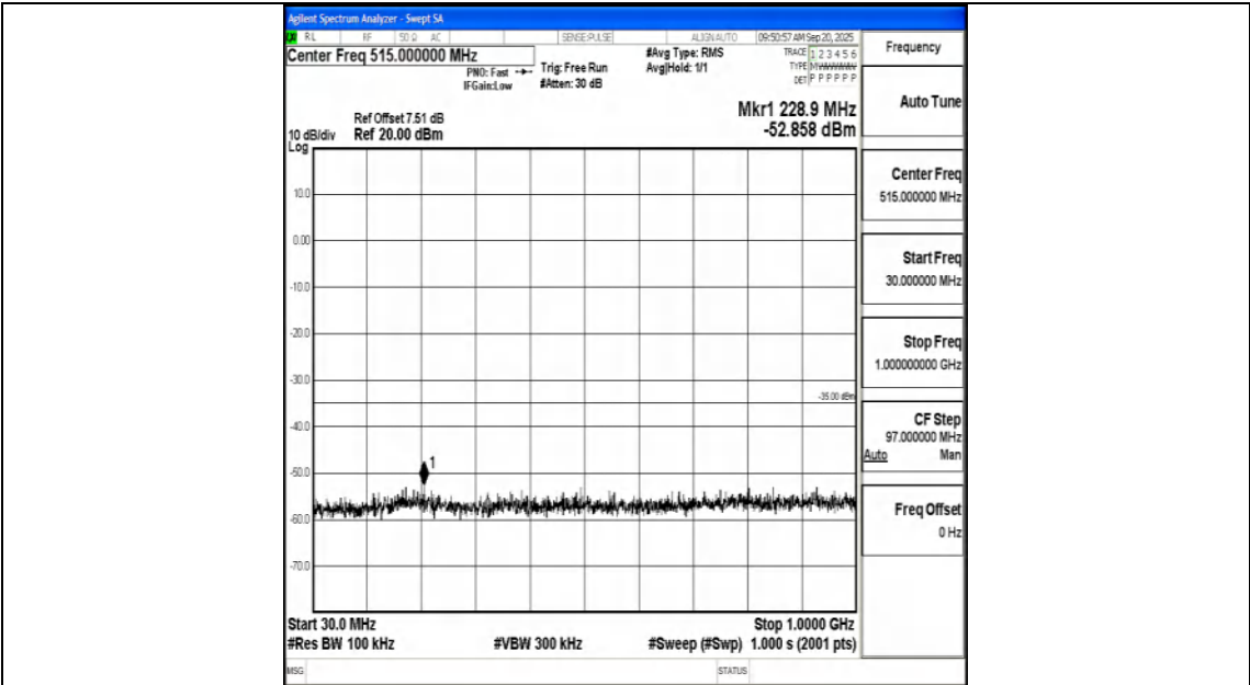
Band7_20MHz_QPSK_21350_1RB#0_30~1000_30~1000
