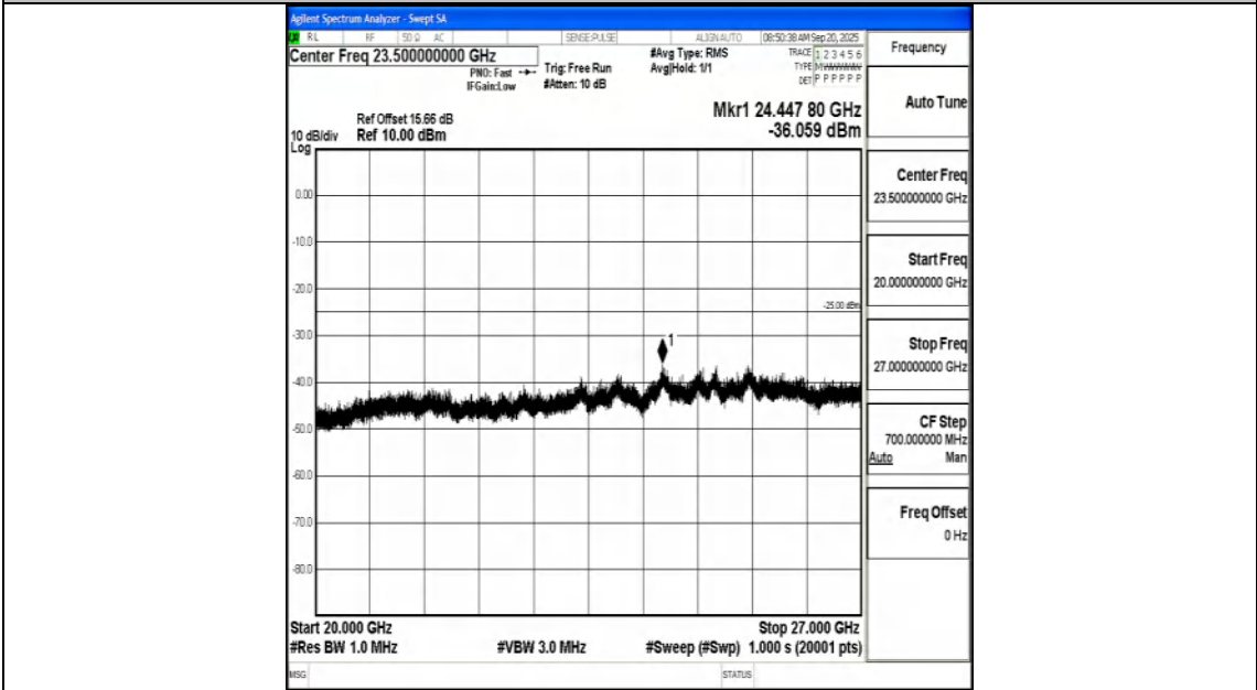
Band7_5MHz_16QAM_21100_1RB#0_20000~27000_20000~27000
