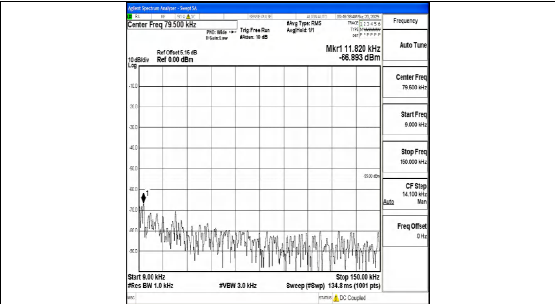
Band7_20MHz_QPSK_20850_1RB#0_0.009~0.15_0.009~0.15
