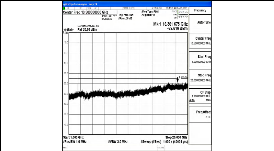
Band7_10MHz_QPSK_20800_1RB#0_1000~20000_1000~20000
