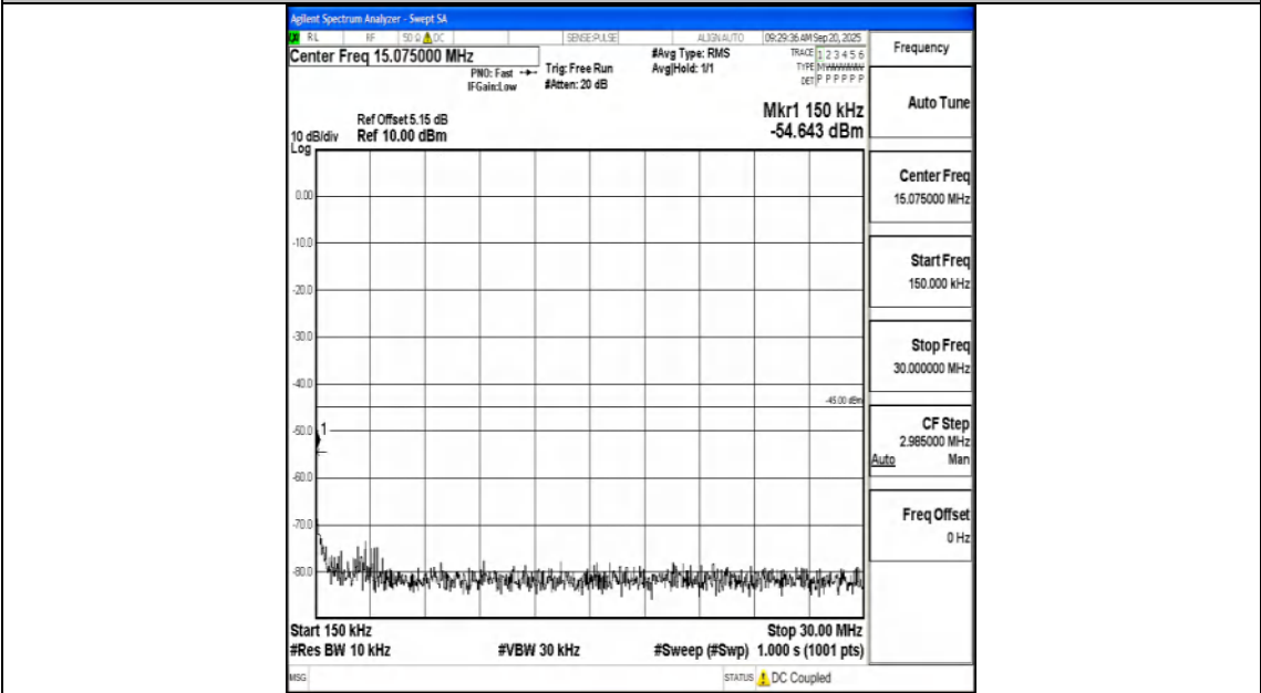
Band7_15MHz_QPSK_20825_1RB#0_0.15~30_0.15~30
