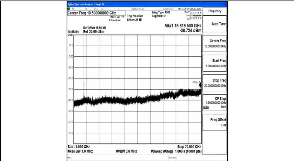
Band7_10MHz_16QAM_21100_1RB#0_1000~20000_1000~20000
