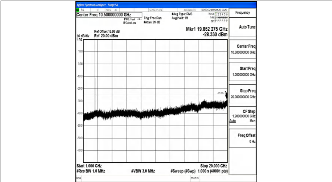
Band7_5MHz_16QAM_21100_1RB#0_1000~20000_1000~20000
