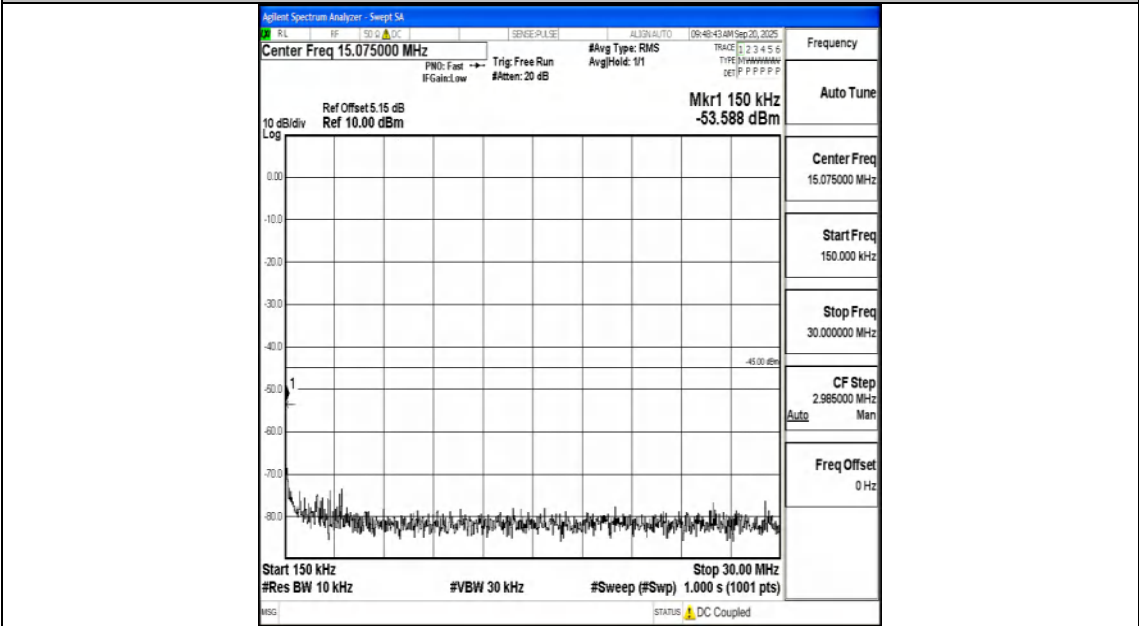
Band7_20MHz_QPSK_20850_1RB#0_0.15~30_0.15~30
