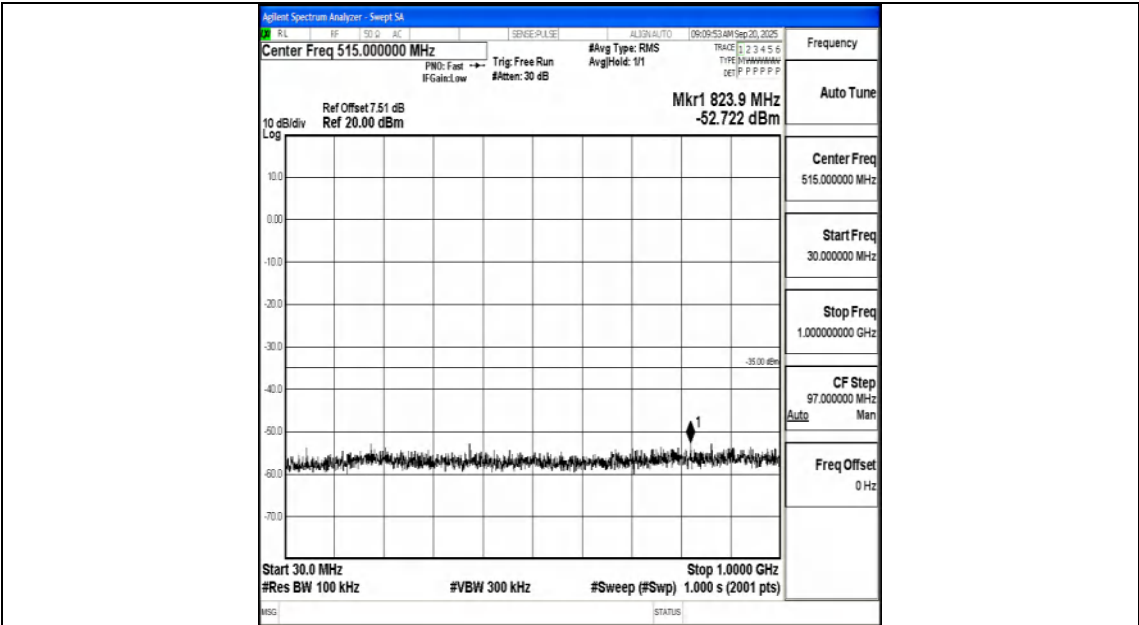
Band7_10MHz_QPSK_20800_1RB#0_30~1000_30~1000
