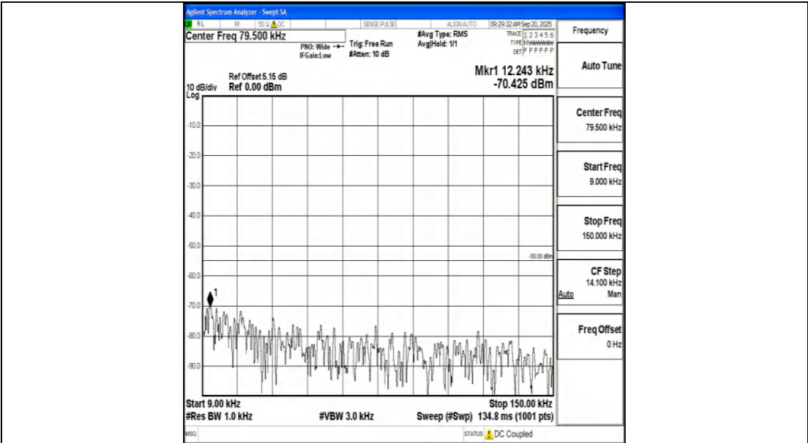
Band7_15MHz_QPSK_20825_1RB#0_0.009~0.15_0.009~0.15
