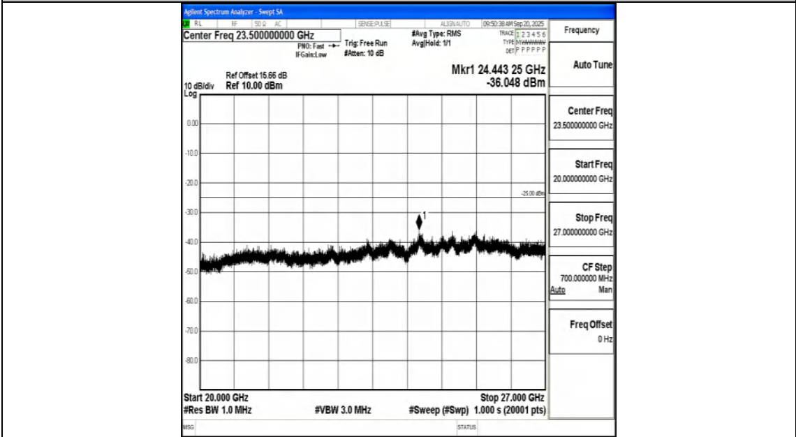
Band7_20MHz_16QAM_21100_1RB#0_20000~27000_20000~27000
