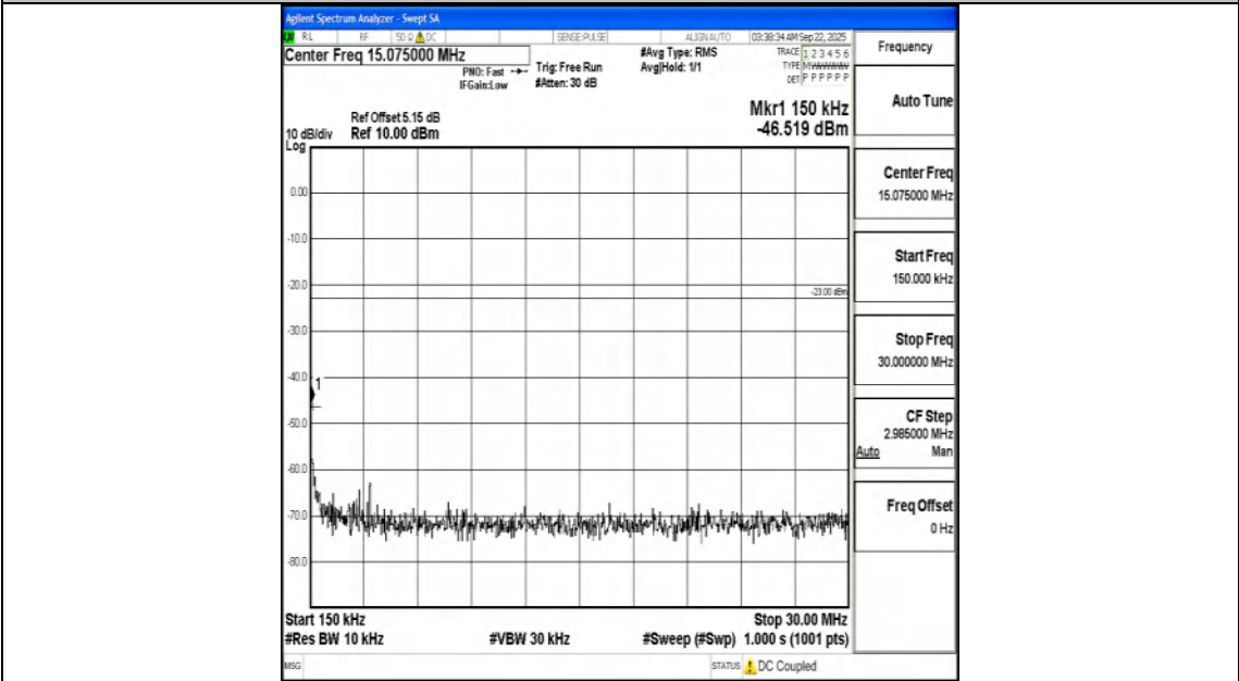
Band71_5MHz_QPSK_133447_1RB#0_0.15~30_0.15~30
