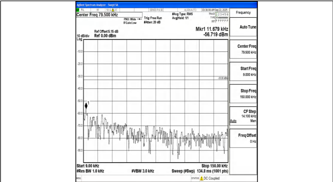
Band71_5MHz_QPSK_133297_1RB#0_0.009~0.15_0.009~0.15
