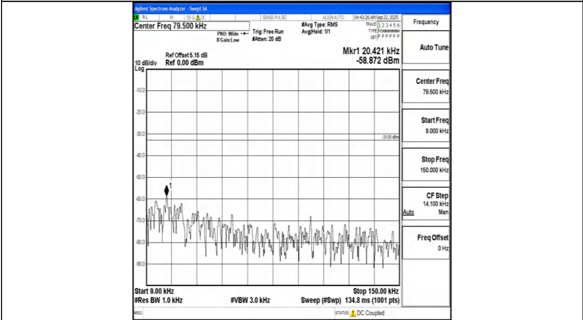
Band71_15MHz_16QAM_133397_1RB#0_0.009~0.15_0.009~0.15
