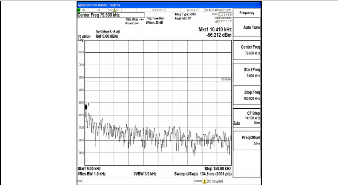
Band71_5MHz_QPSK_133447_1RB#0_0.009~0.15_0.009~0.15
