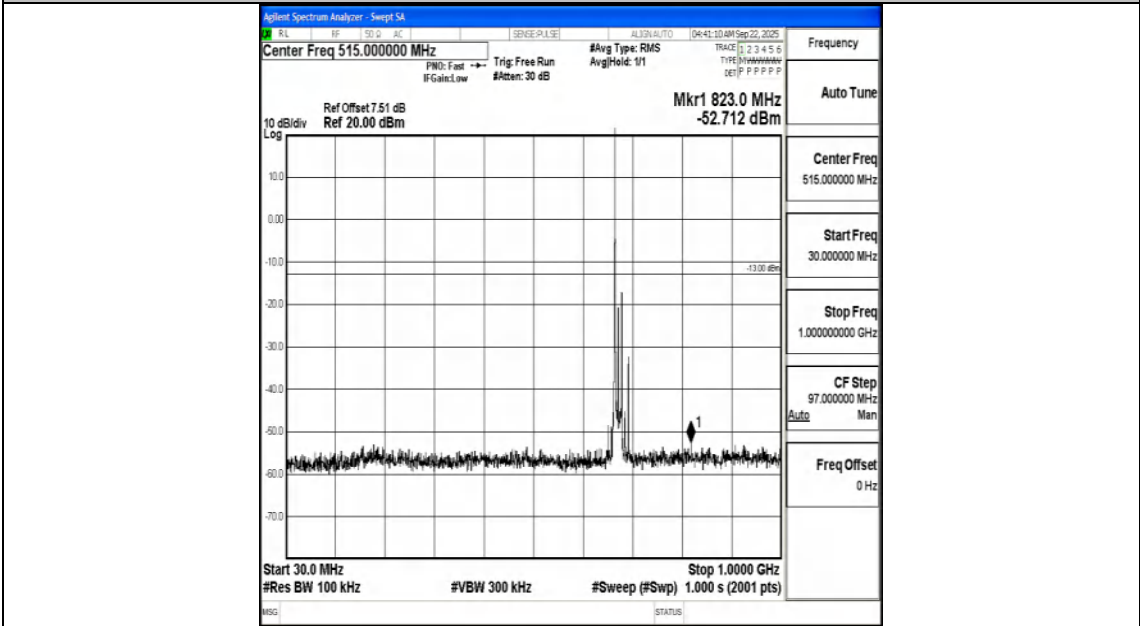
Band71_15MHz_16QAM_133297_1RB#0_30~1000_30~1000
