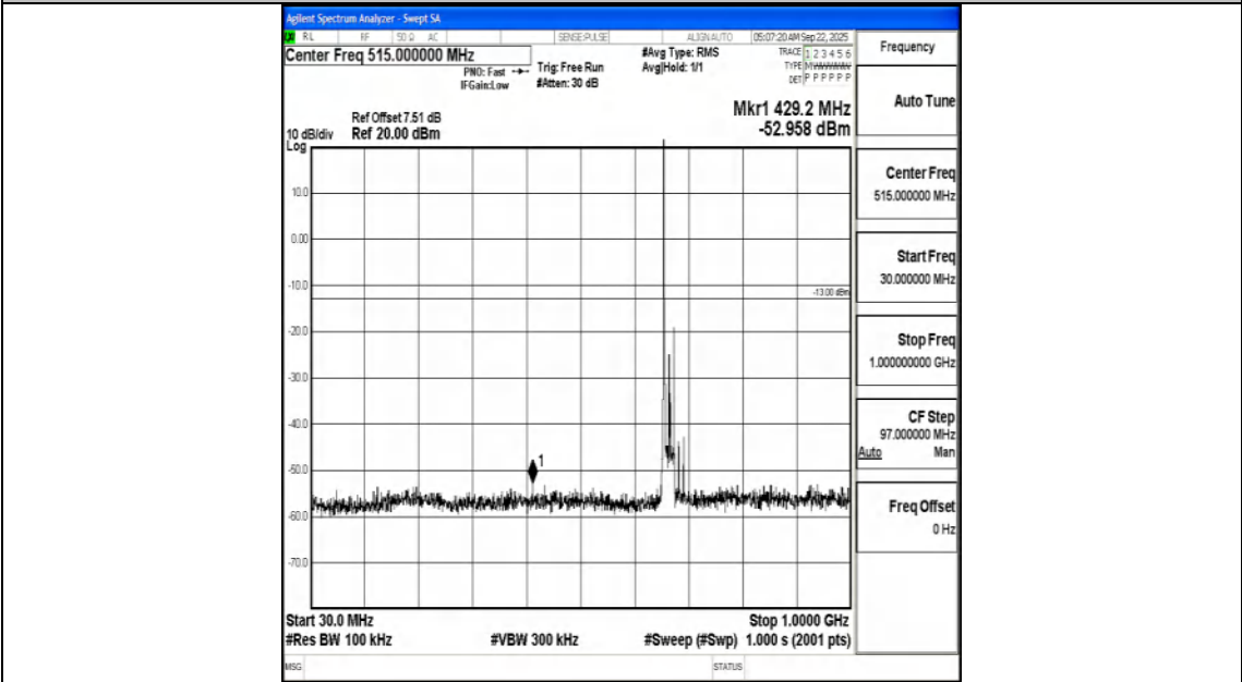
Band71_20MHz_16QAM_133222_1RB#0_30~1000_30~1000
