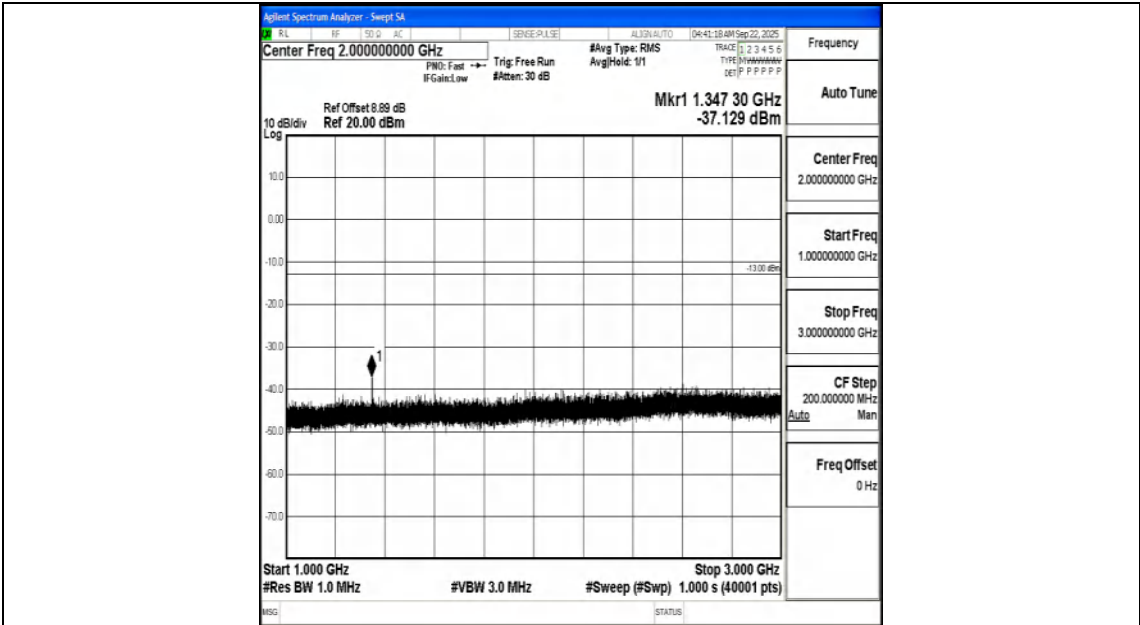
Band71_15MHz_16QAM_133297_1RB#0_1000~3000_1000~3000
