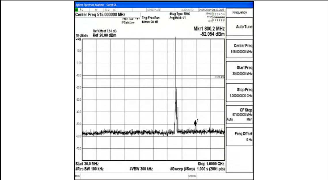
Band71_10MHz_16QAM_133172_1RB#0_30~1000_30~1000
