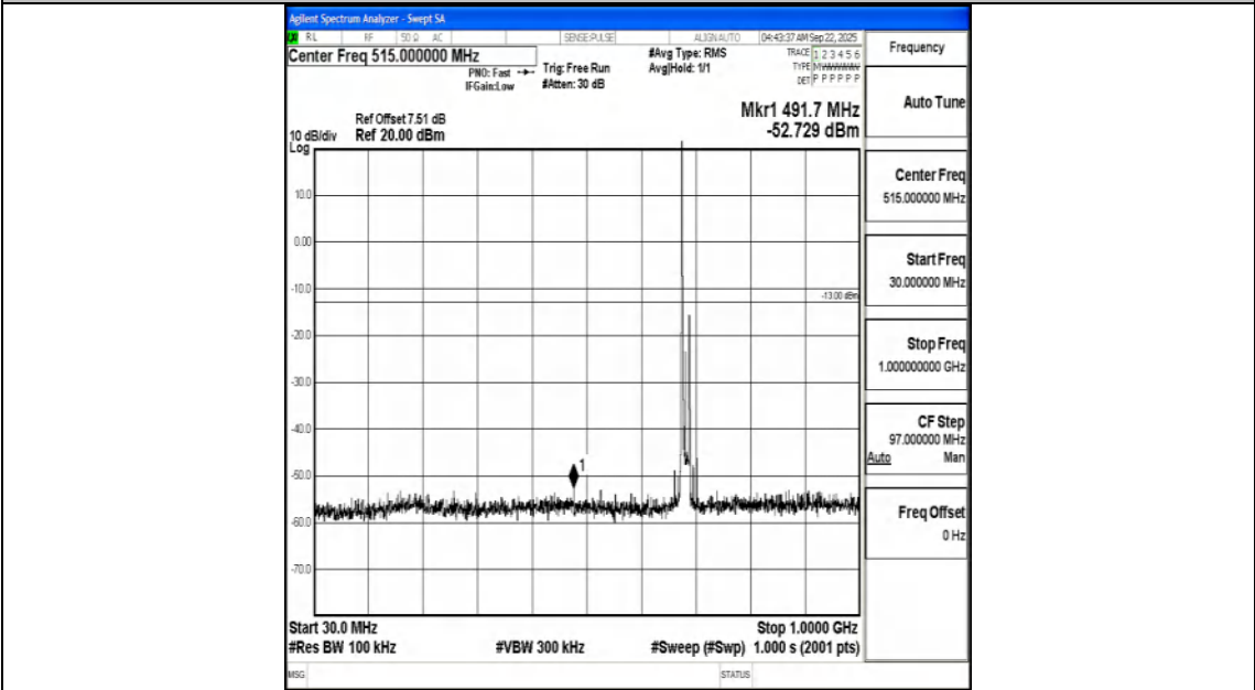
Band71_15MHz_16QAM_133397_1RB#0_30~1000_30~1000
