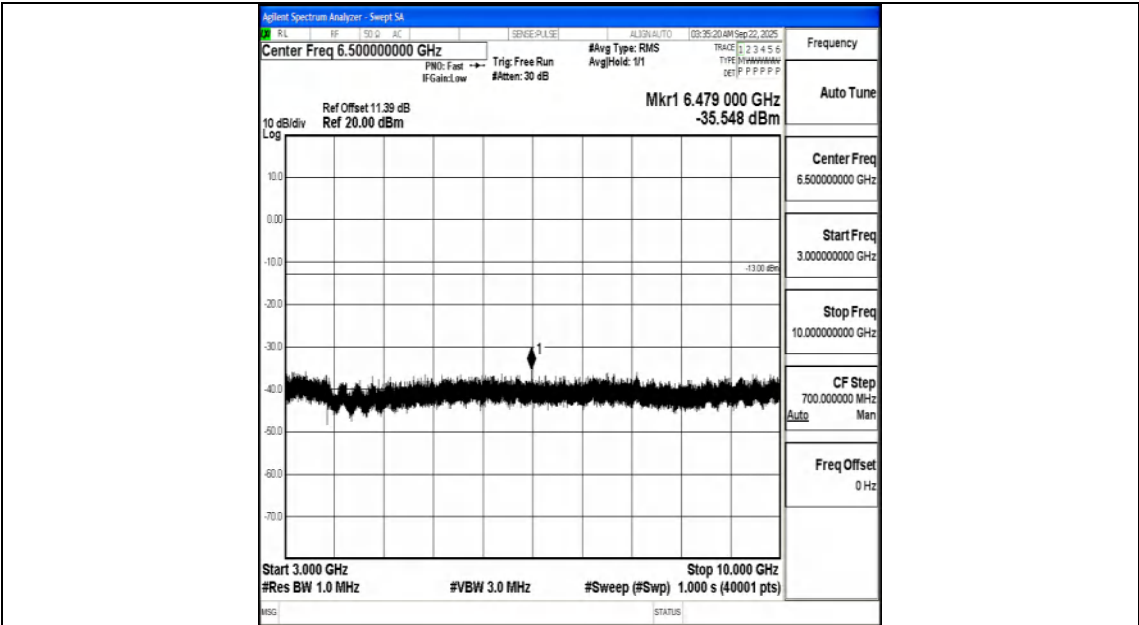
Band71_5MHz_16QAM_133147_1RB#0_3000~10000_3000~10000
