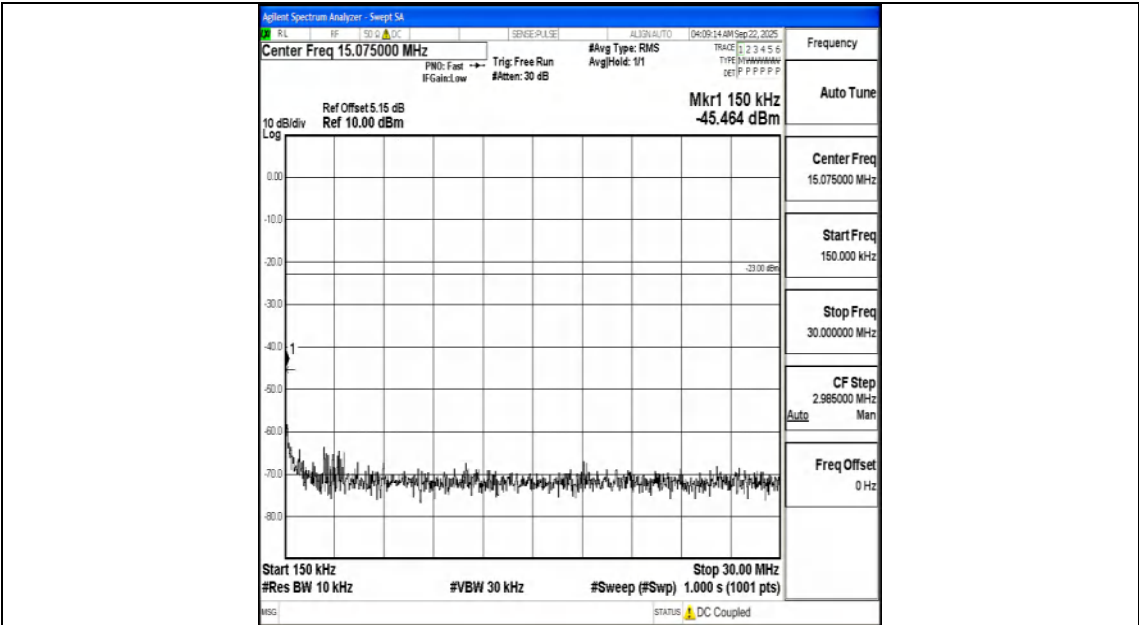
Band71_10MHz_16QAM_133172_1RB#0_0.15~30_0.15~30
