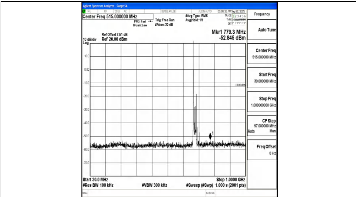
Band71_20MHz_QPSK_133322_1RB#0_30~1000_30~1000
