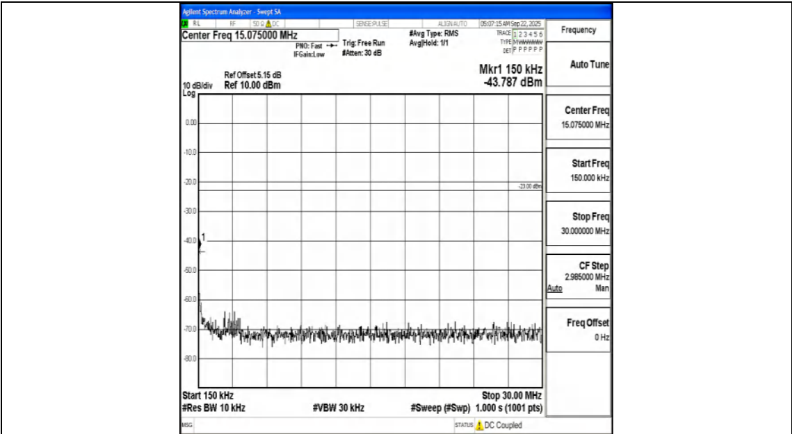
Band71_20MHz_16QAM_133222_1RB#0_0.15~30_0.15~30
