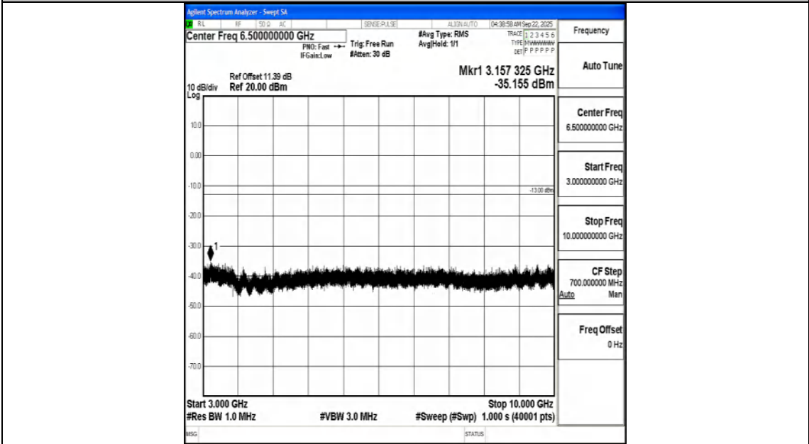
Band71_15MHz_16QAM_133197_1RB#0_3000~10000_3000~10000
