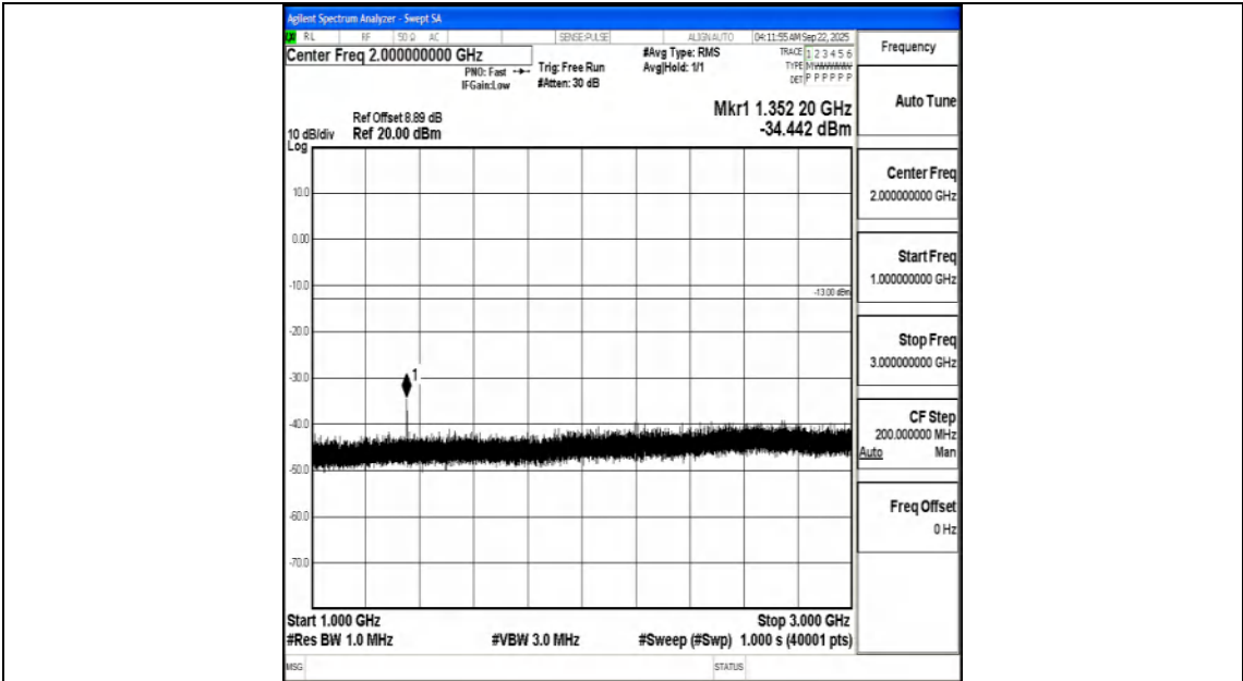
Band71_10MHz_16QAM_133297_1RB#0_1000~3000_1000~3000
