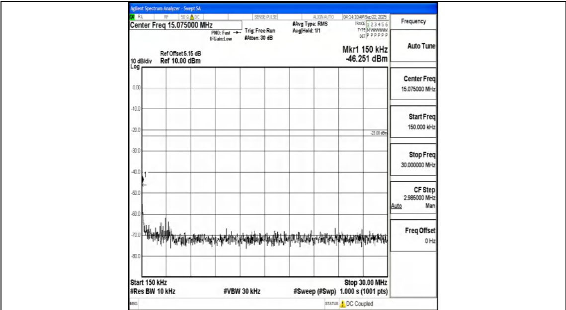
Band71_10MHz_16QAM_133422_1RB#0_0.15~30_0.15~30
