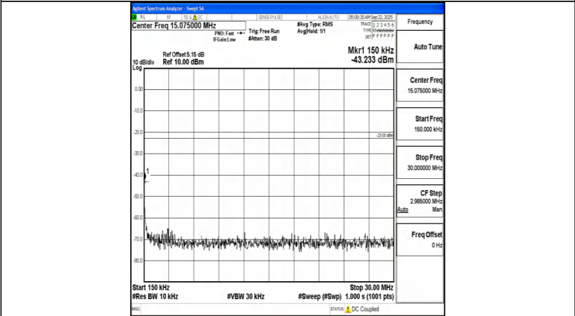
Band71_20MHz_QPSK_133322_1RB#0_0.15~30_0.15~30
