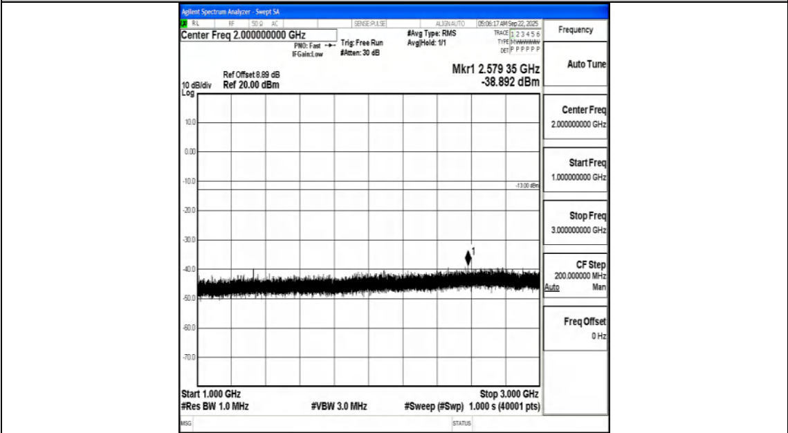
Band71_20MHz_QPSK_133222_1RB#0_1000~3000_1000~3000
