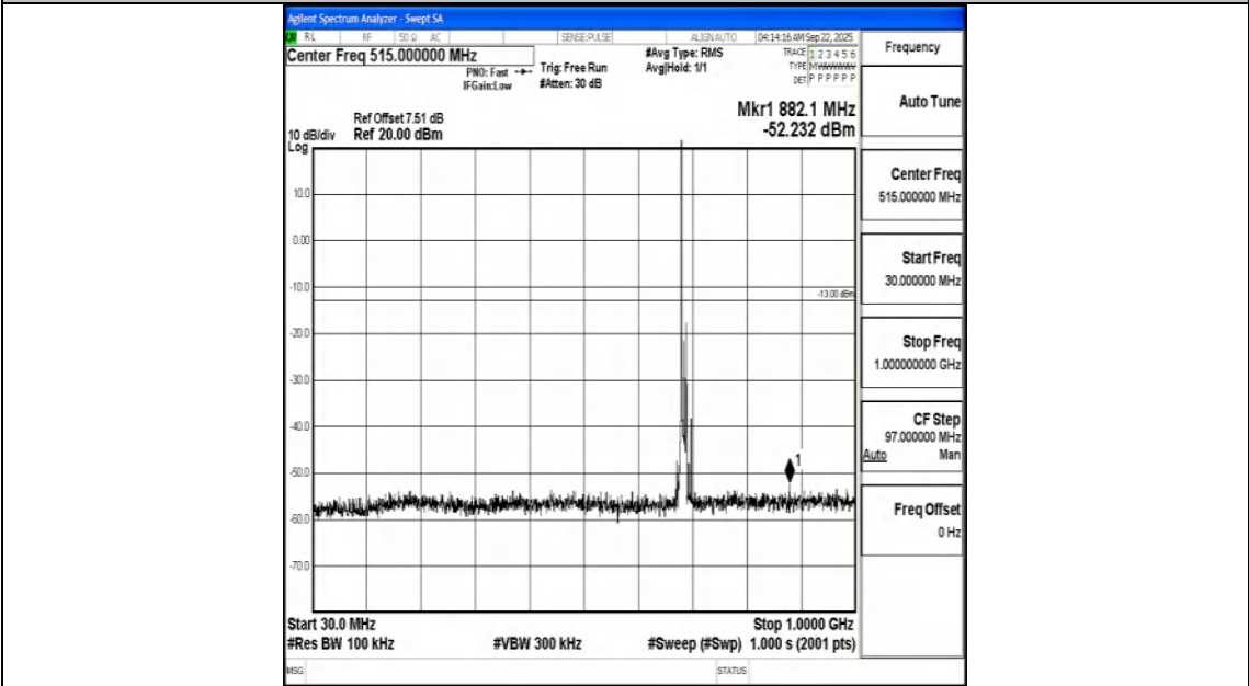
Band71_10MHz_16QAM_133422_1RB#0_30~1000_30~1000
