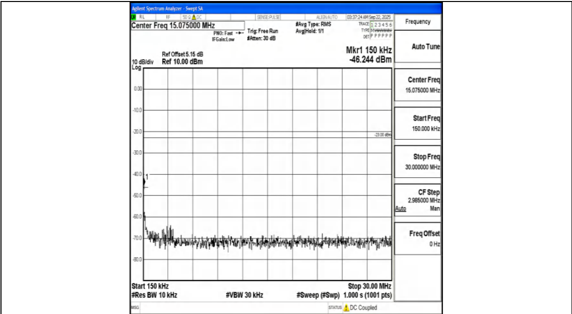
Band71_5MHz_16QAM_133297_1RB#0_0.15~30_0.15~30
