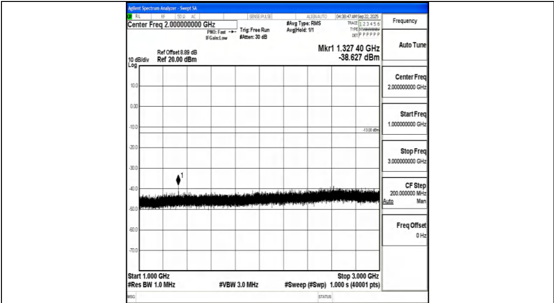
Band71_15MHz_16QAM_133197_1RB#0_1000~3000_1000~3000
