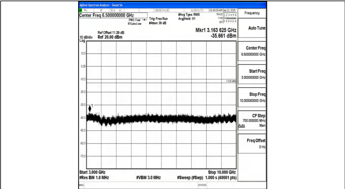
Band71_5MHz_16QAM_133447_1RB#0_3000~10000_3000~10000
