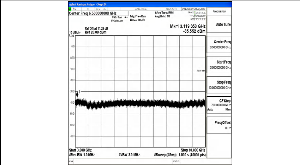
Band71_10MHz_16QAM_133297_1RB#0_3000~10000_3000~10000
