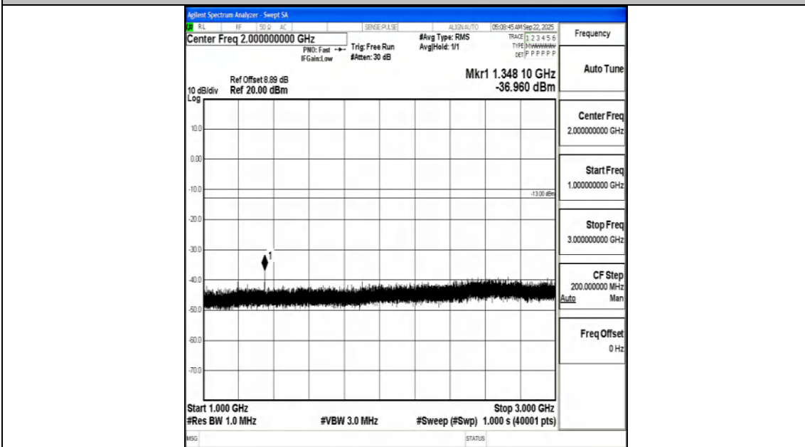
Band71_20MHz_QPSK_133322_1RB#0_1000~3000_1000~3000
