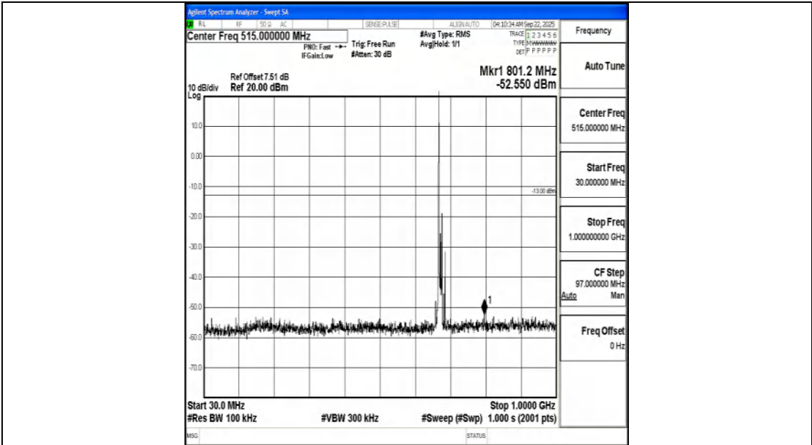
Band71_10MHz_QPSK_133297_1RB#0_30~1000_30~1000
