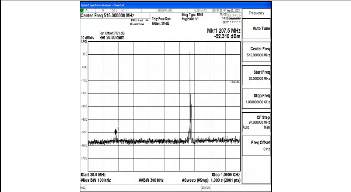
Band71_5MHz_16QAM_133297_1RB#0_30~1000_30~1000
