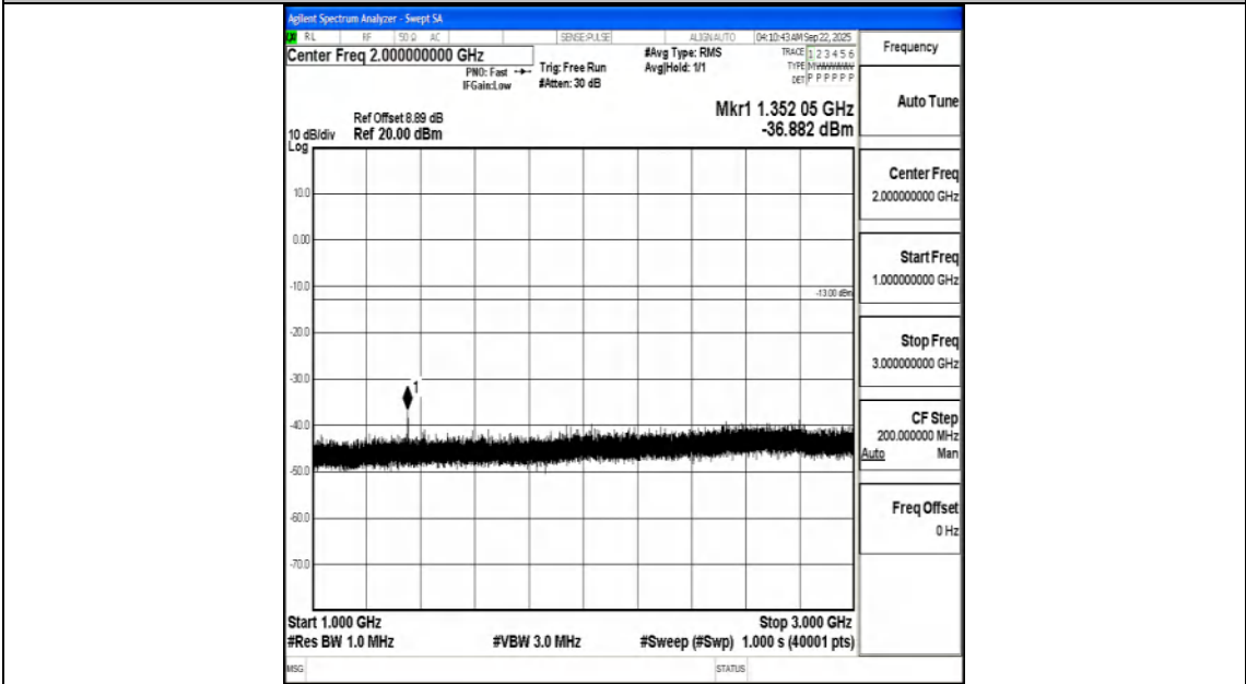
Band71_10MHz_QPSK_133297_1RB#0_1000~3000_1000~3000
