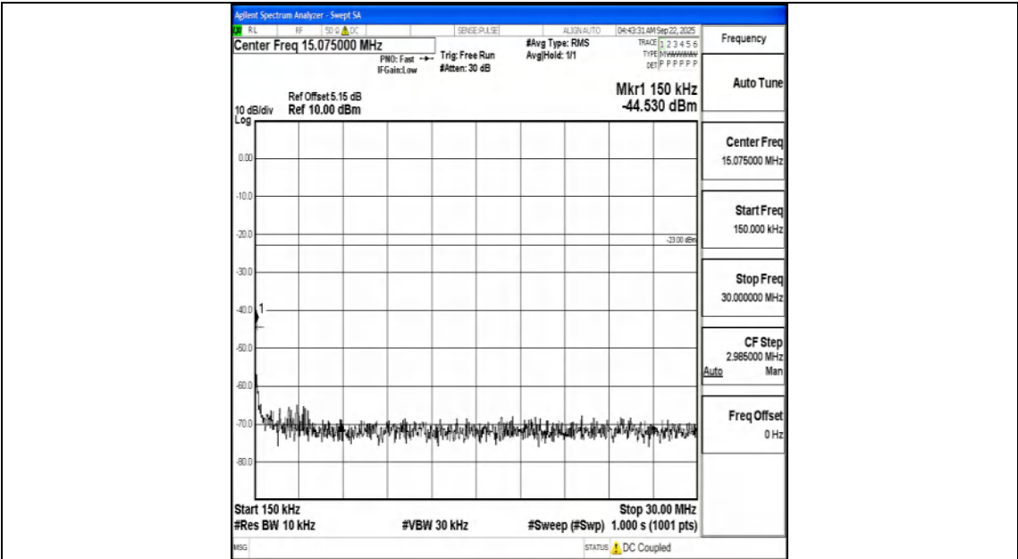
Band71_15MHz_16QAM_133397_1RB#0_0.15~30_0.15~30
