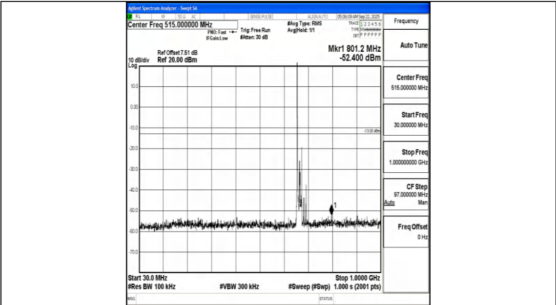
Band71_20MHz_QPSK_133222_1RB#0_30~1000_30~1000
