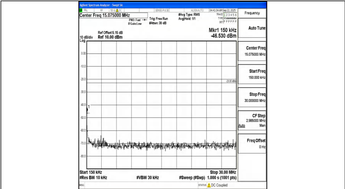
Band71_15MHz_16QAM_133297_1RB#0_0.15~30_0.15~30
