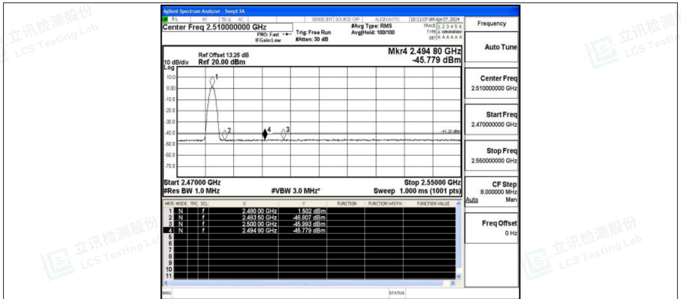
DH5_Ant1_High_2480_Peak
