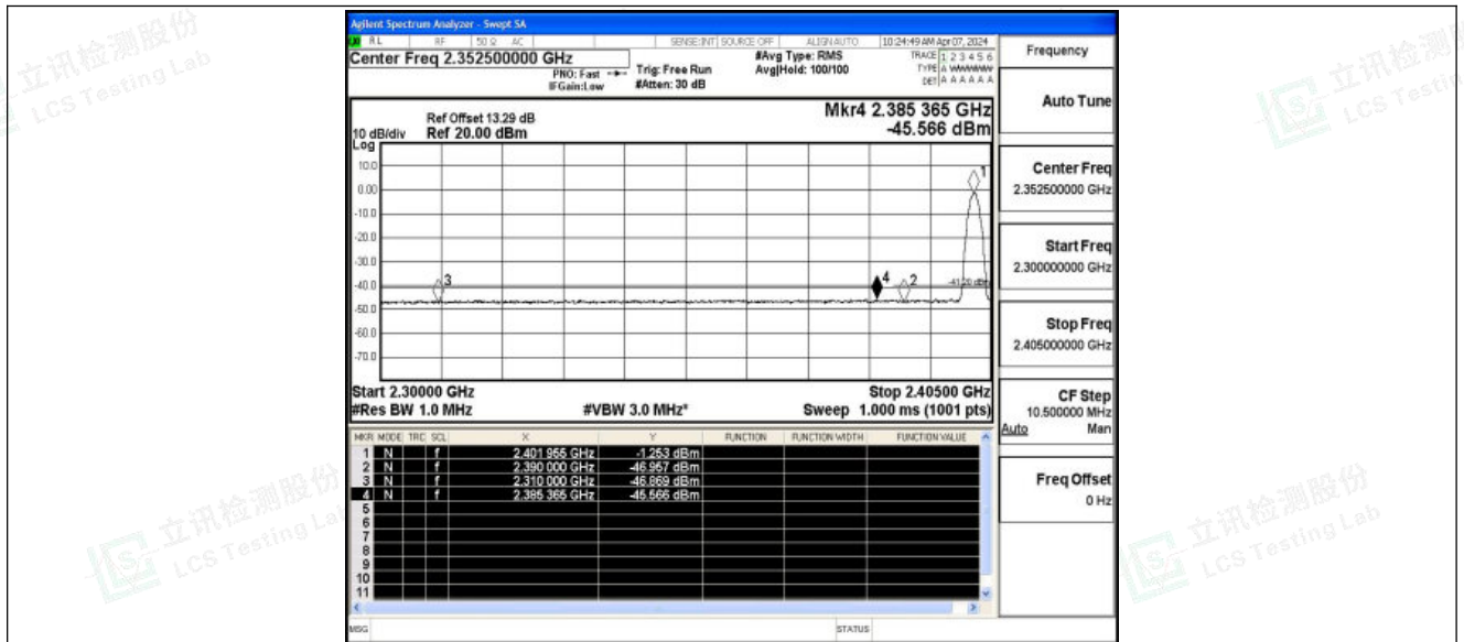
3DH5_Ant1_Low_2402_Peak
