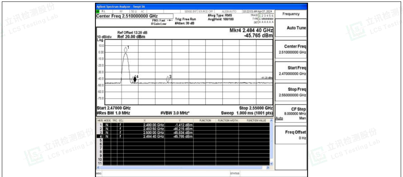
2DH5_Ant1_High_2480_Peak
