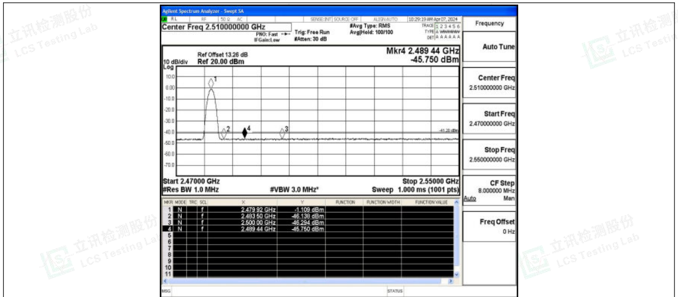
3DH5_Ant1_High_2480_Peak
