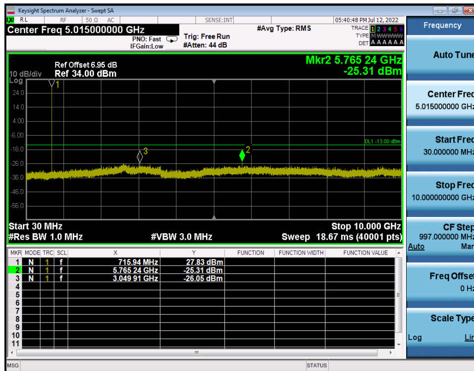
LTE Band 12 / 1.4MHz / 16QAM - RB Size/Offset (1/5) - High Channel
