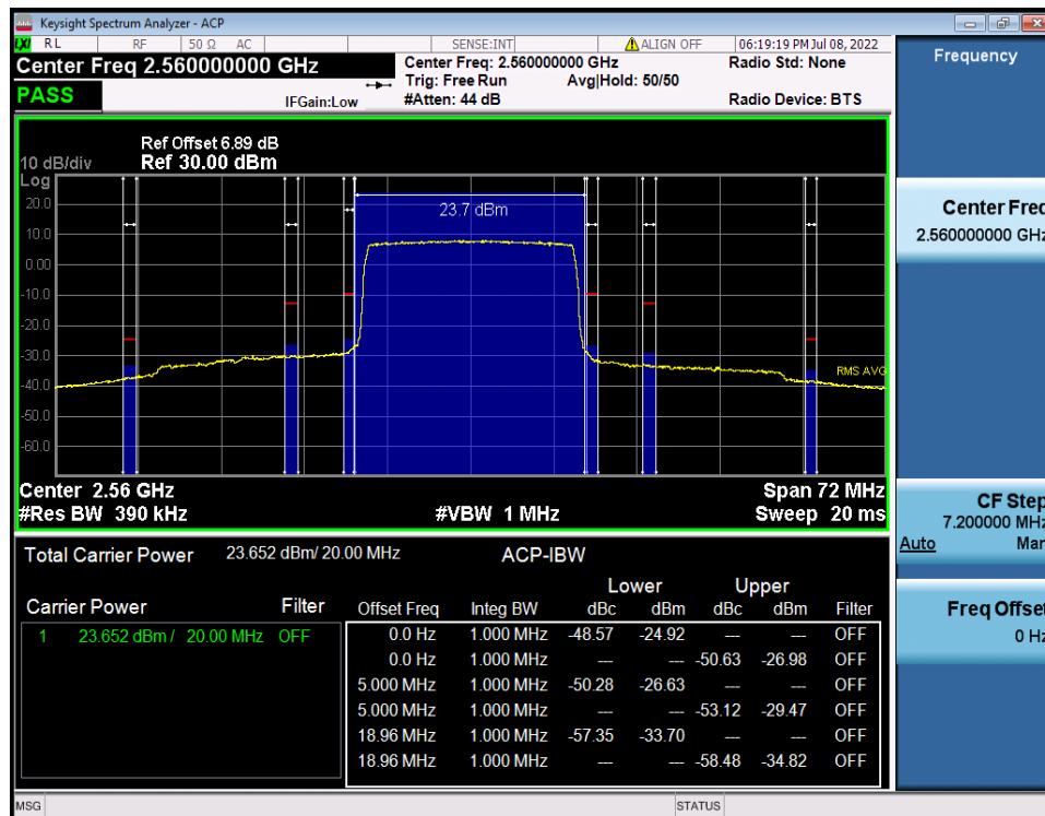
LTE Band 7 / 20MHz / QPSK - RB Size/Offset (100/0)
