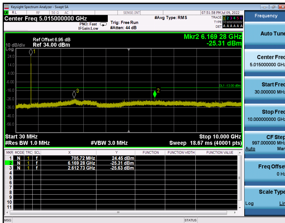
LTE Band 12 / 5MHz / QPSK - RB Size/Offset (12/6) - Mid Channel
