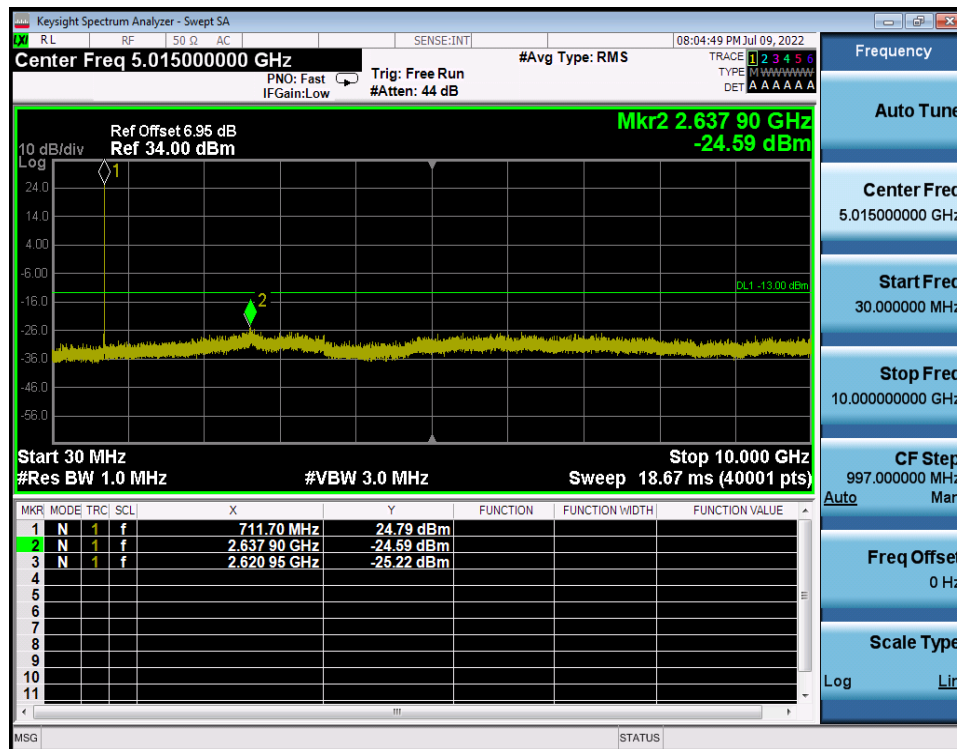
LTE Band 12 / 5MHz / QPSK - RB Size/Offset (12/6) - High Channel
