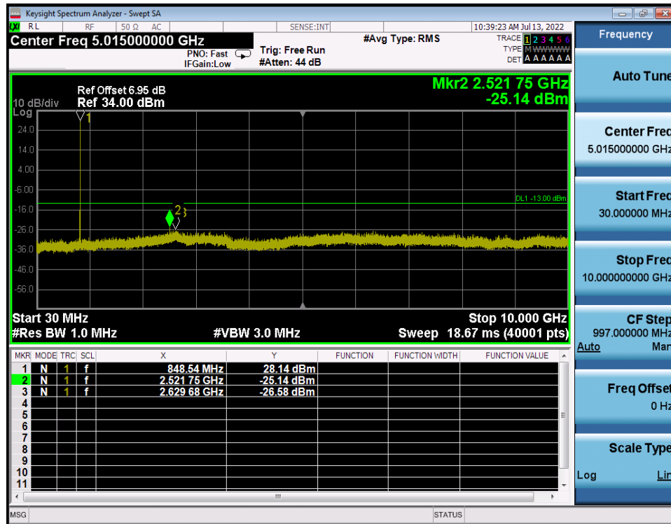
LTE Band 26 / 10MHz / 16QAM - RB Size/Offset (1/49) - High Channel
