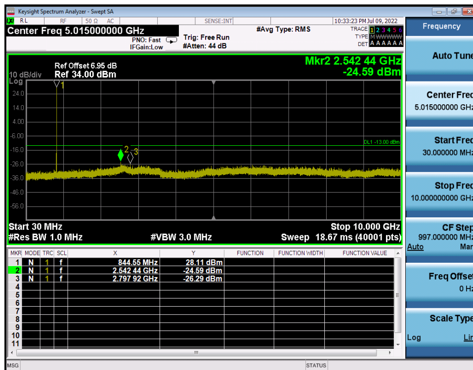
LTE Band 26 / 5MHz / QPSK - RB Size/Offset (1/0) - High Channel
