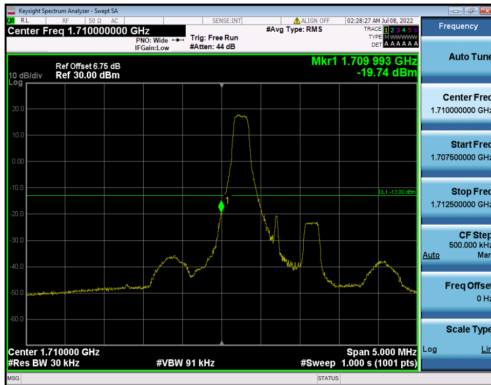
LTE Band 4 / 1.4MHz / QPSK - RB Size/Offset (1/0)
