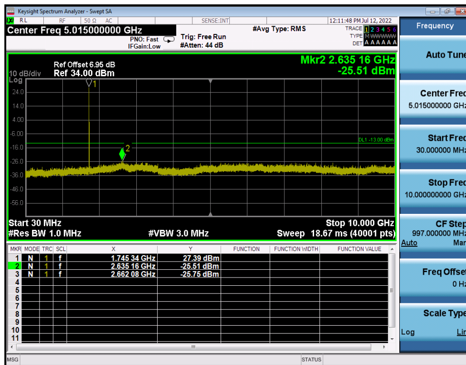
LTE Band 4 / 20MHz / 16QAM - RB Size/Offset (1/50) - High Channel
