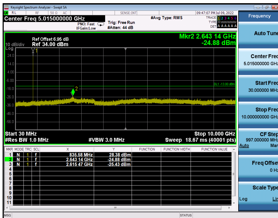
LTE Band 26 / 3MHz / QPSK - RB Size/Offset (8/0) - Mid Channel
