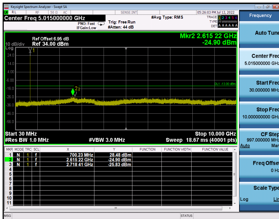
LTE Band 12 / 1.4MHz / 16QAM - RB Size/Offset (3/3) - Low Channel
