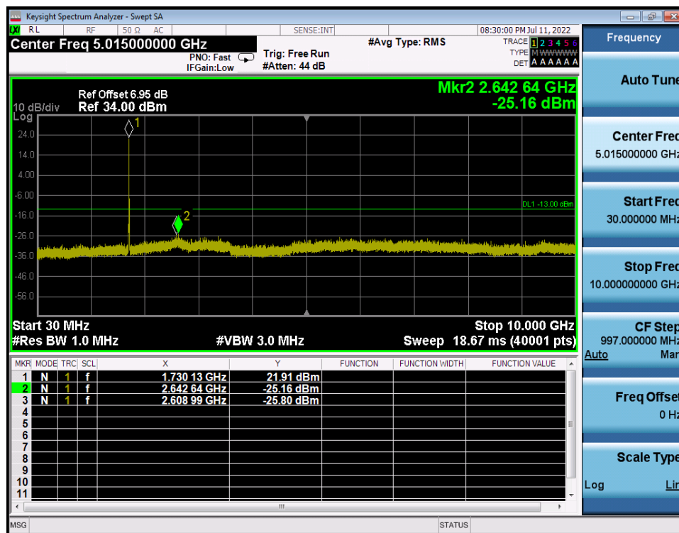
LTE Band 4 / 15MHz / QPSK - RB Size/Offset (36/18) - Mid Channel
