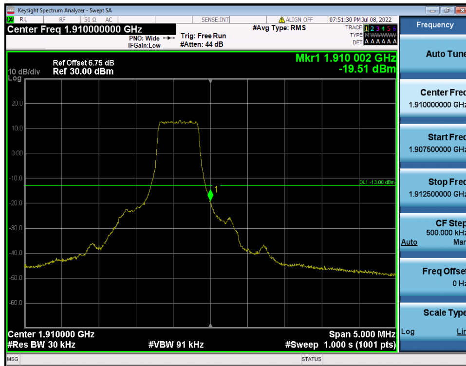
LTE Band 2 / 1.4MHz / 16QAM - RB Size/Offset (3/3)
