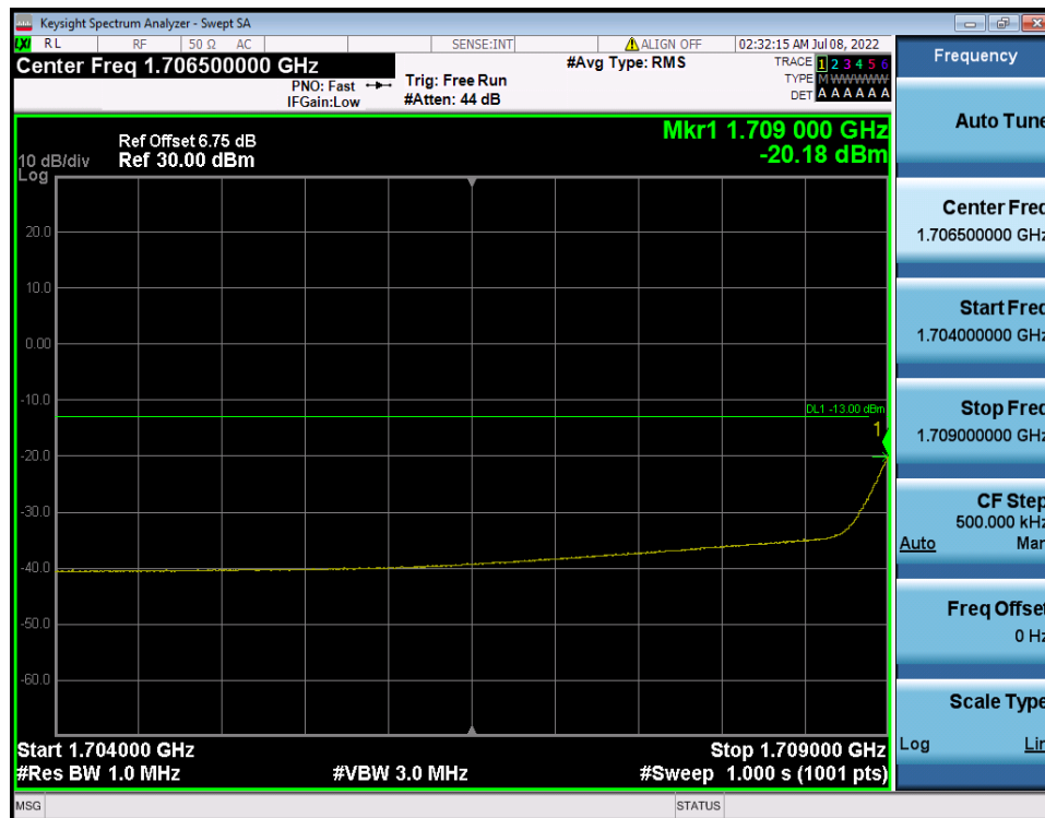
LTE Band 4 / 1.4MHz / QPSK - RB Size/Offset (1/2)
