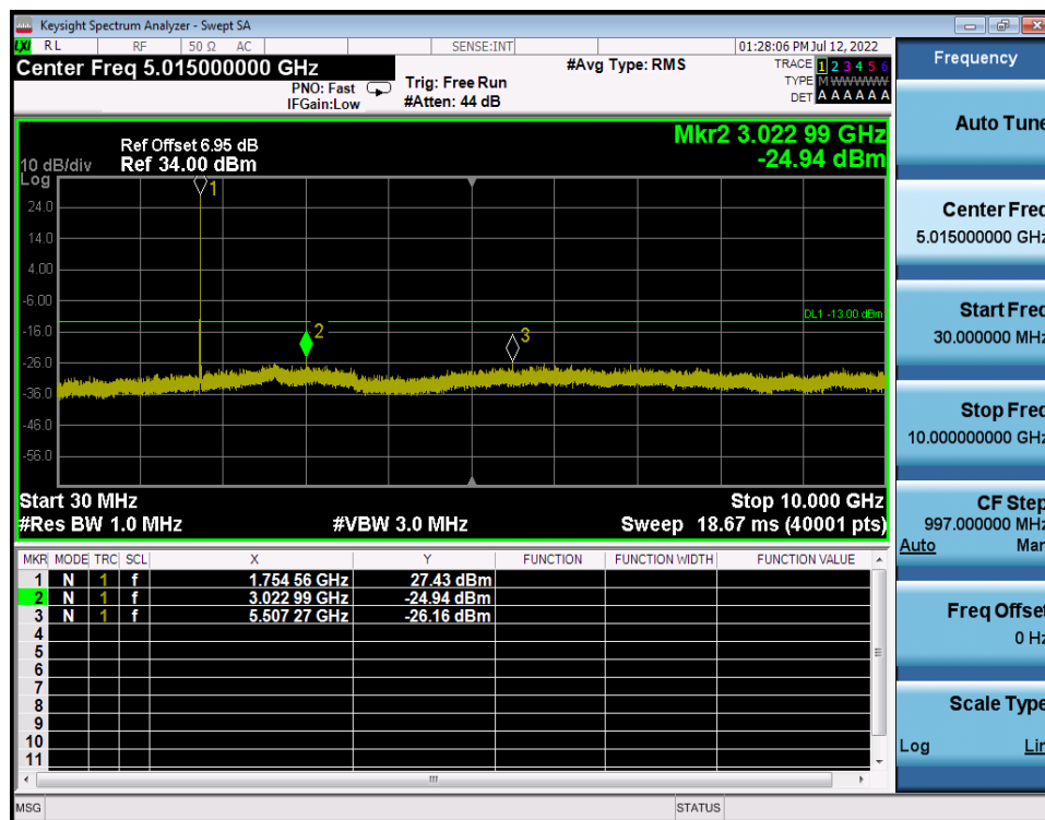
LTE Band 4 / 10MHz / 16QAM - RB Size/Offset (1/49) - High Channel
