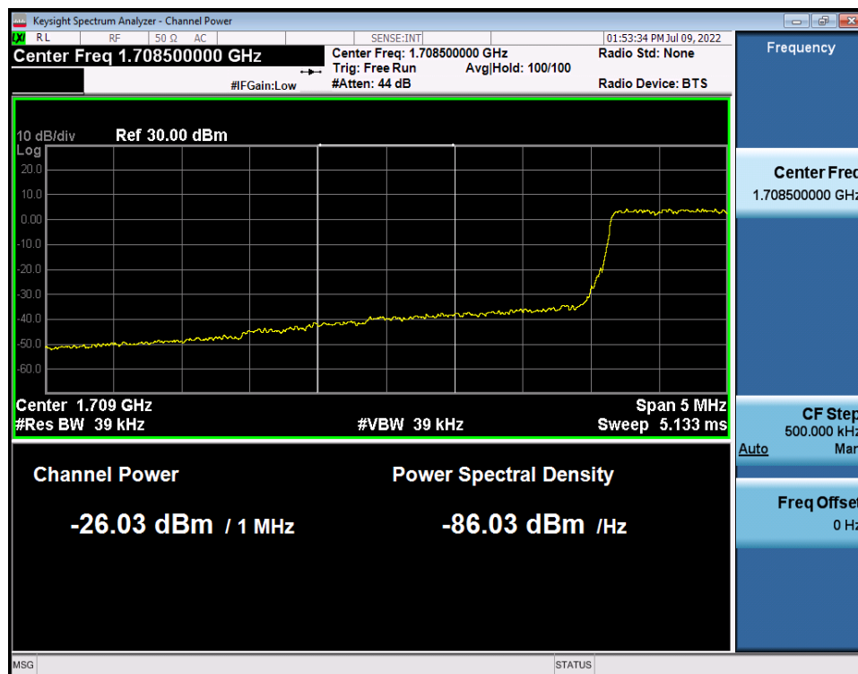
LTE Band 4 / 3MHz / 16QAM - RB Size/Offset (15/0)
