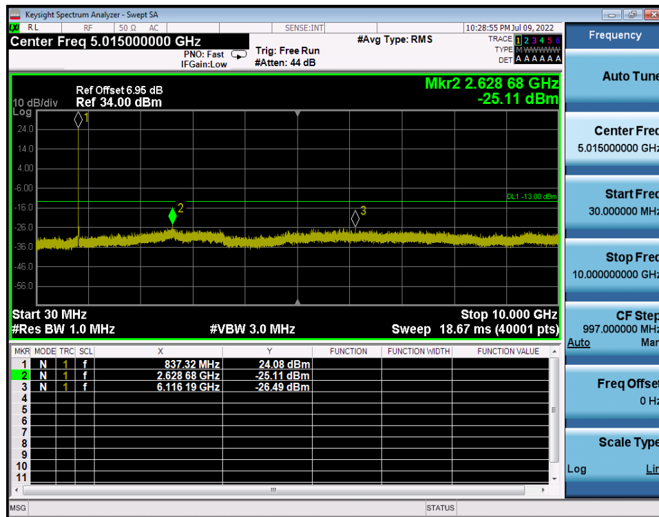
LTE Band 26 / 5MHz / QPSK - RB Size/Offset (12/13) - Mid Channel
