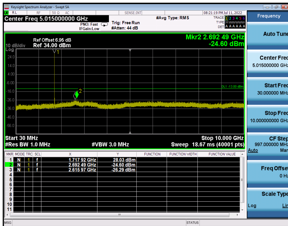
LTE Band 4 / 15MHz / QPSK - RB Size/Offset (1/36) - Low Channel
