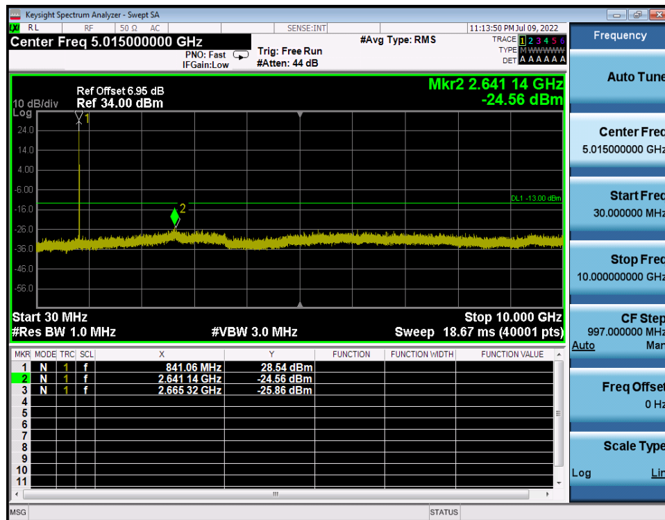
LTE Band 26 / 10MHz / QPSK - RB Size/Offset (1/49) - Mid Channel
