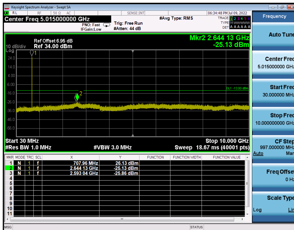
LTE Band 12 / 1.4MHz / QPSK - RB Size/Offset (6/0) - Mid Channel
