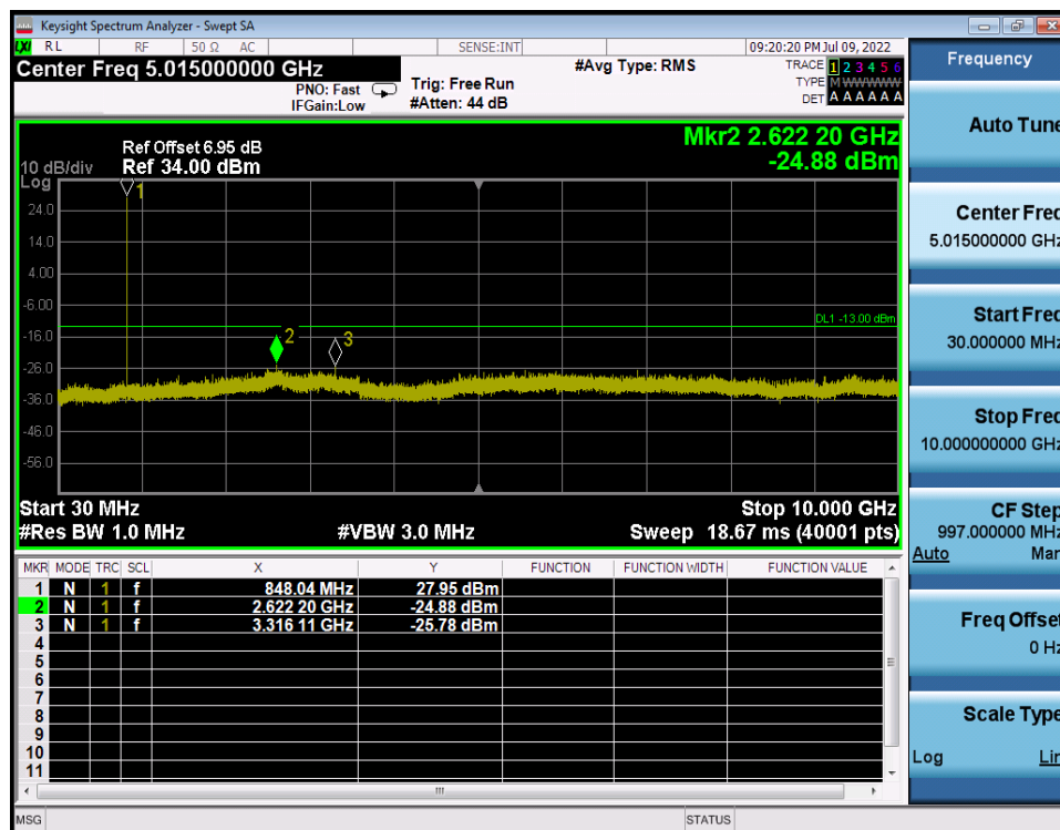
LTE Band 26 / 1.4MHz / QPSK - RB Size/Offset (3/2) - High Channel
