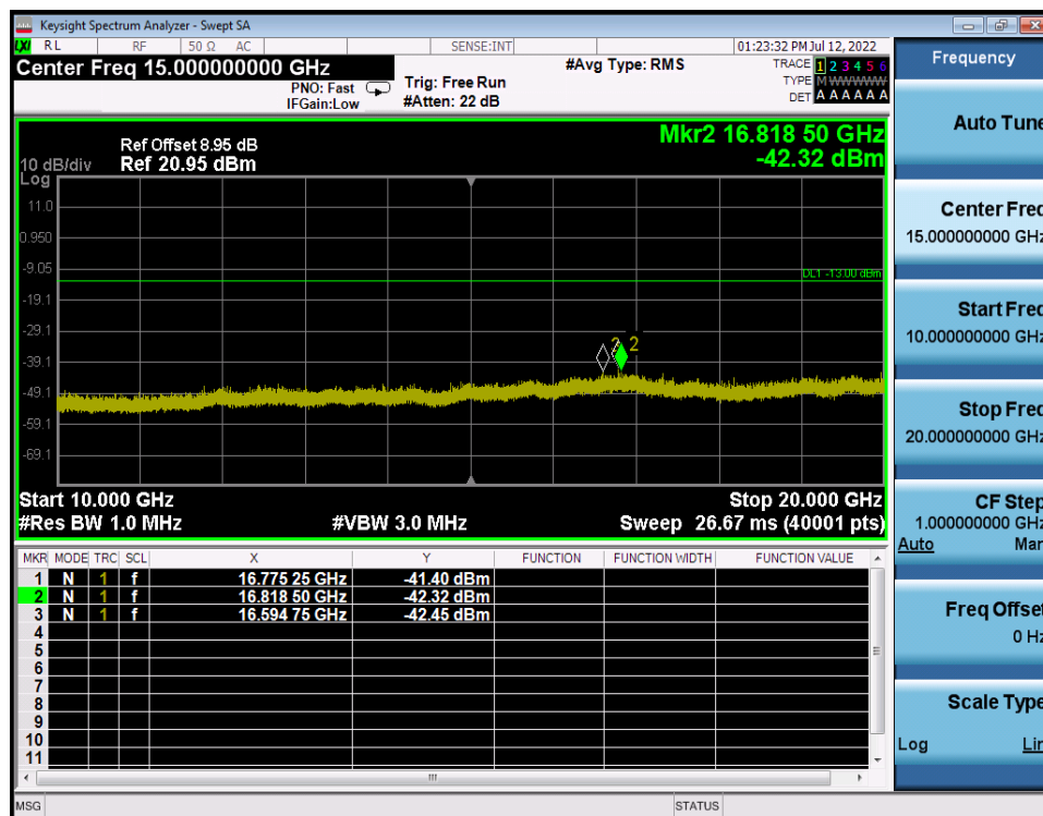
LTE Band 4 / 10MHz / 16QAM - RB Size/Offset (25/0) - Mid Channel
