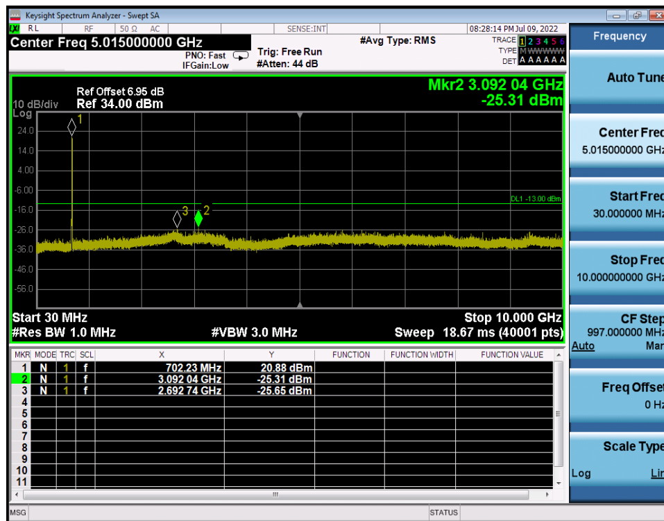
LTE Band 12 / 10MHz / QPSK - RB Size/Offset (50/0) - Low Channel
