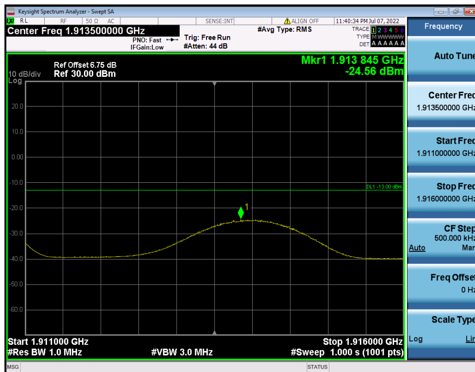
LTE Band 2 / 5MHz / QPSK - RB Size/Offset (1/0)
