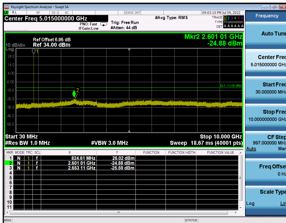
LTE Band 26 / 1.4MHz / QPSK - RB Size/Offset (6/0) - Low Channel
