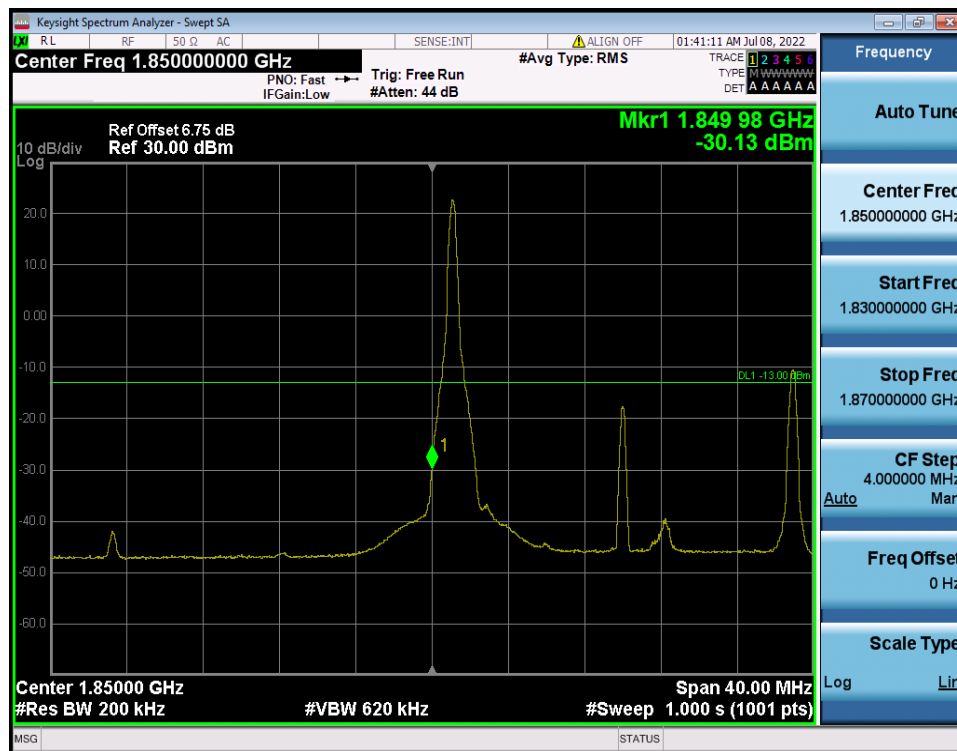
LTE Band 2 / 20MHz / QPSK - RB Size/Offset (1/0)
