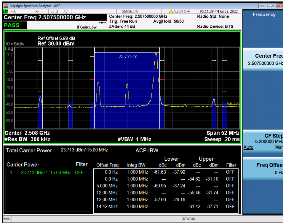
LTE Band 7 / 15MHz / QPSK - RB Size/Offset (1/74)
