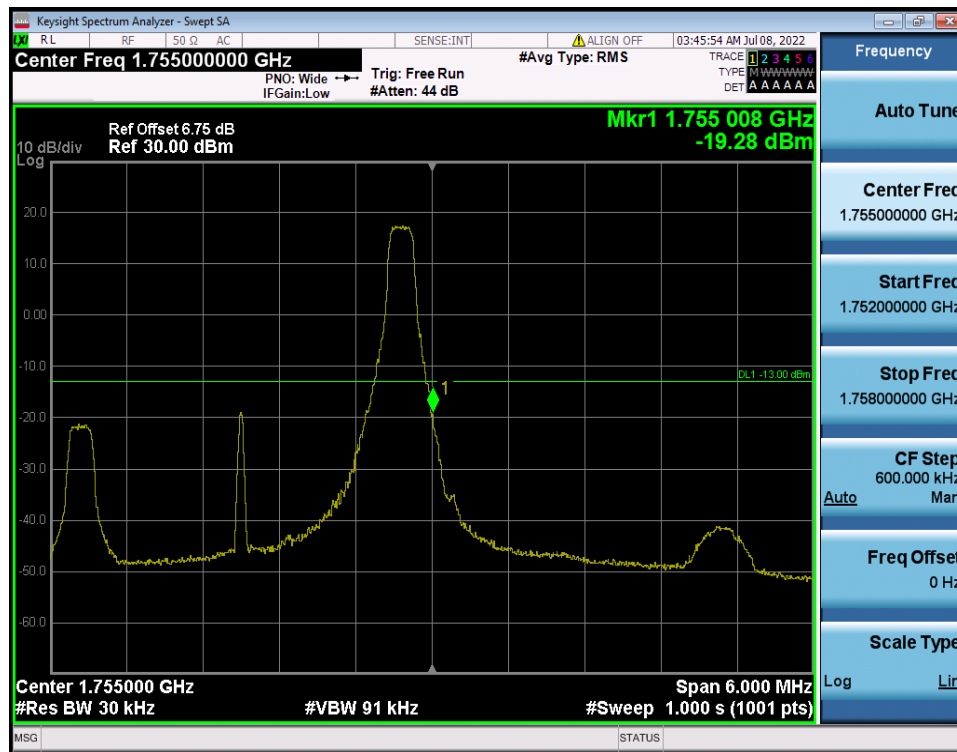
LTE Band 4 / 3MHz / QPSK - RB Size/Offset (1/14)
