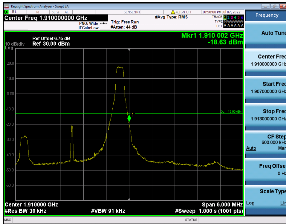
LTE Band 2 / 3MHz / QPSK - RB Size/Offset (1/14)
