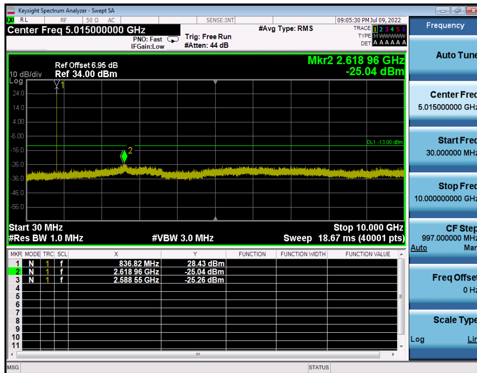
LTE Band 26 / 1.4MHz / QPSK - RB Size/Offset (1/2) - Mid Channel
