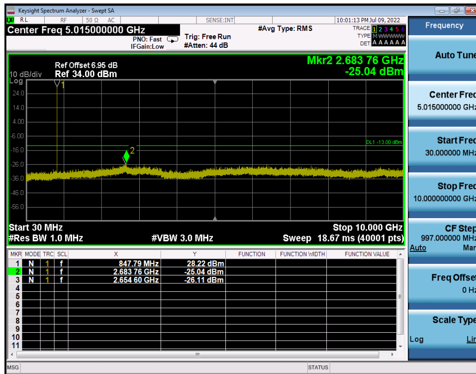
LTE Band 26 / 3MHz / QPSK - RB Size/Offset (8/4) - High Channel
