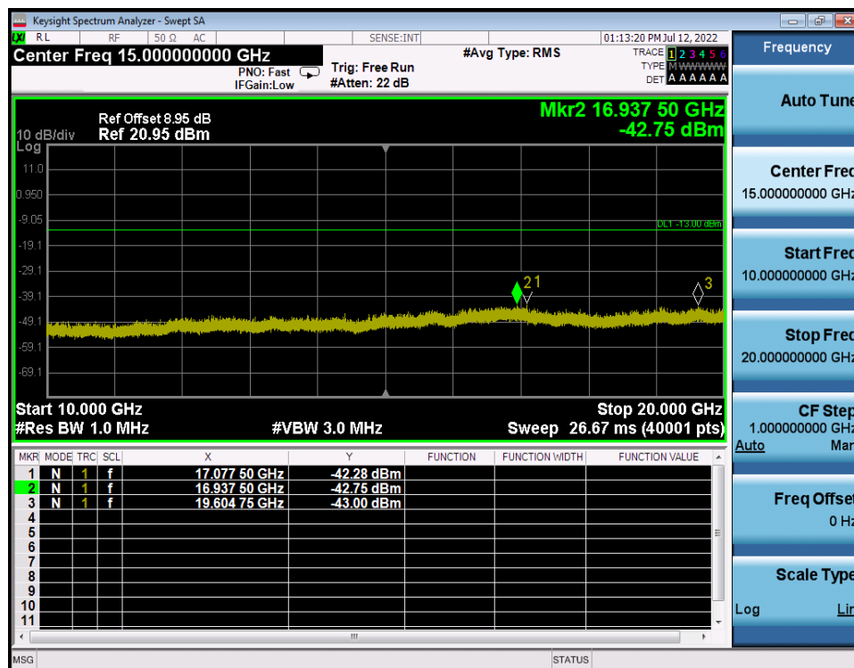
LTE Band 4 / 10MHz / 16QAM - RB Size/Offset (1/49) - Low Channel
