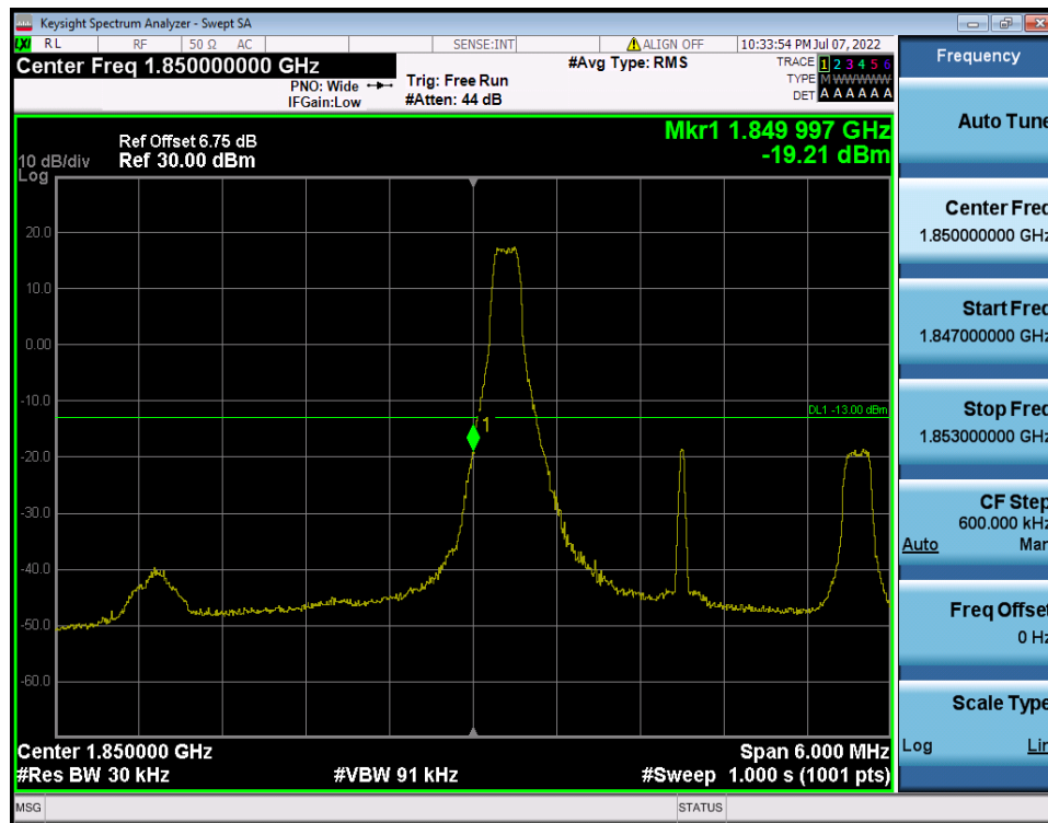
LTE Band 2 / 3MHz / QPSK - RB Size/Offset (8/0)
