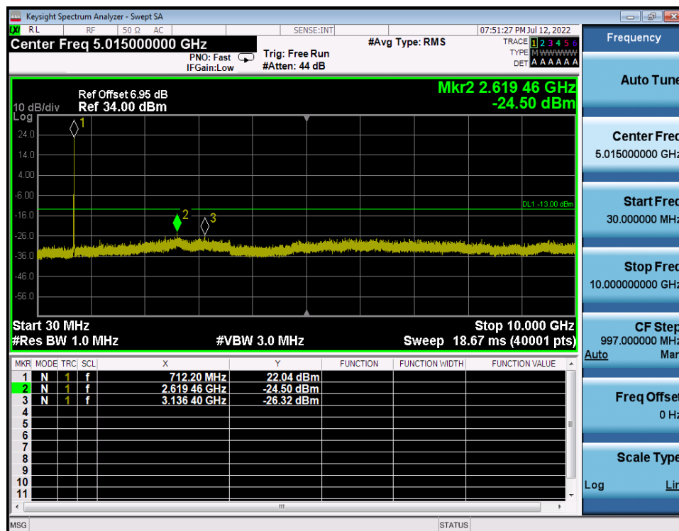
LTE Band 12 / 10MHz / 16QAM - RB Size/Offset (25/25) - High Channel
