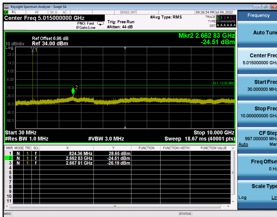
LTE Band 26 / 3MHz / QPSK - RB Size/Offset (8/0) - Low Channel
