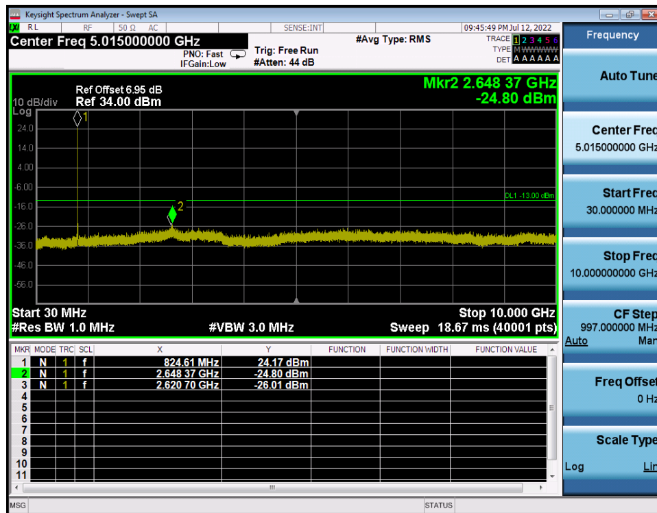
LTE Band 26 / 5MHz / 16QAM - RB Size/Offset (12/0) - Low Channel
