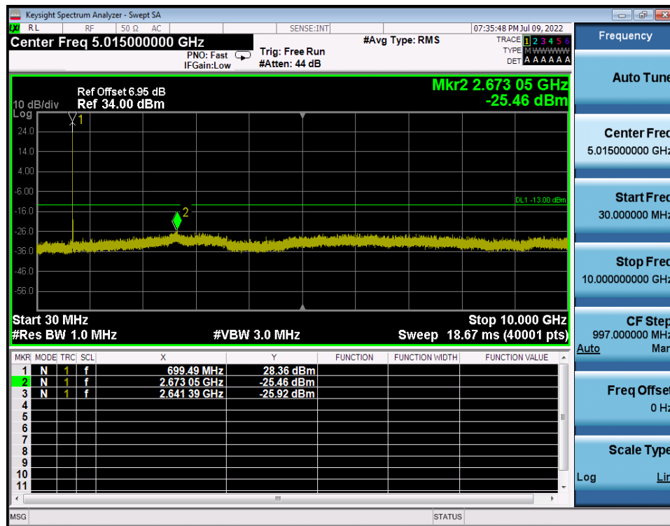
LTE Band 12 / 5MHz / QPSK - RB Size/Offset (1/0) - Low Channel
