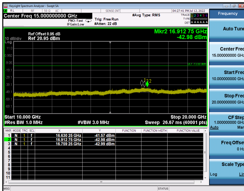
LTE Band 2 / 15MHz / 16QAM - RB Size/Offset (27/48) - Mid Channel
