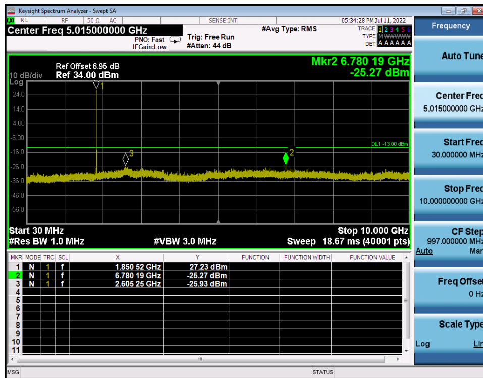
LTE Band 2 / 5MHz / QPSK - RB Size/Offset (1/0) - Low Channel
