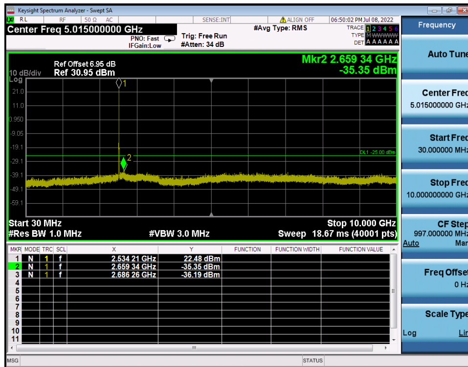
LTE Band 7 / 5MHz / 16QAM - RB Size/Offset (25/0) - Mid Channel
