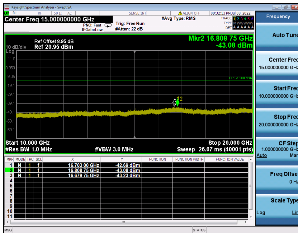
LTE Band 2 / 3MHz / 16QAM - RB Size/Offset (1/14) - High Channel
