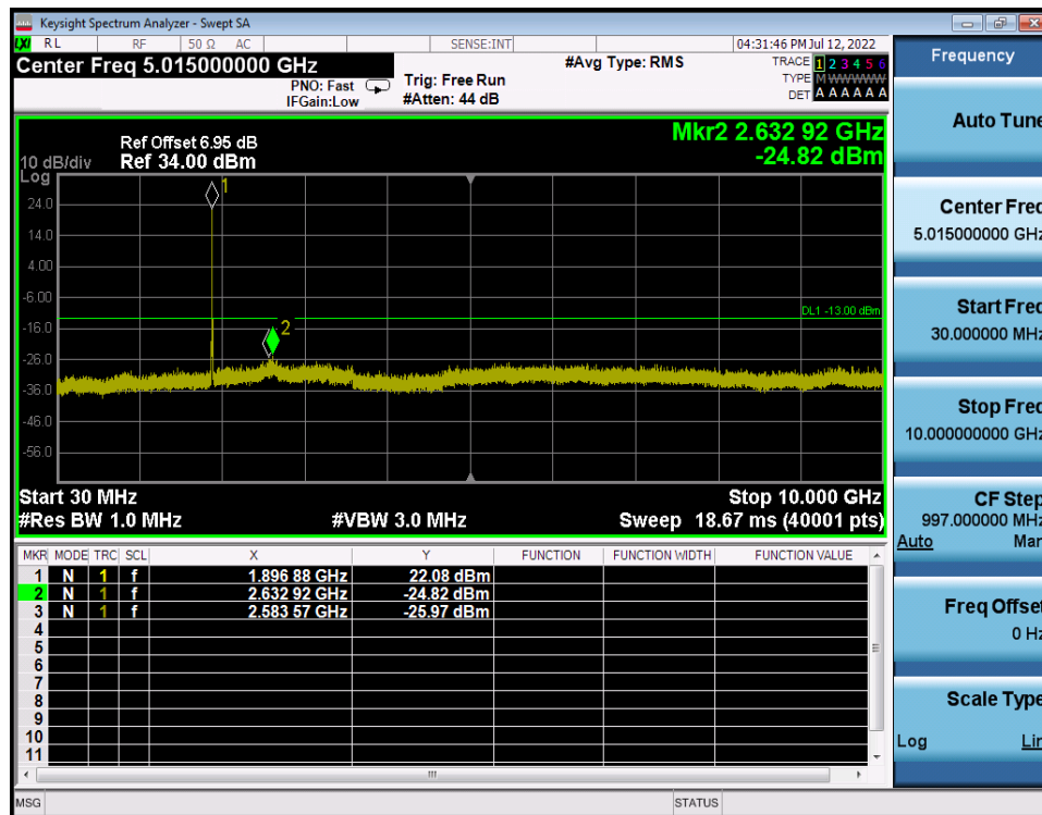
LTE Band 2 / 15MHz / 16QAM - RB Size/Offset (27/0) - High Channel
