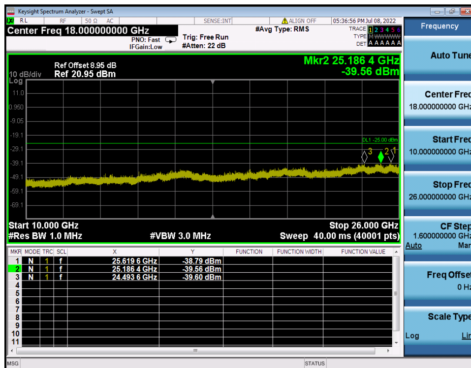
LTE Band 7 / 15MHz / QPSK - RB Size/Offset (36/0) - High Channel
