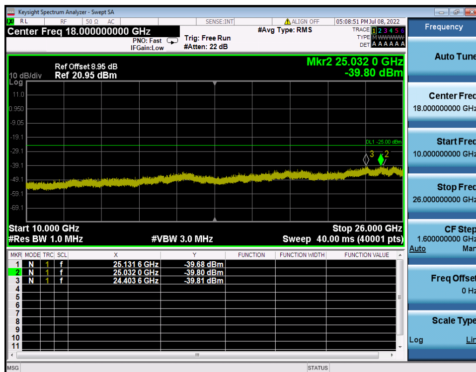
LTE Band 7 / 15MHz / QPSK - RB Size/Offset (1/0) - Low Channel
