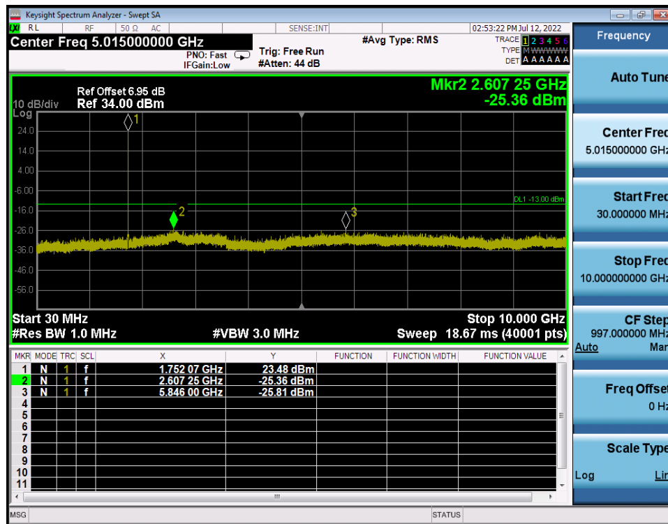
LTE Band 4 / 5MHz / 16QAM - RB Size/Offset (12/0) - High Channel
