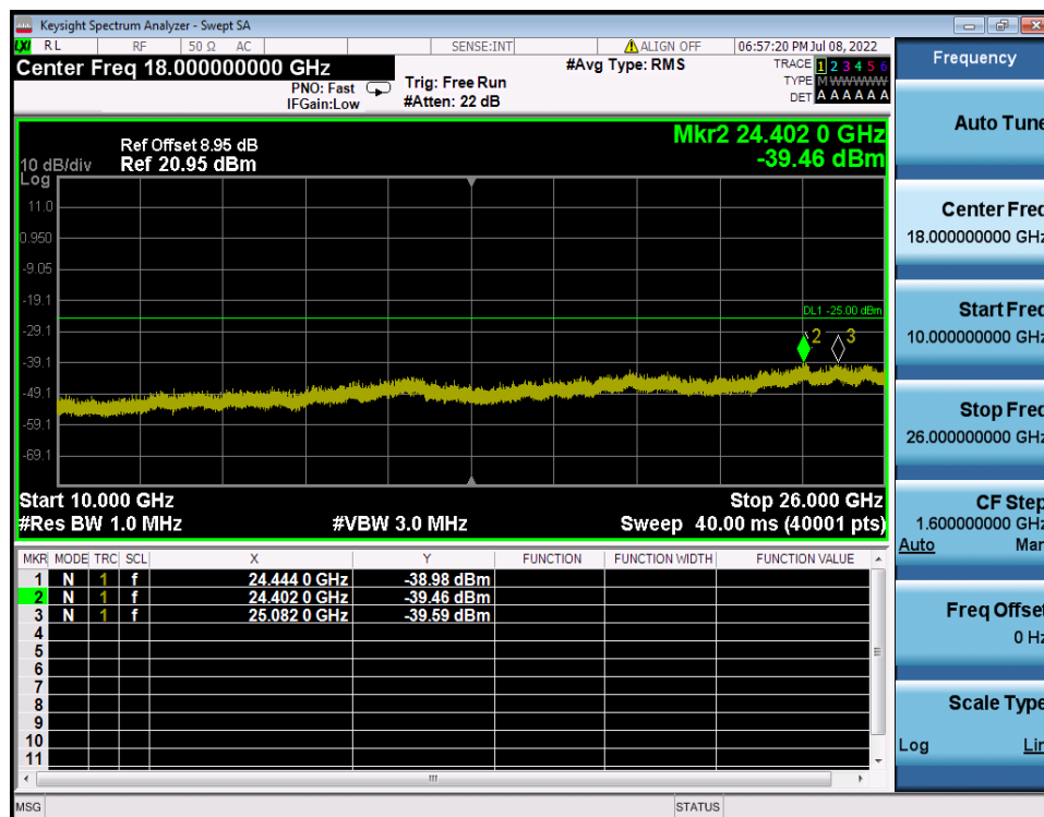
LTE Band 7 / 5MHz / 16QAM - RB Size/Offset (12/6) - High Channel
