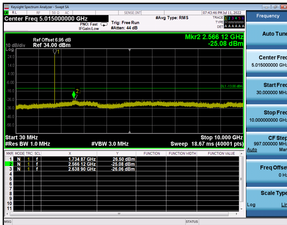
LTE Band 4 / 5MHz / QPSK - RB Size/Offset (1/24) - Mid Channel
