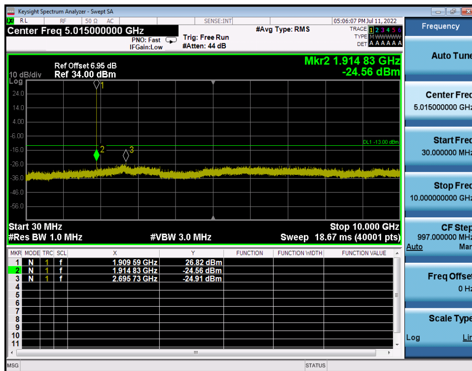
LTE Band 2 / 1.4MHz / QPSK - RB Size/Offset (1/2) - High Channel
