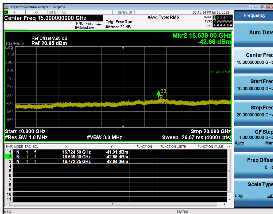
LTE Band 2 / 20MHz / QPSK - RB Size/Offset (50/0) - Mid Channel
