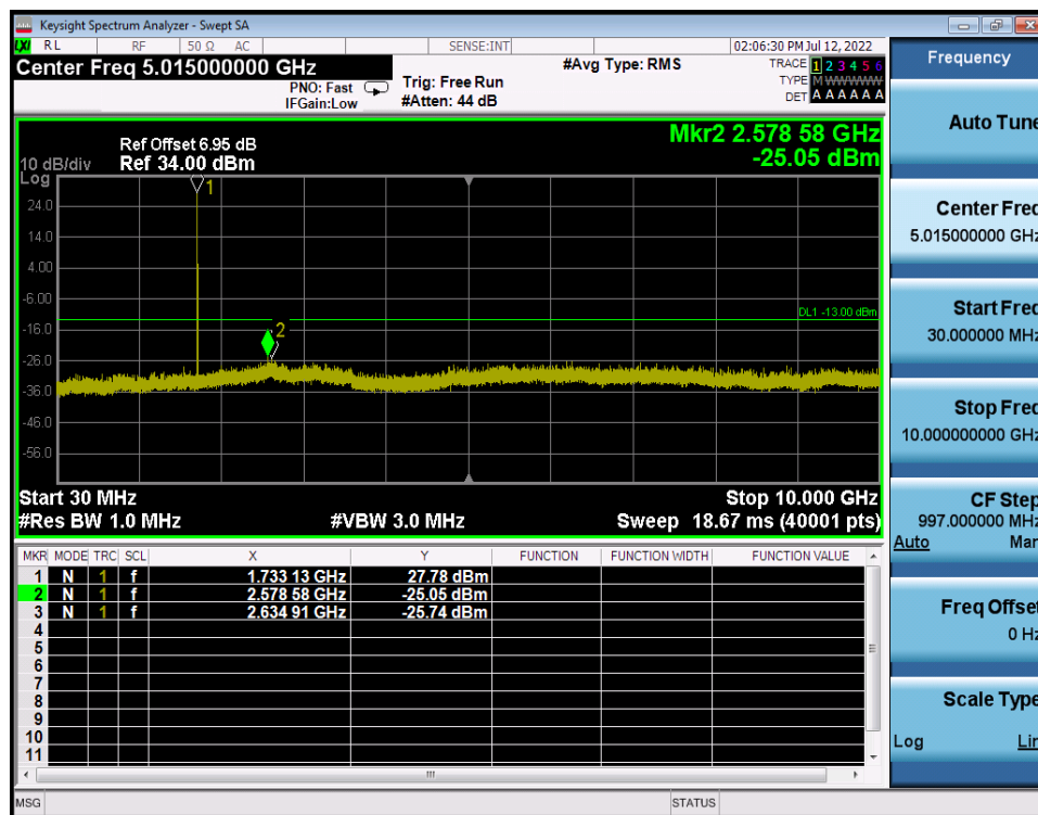
LTE Band 4 / 1.4MHz / 16QAM - RB Size/Offset (1/5) - Mid Channel
