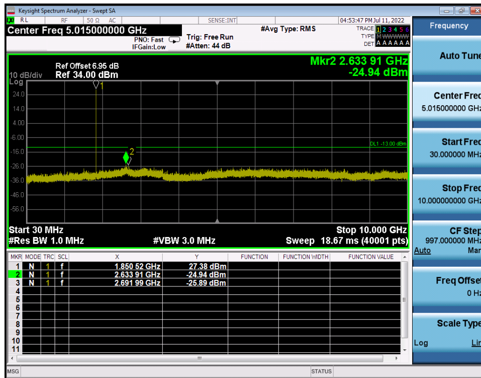
LTE Band 2 / 1.4MHz / QPSK - RB Size/Offset (1/0) - Low Channel
