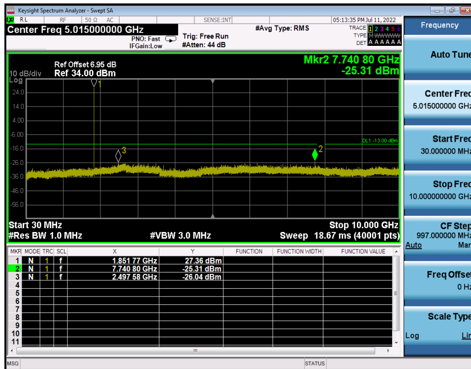
LTE Band 2 / 3MHz / QPSK - RB Size/Offset (1/7) - Low Channel
