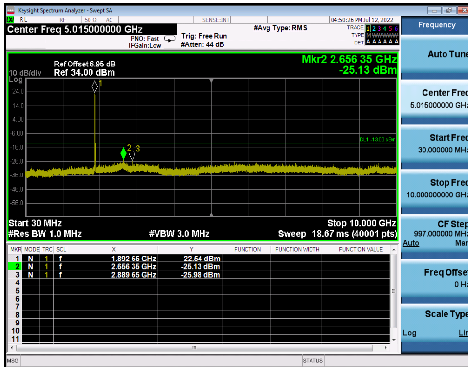
LTE Band 2 / 20MHz / 16QAM - RB Size/Offset (27/0) - High Channel
