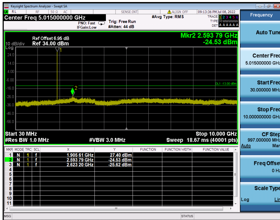
LTE Band 2 / 5MHz / 16QAM - RB Size/Offset (1/0) - High Channel
