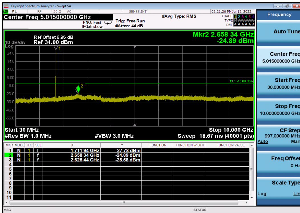
LTE Band 4 / 3MHz / 16QAM - RB Size/Offset (8/4) - Low Channel
