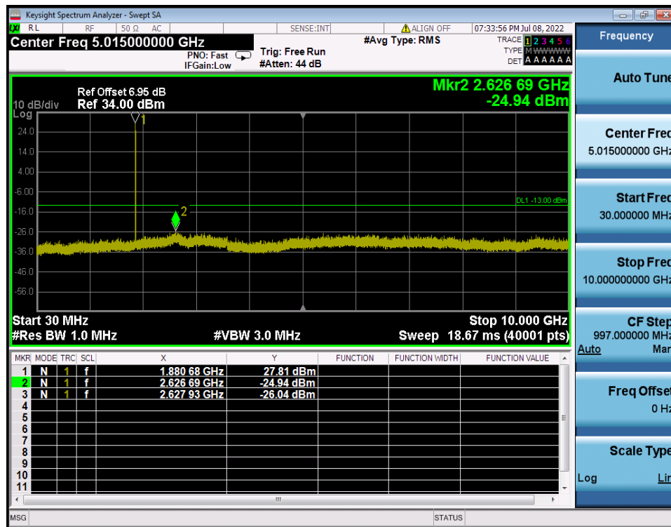
LTE Band 2 / 1.4MHz / 16QAM - RB Size/Offset (1/5) - Mid Channel
