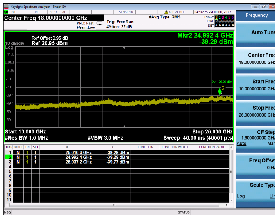
LTE Band 7 / 10MHz / QPSK - RB Size/Offset (25/0) - High Channel
