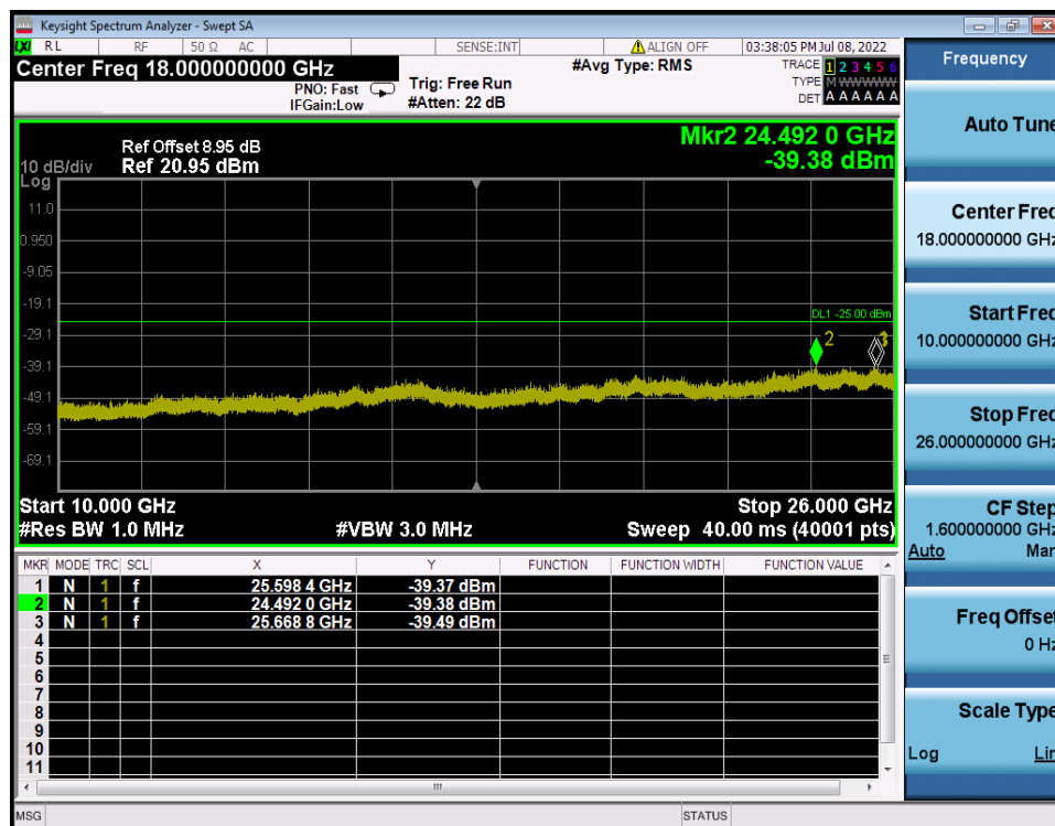
LTE Band 7 / 20MHz / 16QAM - RB Size/Offset (27/0) - Mid Channel
