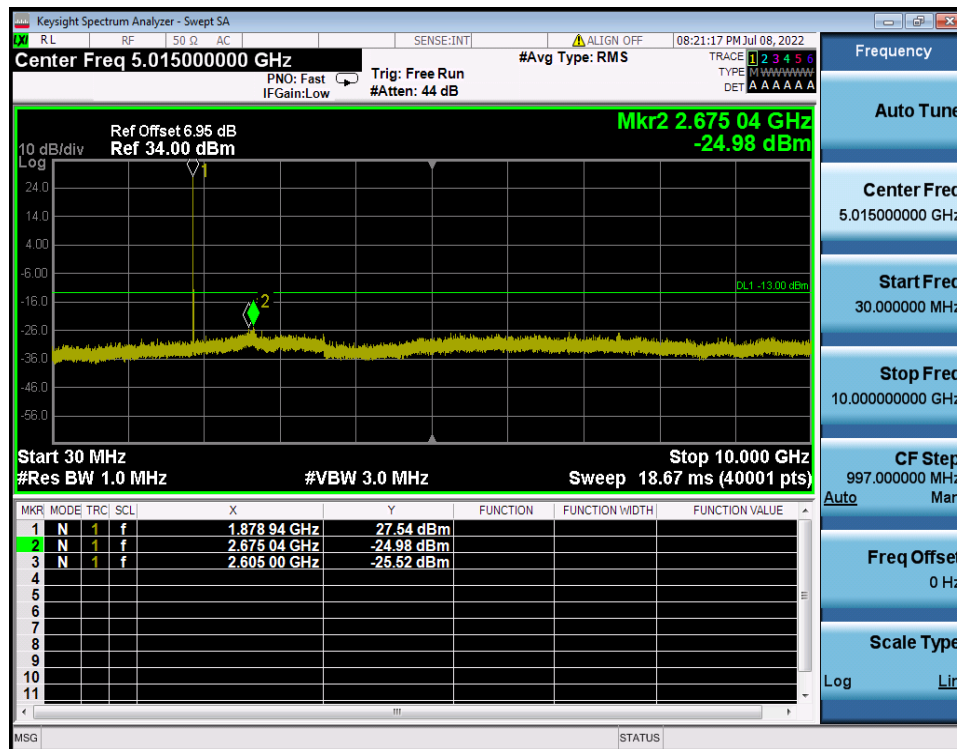
LTE Band 2 / 3MHz / 16QAM - RB Size/Offset (8/0) - Mid Channel
