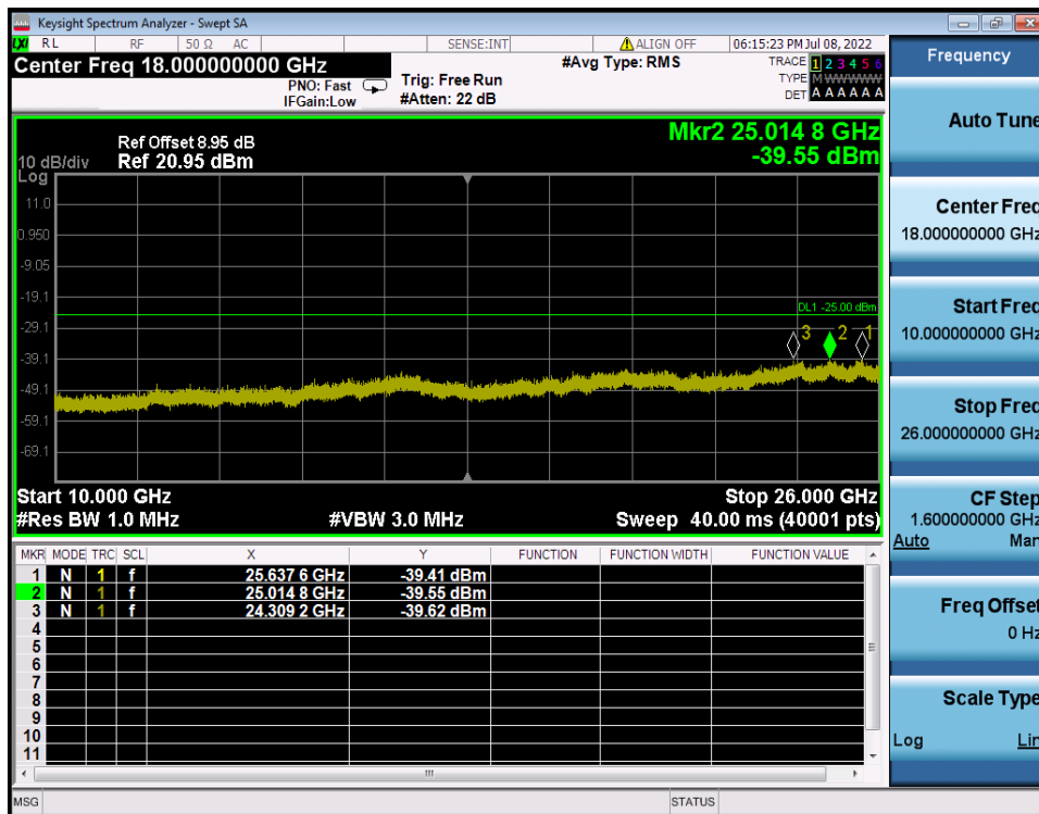
LTE Band 7 / 20MHz / QPSK - RB Size/Offset (50/0) - High Channel
