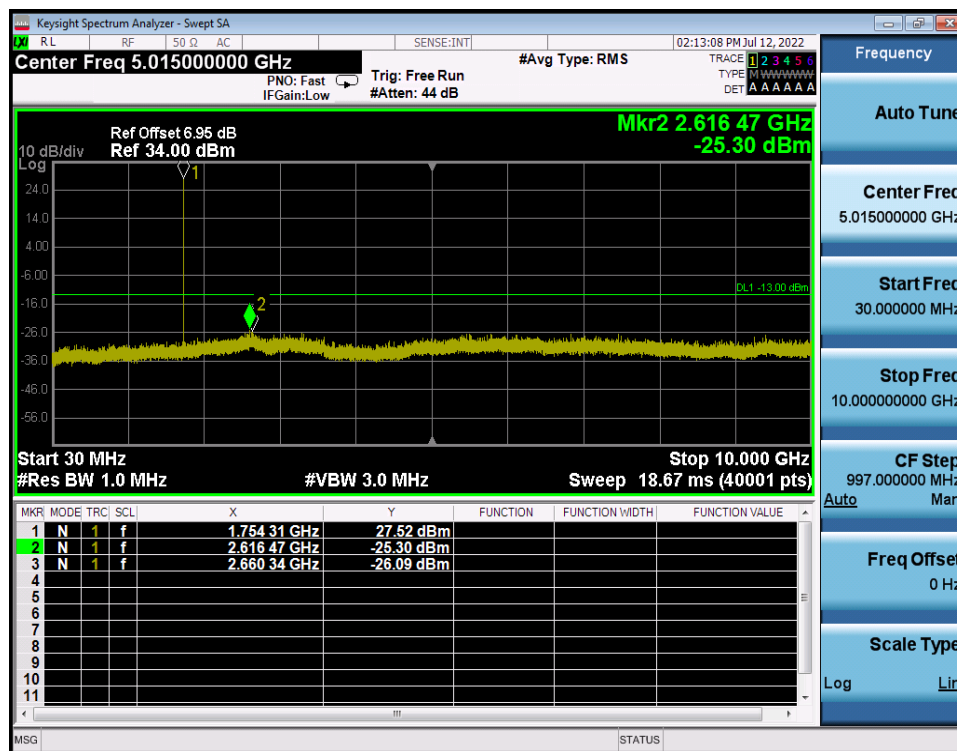
LTE Band 4 / 1.4MHz / 16QAM - RB Size/Offset (3/0) - High Channel
