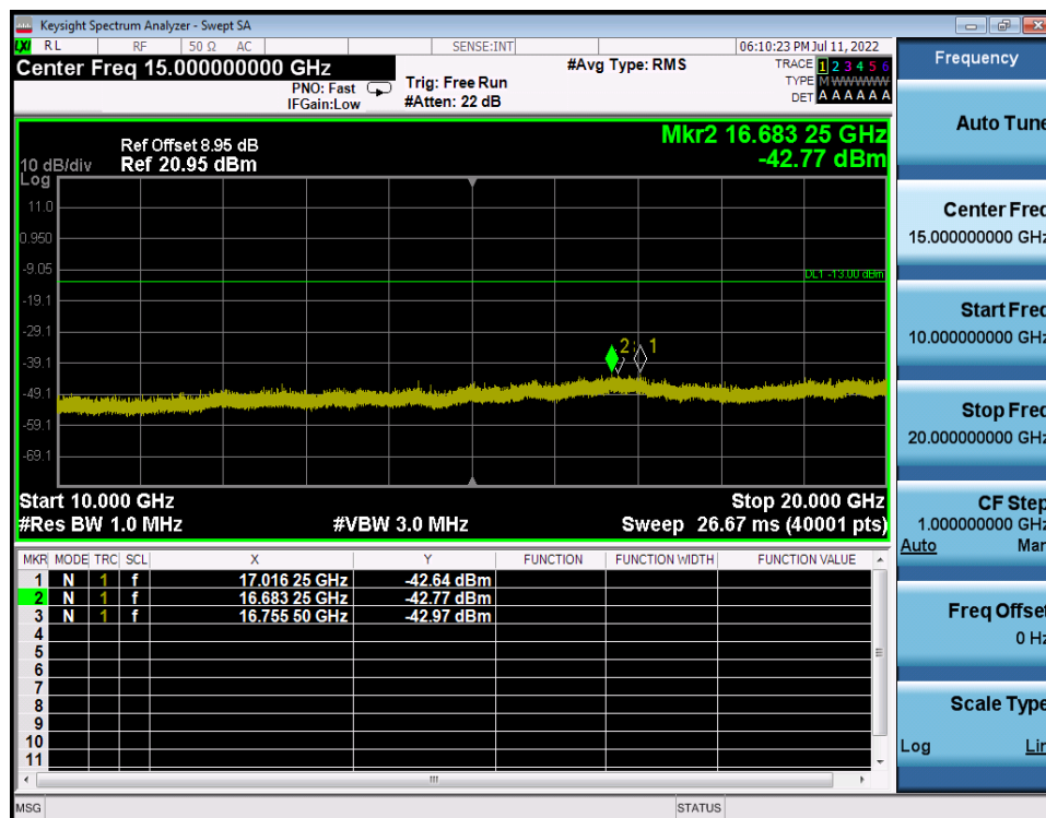
LTE Band 2 / 10MHz / QPSK - RB Size/Offset (25/0) - High Channel
