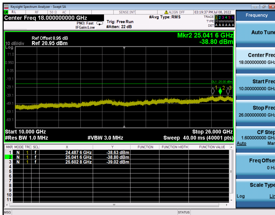
LTE Band 7 / 15MHz / 16QAM - RB Size/Offset (27/24) - Mid Channel
