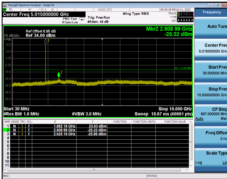
LTE Band 2 / 5MHz / QPSK - RB Size/Offset (12/13) - Mid Channel
