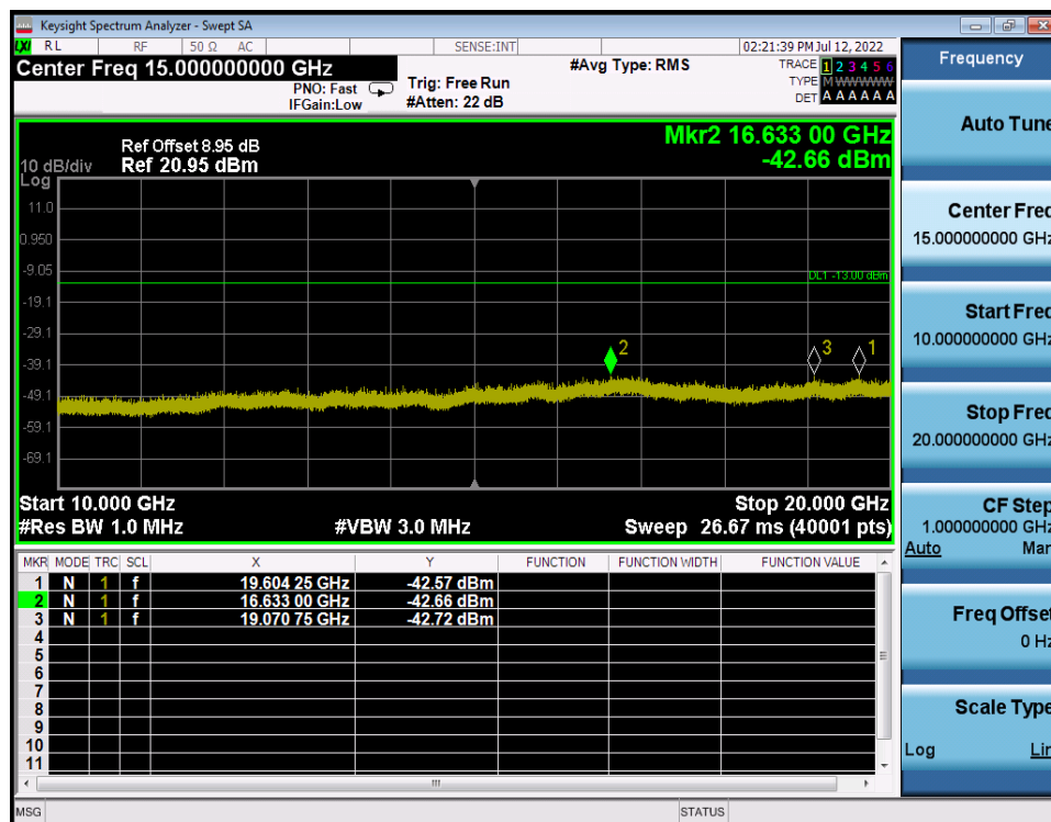
LTE Band 4 / 3MHz / 16QAM - RB Size/Offset (8/4) - Low Channel
