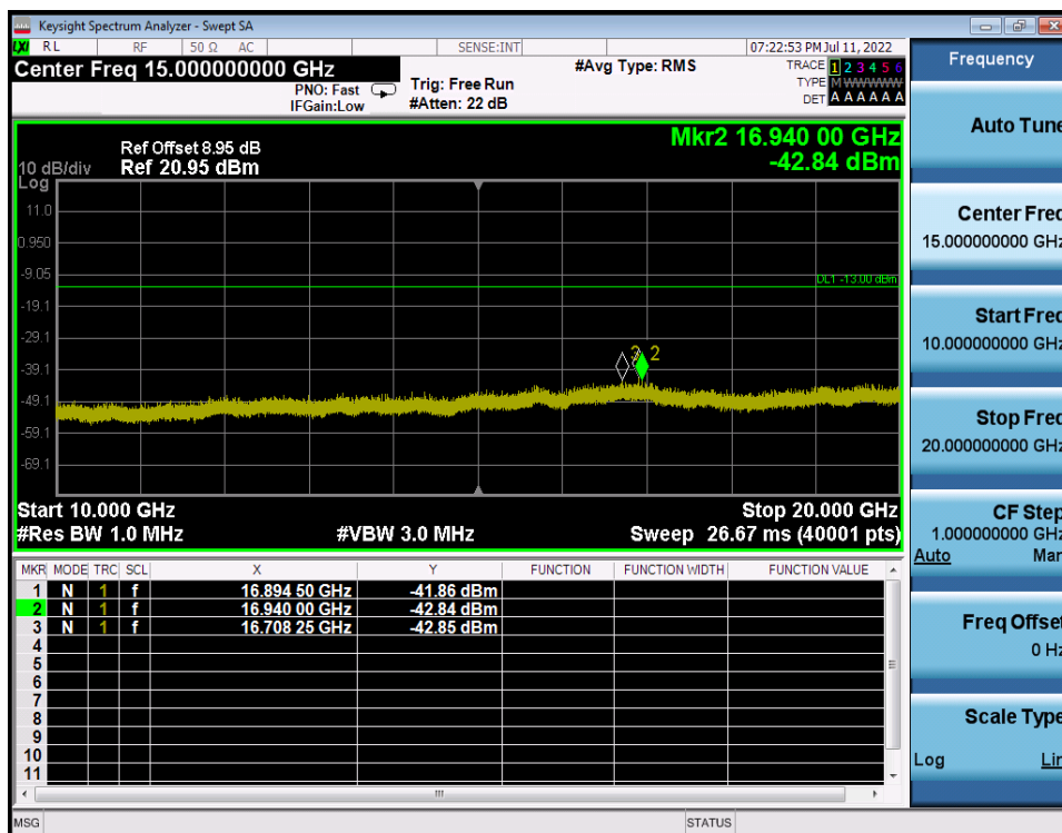
LTE Band 4 / 3MHz / QPSK - RB Size/Offset (1/7) - Mid Channel
