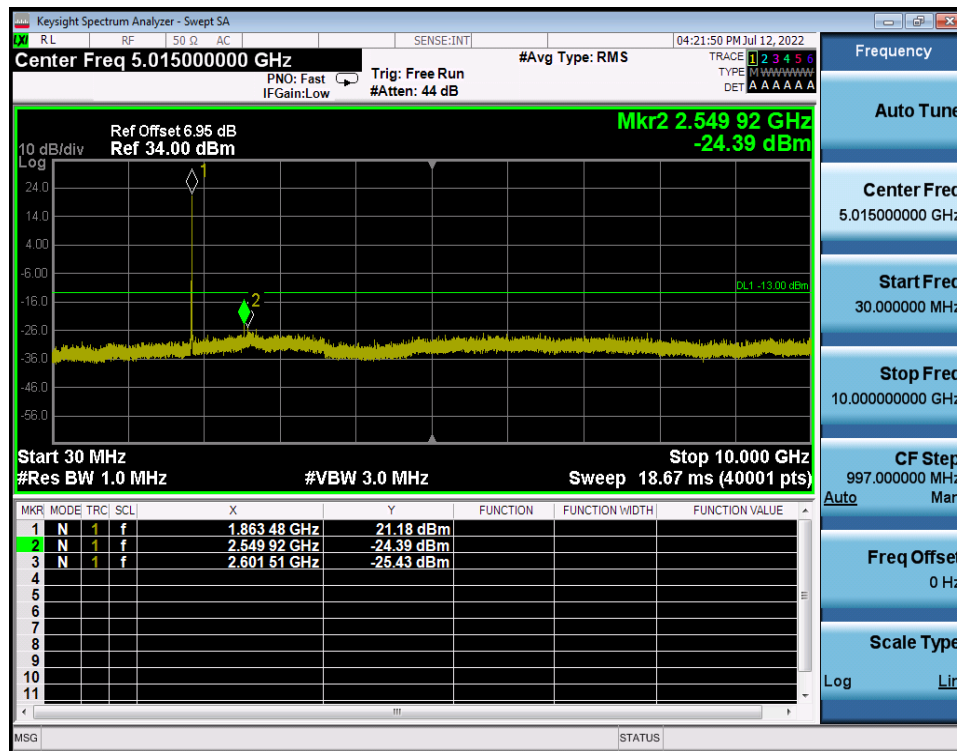
LTE Band 2 / 15MHz / 16QAM - RB Size/Offset (27/48) - Low Channel
