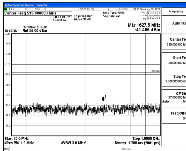
Band2-15MHz-QPSK-19125-1RB#0-Range4:1000~10000MHz
